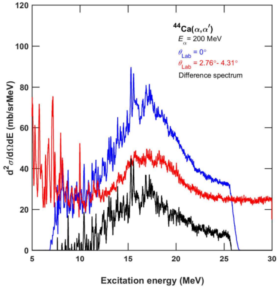
Figure 4.11: Same as Fig. 4.10 but for ^{44}\text{Ca}(\alpha, \alpha') . The 0^\circ - 2^\circ spectrum was scaled by a factor of 1.45.
