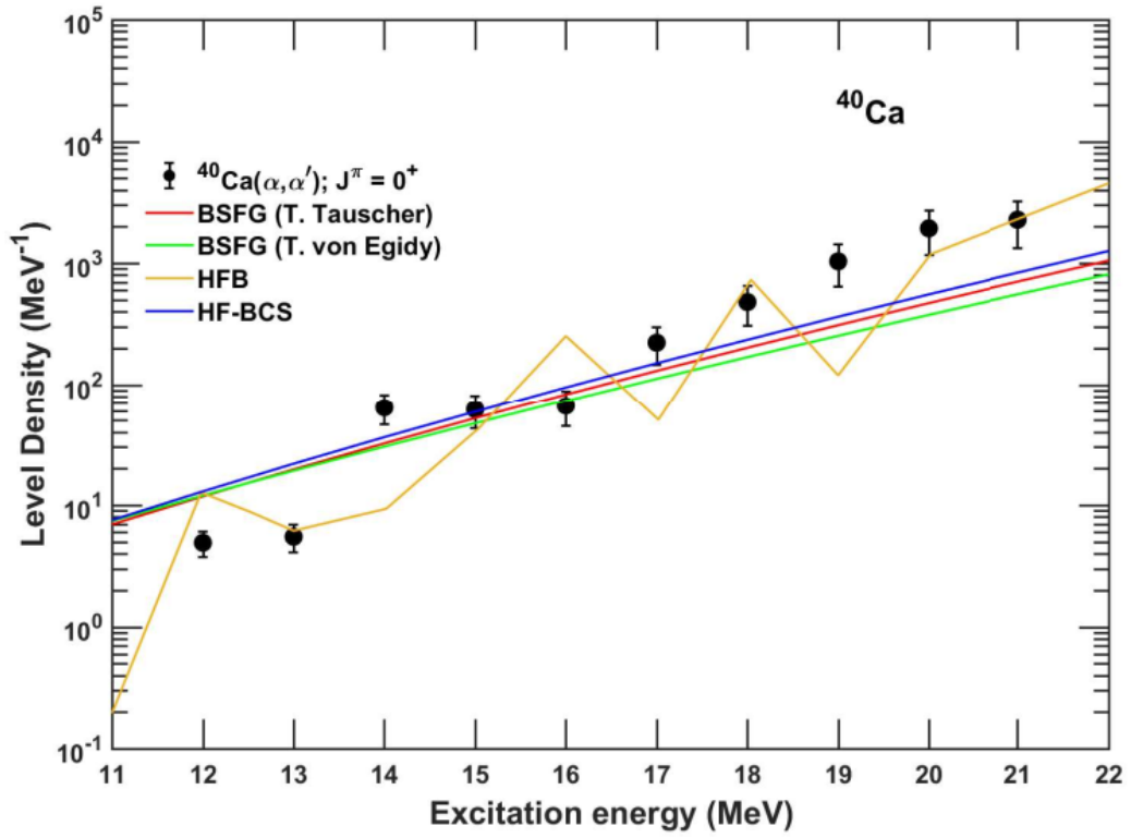
Figure 4.37: Level density of 0^+ states extracted from ^{40}\text{Ca}(\alpha, \alpha') and the theoretical models: BSFG of Ref. [Egi05] (green line), BSFG of Ref. [Rau97] (red line), HFB of Ref. [Hil06] (dark yellow line) and HF-BCS of Ref. [Dem01] (blue line).
