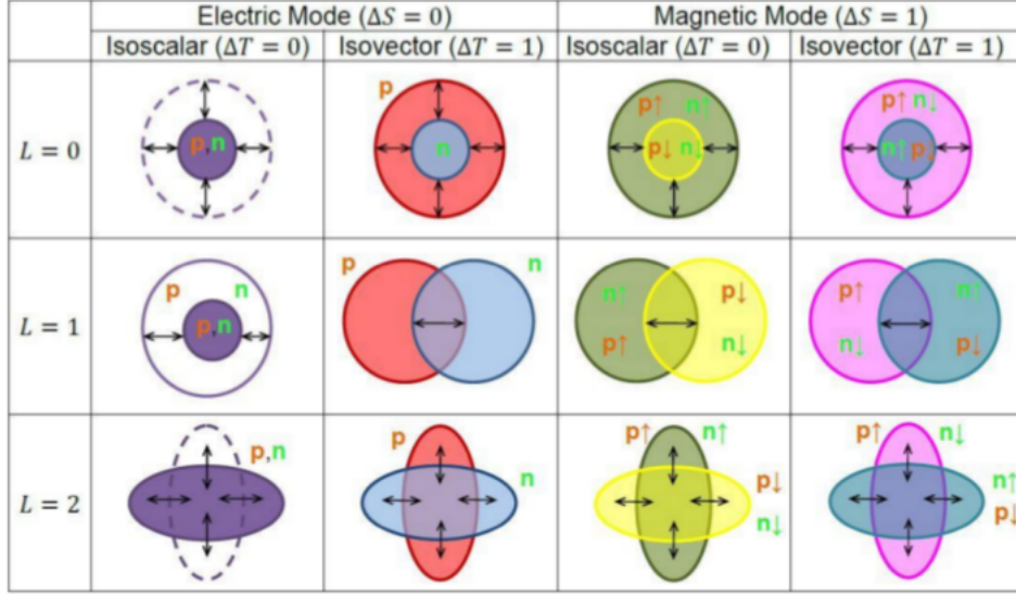
Figure 2.1: Schematic picture of various collective modes, taken from [Don16]
