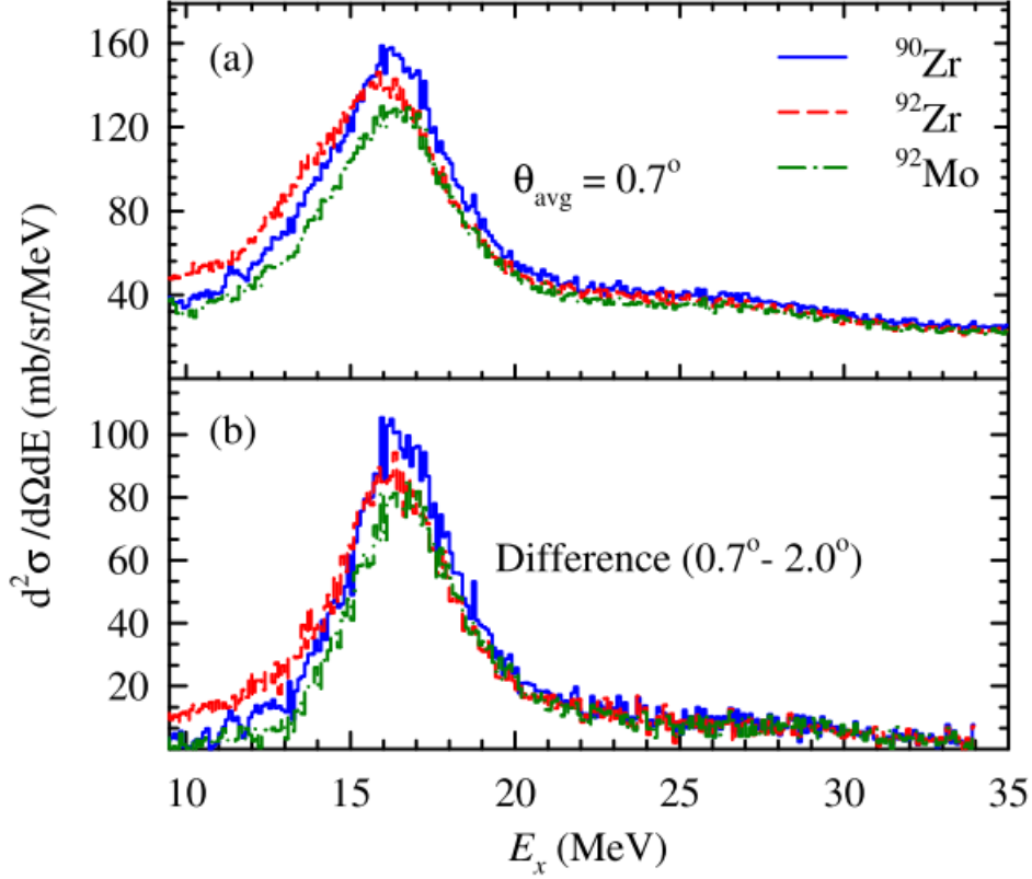
Figure 1.2: Upper: Double-differential cross sections measured at an averaged angle 0.7^\circ for ^{90}\text{Zr} , ^{92}\text{Zr} and ^{92}\text{Mo} . Lower: Difference spectra of average angles 0.7^\circ & 2.0^\circ for the same nuclei. Taken from [Gup16]
