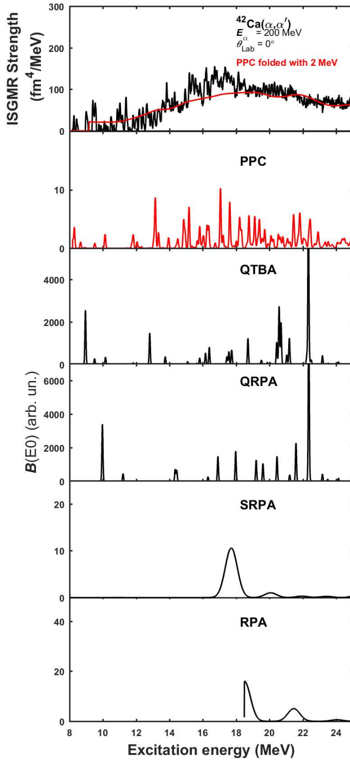
Figure 4.23: From top to bottom: ISGMR strength distribution for ^{42}\text{Ca}(\alpha, \alpha') overlaid with PPC result (in red) folded with 2 MeV; strength functions within the framework of PPC, QTBA, QRPA, SRPA and RPA.
