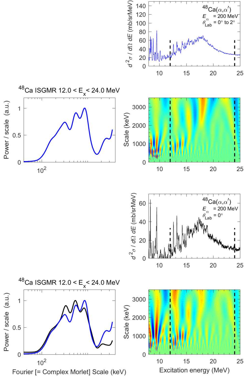
Figure 4.25: Top Segment: Experimental double-differential cross section for ^{48}\text{Ca}(\alpha, \alpha') at \theta_{\text{Lab}} = 0^\circ - 2^\circ (top right panel), wavelet coefficients from CWT (right panel on the second row down) and power spectrum (left panel on the second row down). Bottom segment: Difference spectrum for ^{48}\text{Ca}(\alpha, \alpha') (right panel on the third row down), wavelet coefficients from CWT (right panel on the lowest row) and corresponding power spectrum in black superimposed on power spectrum from \theta_{\text{Lab}} = 0^\circ data (left panel on the lowest row).
