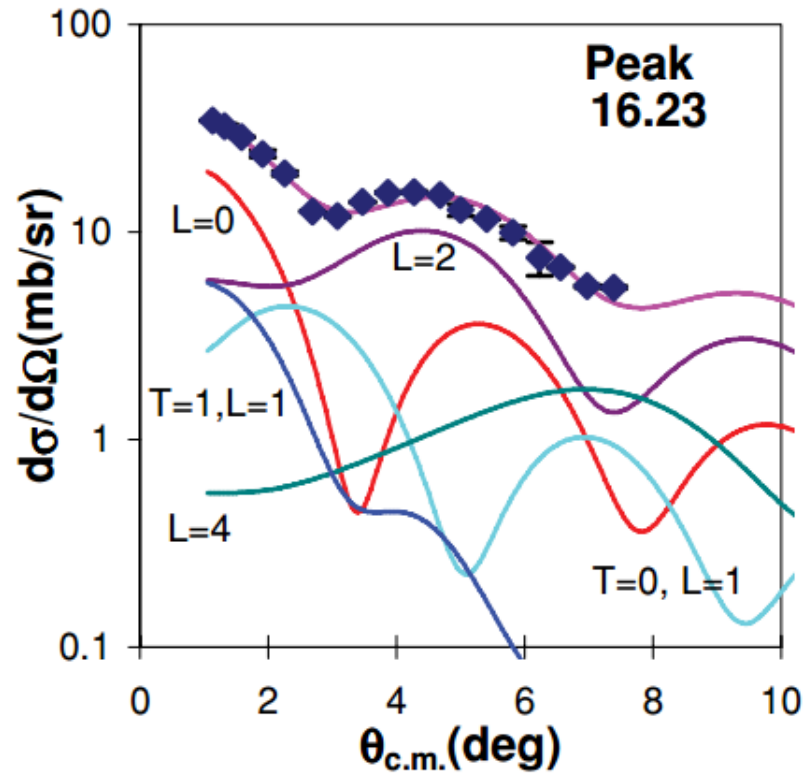
Figure 1.6: The angular distributions of the ^{48}\text{Ca} cross section at E_x = 16.23 MeV from the TAMU work. Taken from [Lui11].
