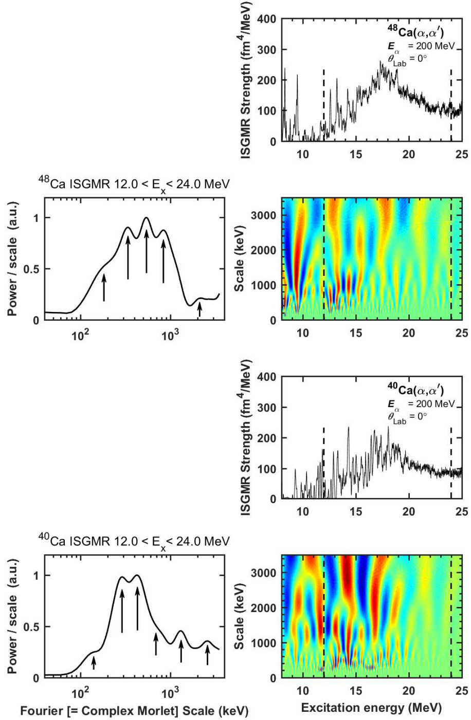
Figure 4.29: Top Segment: ISGMR strength distribution for ^{48}\text{Ca}(\alpha, \alpha') (top right panel), wavelet coefficients from CWT (right panel on the second row) and power spectrum (left panel on the second row). Bottom Segment: ISGMR strength distribution for ^{40}\text{Ca}(\alpha, \alpha') (right panel on the third row), wavelet coefficients from CWT (right panel on the last row) and power spectrum (left panel on the last row) with characteristic energy scales indicated by the black arrows. Excitation-energy region of 12 - 24 MeV was considered as indicated between the dashed black lines.
