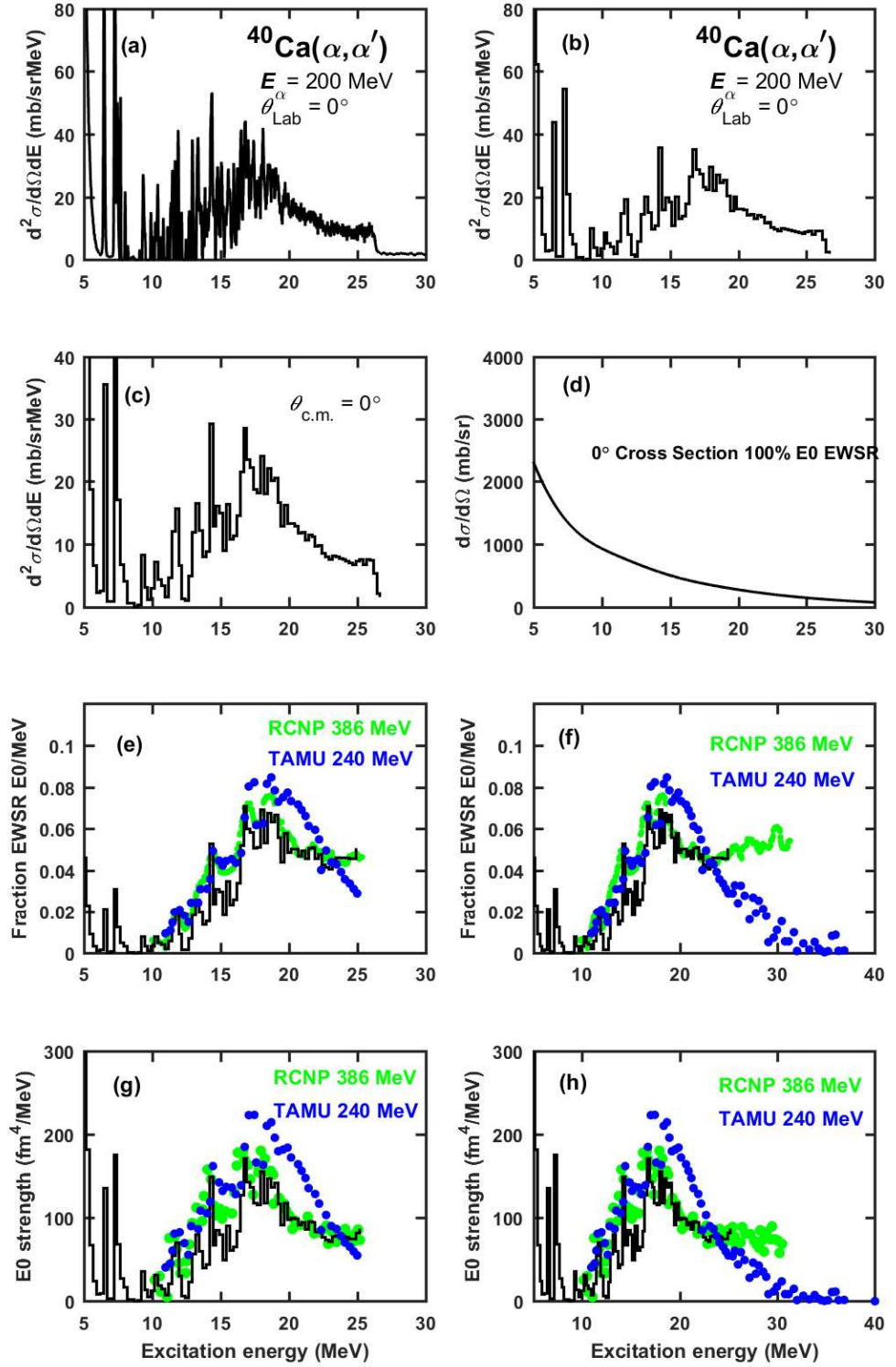
Figure 4.17: Same as Fig. 4.14 but for ^{40}\text{Ca}(\alpha, \alpha') .
