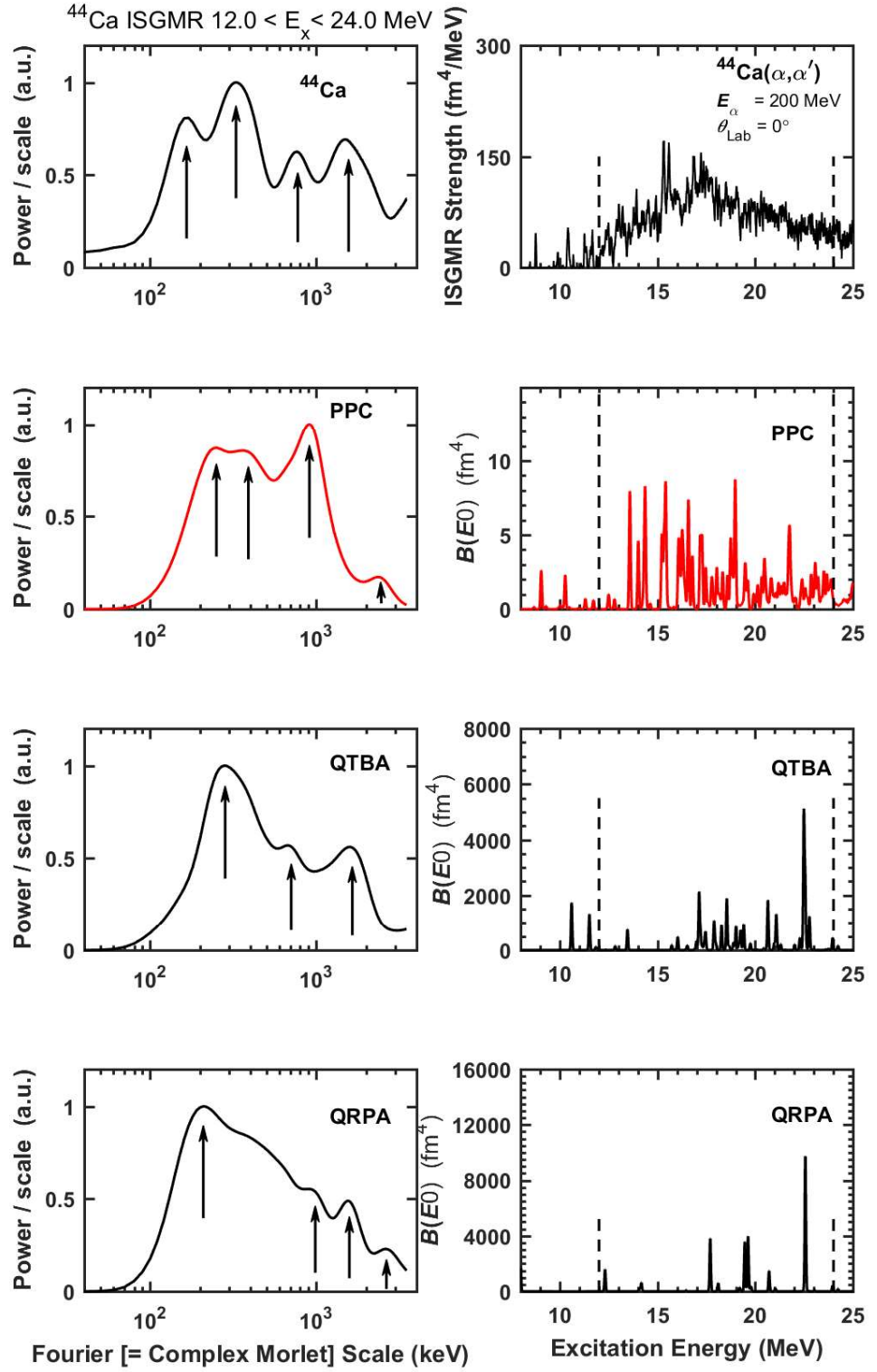
Figure 4.32: Same as Fig. 4.31 but for ^{44}\text{Ca}
