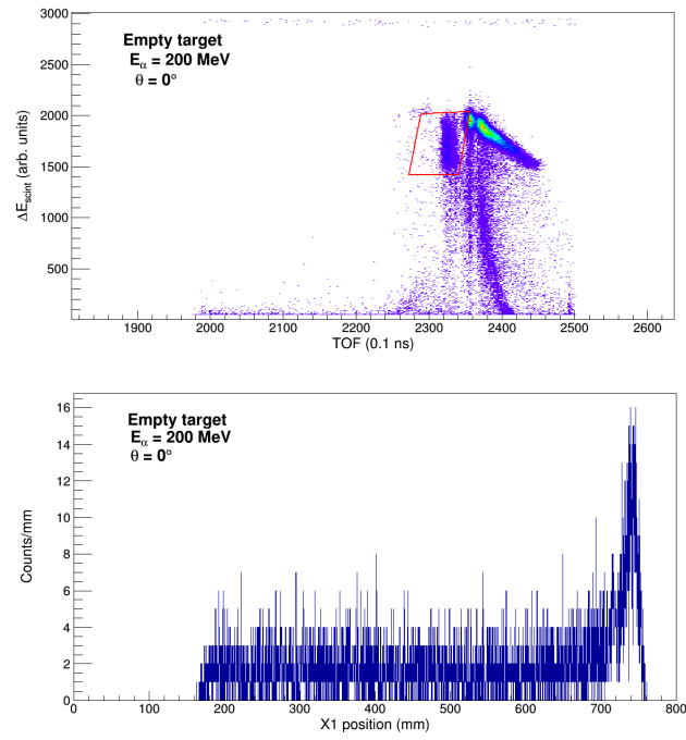
Figure 3.10: Top: Paddle1-versus-TOF PID plot for \alpha particles incident on an empty target showing the alpha PID gate. Bottom: Position spectrum for the empty obtained from the alpha PID software gate (marked in red).
