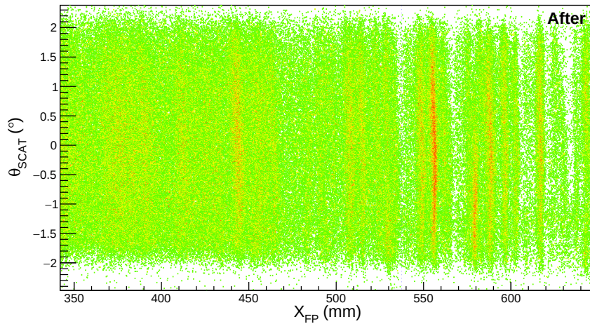
Figure 3.27: x_{\text{fp}} versus \theta_{\text{SCAT}} plot after the lineshape correction.
