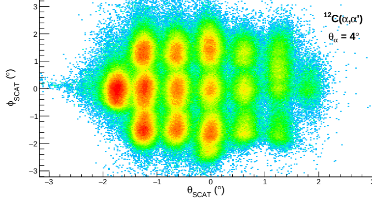
Figure 3.23: Calibrated horizontal and vertical scattering angle for the pepperpot collimator relative to \theta_{\text{K600}} = 4^{\circ} .
