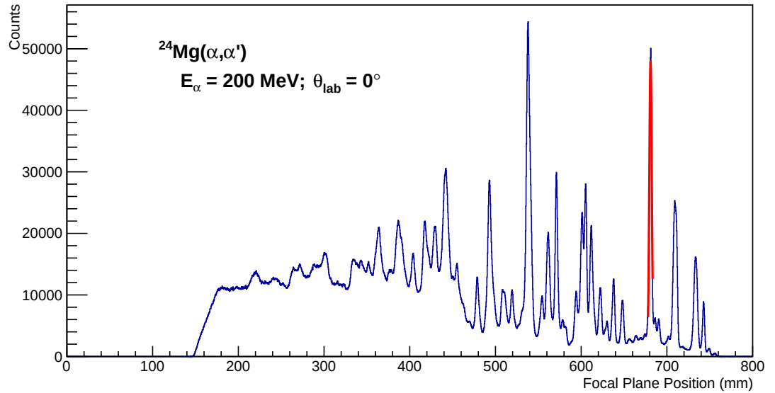
Figure 3.14: The lineshape-corrected and background-subtracted focal plane position spectrum for inelastic \alpha scattering from ^{24}\text{Mg} . The peak in red is the 9.305 MeV 0^+ state that was used to obtain the TOF and position offsets.
