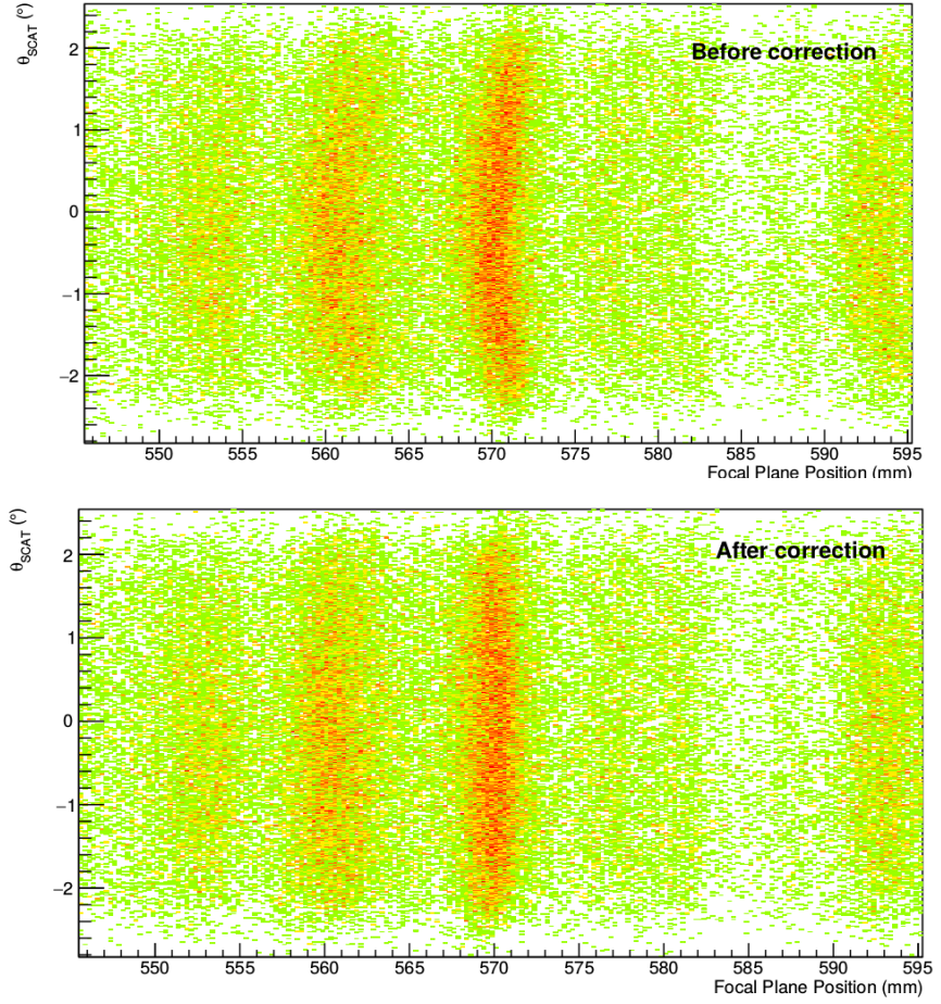
Figure 3.11: A plot of scattering angle versus the focal plane position (top) before and after (bottom) lineshape correction for ^{24}\text{Mg} .
