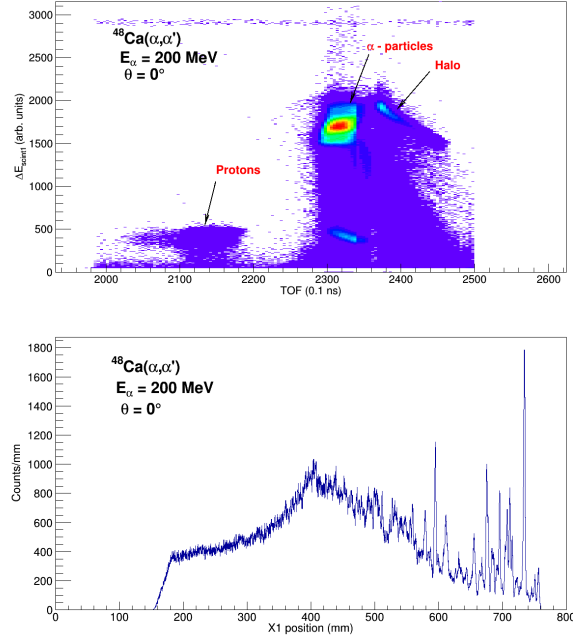
Figure 3.6: Top: A plot of energy deposited in paddle 1 versus TOF for \alpha particles incident on ^{48}\text{Ca} target showing various PID loci. Bottom: Position spectrum obtained from the \alpha PID gate.
