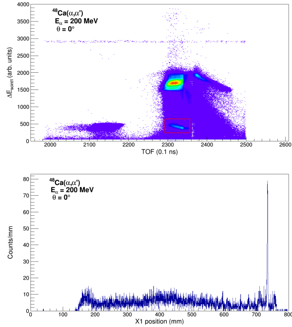
Figure 3.9: Top: Paddle1-versus-TOF PID plot for \alpha particles incident on a ^{48}\text{Ca} target showing the background below the alpha PID gate. Bottom: Position spectrum obtained from the background below the alpha PID gate.
