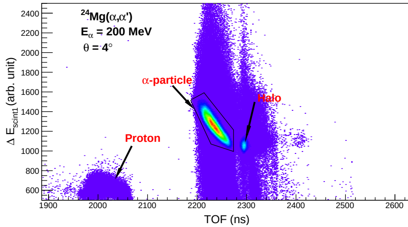
Figure 3.19: A plot of energy deposited in paddle 1 versus TOF for \alpha particles incident on a ^{24}\text{Mg} target showing various PID loci.
