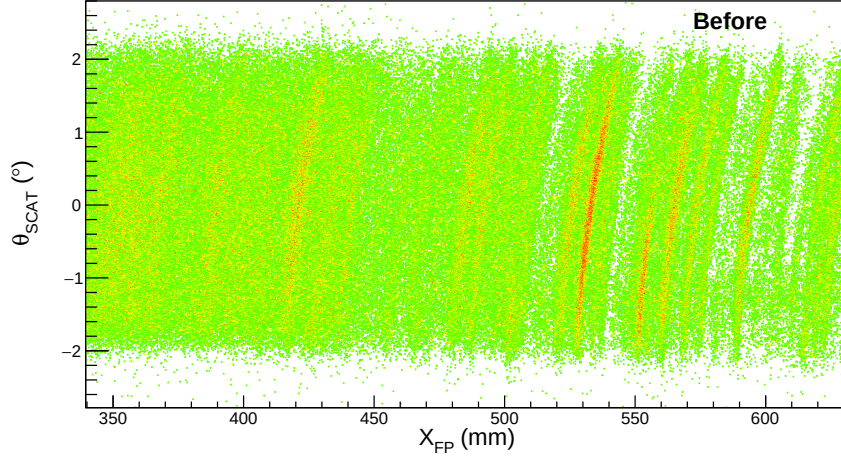
Figure 3.26: x_{\text{fp}} versus \theta_{\text{SCAT}} plot before the lineshape correction.
