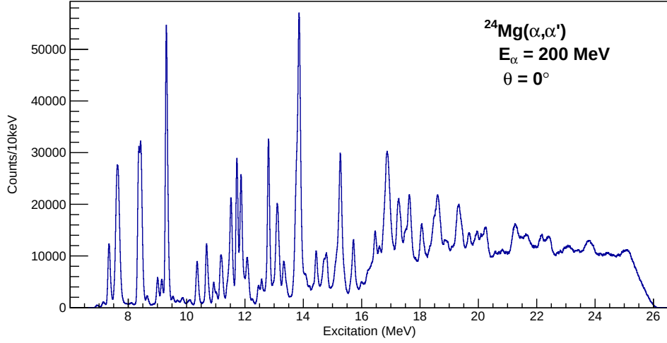
Figure 3.16: The ^{24}\text{Mg} excitation-energy spectrum accessible in the PR260 0^\circ measurements.
