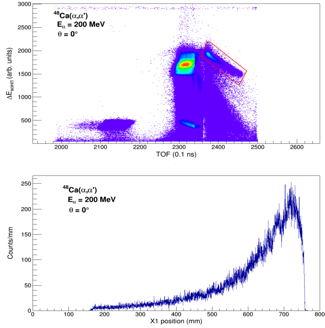
Figure 3.8: Top: Paddle1-versus-TOF PID plot for \alpha particles incident on ^{48}\text{Ca} target showing the beam halo PID gate. Bottom: Position spectrum obtained from the beam halo PID gate.
