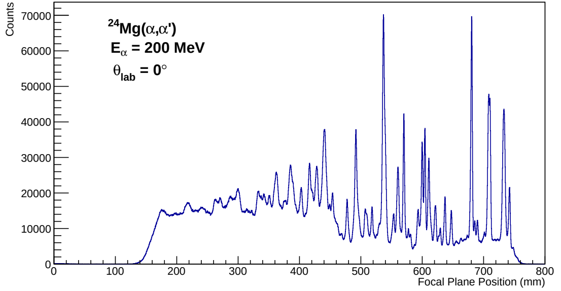
Figure 3.13: The focal plane position spectrum for inelastic \alpha scattering from ^{24}\text{Mg} target before the background subtraction.
