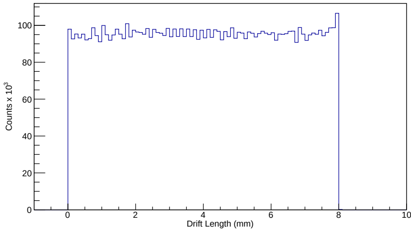
Figure 3.20: Drift length.
