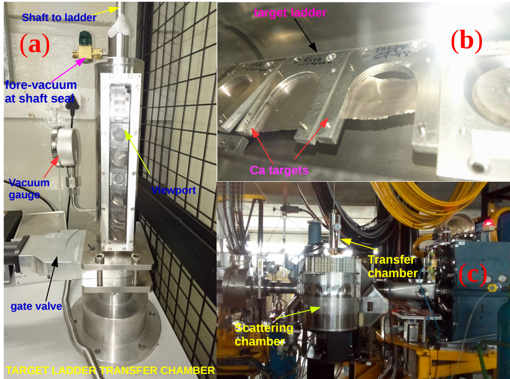
Figure 3.5: (a) Target-ladder-transfer chamber. (b) Ca targets mounted on the target-ladder inside the transfer chamber. (c) The transfer chamber mounted on the spectrometer scattering chamber.
