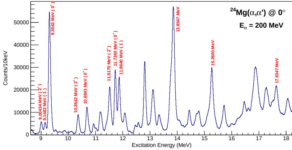
Figure 3.17: A magnified ^{24}\text{Mg} excitation-energy spectrum showing identified states used for the calibration. The energy resolution is 85.7 keV full width at half maximum (FWHM), based on the 9.305 MeV 0^+ state.
