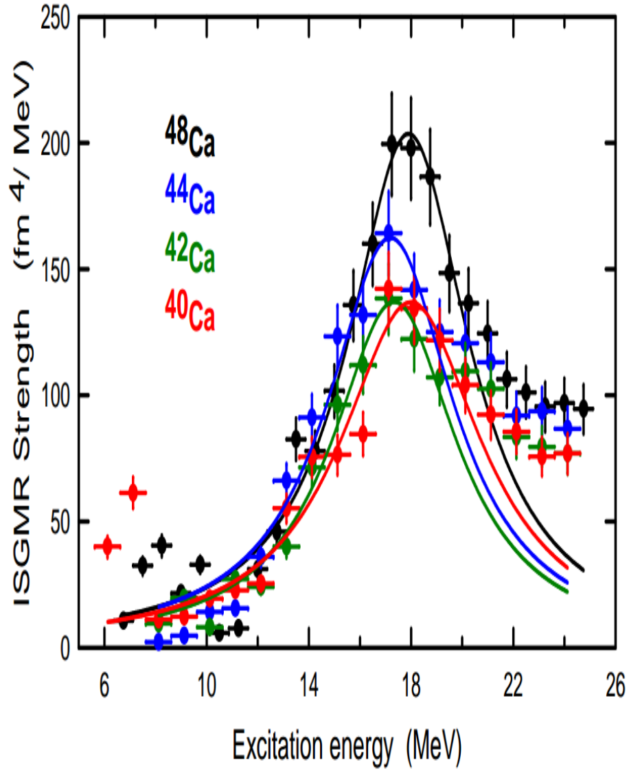
Figure 4.19: ISGMR strength distribution for ^{48}\text{Ca} (black circles), ^{44}\text{Ca} (blue circles), ^{42}\text{Ca} (green circles) and ^{40}\text{Ca} (red circles). The solid lines represent the Lorentzian fit.
