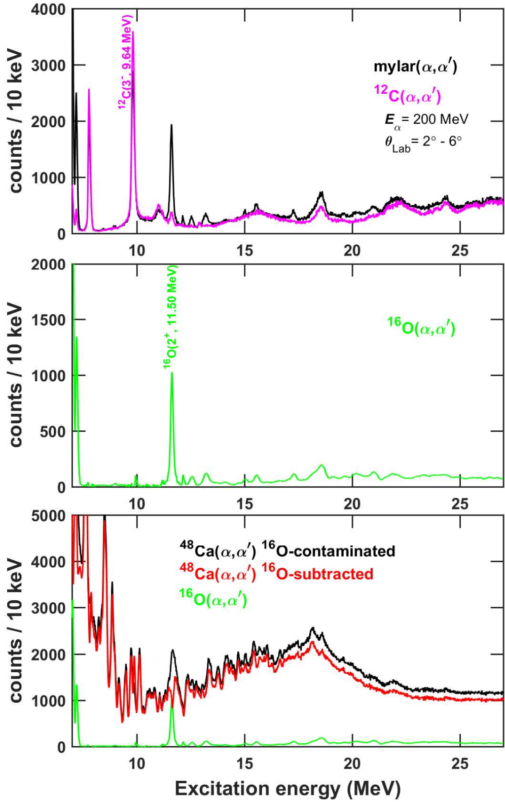
Figure 4.6: Panel (a): Mylar spectrum (black) with superimposed ^{12}\text{C} spectrum (magenta). Panel (b): Extracted ^{16}\text{O} spectrum. Panel (c): Spectra of oxygen-contaminated ^{48}\text{Ca} (black), extracted ^{16}\text{O} (green) and oxygen-free ^{48}\text{Ca} (red)
