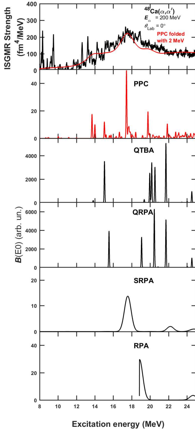
Figure 4.21: From top to bottom: ISGMR strength distribution for ^{48}\text{Ca}(\alpha, \alpha') overlaid with PPC result (in red) folded with 2 MeV; strength functions within the framework of PPC, QTBA, QRPA, SRPA and RPA.
