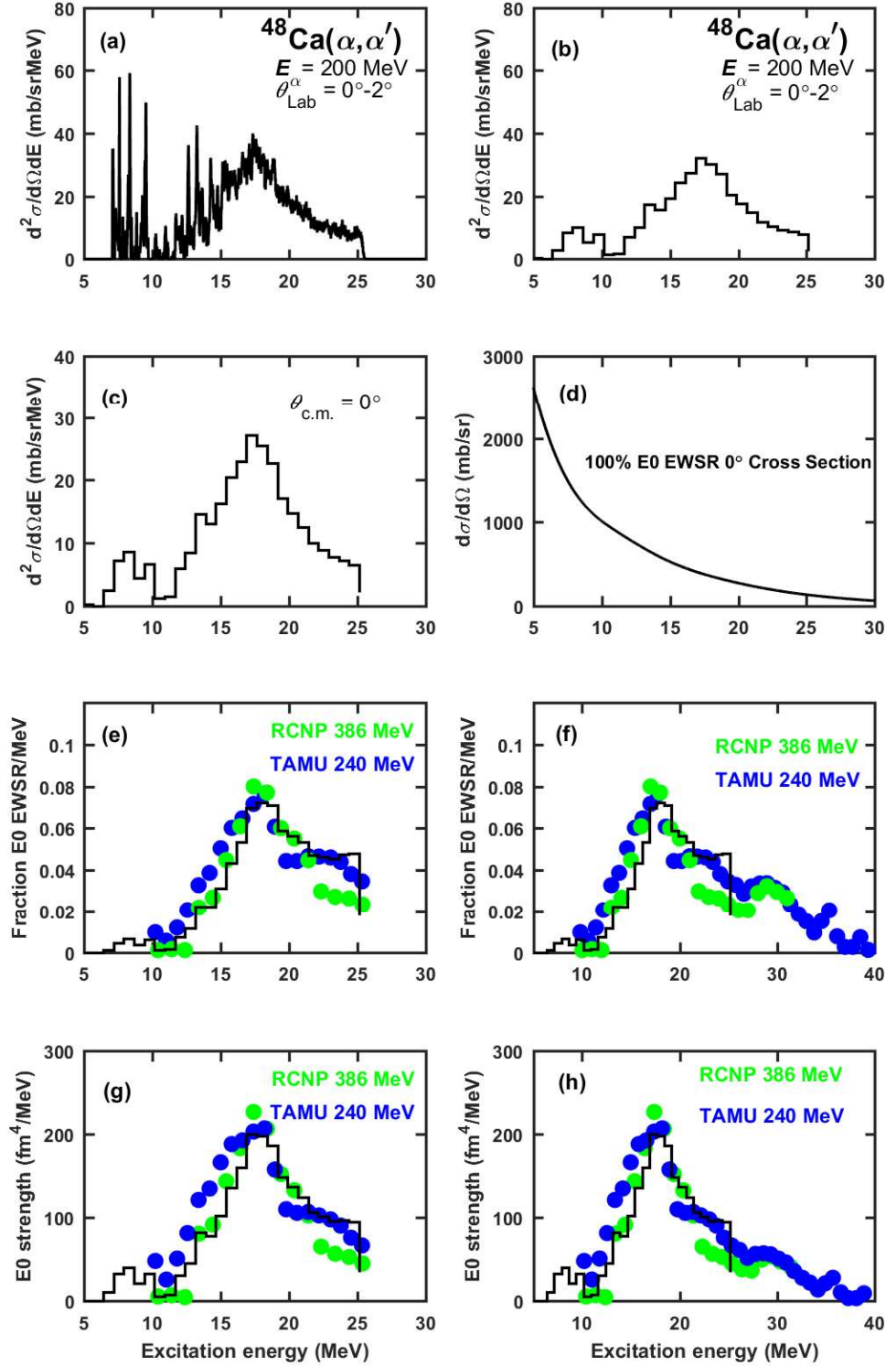
Figure 4.14: An outline of the conversion process from the double-differential cross section of ^{48}\text{Ca}(\alpha, \alpha') to fraction E0 EWSR per MeV and then to E0 strength distribution. See text for detailed explanation.
