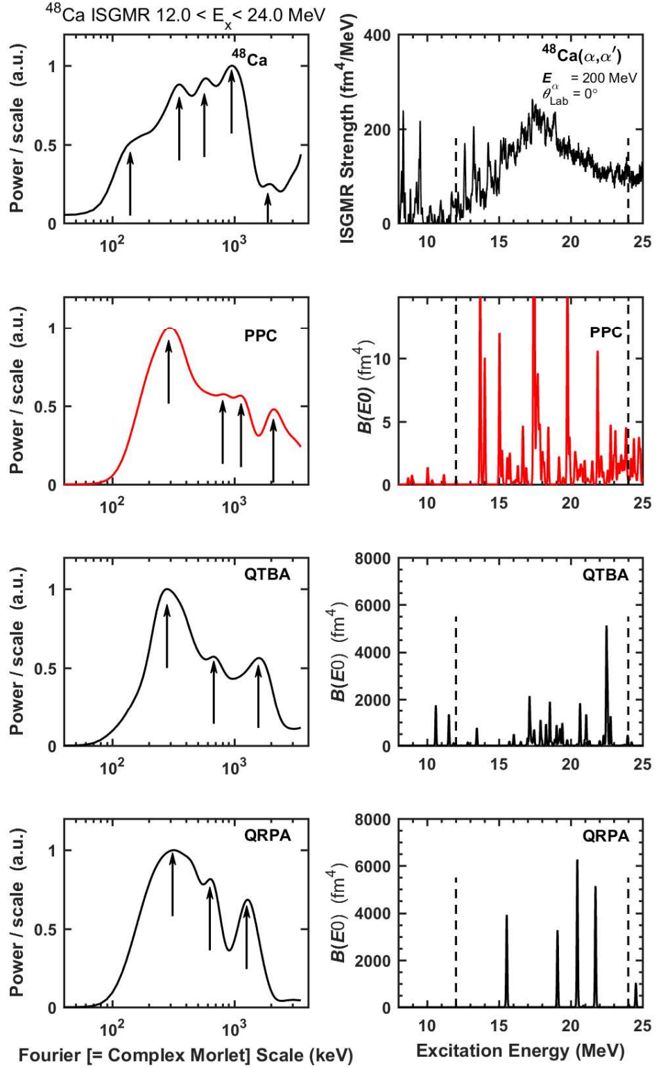
Figure 4.31: From top to bottom: On the right hand side is the ^{48}\text{Ca}(\alpha, \alpha') spectrum, the ^{48}\text{Ca} - PPC spectrum, the ^{48}\text{Ca} - QTBA spectrum and the ^{48}\text{Ca} - QRPA spectrum. On the left hand side are the corresponding power spectra with the characteristic scales pointed out with black arrows.
