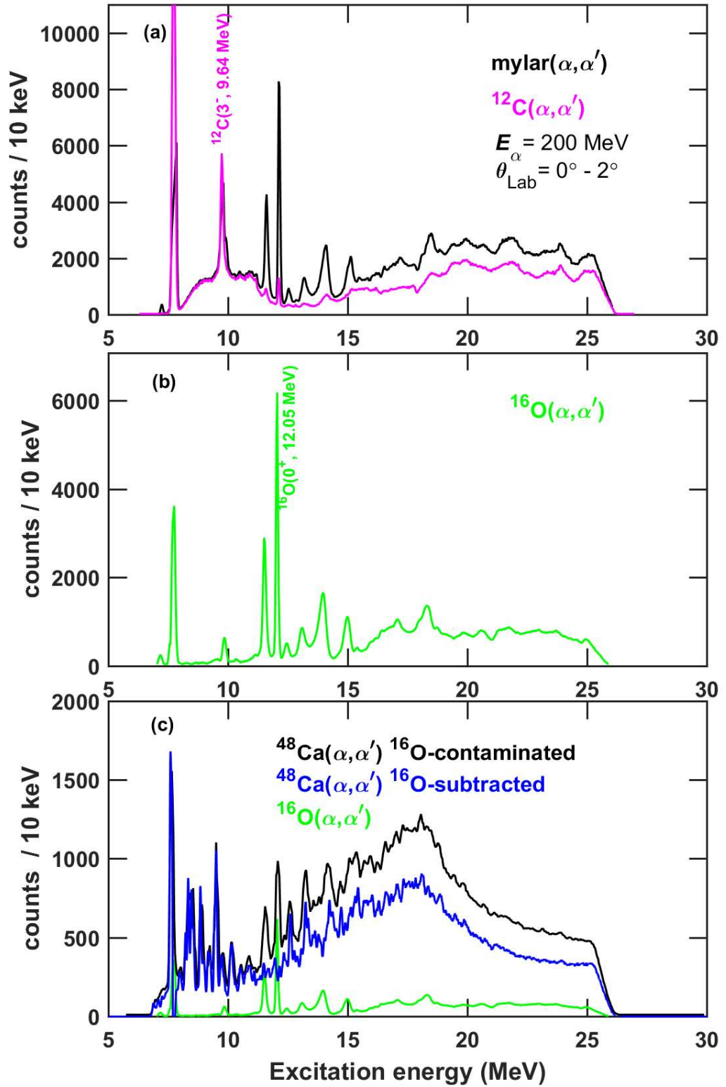
Figure 4.3: Panel (a): Mylar spectrum (black) with superimposed ^{12}\text{C} spectrum (magenta). Panel (b): Extracted ^{16}\text{O} spectrum. Panel (c): Spectra of oxygen-contaminated ^{48}\text{Ca} (black), extracted ^{16}\text{O} (green) and oxygen-free ^{48}\text{Ca} (blue).
