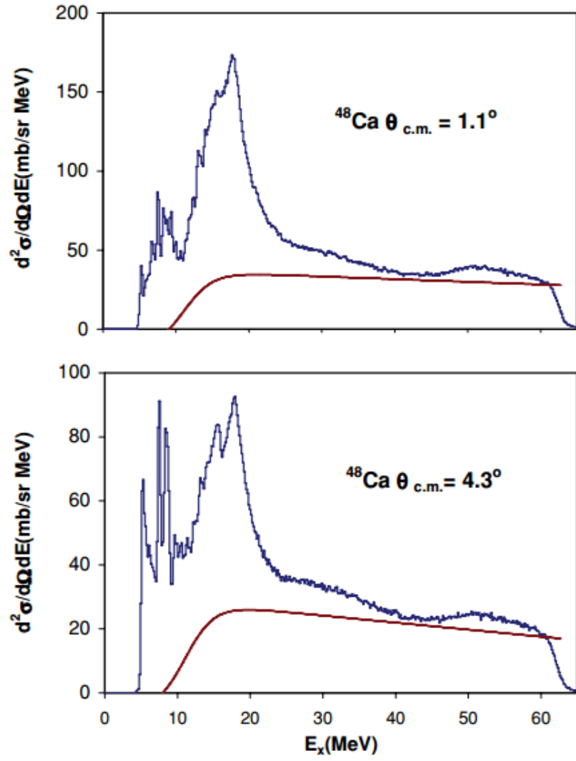
Figure 1.5: Inelastic alpha scattering spectra at E_\alpha = 240 MeV and \theta_{\text{c.m.}} = 1.1^\circ and 4.3^\circ for ^{48}\text{Ca} . Taken from [Lui11].
