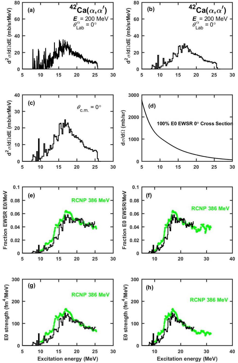
Figure 4.16: Same as Fig. 4.14 but for ^{42}\text{Ca}(\alpha, \alpha') .
