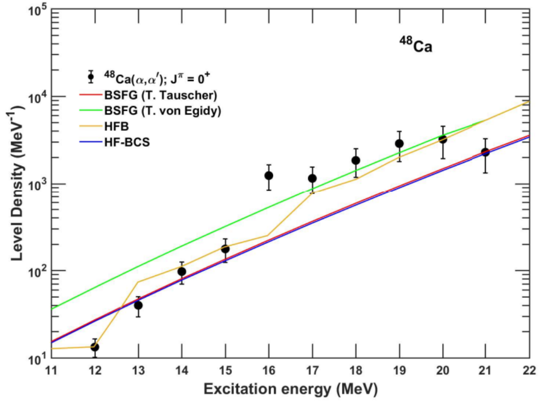
Figure 4.36: Level density of 0^+ states extracted from ^{48}\text{Ca}(\alpha, \alpha') and the theoretical models: BSFG of Ref. [Egi05] (green line), BSFG of Ref. [Rau97] (red line), HFB of Ref. [Hil06] (dark yellow line) and HF-BCS of Ref. [Dem01] (blue line).
