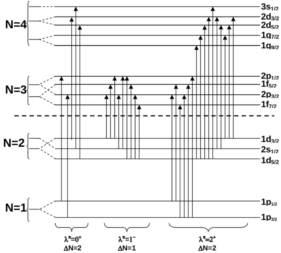
Figure 2.2: Schematic representation of E0 , E1 and E2 single-particle transitions between shell-model states, taken from [She04].
