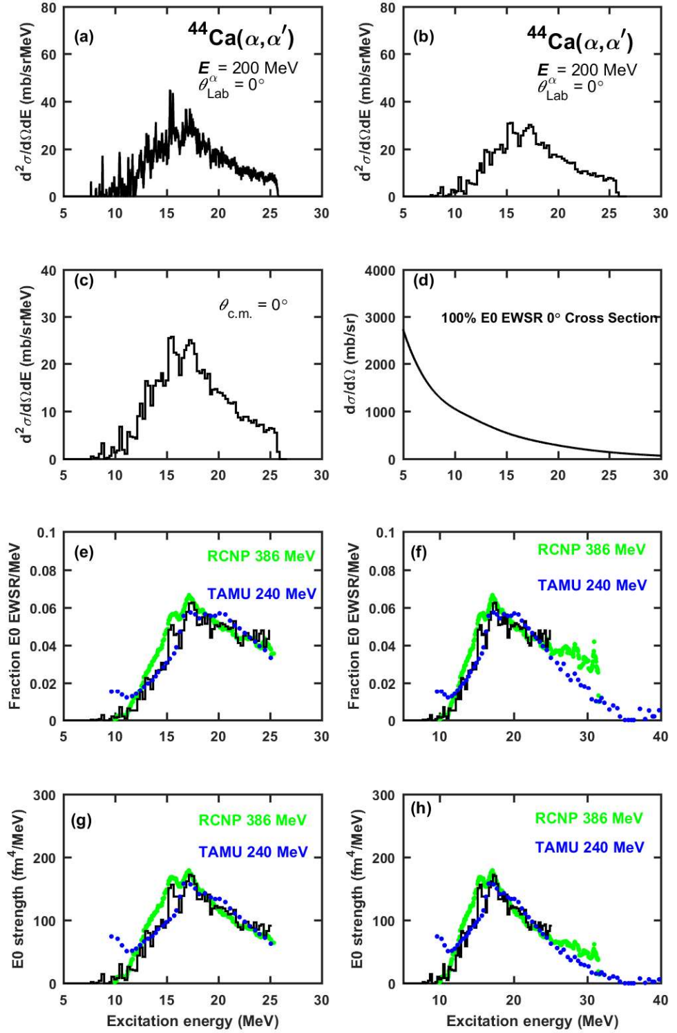
Figure 4.15: Same as Fig. 4.14 but for ^{44}\text{Ca}(\alpha, \alpha') .
