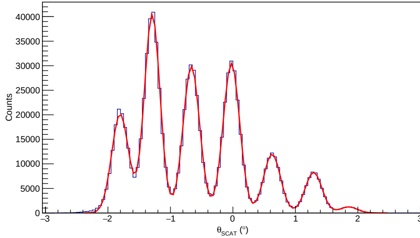
Figure 3.22: The resultant scattering angle \theta_{\text{SCAT}} plot for the pepperpot run 2022 at x_{\text{fp}} = 613 mm which illustrates the reconstructed scattering angle relative to \theta_{\text{K600}} .
