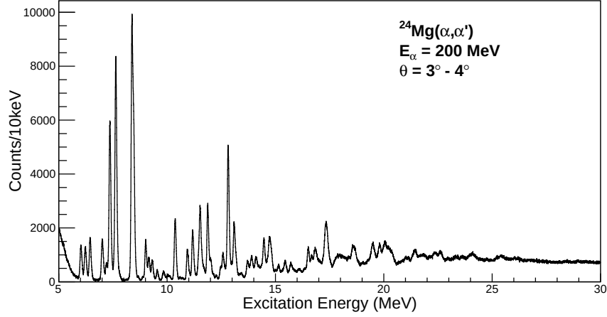
Figure 3.28: Measured excitation energy spectrum for the ^{24}\text{Mg}(\alpha, \alpha') reaction, used for energy calibration.
