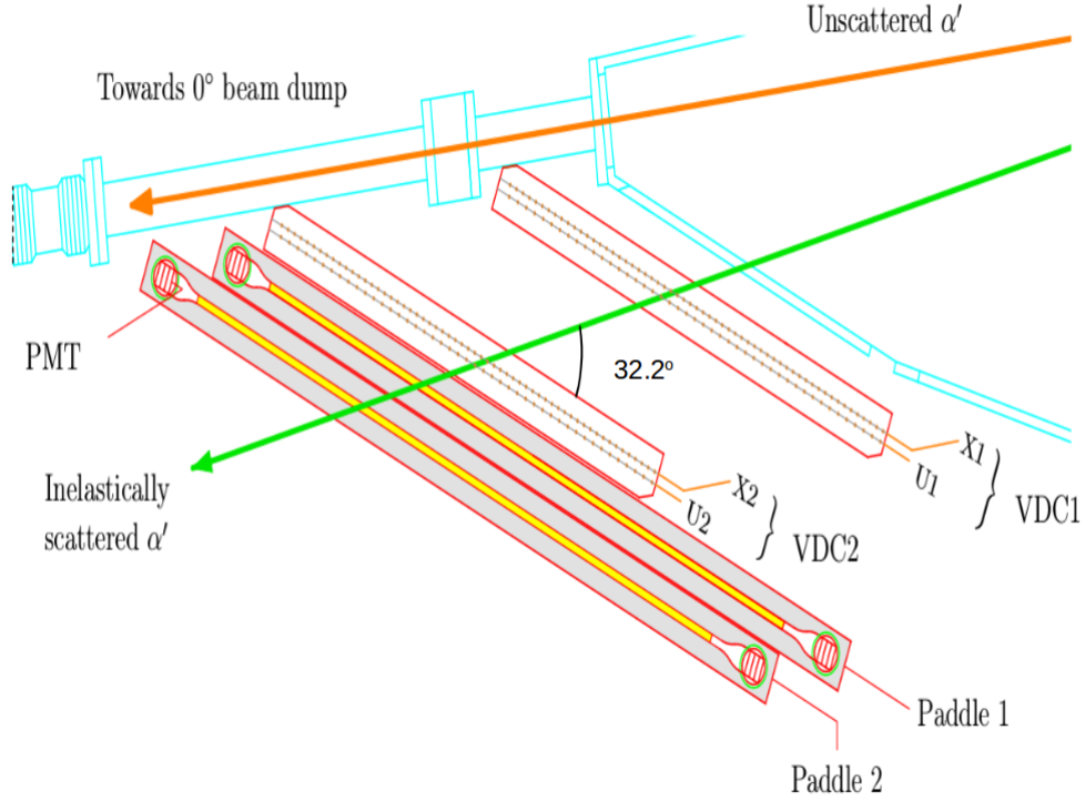
Figure 3.3: A schematic view of the focal plane detectors.
