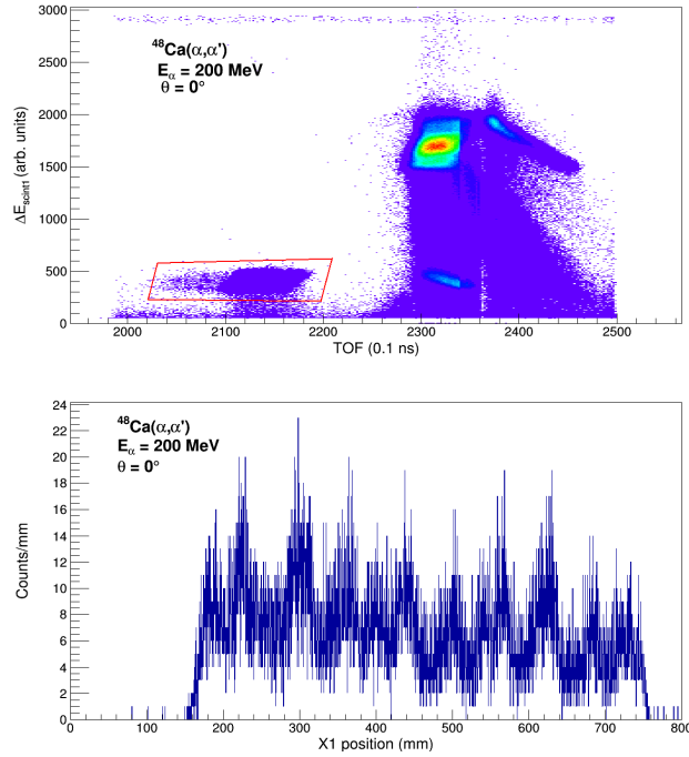
Figure 3.7: Top: Paddle1-versus-TOF PID plot for \alpha particles incident on ^{48}\text{Ca} target showing the proton PID gate. Bottom: Position spectrum obtained from the proton PID gate.
