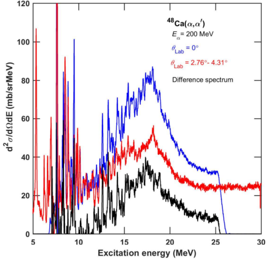
Figure 4.10: Double-differential cross section for ^{48}\text{Ca}(\alpha, \alpha') at E_\alpha = 200 MeV. The blue spectrum is for 0^\circ \leq \theta_{\text{Lab}} \leq 2^\circ (see Fig. 4.5), the red is for 2.76^\circ \leq \theta_{\text{Lab}} \leq 4.31^\circ (which correspond to 3^\circ \leq \theta_{\text{c.m.}} \leq 4.5^\circ , see angle region shown in Fig. 4.9 and is cut from the ^{48}\text{Ca} spectrum shown in Fig. 4.8) and the black is the difference spectrum obtained by subtracting the 2.76^\circ - 4.31^\circ spectrum (red) from the 0^\circ spectrum (blue). Note that the 0^\circ - 2^\circ spectrum was scaled by a factor of 1.32 in order to make the cross-section equivalent to that which would be measured at \theta_{\text{Lab}} = 0^\circ .
