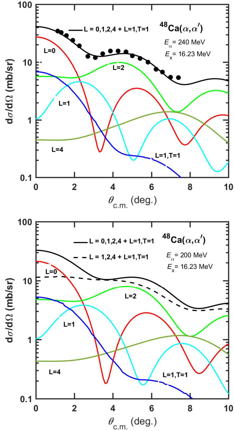
Figure 4.9: Angular distributions of the differential cross-sections for inelastic alpha particle scattering on ^{48}\text{Ca} at E_x = 16.23 MeV and at E_\alpha = 240 MeV (upper panel) and E_\alpha = 200 MeV (lower panel) for L = 0, 1, 2, 4 and L = 1, T = 1 . The black dashed line represent the sum of L = 1, 2, 4 and L = 1, T = 1 , while the solid black line represents the sum of all the multipoles shown. Note that the data shown in the upper panel are from Lui et al. [Lui11].
