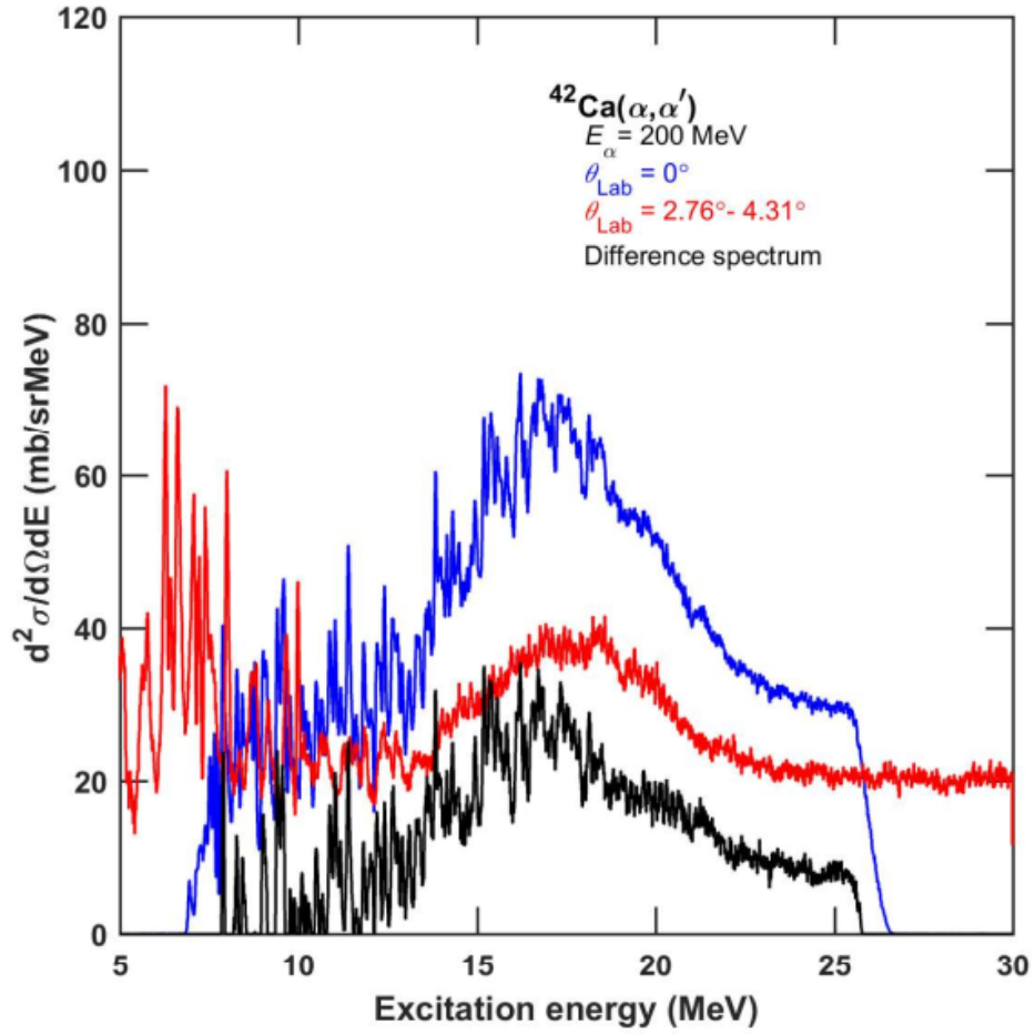
Figure 4.12: Same as Fig. 4.10 but for ^{42}\text{Ca}(\alpha, \alpha') . The 0^\circ - 2^\circ spectrum was scaled by a factor of 1.33.
