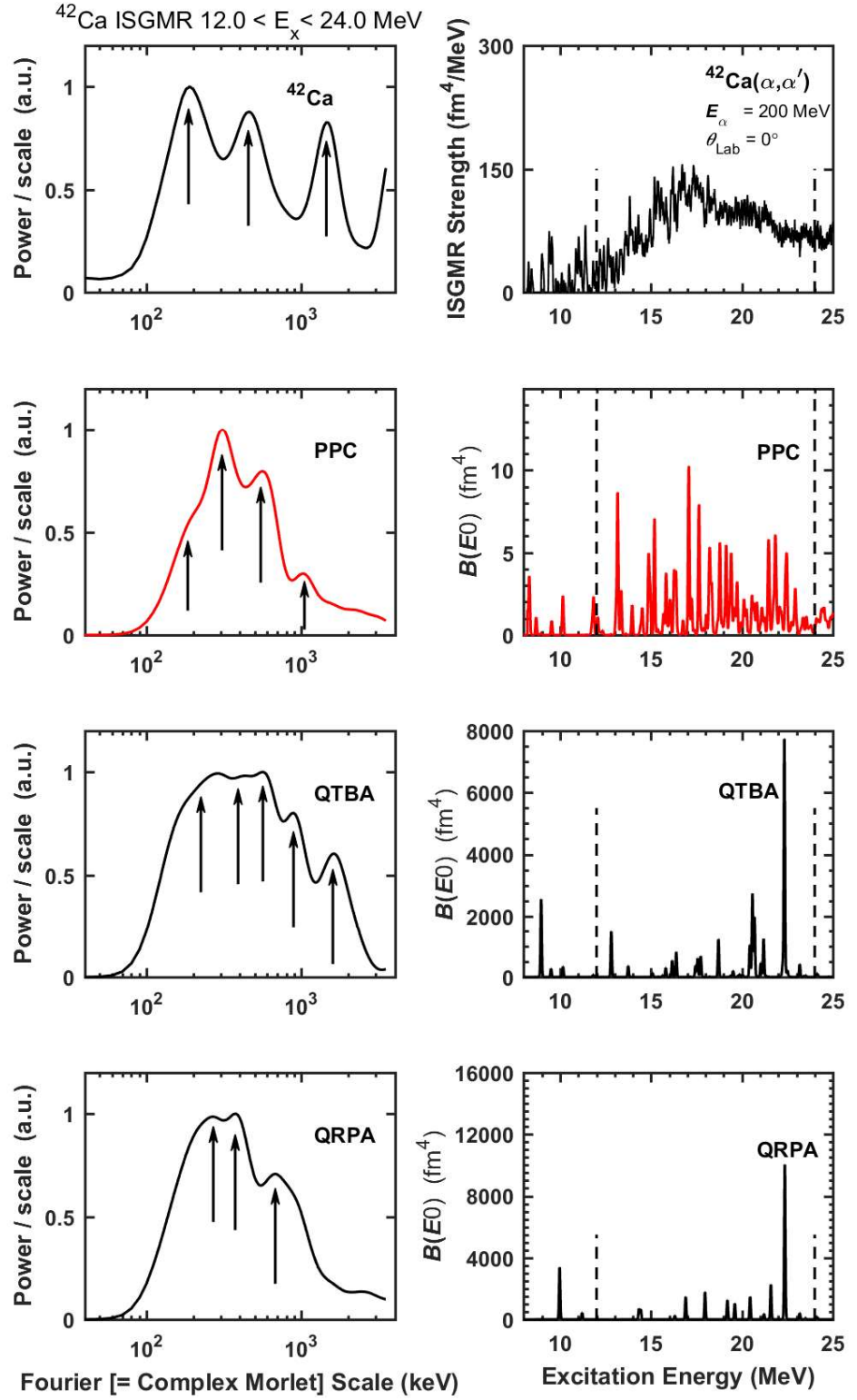
Figure 4.33: Same as Fig. 4.31 but for ^{42}\text{Ca}
