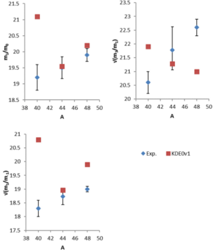
Figure 1.4: Experimental results for the ISGMR energies in ^{40}\text{Ca} [You97], ^{44}\text{Ca} [But17], and ^{48}\text{Ca} [Lui11] (blue diamonds) are compared with theoretical predictions (red squares). Here, \sqrt{m_1/m_{-1}} (left panel down), m_1/m_0 (top left panel) and \sqrt{m_3/m_1} (top right panel) are the constrained energy, centroid energy and scaling energy, respectively. Taken from [But17].
