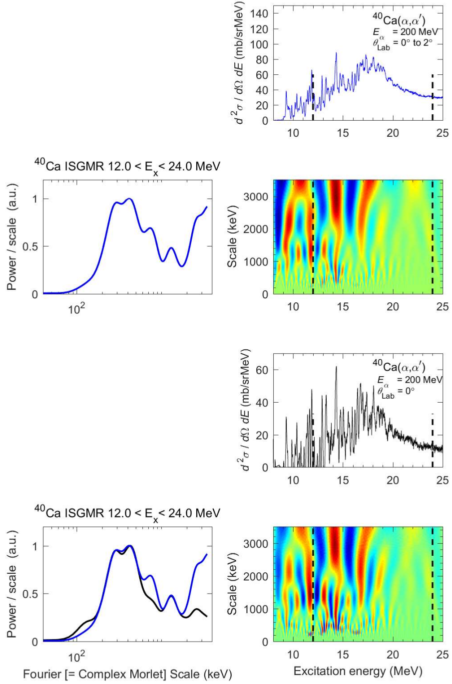
Figure 4.28: Same as Fig 4.25, but for ^{40}\text{Ca} .
