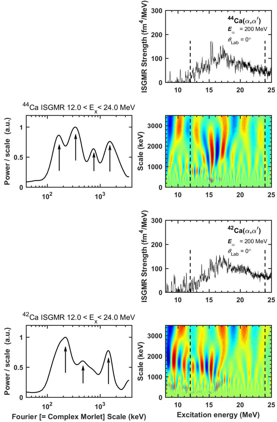
Figure 4.30: Same as Fig 4.29, but for ^{44}\text{Ca} and ^{42}\text{Ca} .
