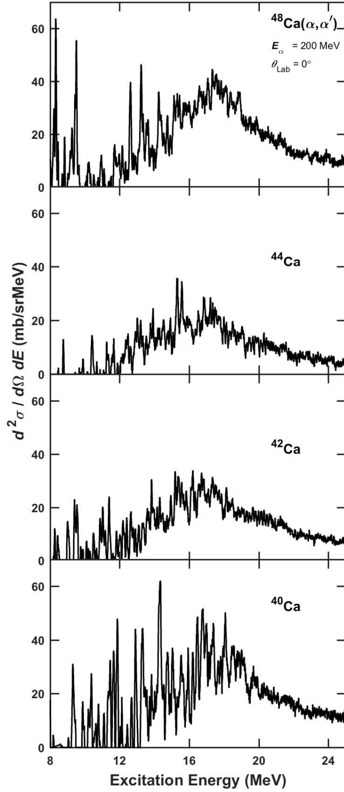
Figure 4.18: Double-differential cross section of the difference spectra for ^{40,42,44,48}\text{Ca} at E_\alpha = 200 MeV.
