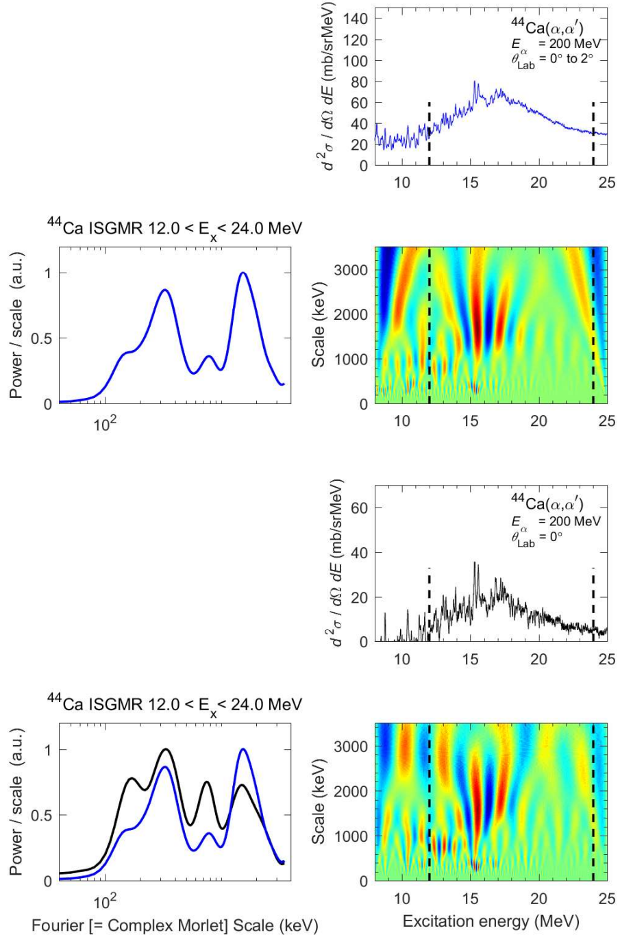
Figure 4.26: Same as Fig 4.25, but for ^{44}\text{Ca} .
