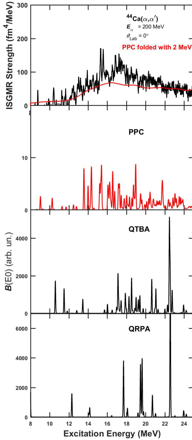
Figure 4.22: From top to bottom: ISGMR strength distribution for ^{44}\text{Ca}(\alpha, \alpha') overlaid with PPC result (in red) folded with 2 MeV; strength functions within the framework of PPC, QTBA and QRPA.
