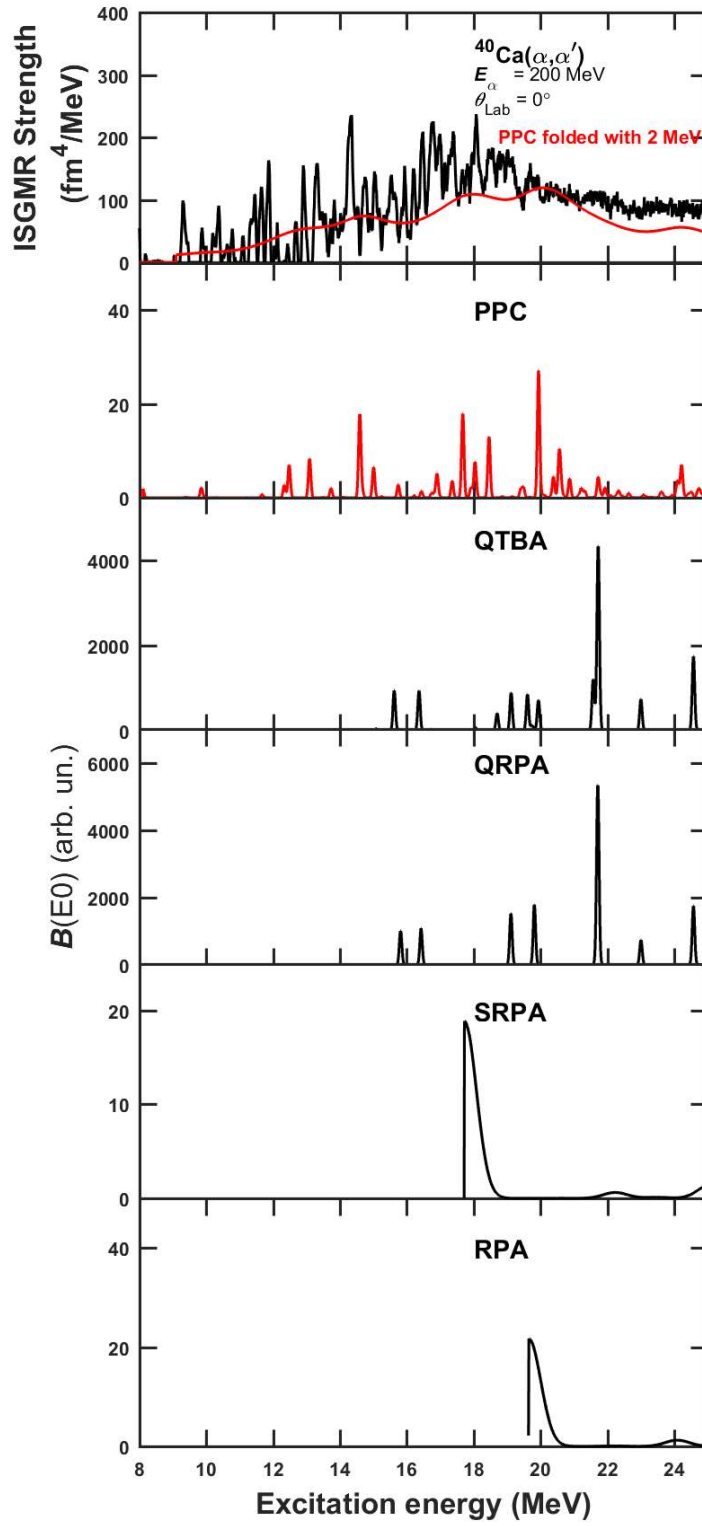
Figure 4.24: From top to bottom: ISGMR strength distribution for ^{40}\text{Ca}(\alpha, \alpha') overlaid with PPC result (in red) folded with 2 MeV; strength functions within the framework of PPC, QTBA, QRPA, SRPA and RPA.
