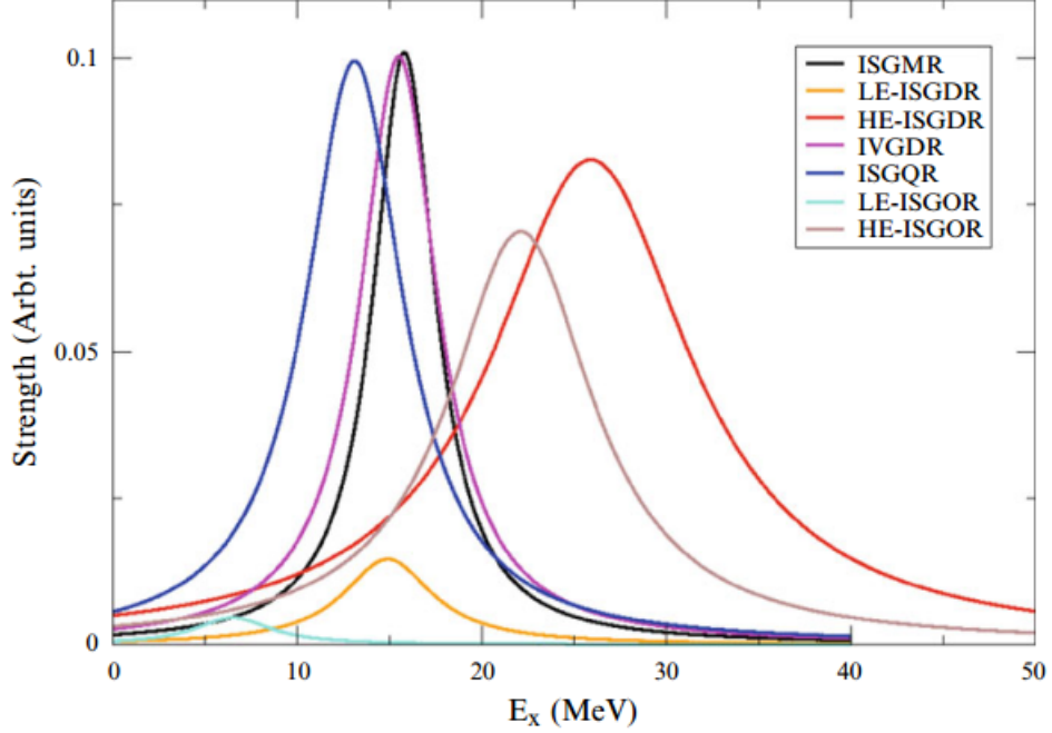
Figure 1.1: Notional strength distributions for various giant resonances overlapping in excitation energy. Taken from [Pat15].
