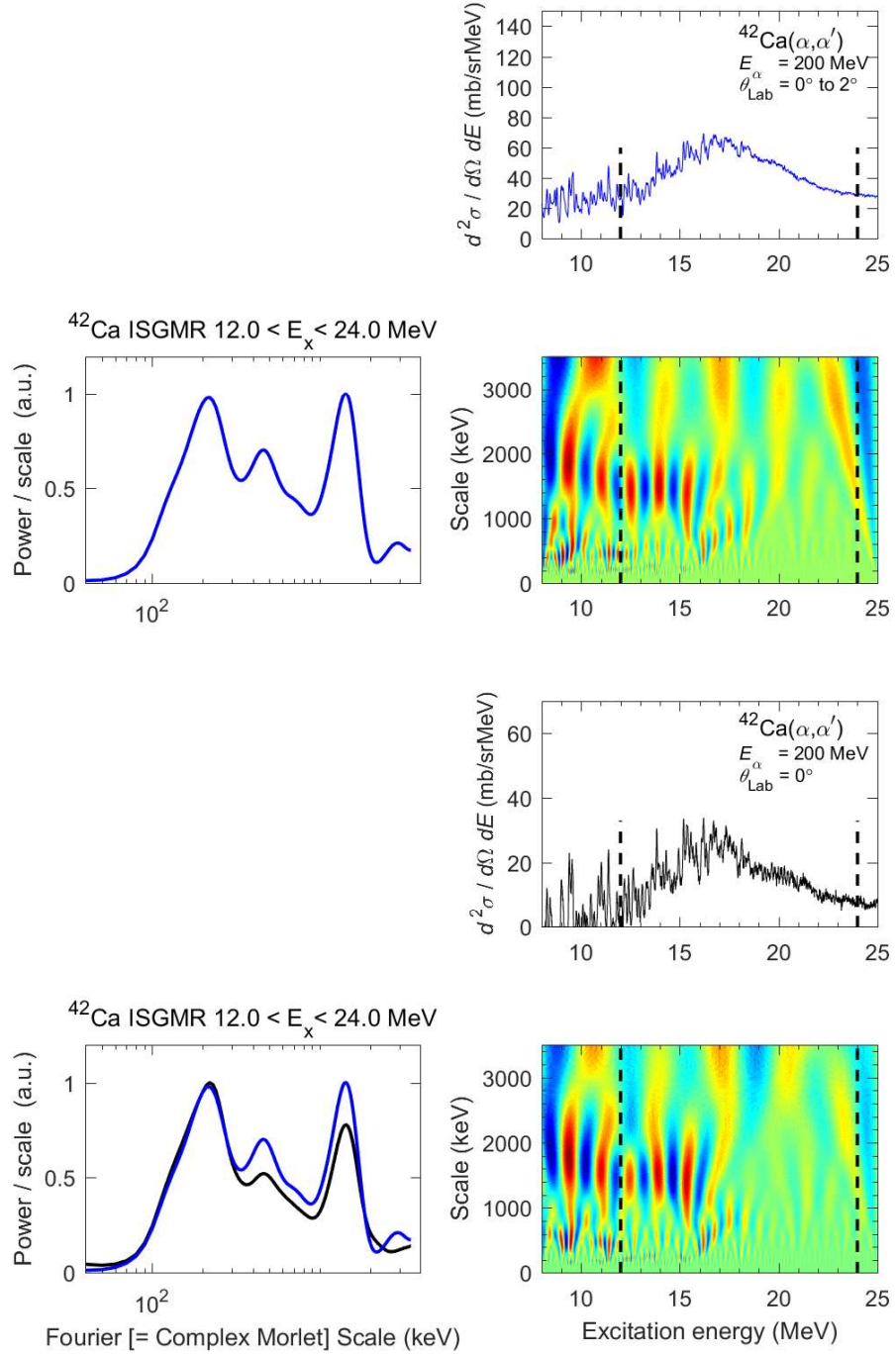
Figure 4.27: Same as Fig 4.25, but for ^{42}\text{Ca} .
