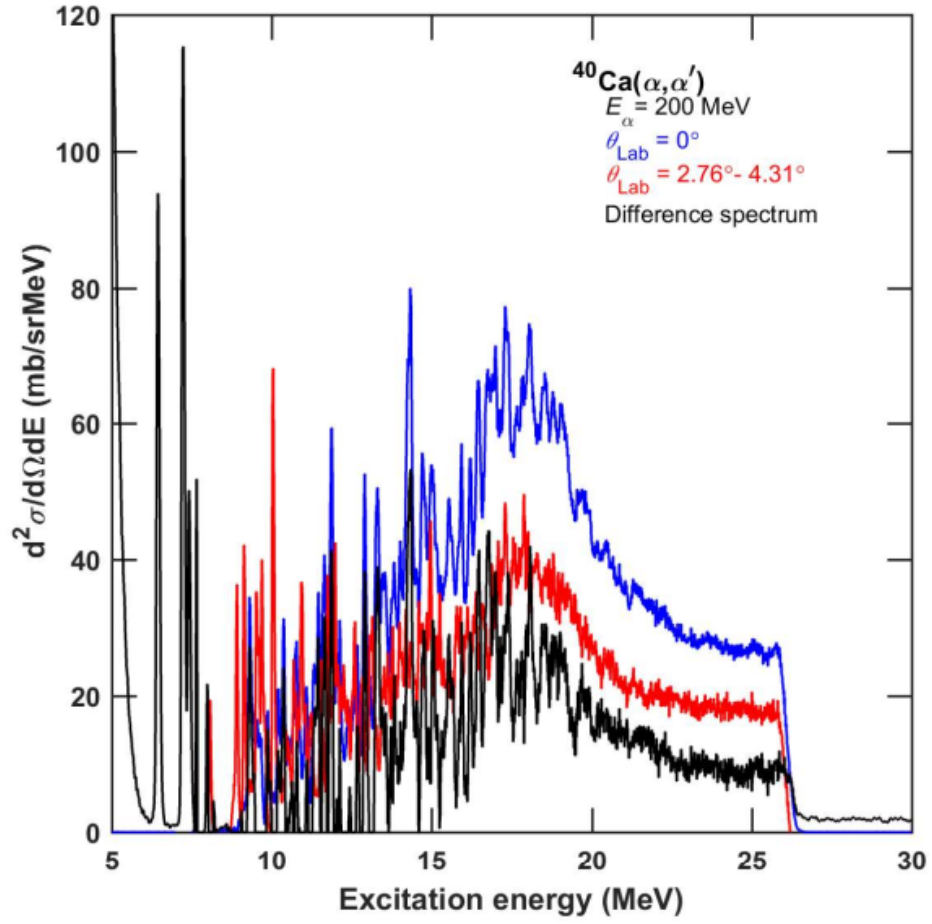
Figure 4.13: Same as Fig. 4.10 but for ^{40}\text{Ca}(\alpha, \alpha') . The 0^\circ - 2^\circ spectrum was scaled by a factor of 1.35.
