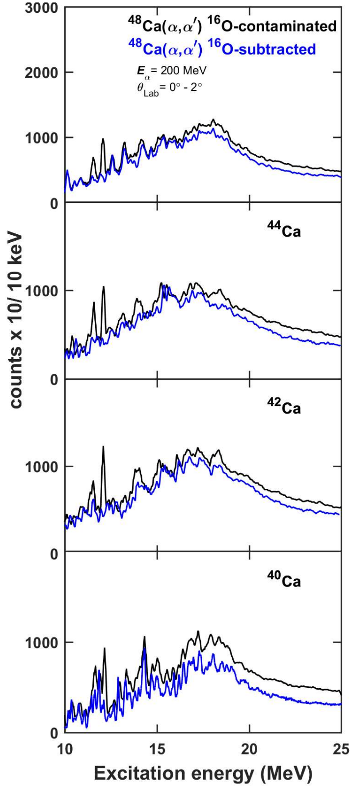
Figure 4.4: Superposition of experimental oxygen-contaminated and oxygen-subtracted excitation energy spectra for ^{48,44,42,40}\text{Ca}(\alpha, \alpha') at E_\alpha = 200 \text{ MeV} and \theta_{\text{Lab}} = 0^\circ - 2^\circ .
