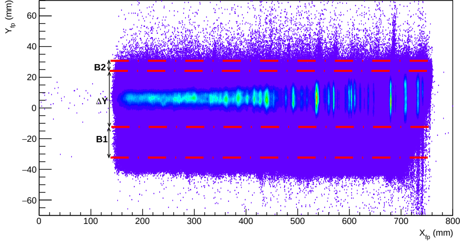
Figure 3.12: A scatter plot of Y_{fp} versus X_{fp} showing the background regions B1 and B2, and the central region \Delta Y containing events of interest on top of the backgrounds.
