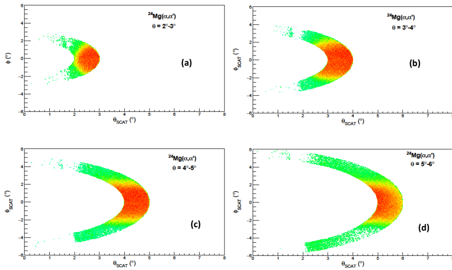
Figure 3.25: The focal plane angle versus scattering angle plots at various angle cut.
