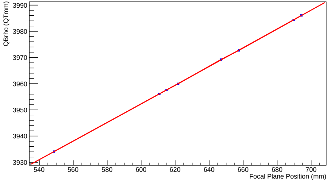
Figure 3.15: A second-order polynomial fit of the momentum of the scattered particle plotted against the corrected focal plane position.
