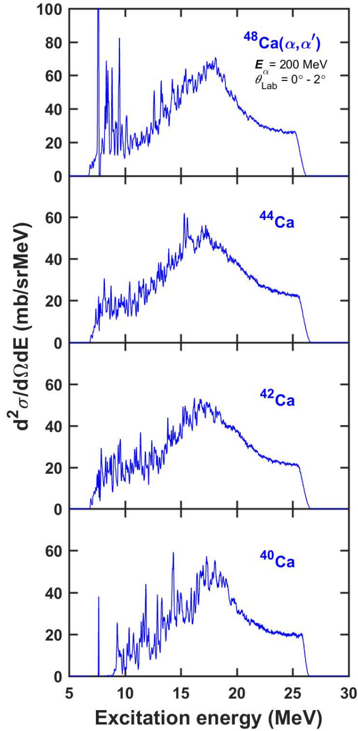
Figure 4.5: Double-differential cross sections obtained from oxygen-free spectra of ^{48,44,42,40}\text{Ca} .
