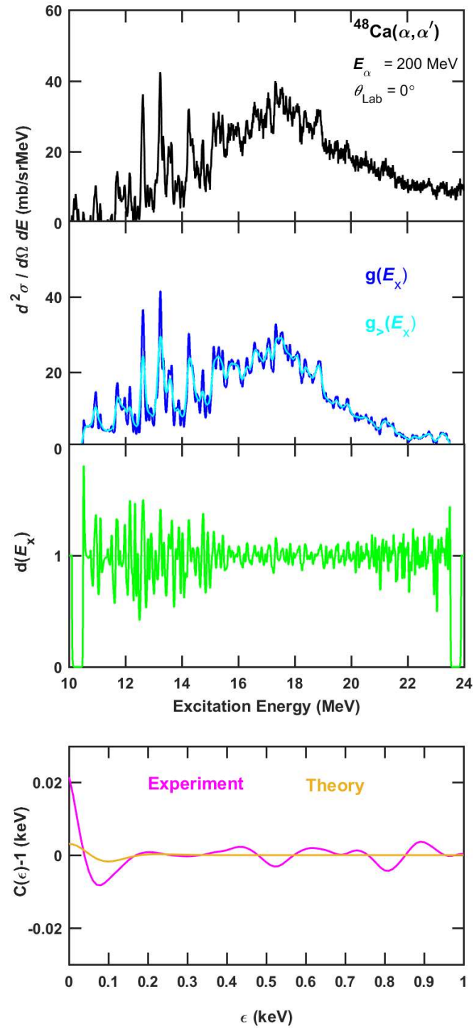
Figure 4.35: Upper part top: Spectrum of the ^{48}\text{Ca}(\alpha, \alpha') reaction at 0^\circ . Upper part middle: Smoothed spectra g(E_x) and g_>(E_x) . Upper part bottom: Stationary spectrum d(E_x) . Lower part: Experimental (magenta line) and theoretical (dark yellow line) autocorrelation functions.
