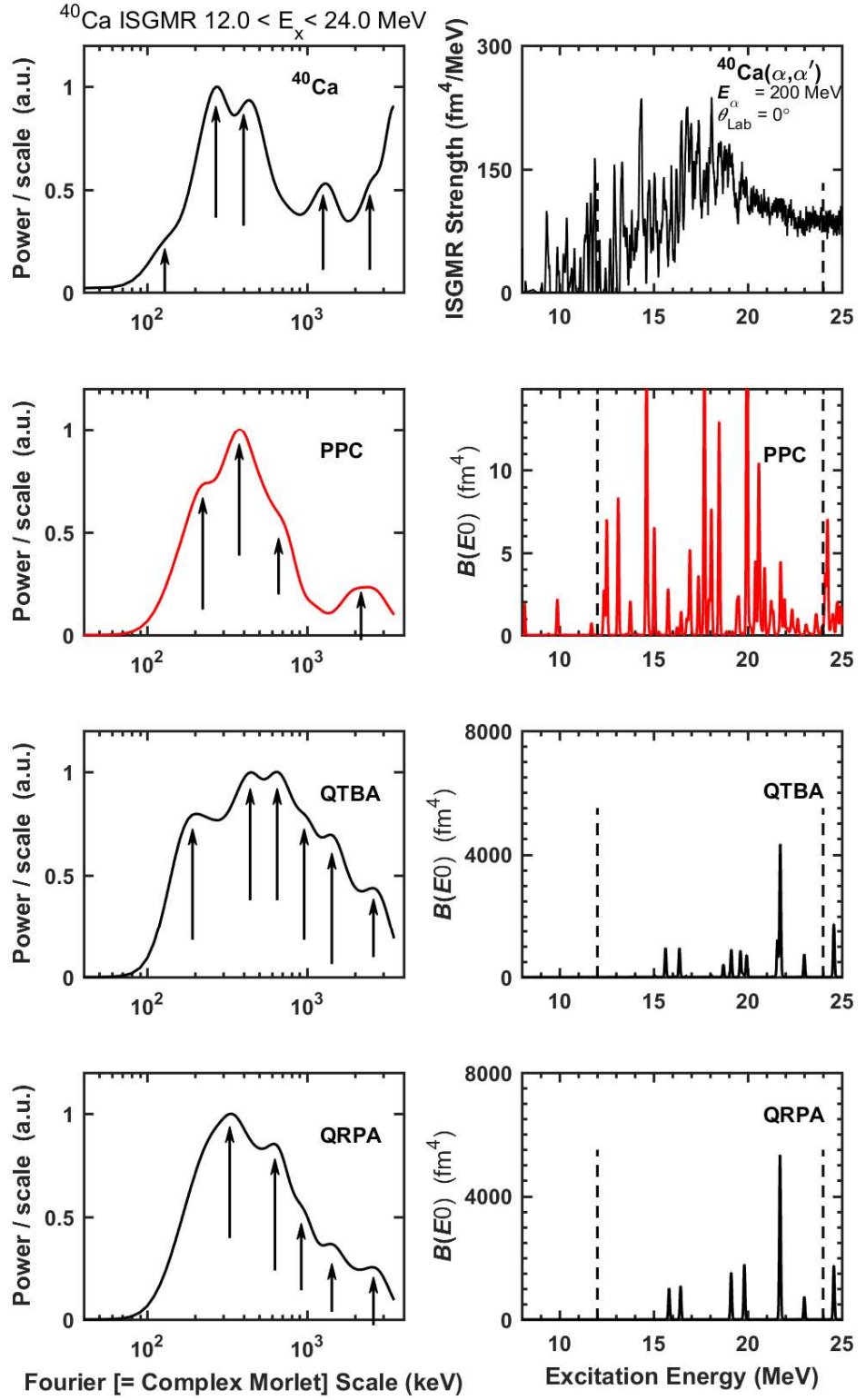
Figure 4.34: Same as Fig. 4.31 but for ^{40}\text{Ca}
