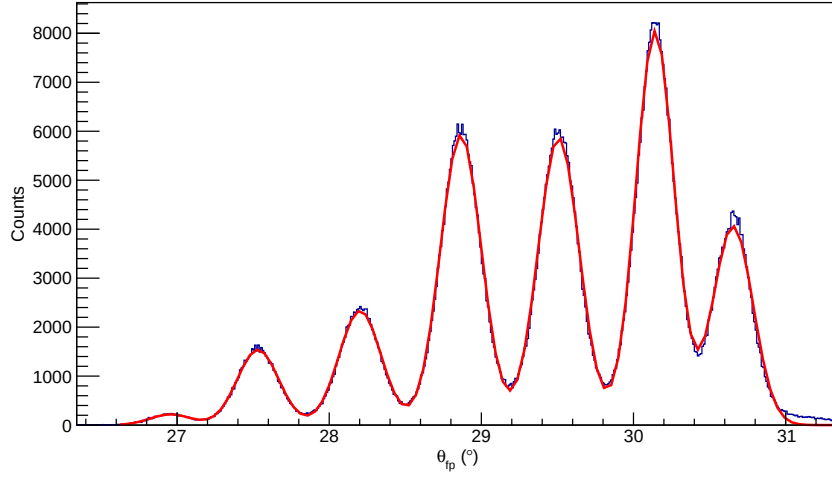
Figure 3.21: A focal plane angle \theta_{\text{fp}} plot for the pepperpot run showing the associated Gaussian fits to the observed peaks for x_{\text{fp}} = 613 mm.
