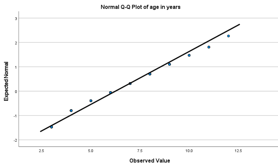
Figure 4.2: A line graph depicting test of normality for age group.
