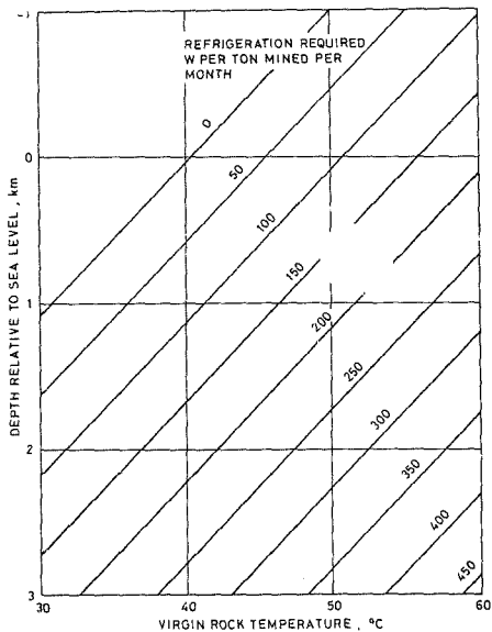
Figure 1.1 : Refrigeration requirements as a function of VRT
