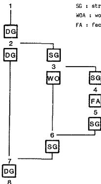
Figure 3.2 : Stope as a network
