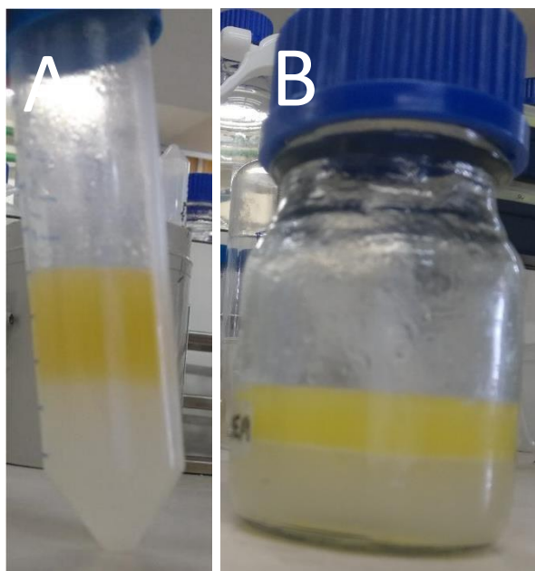
Figure 4.5. The water-washed results of test 1 and 2 biodiesel production. (A) This is the water washed sample from the biodiesel formation using EcN produced media as an ethanol substitute with clear biodiesel on upper level and contamination in the lower layer. (B) This is the water-washed sample from the biodiesel formation using EcN produced media as an ethanol and catalyst substitute with clear biodiesel on upper level and contamination in the lower layer.
