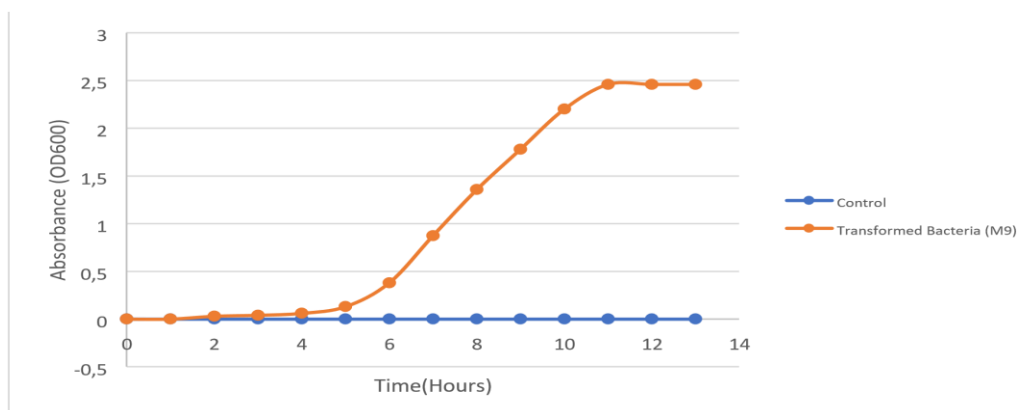
Figure 3.5: The growth curve of Kanamycin transformed E. coli Nissle in M9 media showing the absorbance (OD600) over a period of time(hours). The results show the growth of E. coli Nissle over a 13-hour period with the absorbance read every hour. The average of three test growth curves containing the E. coli Nissle and a control containing no E. coli Nissle was completed over the 13-hour period
