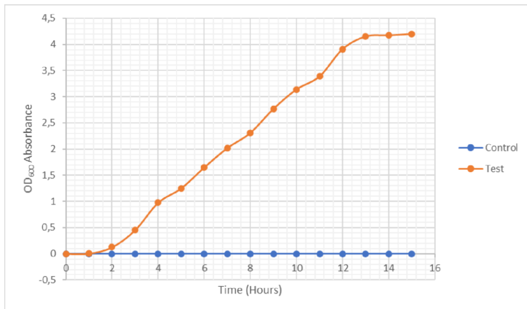
Figure 3.2: The growth curve of E. coli Nissle in LB media showing the absorbance (OD 600 ) over a period of time(hours). The results show the growth of E. coli Nissle over a 15-hour period with the absorbance read every hour. The average of three test growth curves containing the E. coli Nissle and a control containing no E. coli Nissle was completed over the 15-hour period.
