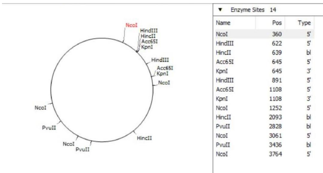
Figure 2.2 Restriction enzyme sites on the plasmid pIRES2-EGFP map. The main sites of interest are the HindIII and HincII sites
