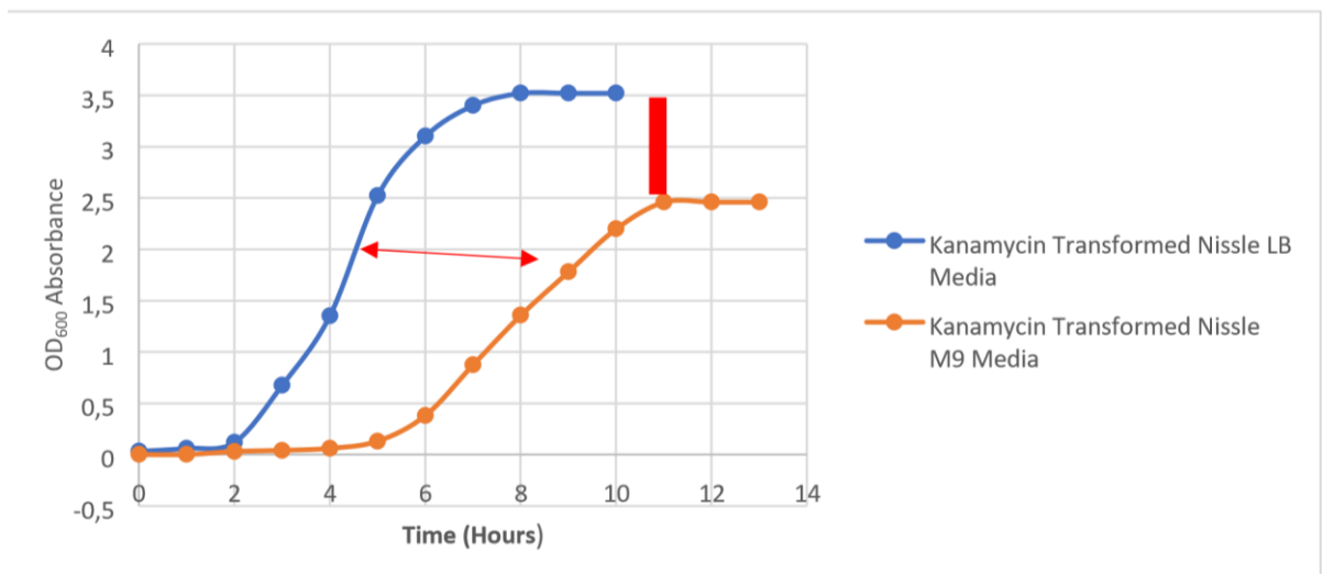
Figure 4.3: The growth curve of transformed E. coli Nissle in LB media and M9 media showing the absorbance (OD 600 ) over a period of time(hours). The results show a major difference between the two growth curves and that the EcN still takes longer to adjust to the M9 media due to the bare minimum growth salts present in the media
