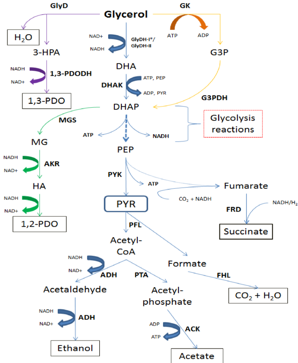
Figure 1.3: Diagram which displays glycerol metabolism in E. coli as well as other members of Enterobacteriaceae family. This indicates fermentative key products which are shown with black boxes. The various pathways are all colour coded as such: (A). The purple and orange colours show the reductive and oxidative pathways of the members of the Enterobacteriaceae family respectively. (B). As described in the text, E. coli use the blue and green pathways. Various enzymes are responsible for the reactions which are shown alongside their respective reaction (Gonzalez et al, 2008).
