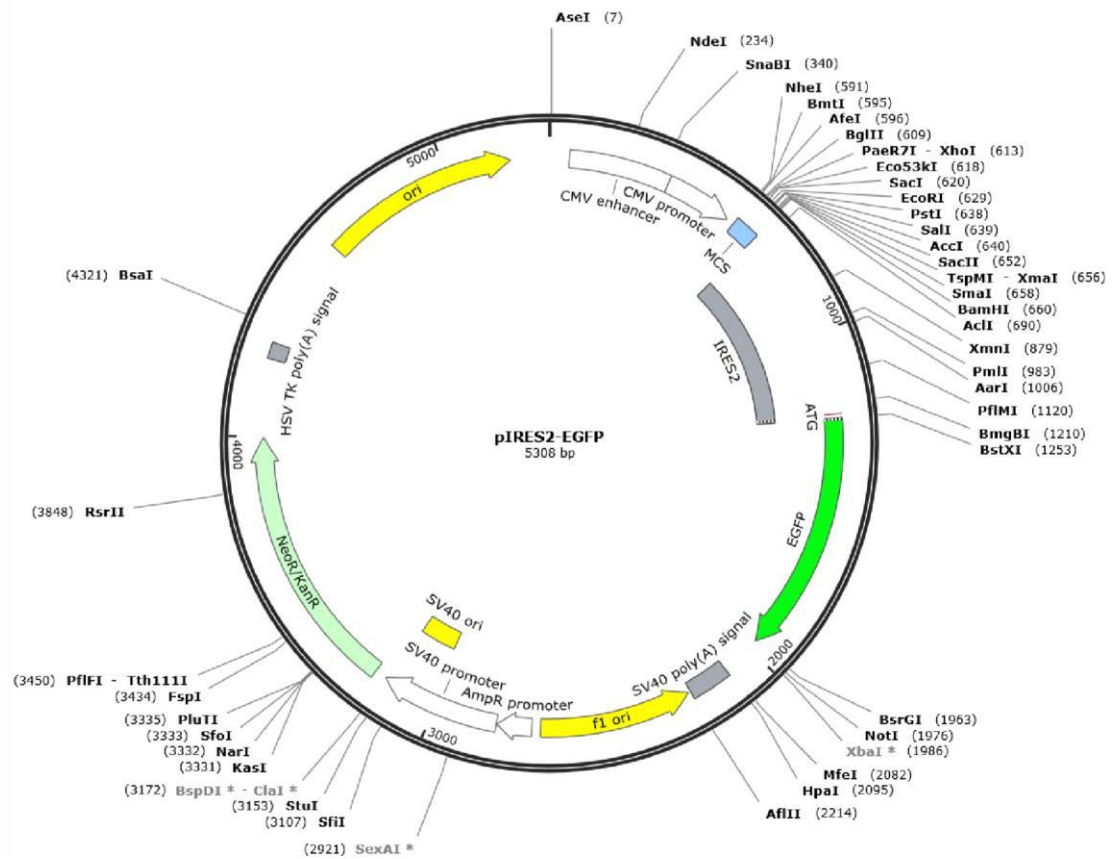
Figure 2.1. The plasmid pIRES2-EGFP. The main points of interest in this figure are the light green arrow between the 3000 – 4000 indicators which refers to the kanamycin resistance gene and the other one is the neon green arrow between the 1000– 2000 indicator which refers to the EGFP (pIRES2-EGFP Sequence and Map, 2022).
