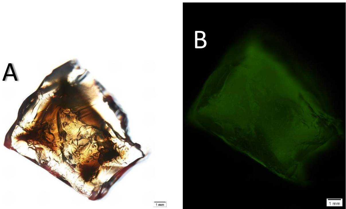
Figure 3.7: Microscopic image of the E. coli Nissle biofilm on the calcium alginate carrier. The image on the left (A) displays the bright field view of the biofilm on the alginate carrier at 4X magnification. The biofilm is indicated by the dark colouring in the middle of the alginate. The image on the right (B) displays the florescence view of the biofilm on the alginate carrier at 4X magnification. The biofilm is indicated by the green fluorescence on the alginate.
