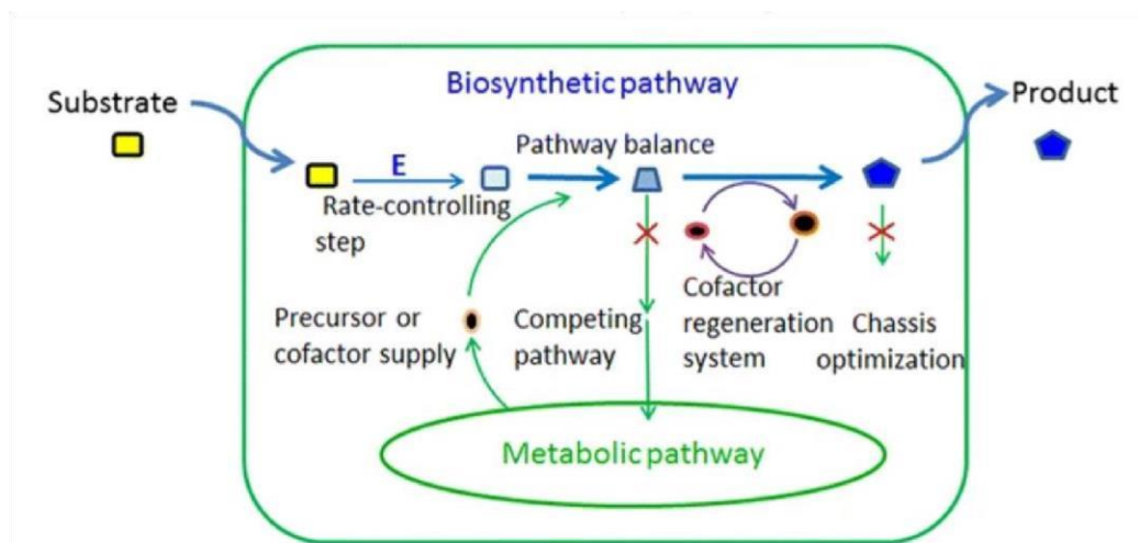
Figure 1. 4: An example of how a whole cell biocatalyst system would function and overall ways for optimization. This displays the conversion of a substrate to a product using a cell's internal pathways (Straathof et al , 2002).
