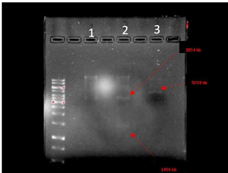
Figure 3.3: A 1% Agarose gel of the extracted plasmid showing two sites that have gone through restriction enzyme digestion. Lane 1 contains the uncut plasmid DNA. Lane 2 contains the HincII cut DNA fragments. Lane 3 contains the HindIII cut DNA fragments.
