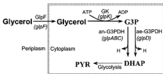
Figure 1.2: Aerobic glycerol metabolism in E. coli . Glycerol is metabolised by an ATP- dependant glycerol kinase (GK), as well as aerobic G3PDH (ae- G3PDH) and the electron (an-G3PDH) which are two respiratory enzymes. This is all completed in the presence of electron acceptors. H is the reducing equivalent (NADPH/NADH/FADH 2 ), PYR is referred to as pyruvate and DHAP is dihydroxyacetone phosphate (Murarka et al. 2008).
