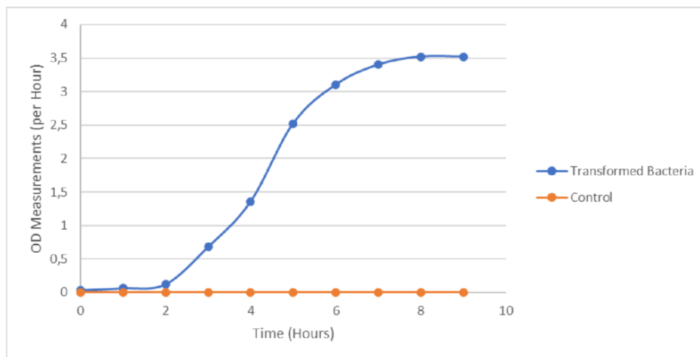
Figure 3.4: The growth curve of Kanamycin transformed E. coli Nissle in LB media showing the absorbance (OD600) over a period of time(hours). The results show the growth of E. coli Nissle over a 9-hour period with the absorbance read every hour. The average of three test growth curves containing the E. coli Nissle and a control containing no E. coli Nissle was completed over the 9-hour period.
