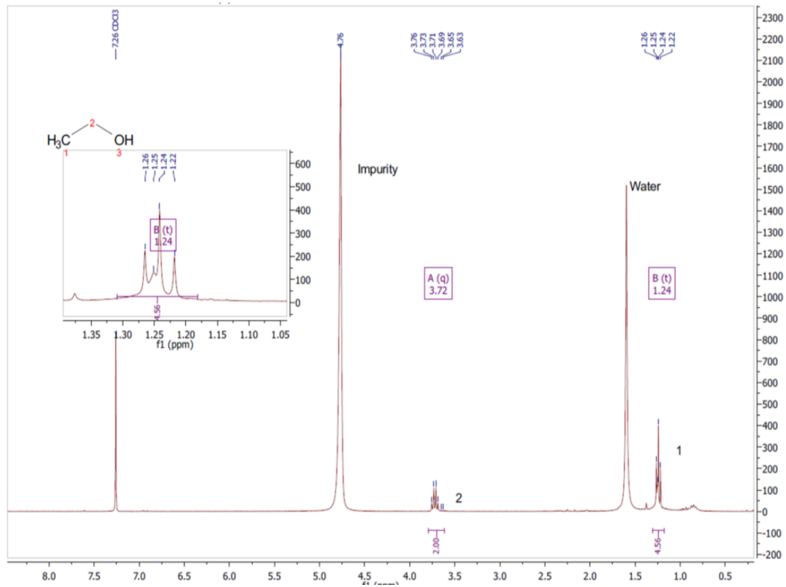
Figure 3.11: The proton NMR of fraction distillation obtained from distilled EcN media utilizing a calcium alginate and 1% agarose as the carrier. The peak at 1,25 ppm labelled “1” relates to the H 3 C group, the peak at 1,55ppm labelled “water” relates to the OH group and the peak at 3,75 ppm labelled “2” relates to the H 2 C group as shown on the legend on the top-left part of the figure. The peak at 7,25 relates to the deuterated chloroform that the ethanol sample was dissolved in. The square box above the deuterated chloroform is a zoomed version of peak “1”. This shows the 2 distinct peaks relating to the H group. The peak at 4,75 ppm labelled “impurity” is some form of contamination that occurred during distillation.
