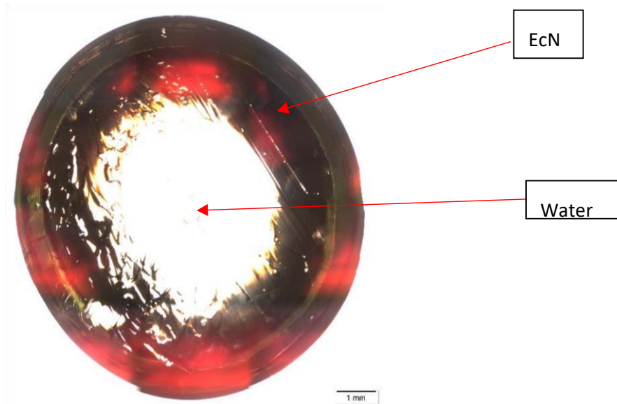
Figure 4 .4: Microscopic image of the E. coli Nissle biofilm on the water pebble carrier. The image indicates that the EcN growth occurs on the outer most layer of the water pebble while water and other aspect of the M9 media permeate further into the centre of the water pebble.
