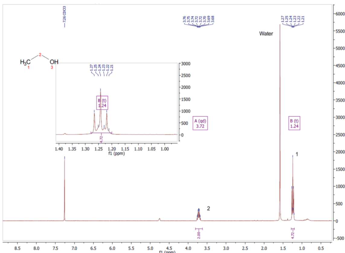
Figure 3.10: The proton NMR of fraction distillation obtained from the distilled EcN media utilizing a water pebble as the carrier. The peak at 1,25 ppm labelled “1” relates to the H 3 C group, the peak at 1,55ppm labelled “water” relates to the OH group and the peak at 3,75 ppm labelled “2” relates to the H 2 C group as shown on the legend on the top-left part of the figure. The peak at 7,25 relates to the deuterated chloroform that the ethanol sample was dissolved in. The square box above the deuterated chloroform is a zoomed version of peak “1”. This shows the 2 distinct peaks relating to the H group.
