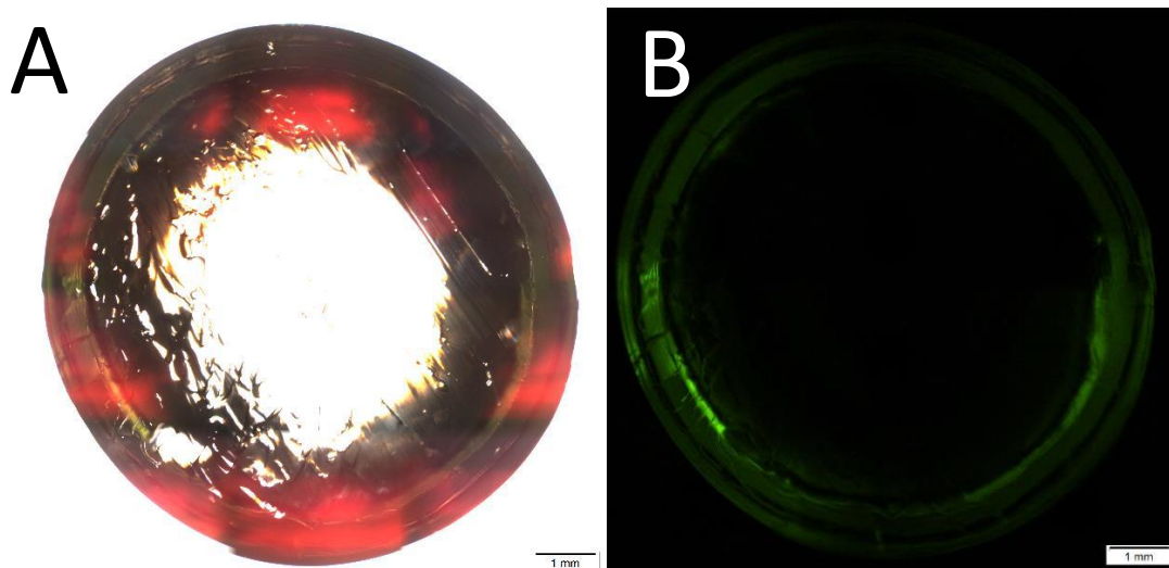
Figure 3.9: Microscopic image of the E. coli Nissle biofilm on the water pebble carrier. The image on the left (A) displays the bright field view of the biofilm in the water pebble at 4X magnification. The biofilm is indicated by the dark colouring around the outer edges of the water pebble. The image on the right (B) displays the florescence view of the biofilm in the water pebble at 4X magnification. The biofilm is indicated by the green fluorescence around the outer edges of the water pebble
