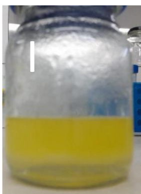
Figure 3.14: Biodiesel production using EcN produced media as an ethanol and catalyst substitute. Sample (I) shows the biodiesel produced from olive oil as a bright yellow liquid with the clear liquid at the bottom being glycerine.
