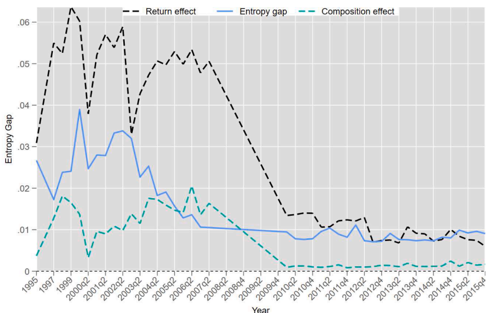
Fig. 3. Entropy measure decomposition results.
