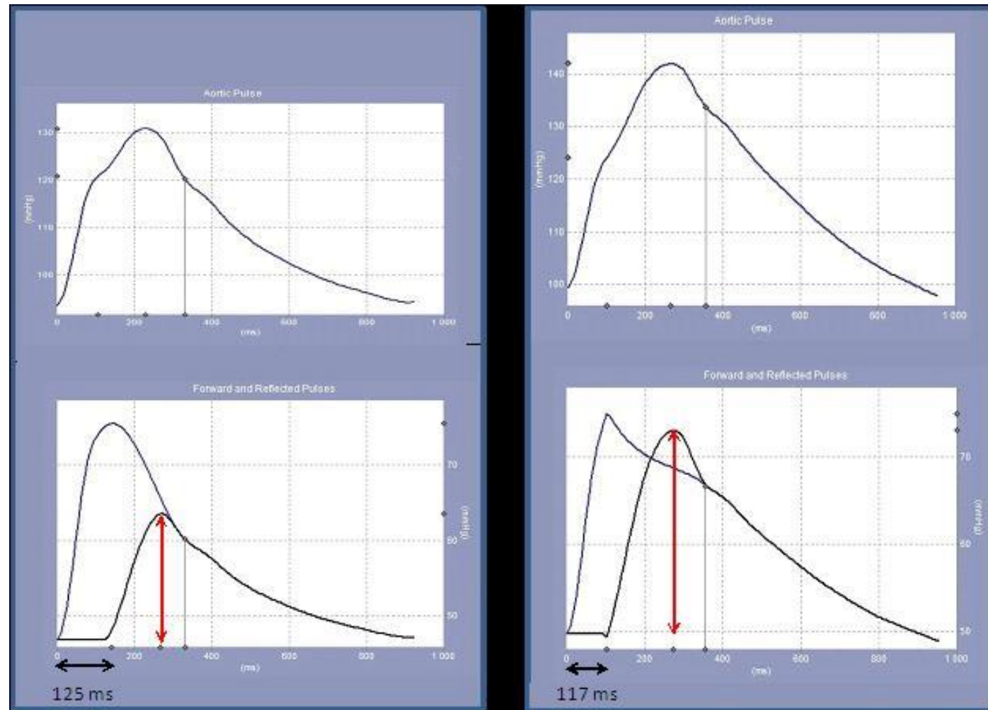
Figure 6.1. Impact of an earlier return of the backward pressure wave on aortic pulse pressure. Left panels show the effect of a late return and right panels the effect of an early return of the backward pressure wave. Upper panels show aortic pulse and lower panels show forward and backward wave pressures.
