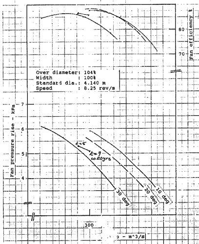
Figure 6.5 Vaal Reefs No. 5 Shaft. Performance of a fan selected with hurdle rate 20% . Years 6 to 20.
