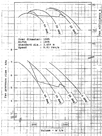
Figure 6.3 Vaal Reefs No. 5 Shaft. Fan performance with initial impeller fitted.
