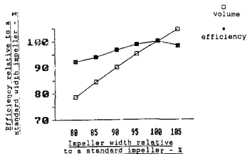
Figure 4.2 The effect of changing impeller width on volume flow rate and efficiency.
