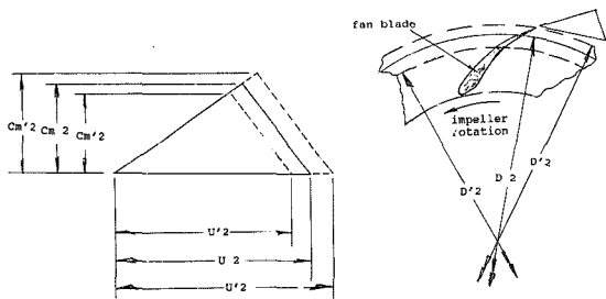
Figure 4.1 The effect of small changes in impeller diameter on velocity triangles
