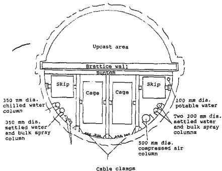
Figure 2.2 Cross section through a shaft as depicted by Lloyd(1)
