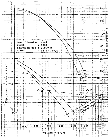
Figure 6.6 Vaal Reef No. 5 Shaft. Performance curve of a fan selected considering the initial duty only.
