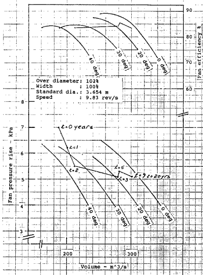
Figure 6.2 Vaal Reefs No. 5 Shaft. Fan performance after a proposed impeller change.
