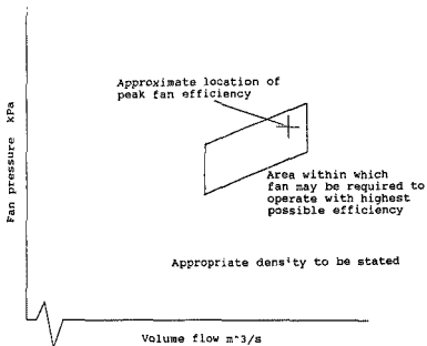
Figure 2.5 A proposal for the presentation of fan duties. (Wallis(12)).
