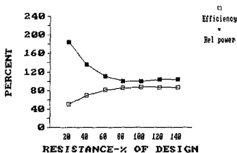
Figure 3.8 Fan performance relative to system resistance
