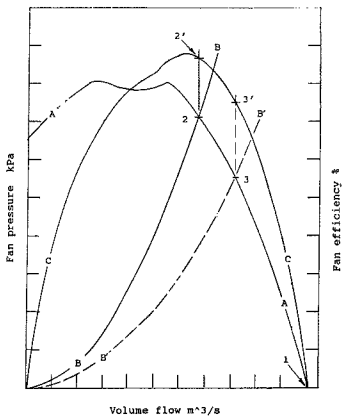
Figure 2.3 A typical main surface fan performance characteristic.
