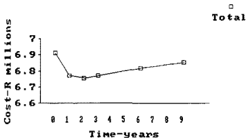
Figure 6.1 Optimum time for impeller change in years, from the date of commissioning.
