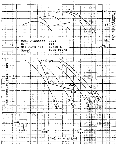
Figure 6.4 Vaal Reefs No. 5 Shaft. Performance of a fan selected with hurdle rate zero. The first nine years.
