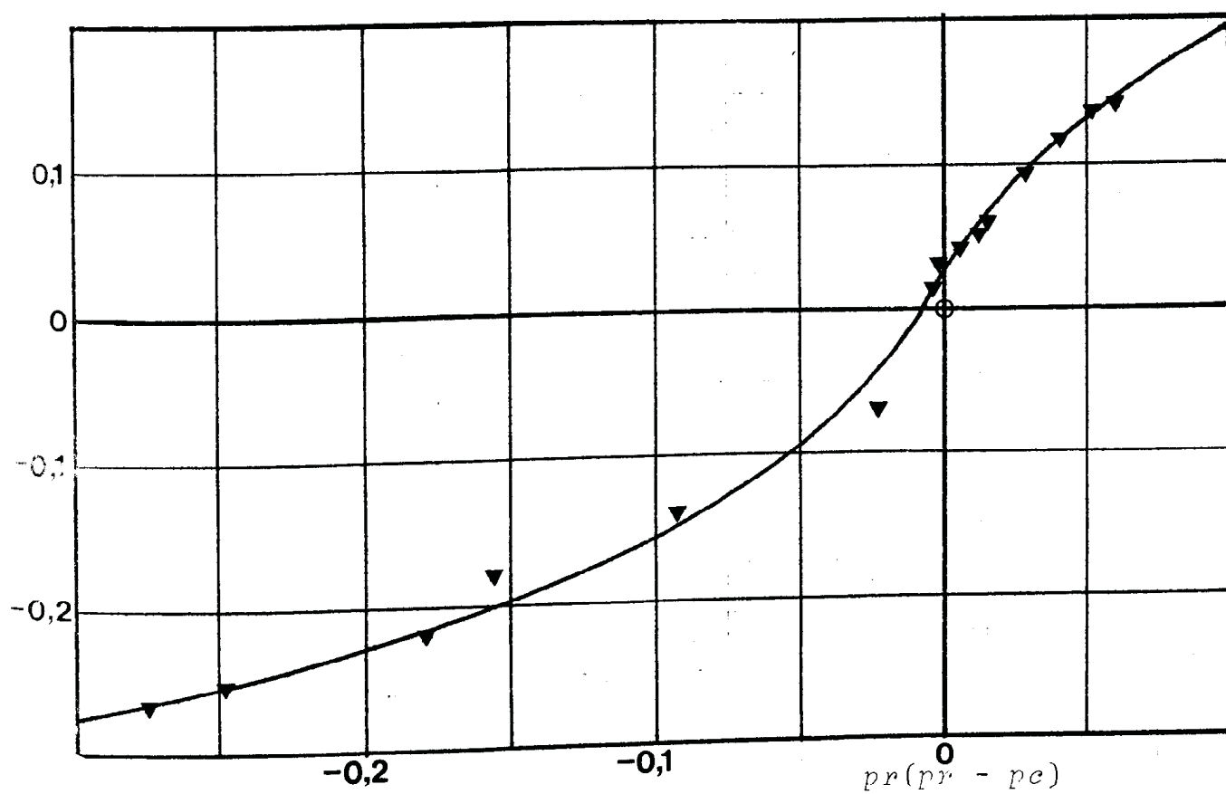
Figure 2.2 g Versus pr(pr - pe) (Normalised)
