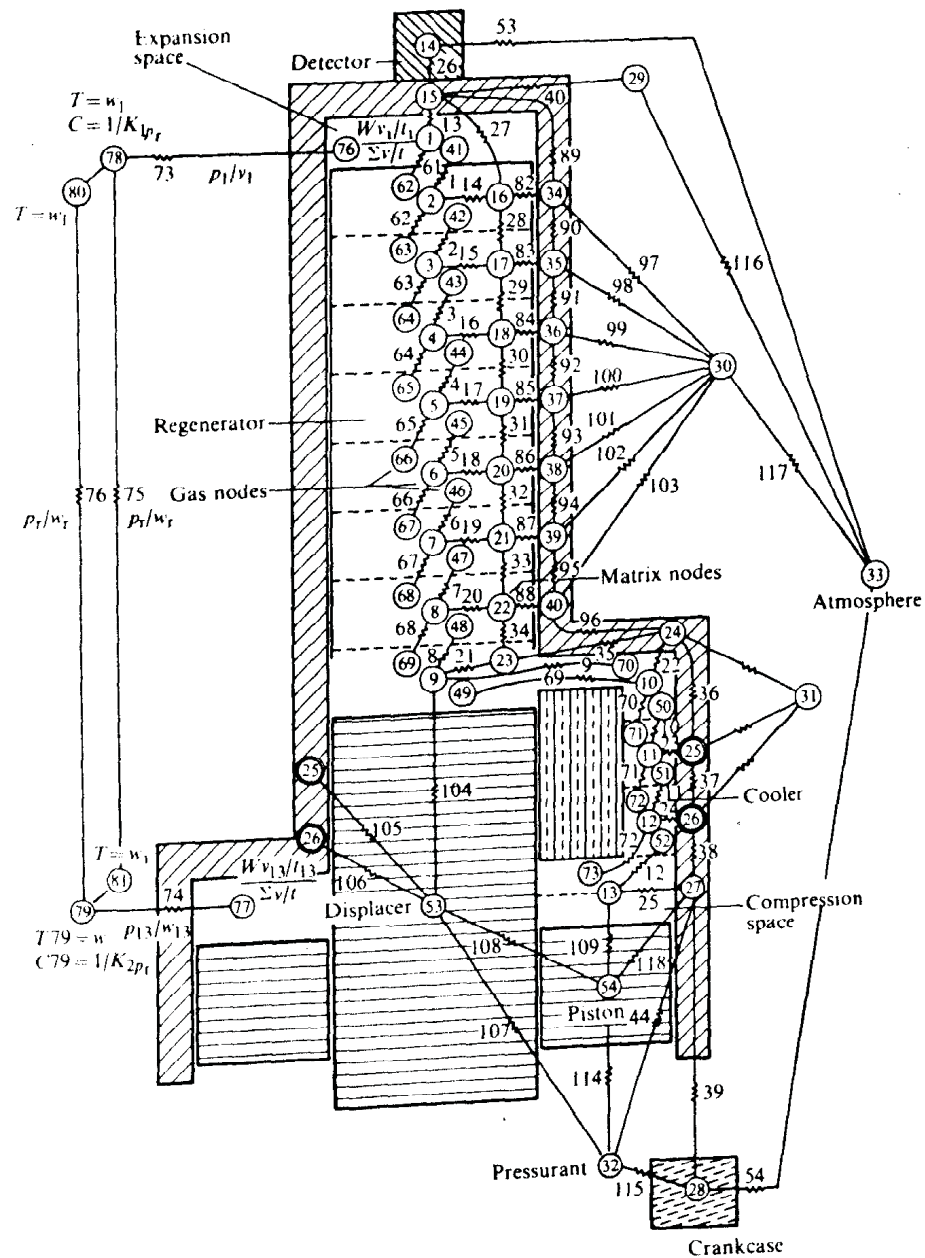
Figure 2.4 Representation of the Nodal Network for Digital Computer Simulation of a Small Stirling-Cycle Cryogenic Cooling Engine (After Finkelstein[Fi75])
