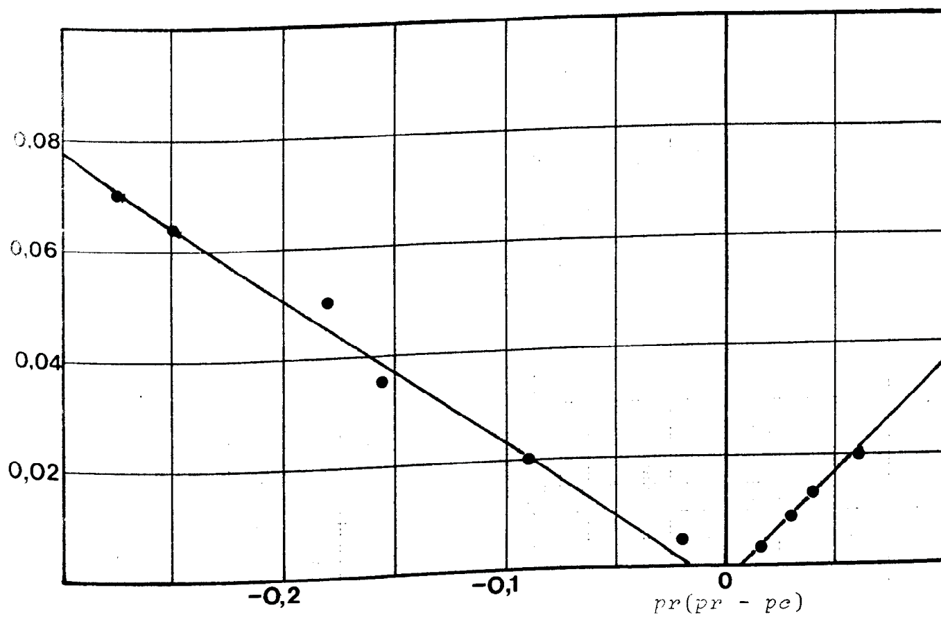
Figure 2.3 g^2 Versus pr(pr - pe) (Normalised)
