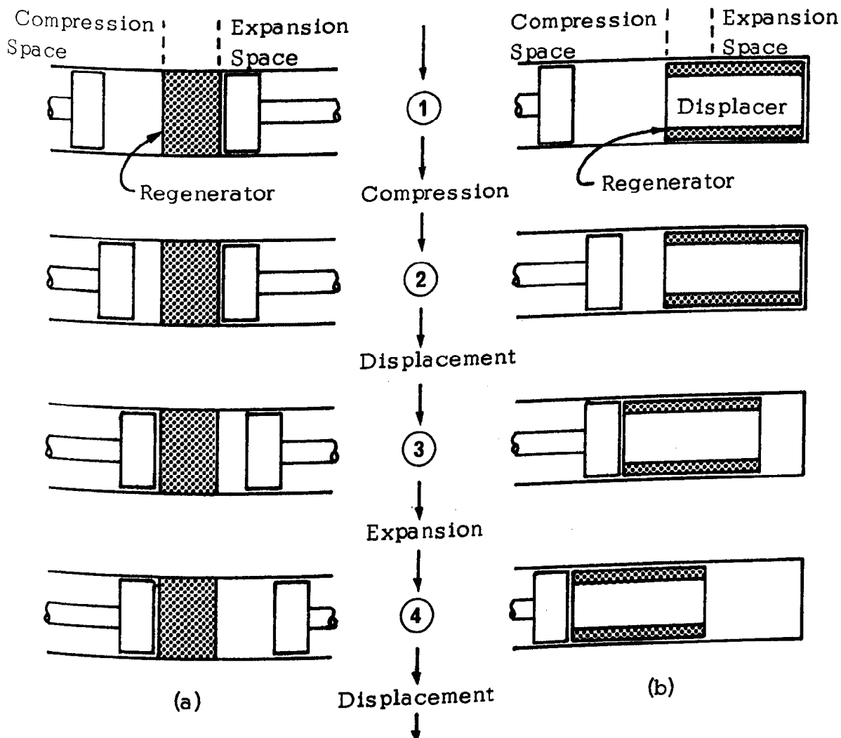
Figure 1.2 Piston and Displacer Motions
