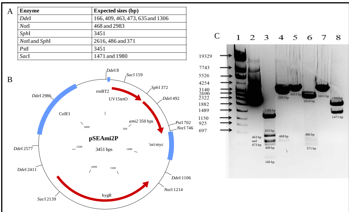
Figure 3.14: Restriction profile of pSEAmi2P. (A) Table displaying the different restriction endonucleases used and the expected fragment sizes, which result from restriction digest of the pSEAmi2P plasmid. (B) Predicted plasmid map of pSEAmi2P vector. (C) Agarose gel depicting the products of restriction digest of pSEAmi2P. [Lane 1] Roche marker IV, [Lane 2] Uncut, [Lane 3] DdeI , [Lane 4] NotI , [Lane 5] SphI , [Lane 6] NotI and SphI , [Lane 7] PstI and [Lane 8] SacI .
