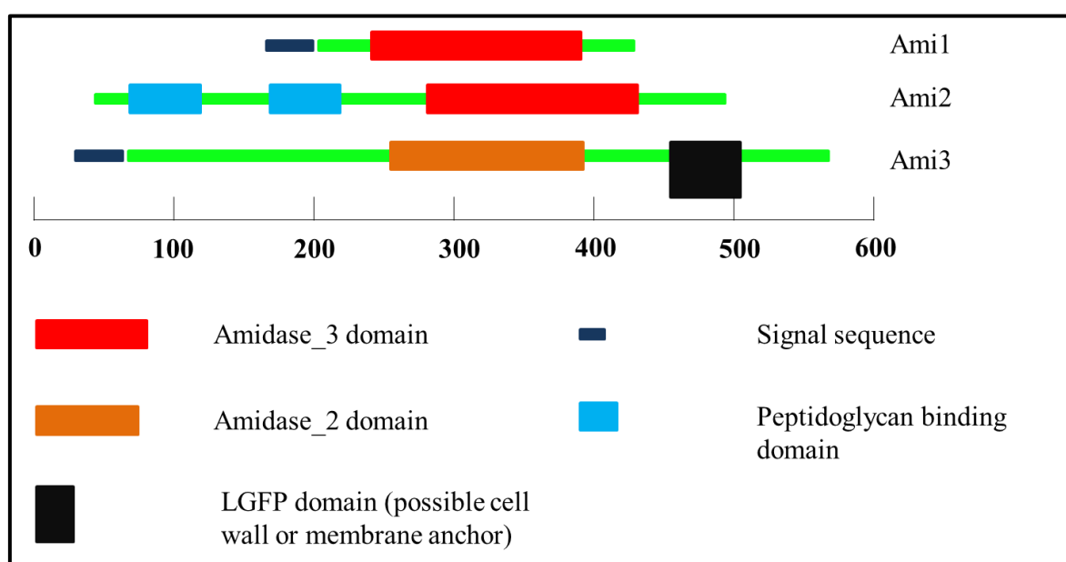
Figure 3.2: Diagrammatic representation of the Msm cell wall amidases and their respective functional domains. Shown are the amidase_3 domains found in Ami1 and Ami2 and the amidase_2 domain present in Ami3. Also shown are the additional domains such as the PG binding domains on Ami2 and the LGFP domain on Ami3.
