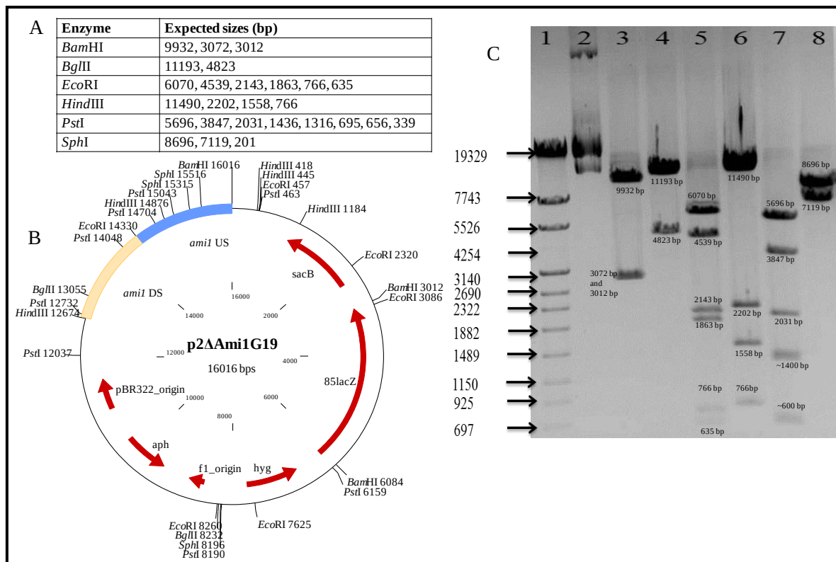
Figure 3.7: Restriction profile of p2ΔAmi1G19. (A) Table displaying the different restriction endonucleases used and the expected fragment sizes, which result from restriction digest of the p2ΔAmi1G19 construct. (B) Plasmid map of the p2ΔAmi1G19 vector. (C) Agarose gel of digested fragments, [Lane 1] Roche marker VI, [Lane 2] Uncut plasmid, [Lane 3] Bam HI, [Lane 4] Bgl II, [Lane 5] Eco RI, [Lane 6] Hind III, [Lane 7] Pst I and [Lane 8] Sph I
