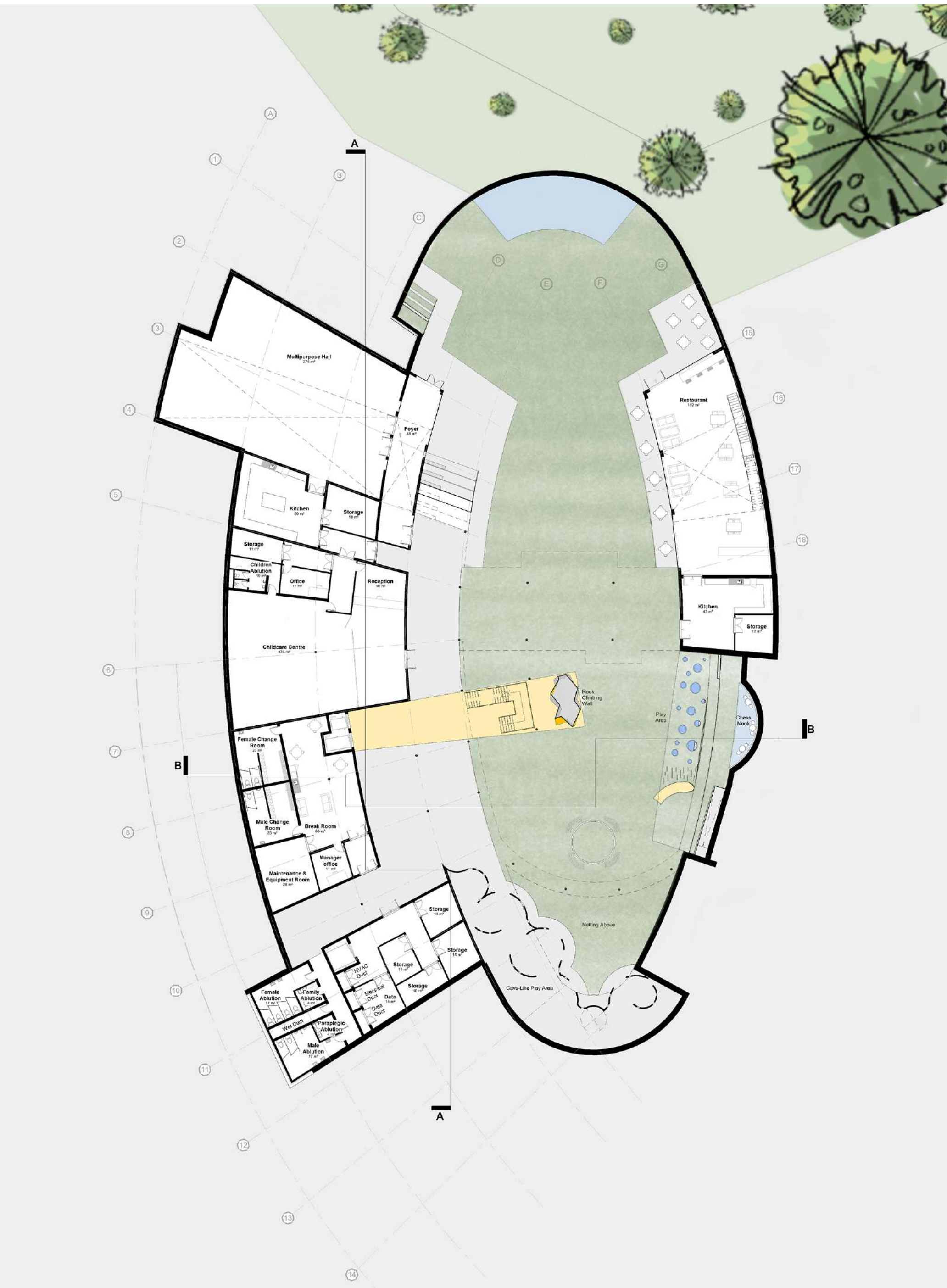
Figure 11.14: Basement Floor Plan (Author, 2024)
