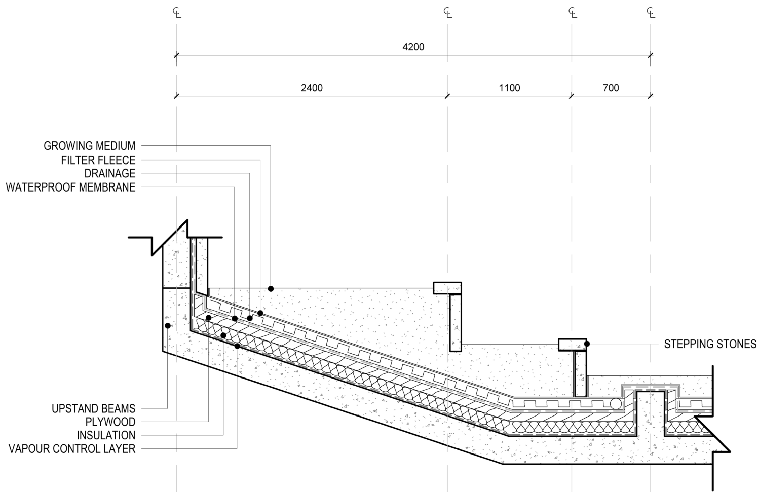
Figure 12.4: Callout Detail (Author, 2024)
