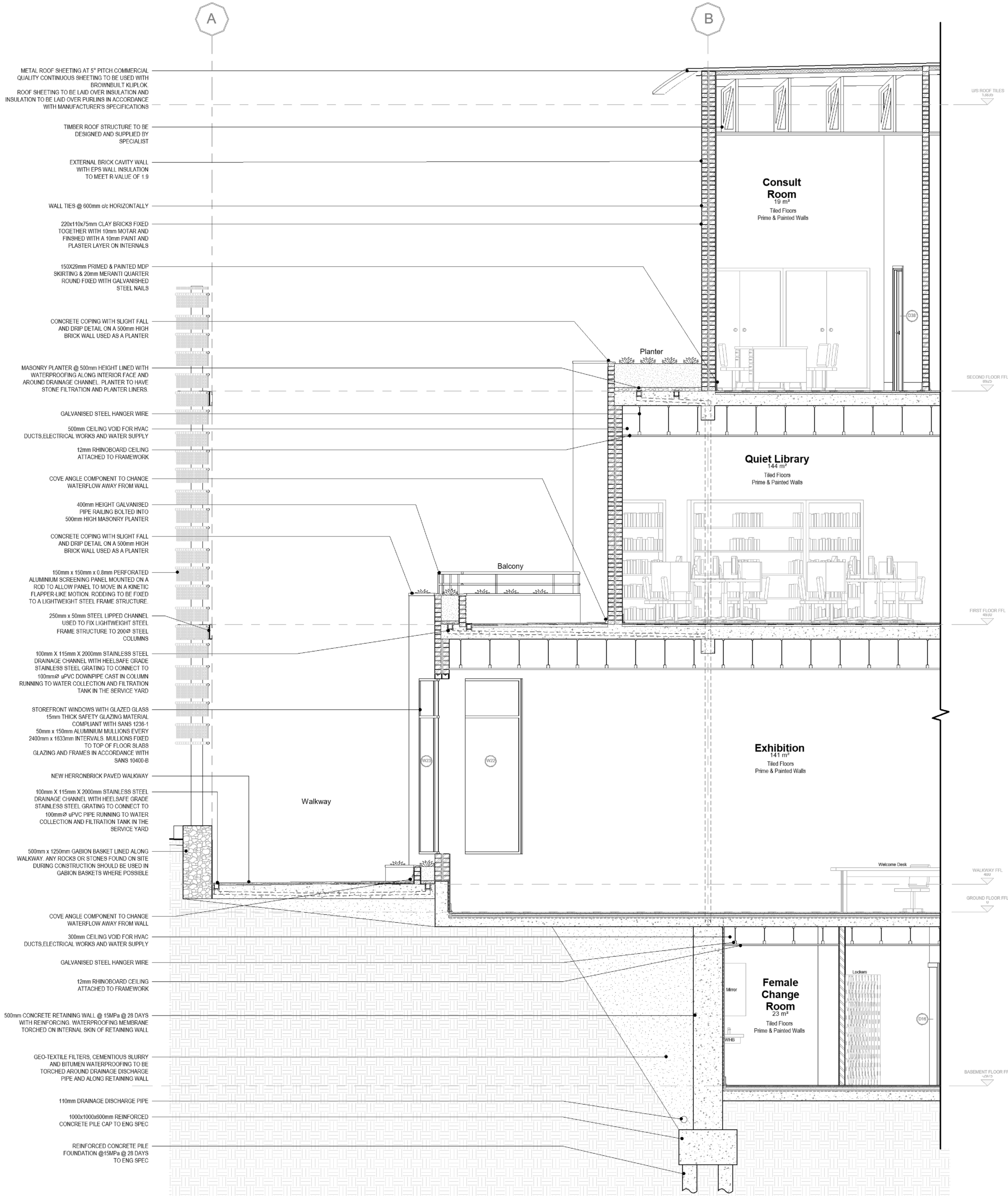
Figure 12.3: Perimeter Section (Author, 2024)
