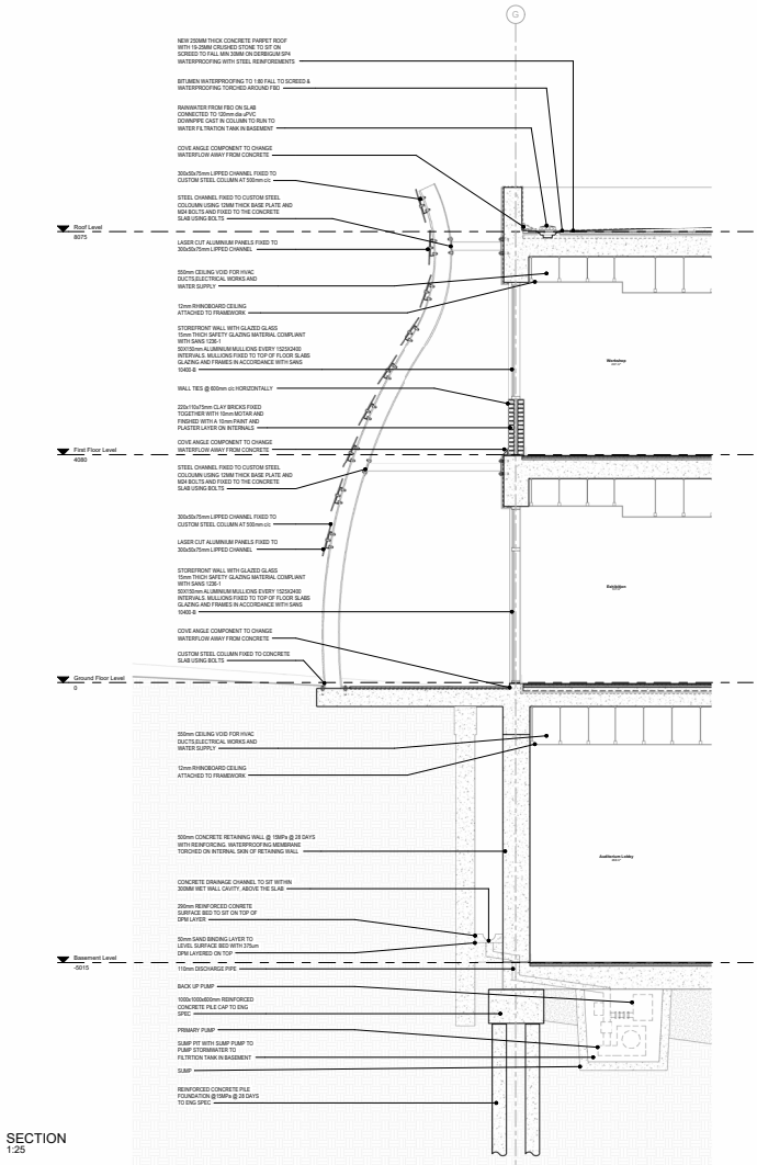
Figure 9.42: Technical Drawings Sheet (Author, 2024)
