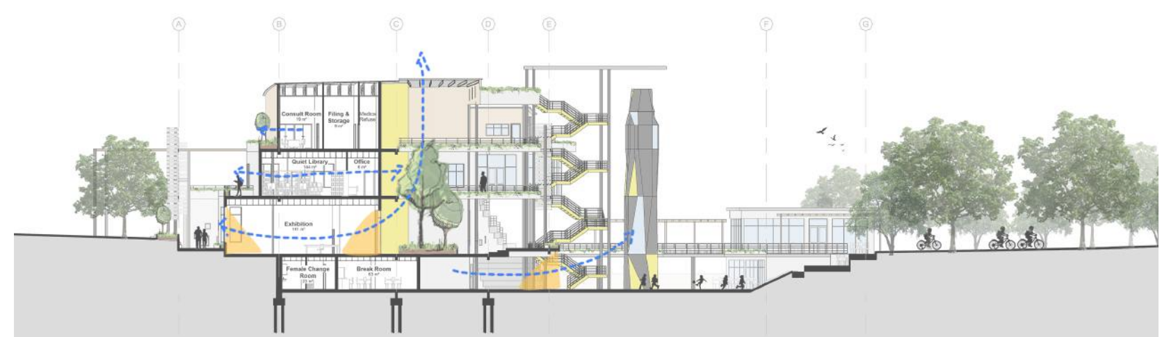
Figure 11.39: Diagram showing natural lighting and ventilation in Section B-B (Author, 2024)
