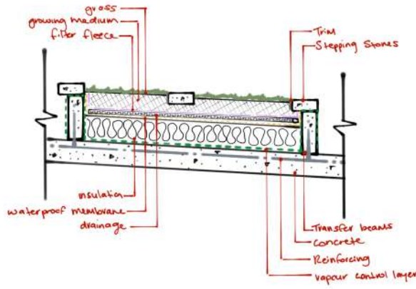
Figure 9.40: Green Roof Drainage Option (Author, 2024)
