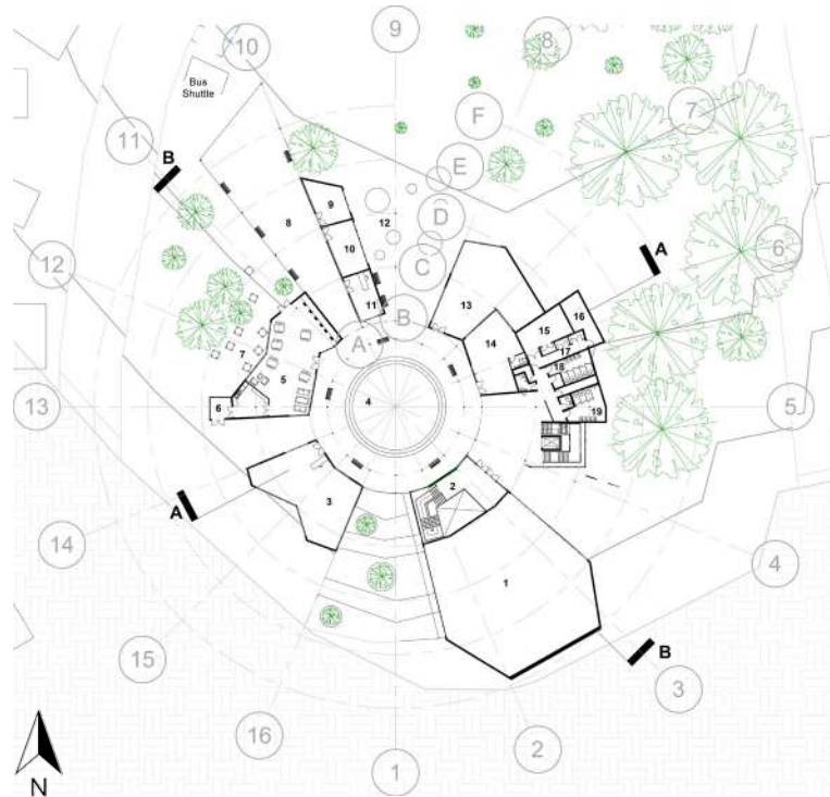
Figure 9.24: Ground Floor Plan (Author, 2024)
