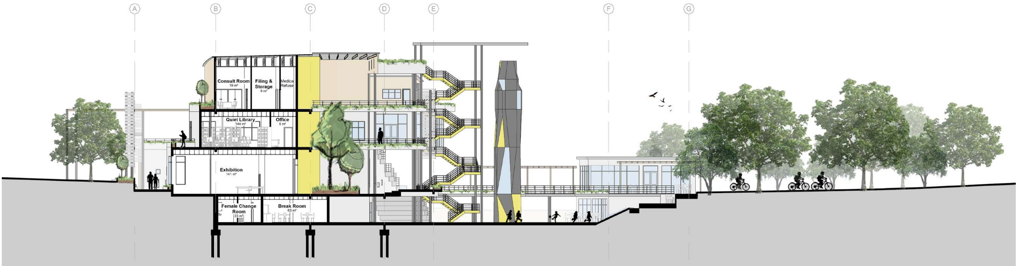
Figure 11.35: Section B-B (Author, 2024)
