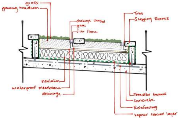
Figure 9.39: Green Roof Drainage Option (Author, 2024)
