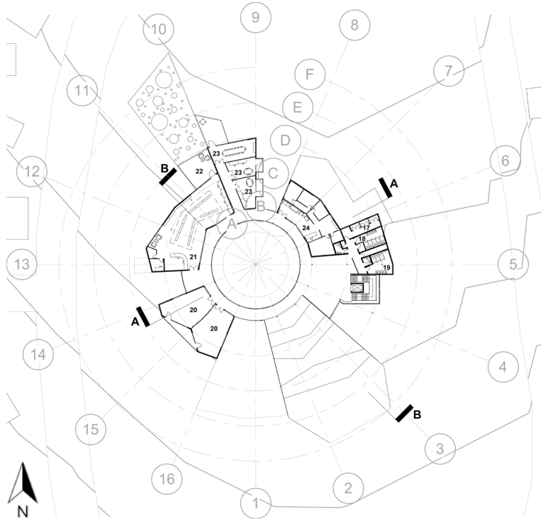
Figure 9.25: First Floor Plan (Author, 2024)
