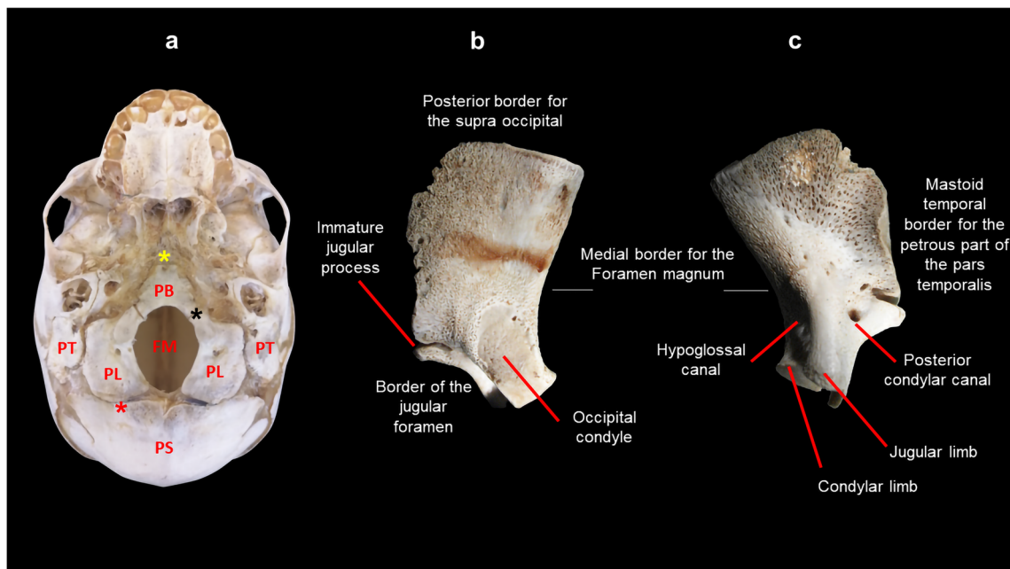
Fig. 1 Prenatal basicranium representing osteological features and borders of the left pars lateralis. a Extracranial view of the basicranium highlighting the PS: pars squama, PL: pars lateralis, FM: foramen magnum, PB: pars basilaris, PT: pars temporalis and synchondroses* (red: PIOS—posterior intraoccipital synchondrosis, black: AIOS—anterior intraoccipital synchondrosis and yellow: SOS—sphenoid-occipital synchondrosis). b Extracranial view of the left pars lateralis representing posterior border for the supraoccipital,
