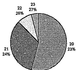
OT (1998): Proportions of Students According to Age
