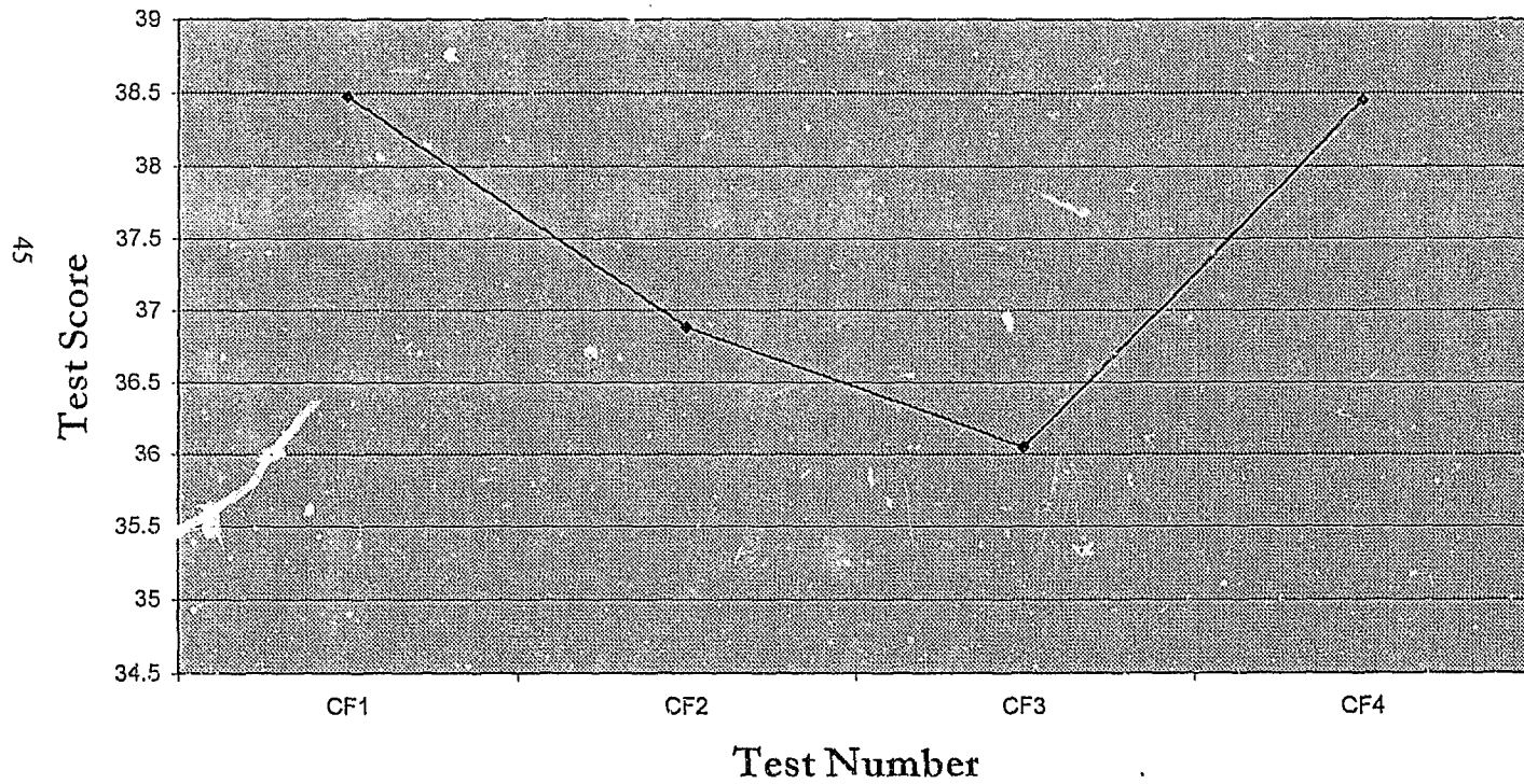
OT (1998): Average CF Test Scores According to Time
