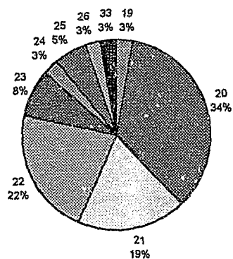
Physio (1997): Proportions of Students According to Age
