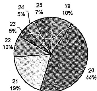
Physio (1998): Proportion of Students According to Age
