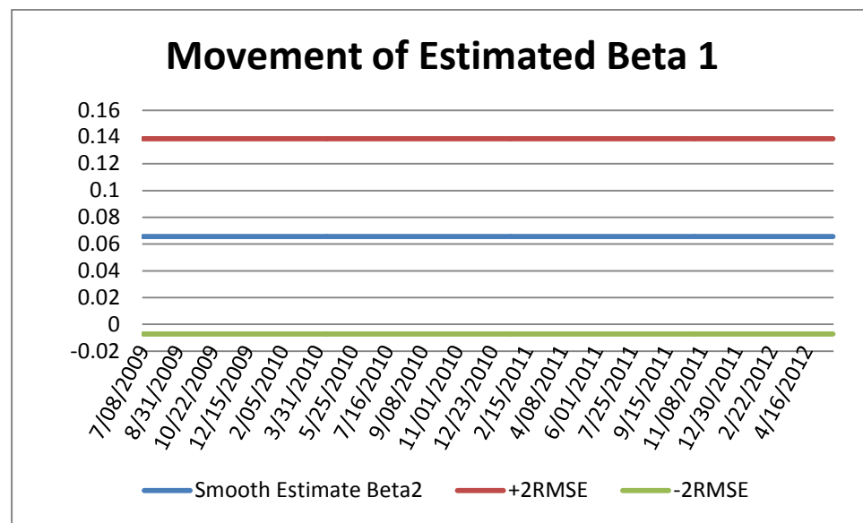
Figure 27: Simple regression with time varying parameters for Government bond 2006
