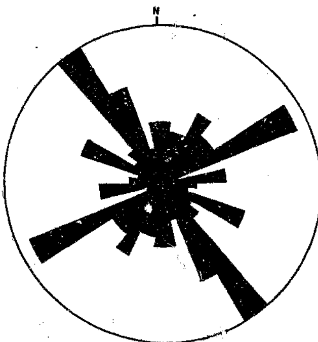
Fig. 4.19: Rose diagram showing the main trend elongation of clasts of the Rosh Pinah Formation and pisolites of the Pickelhaube Formation from throughout the study area during D1.
