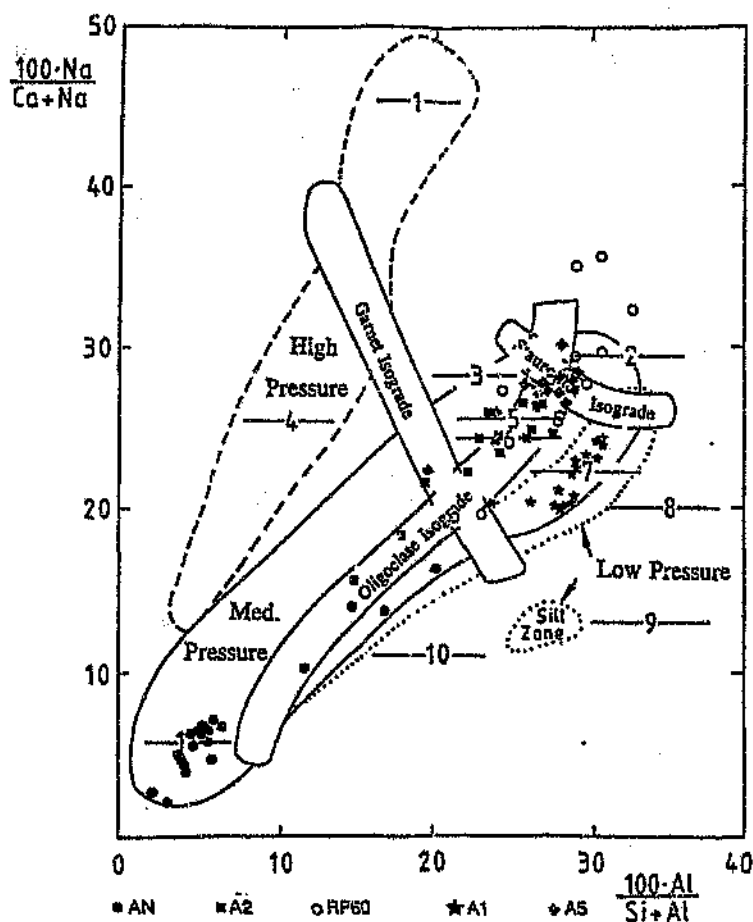
Figure 5.9: Facies fields of metabasites and coexisting pelites after Laird & Albee (1981).
