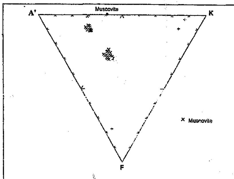
Figure 5.2: A'KF diagram showing mineral compositions within the paragneisses.
