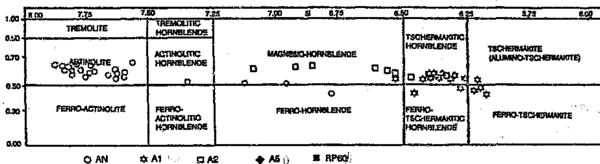
Figure 5.4: Leake (1978) amphibole nomenclature of calcic amphiboles: (Na + K)_A \geq 0.50p ; Ti < 0.50 ; Fe^{3+} \leq Al^{IV} .
