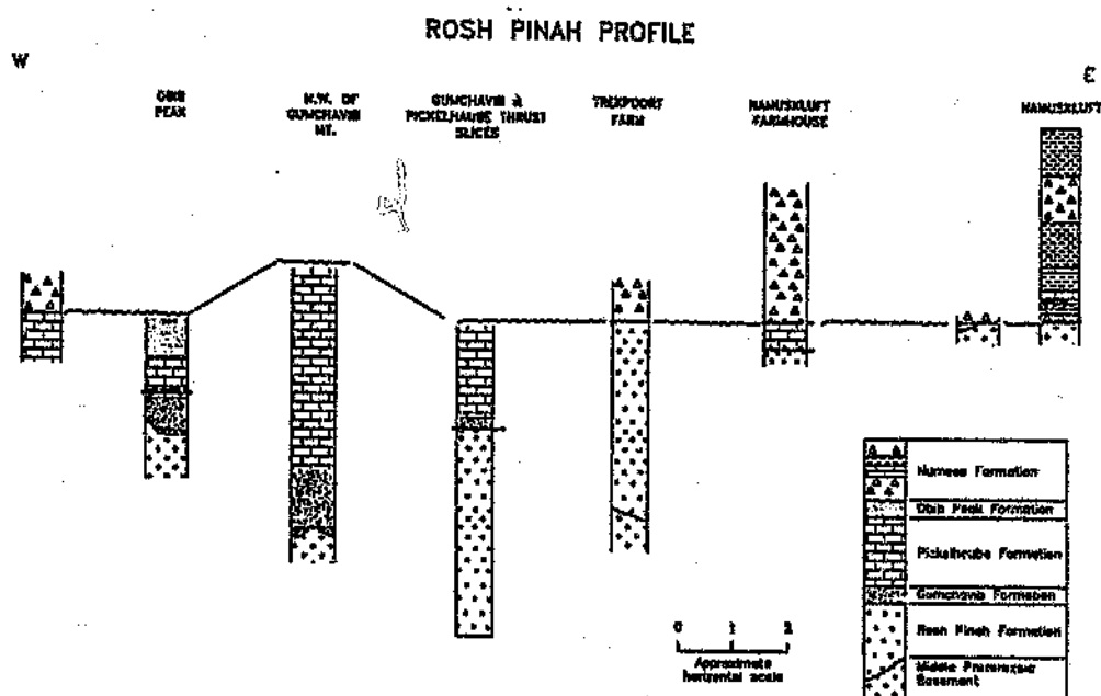
Fig. 6.6: Schematic diagram showing stratigraphic thickness variations within the study area (for locations see Figs. 1.2 and 2.4).
