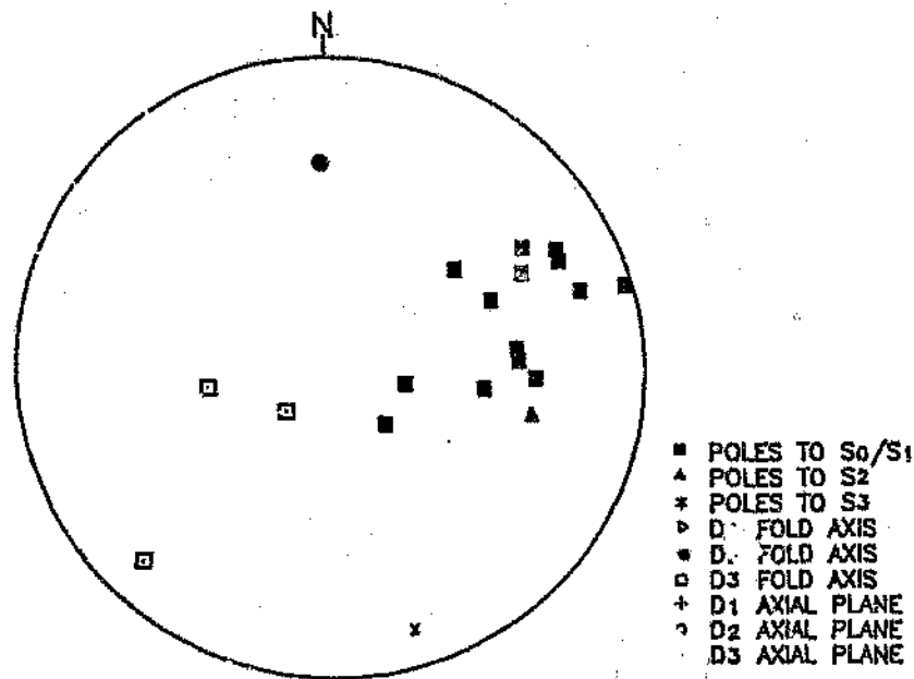
Fig. 4.14: Stereonet projections of structural data for the Rooikat thrust slice.
