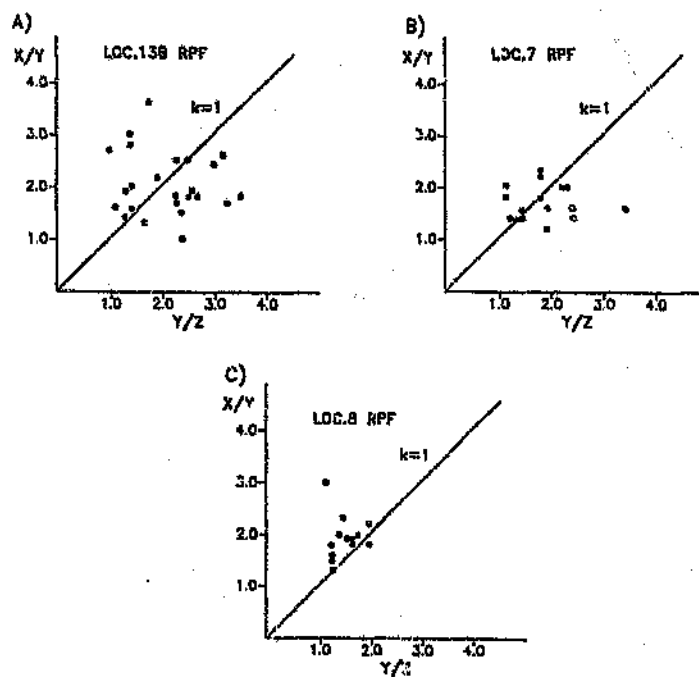
Fig. 4.34: Flnn plots of strain data from (A) locality 13B; (B) locality 7; and (C) locality 8 (localities are shown in Fig. 2.4).
