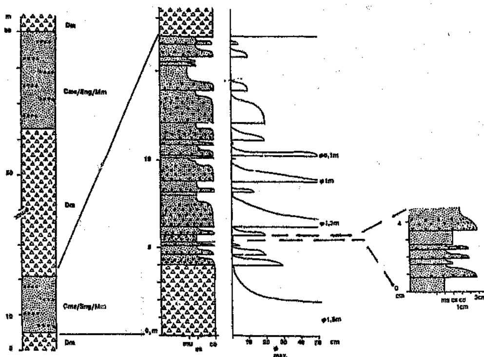
Fig. 3.50: Measured section through the graded beds of the conglomerate/sandstone/mudstone facies association within the Numees Formation, about 2 km south-east of Namuskluft Farmhouse (Fig. 2.4).
