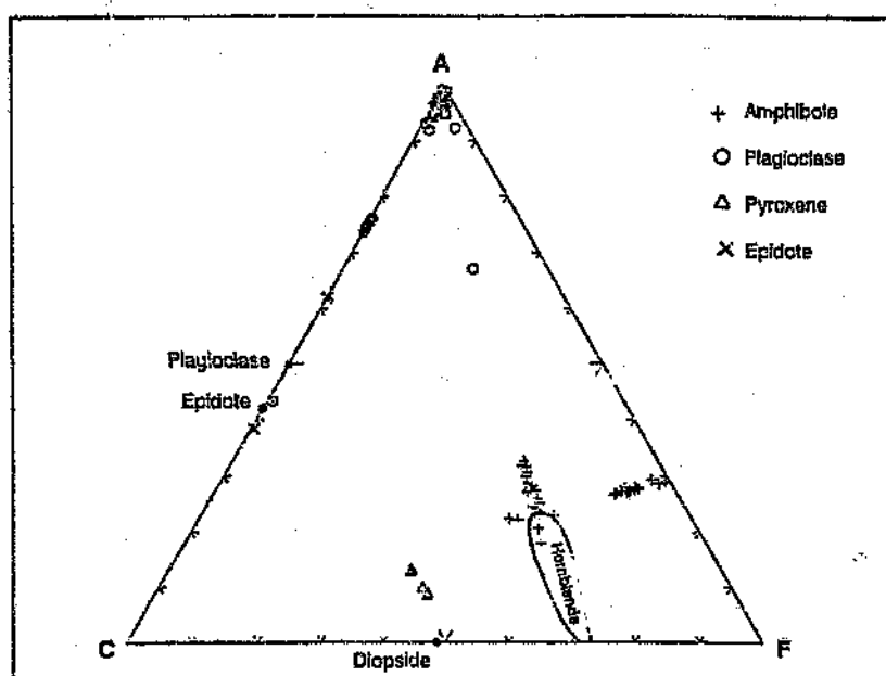
Figure 5.1: ACF diagram showing mineral compositions within the amphibolites.
