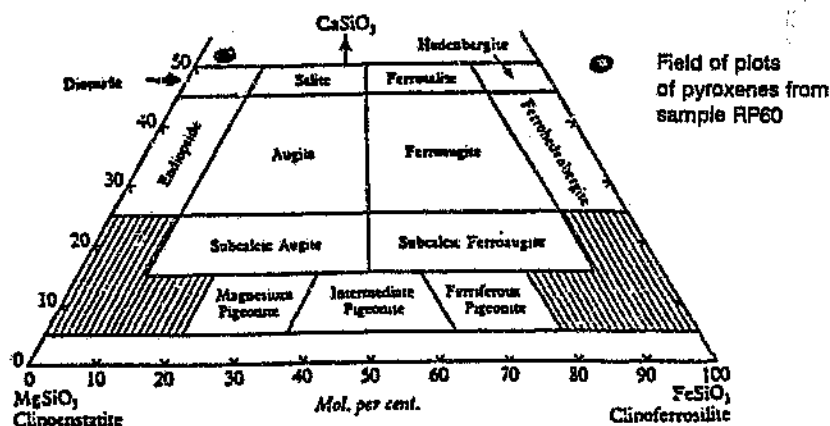
Figure 5.3: Nomenclature of Clinopyroxenes in the system \text{CaMgSi}_2\text{O}_6 - \text{CaFeSi}_2\text{O}_6 - \text{Mg}_2\text{Si}_2\text{O}_6 - \text{Fe}_2\text{Si}_2\text{O}_6 (after Poldervaart & Hess, 1951).
