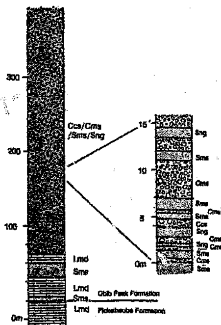
Fig. 3.41: Measured section through parts of the Obib Peak Formation at Obib Peak (Fig. 2.4); note the gradational contact to the underlying Pickelhaube Formation.
