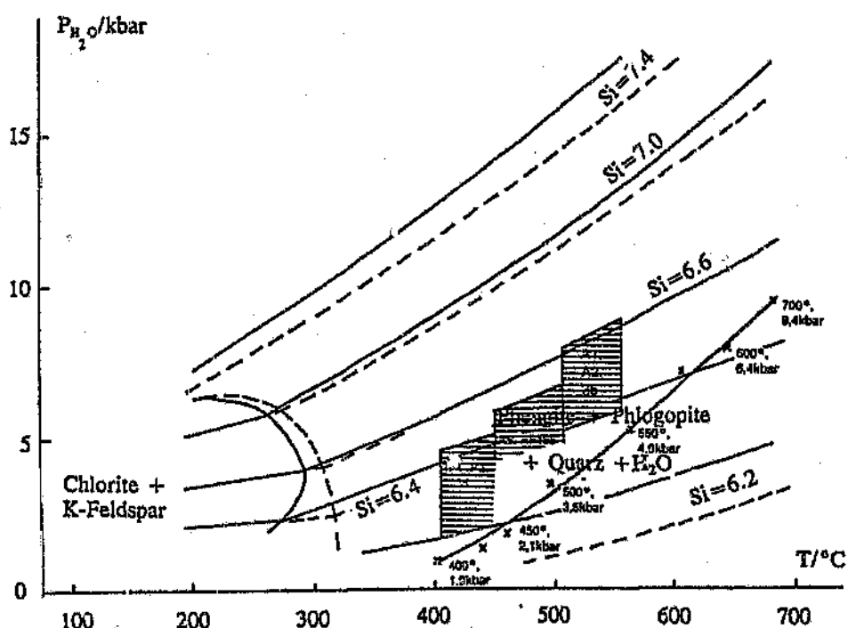
Figure 5.8: P-T diagram with "isoplethes" for Si-contents of phengites after Massone (1991); note great variability of pressures and temperatures of the investigated samples.
