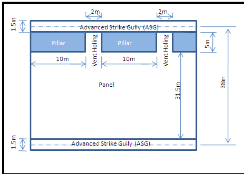
Figure 9 : Panels layout – rectangular sketch for simplicity
