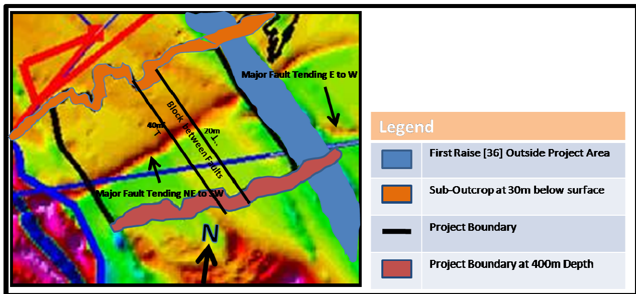
Figure 1 : Aerial magnetic survey (Courtesy of Anglo Platinum)
