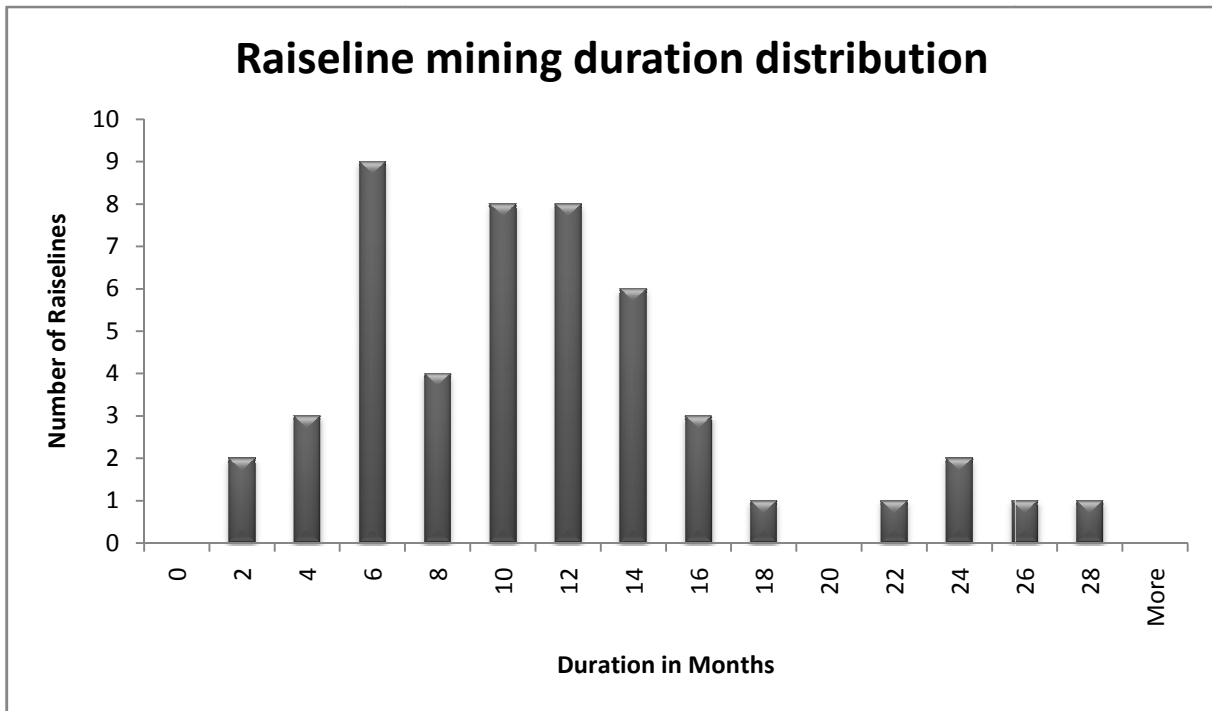
Figure 10: Histogram of mining durations of raiselines
