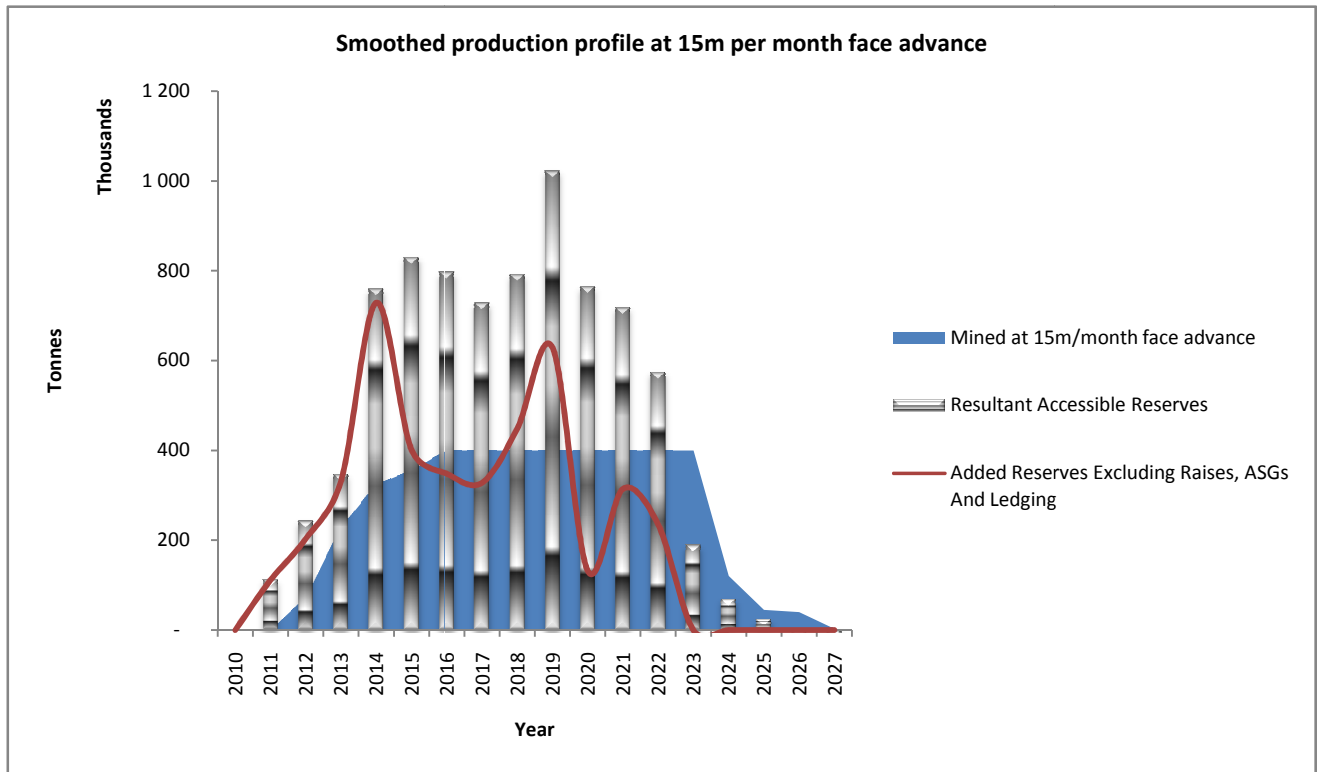
Figure 15 : Smoothed production profile at 15m per month face advance
