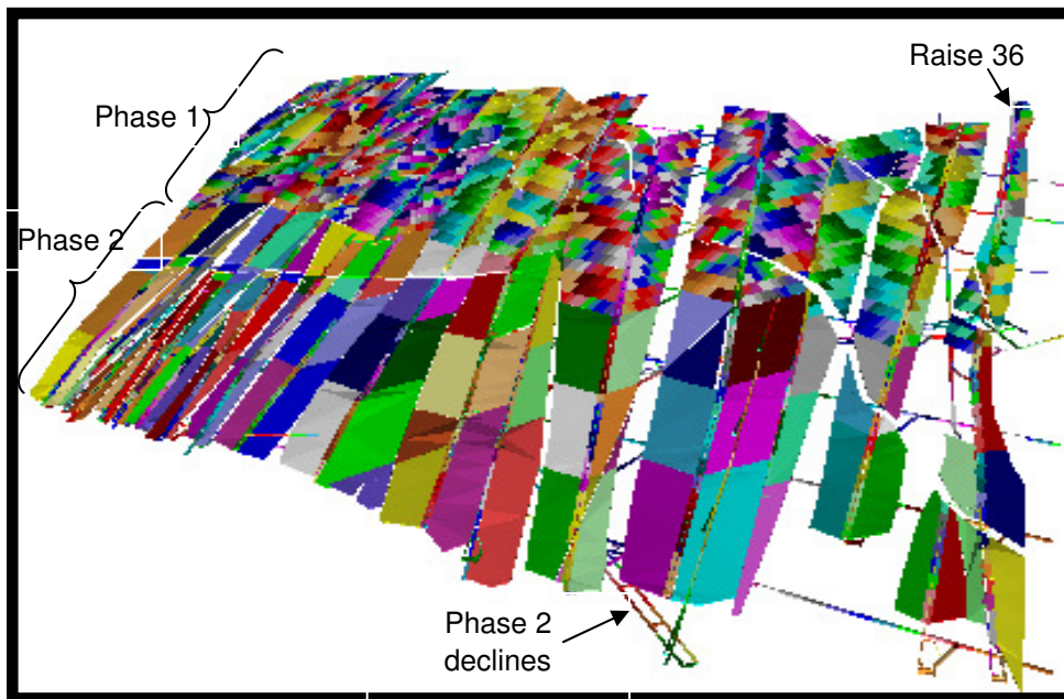
Figure 3 : A 3D perspective view of the project schedule in Mine2-4D®
