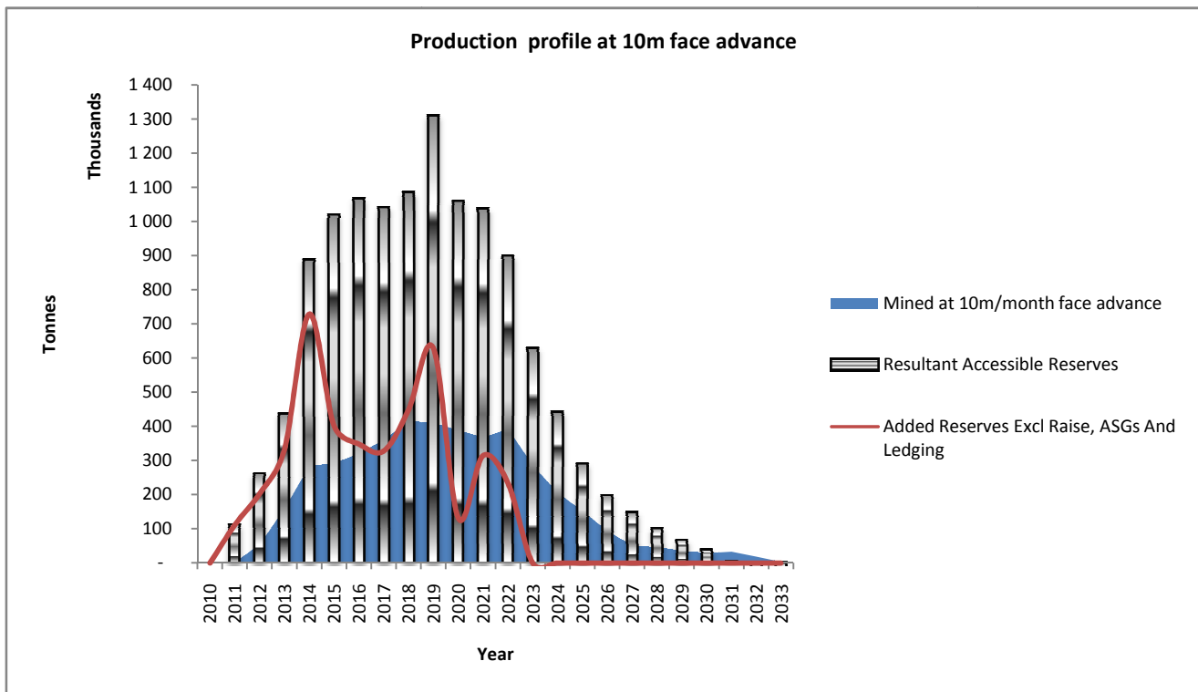
Figure 12 : Face advance of 10m per month
