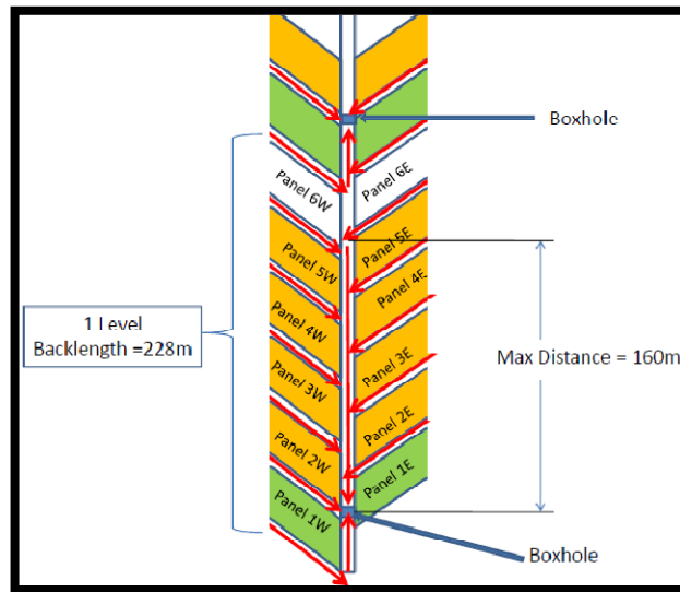
Figure 7 : Backlength planning for a raiseline
