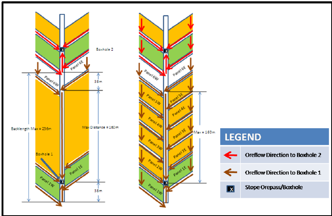
Figure 6 : Oreflow direction in production panels
