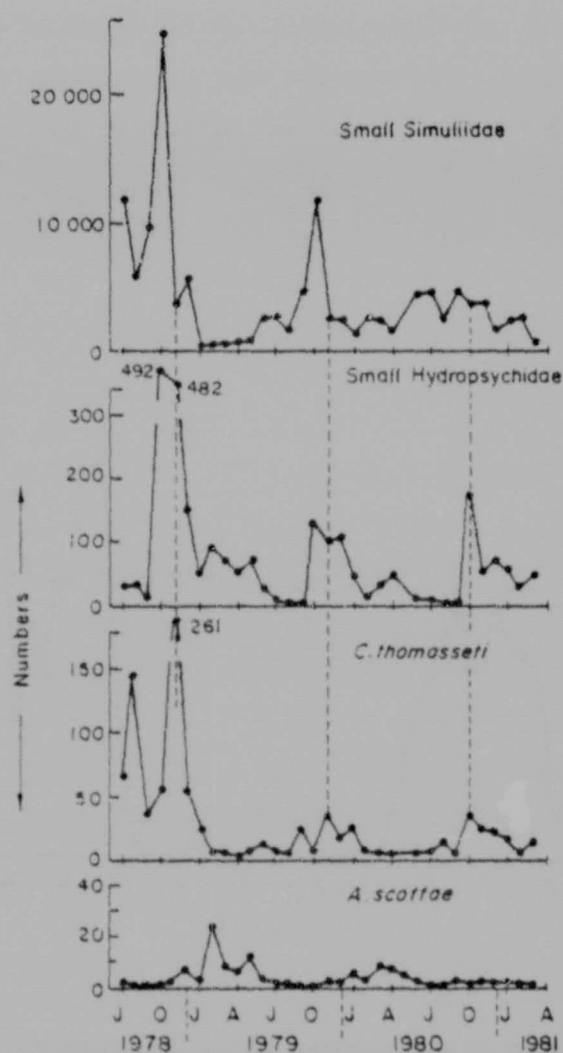
FIGURE 9: Numbers of Simuliidae and Hydropsychidae on stone samples collected at monthly intervals from July 1978 to March 1981. Counts are expressed as Sichel mean numbers per 1 000 cm 2 of stone surface area
