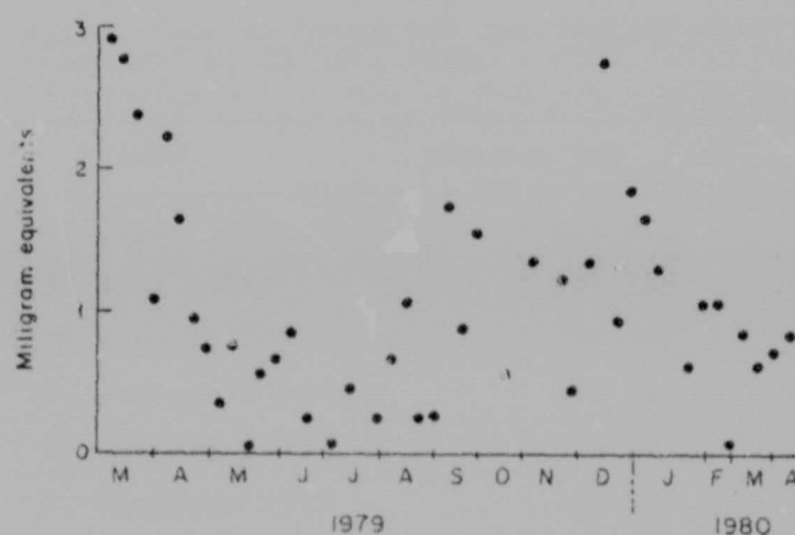
FIGURE 7: Estimated amount of particulate organic carbon in river water samples collected at weekly intervals from 10 March 1979 to 18 April 1980. Particulate organic carbon expressed as milligram equivalents of humic acid per litre of water
