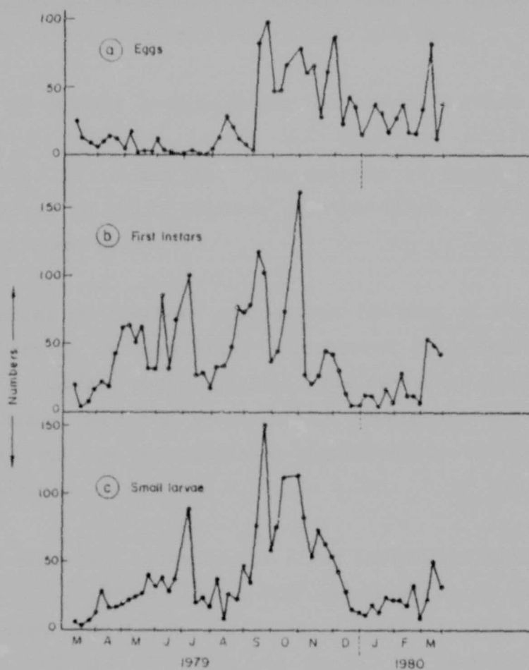
FIGURE 4: Numbers of Simuliidae encountered in 1 000 litres of drifting river water, samples collected upstream of the study rapid at weekly intervals from 4 March 1979 to 20 March 1980
