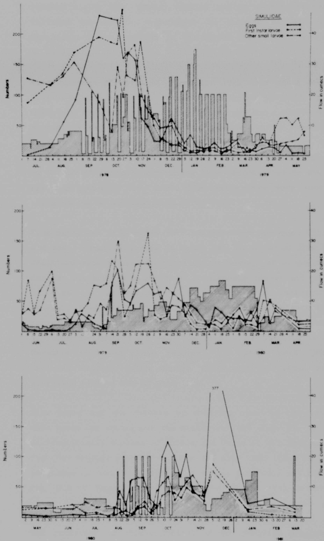
FIGURE 8: Numbers of drifting organisms per 1 000 litres of water and the flow of the Vaal River below the Vaalhartz Weir in cubic metres per second (shaded area) from July 1978 to March 1981
