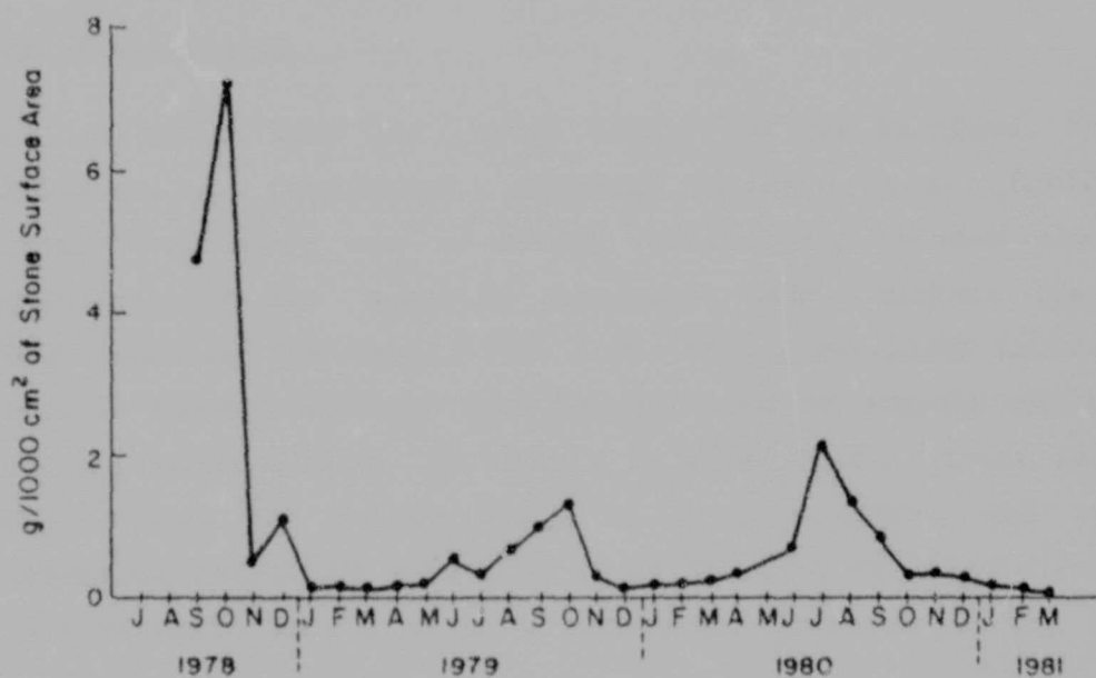
FIGURE 6: Dry weight biomass of the total number of Simuliidae on stone samples at monthly intervals between September 1978 and March 1981, biomass expressed in grams per 1 000 cm 2 of stone surface area
