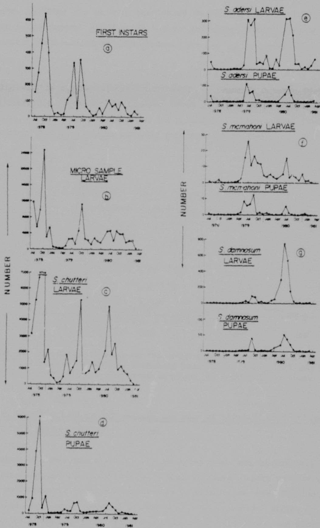
FIGURE 5: Numbers of Simuliidae on stone samples from the study rapid collected at monthly intervals from July 1978 to April 1981, counts expressed as Sichel mean numbers per 1 000 cm 2 of stone surface area
