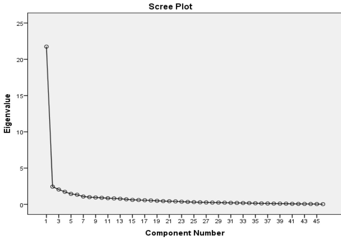
Figure 5.1: Scree plot showing the seven factors retained based on Eigenvalues >1 .
