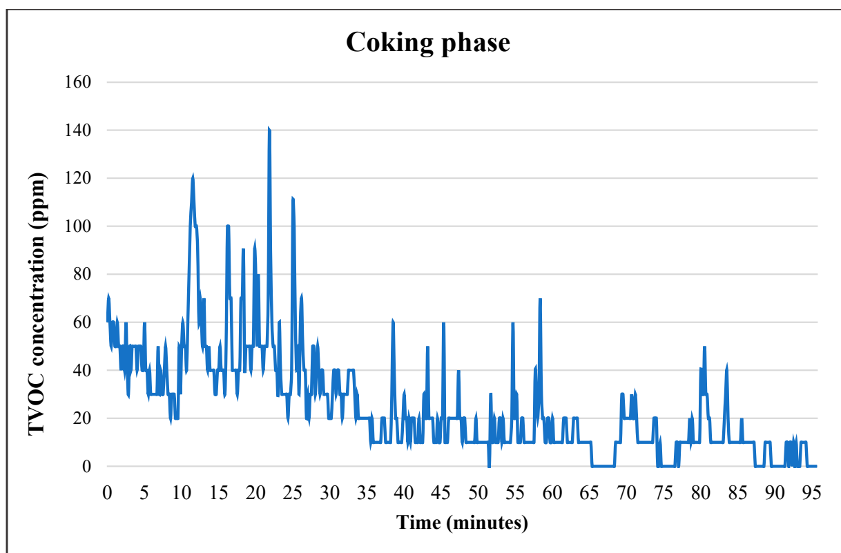
Figure 8. TVOCs during the coking phase.
