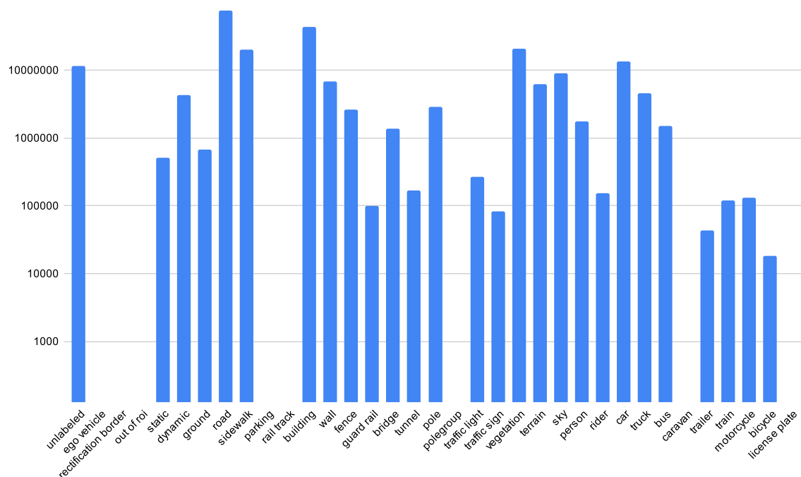
Figure B.1: Scaled Counts of Segmentation Labels from From Games Segmentation Data
