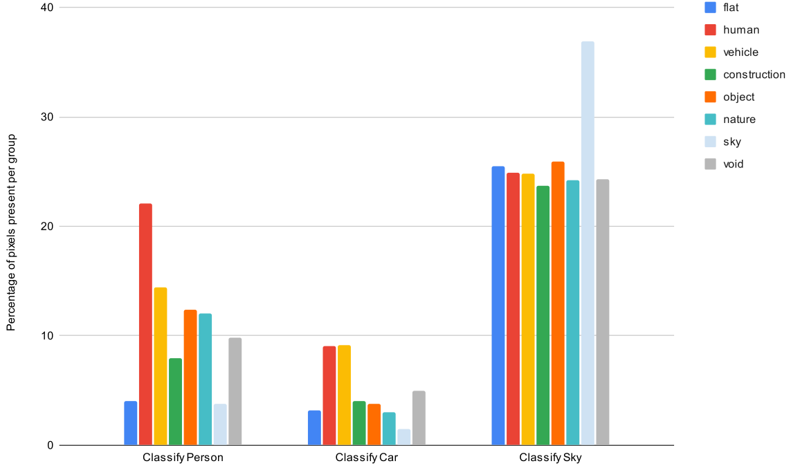
Figure 4.15: Comparison of the GradSUM Model Profiles for the Trained End-to-End Models (Using From Games Dataset)
