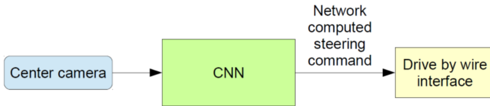
Figure 2.3: A general structure of an end-to-end autonomous vehicle system [Bojarski et al. 2016b]
