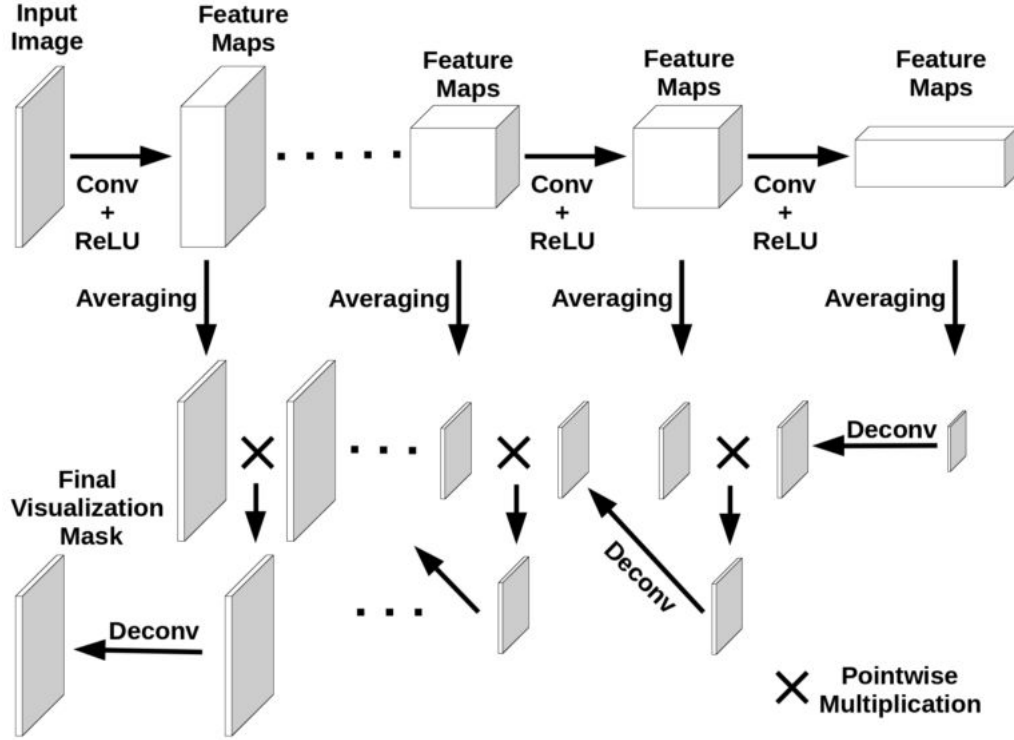
Figure 2.5: Diagram demonstrating the process of VisualBackProp [Bojarski et al. 2016a]
