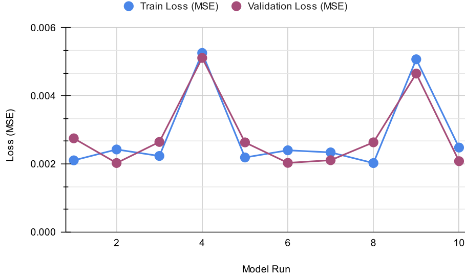
Figure 5.5: Comparison of Model Train Loss and Validation Loss
