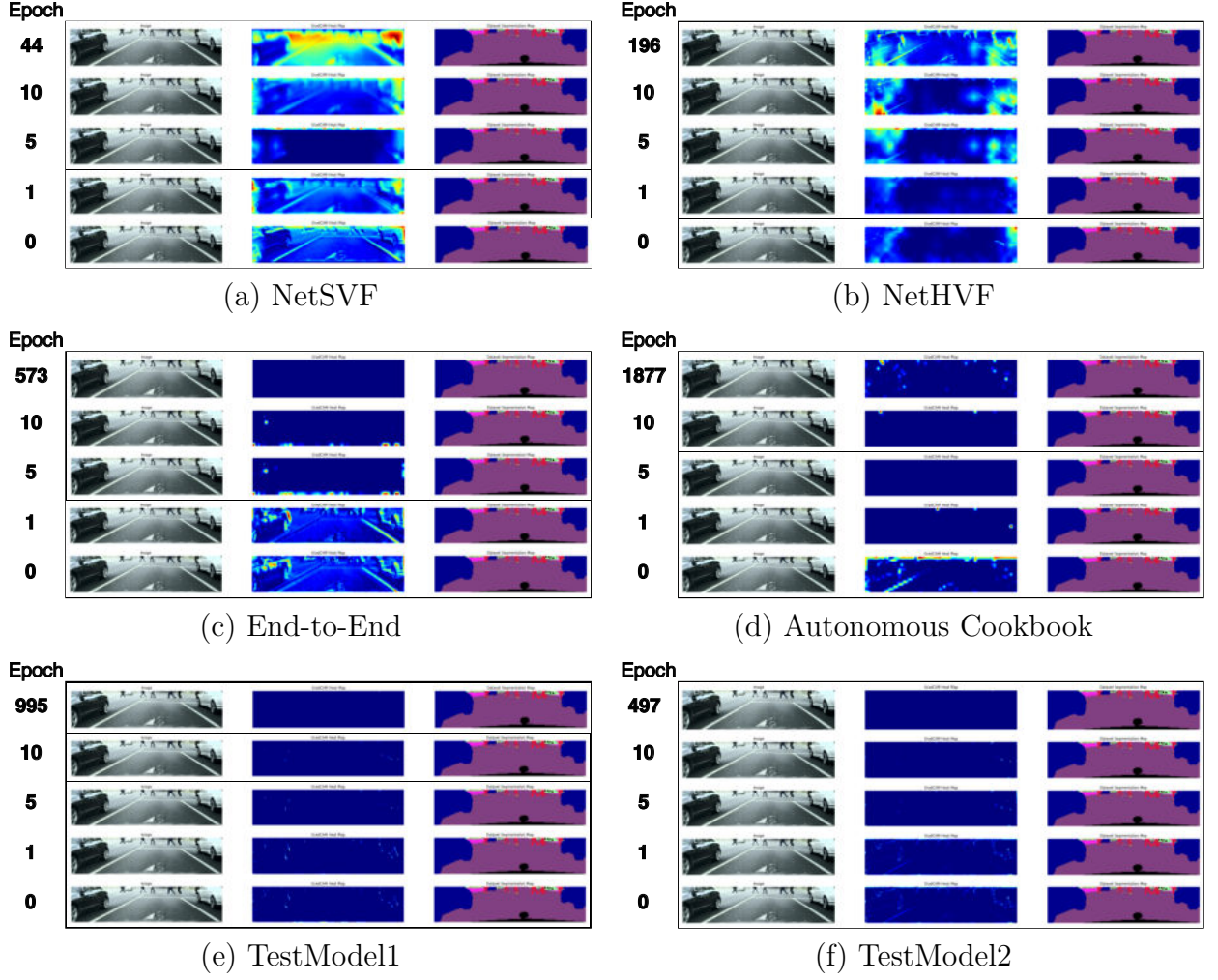
Figure 5.10: Examples of a single GradCAM export over each model over a series of epochs, where the models have been trained on the Udacity dataset
