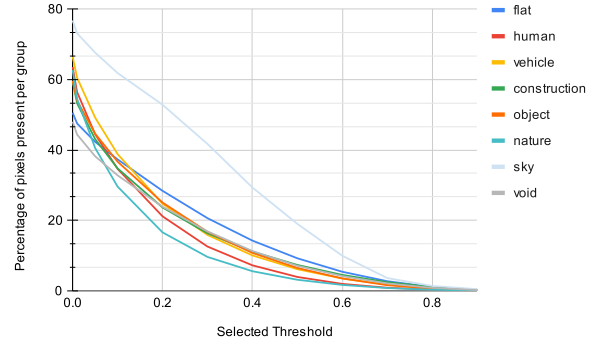
(b) Trends for each threshold (Epoch 1)
