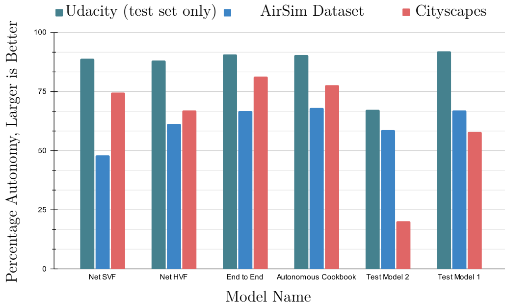
Figure 5.7: Comparison of Model Autonomy over Three Datasets
