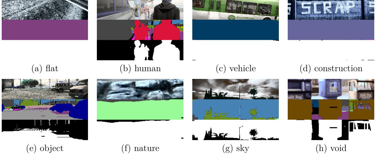
Figure 4.9: Examples of each group from segmentations. Three images are shown: the original cropped RGB image, the cropped segmentation map, and the binary map of the group
