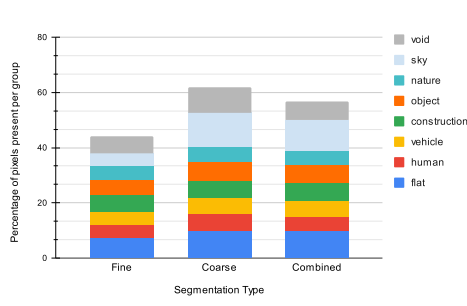
(a) Stacked Chart
