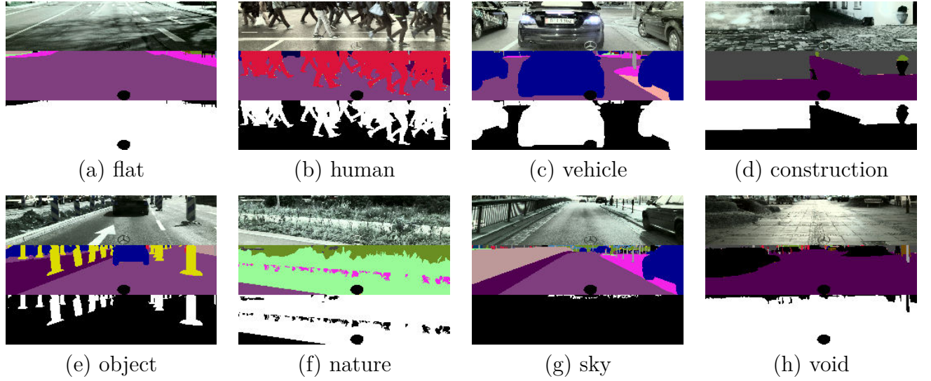
Figure 4.5: Examples of each group from segmentations. Three images are shown: the original cropped RGB image, the cropped segmentation map, and the binary map of the group
