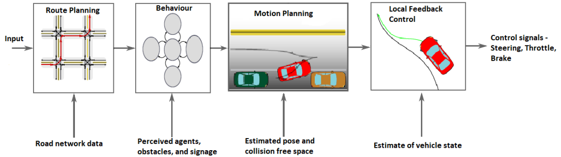
Figure 2.2: An example of a hierarchical autonomous vehicle system [Paden et al. 2016]
