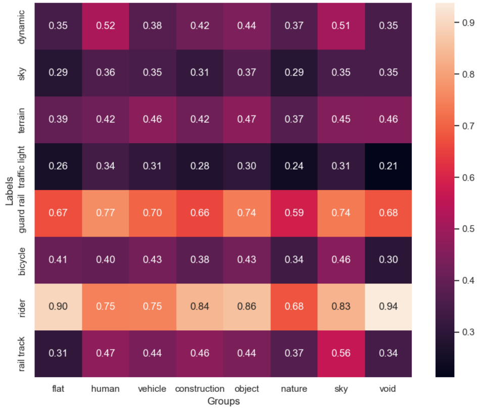
Figure 4.13: GradSUM Results (Percentages per Group) for 100 Random Models Solving the Binary Classification Problem (Averaged Results per Group)
