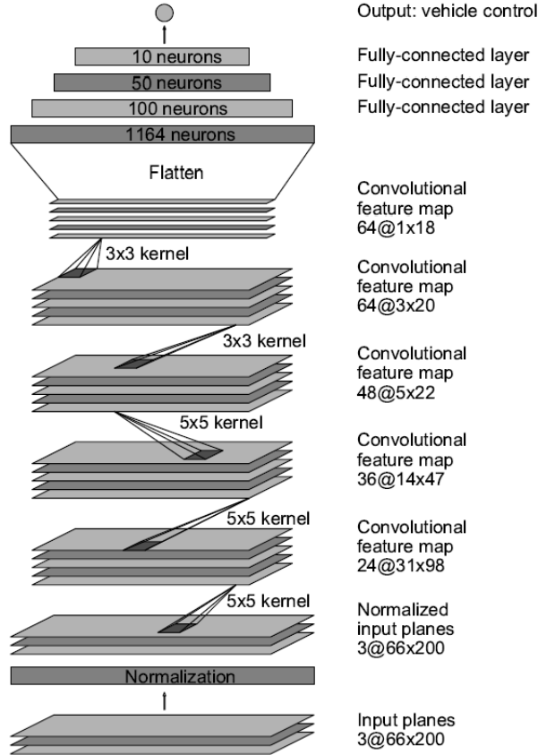
Figure 3.1: A diagrammatic representation of the model used in the article, End-to-End Learning for Self-Driving Cars [Bojarski et al. 2016b]
