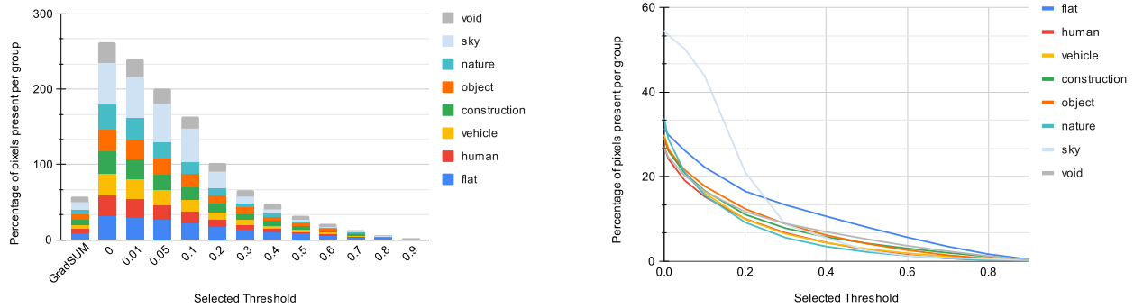
(a) Stacked chart for each threshold (Epoch 296) (b) Trends for each threshold (Epoch 296)
