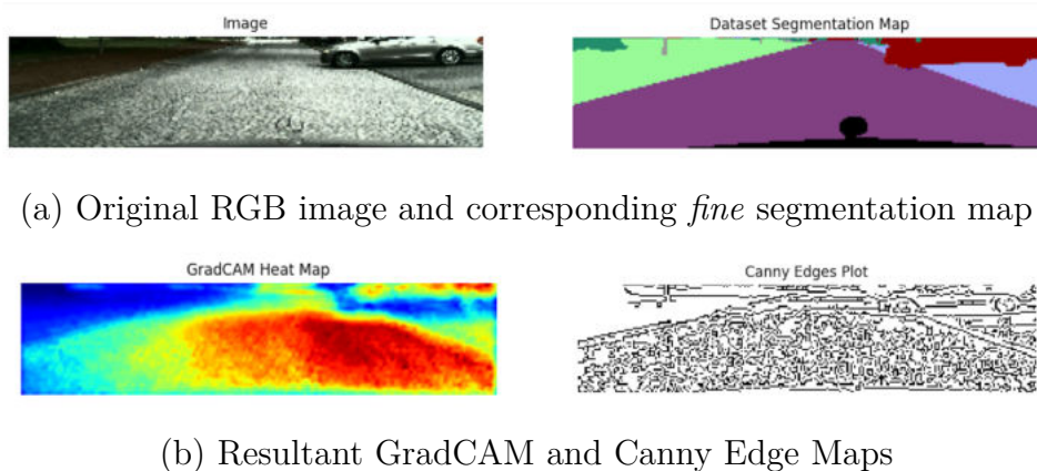
Figure 4.18: Example of a Canny Edge Map Generated on the Cityscapes Dataset
