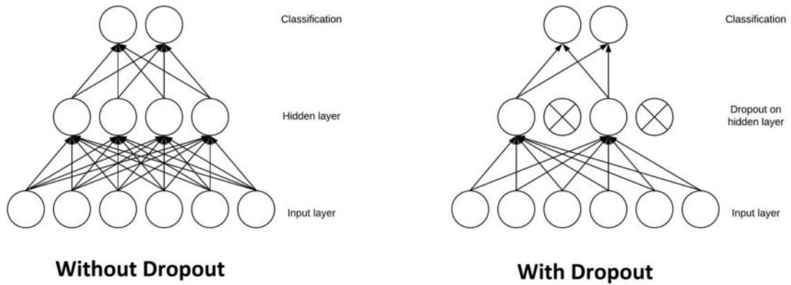
Figure 2.20: Example Neural Network With and Without Drop-out applied to Successive Layers [Baeldung 2023]
