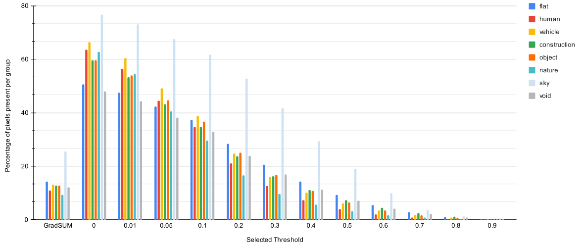
(c) Profiles generated for each threshold group and also GradSUM (Epoch 1)
