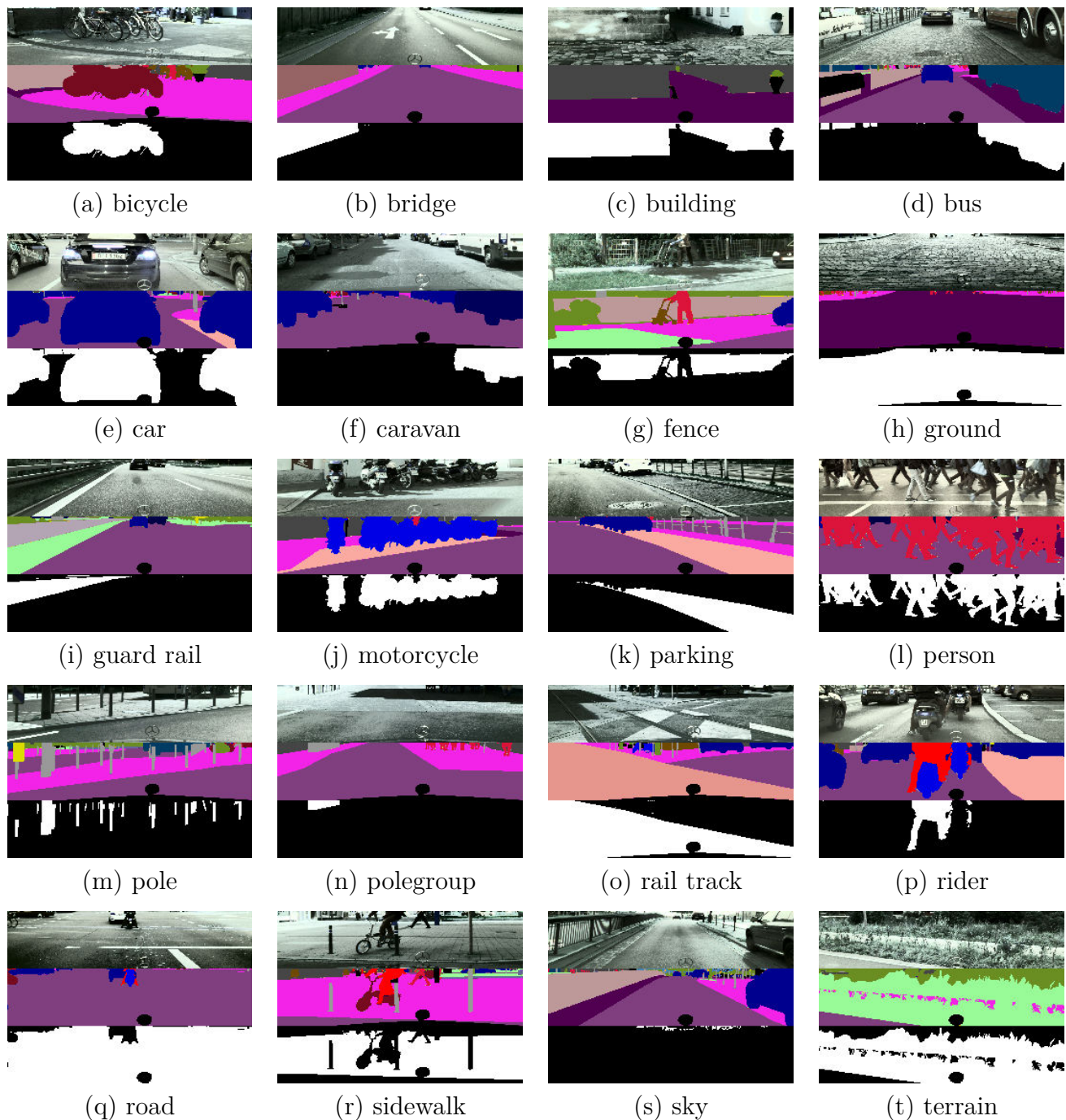
Figure A.2: Examples of Labels from Cityscapes. White represents the label. The original cropped frame, the segmentation map and the label map are shown
