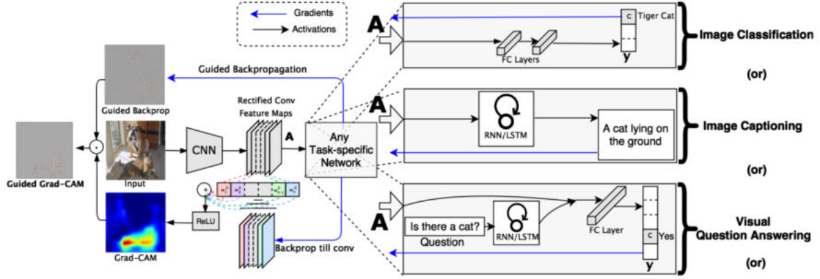
Figure 2.4: Diagram demonstrating the process of GradCAM [Selvaraju et al. 2016]
