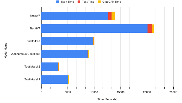
(b) Time Taken (Section (5.4.4))
