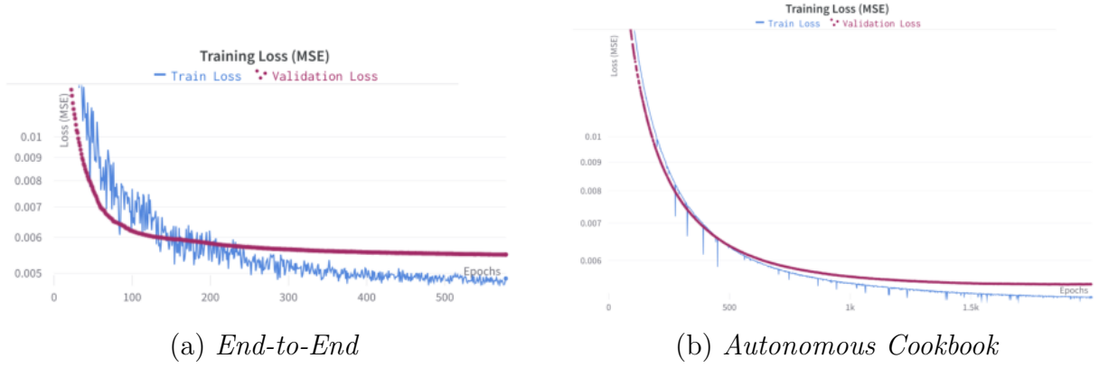
Figure 5.2: Comparison of training and validation loss per model (over each epoch) for the End-to-End and Autonomous Cookbook Architectures
