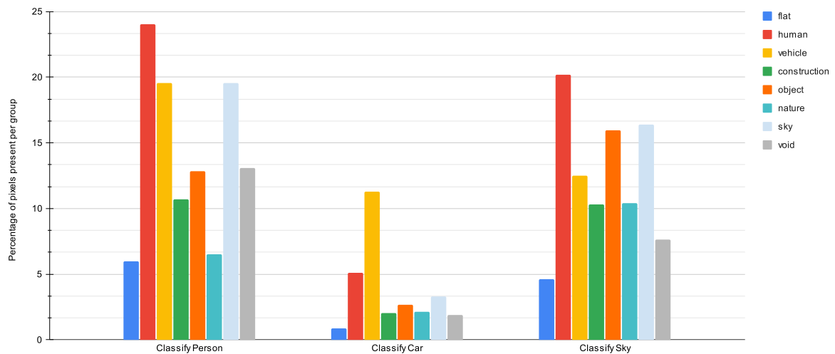
Figure 4.14: Comparison of the GradSUM Model Profiles for the Trained End-to-End Models (Using The Cityscapes Dataset)
