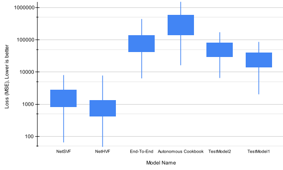
(a) Test Loss Results
