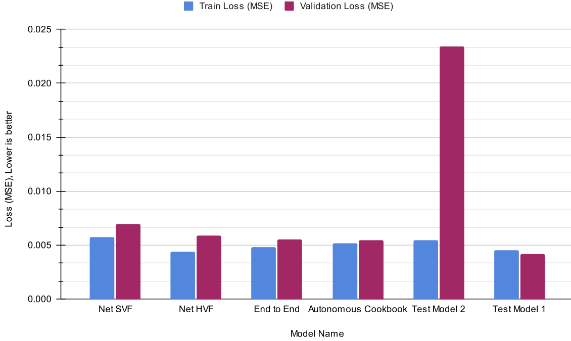
Figure 5.4: Comparison of Model Train Loss and Validation Loss
