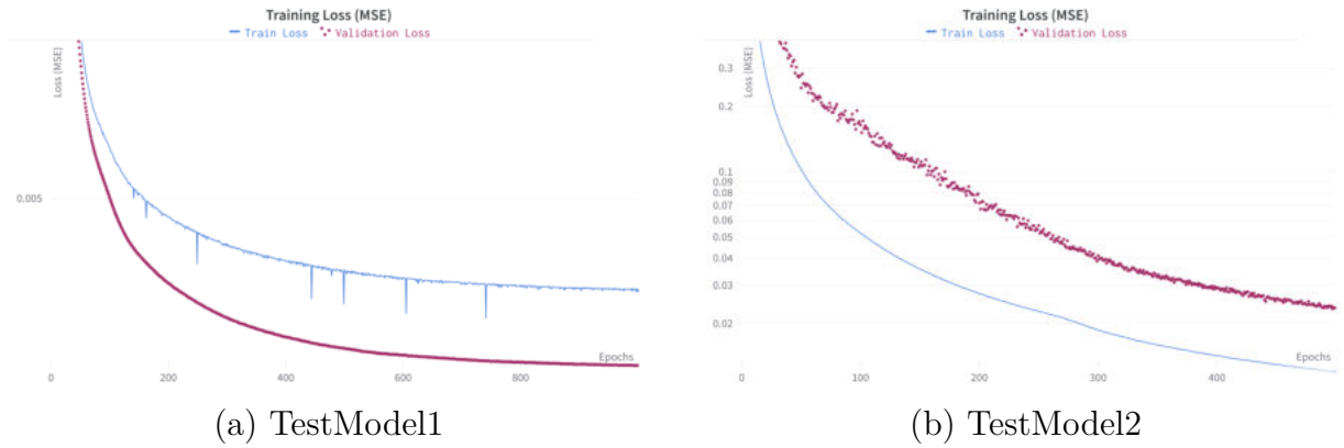
Figure 5.3: Comparison of training and validation loss per model (over each epoch) for TestModel1 and TestModel2 Architectures
