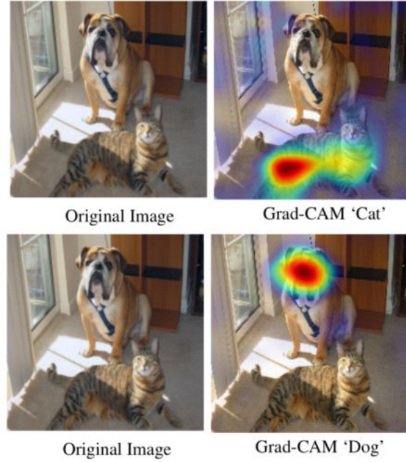
Figure 4.10: Example gradient maps produced by GradCAM [Selvaraju et al. 2016]
