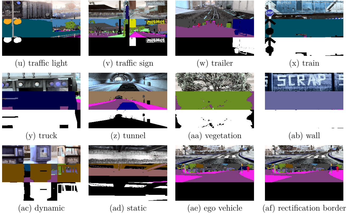
Figure B.3: Examples of Labels from From Games. White represents the label. The original cropped frame, the segmentation map and the label map are shown
