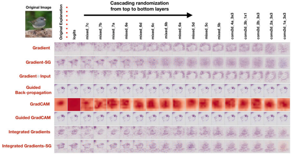
Figure 2.6: Cascading randomization results generated by Adebayo et al. [2018]
