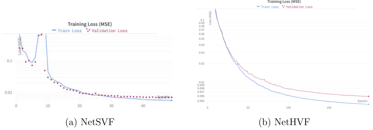
Figure 5.1: Comparison of training and validation loss per model (over each epoch) for NetSVF and NetHVF Architectures
