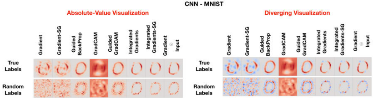
Figure 2.7: Data randomisation results generated by Adebayo et al. [2018]
