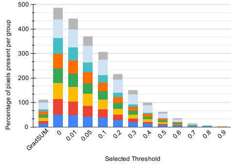
(a) Stacked chart for each threshold (Epoch 1)
