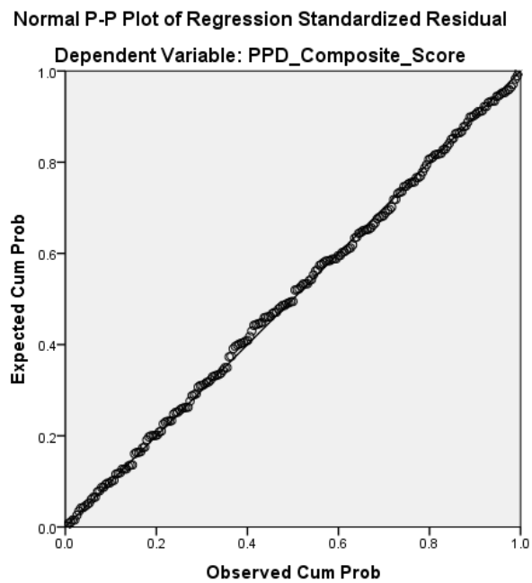
Figure 4-3: The QQ-Plot proving that the PPD data was normally distributed
