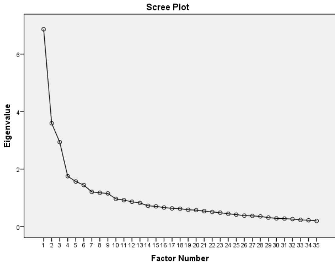
Figure 4-1: The Scree plot
