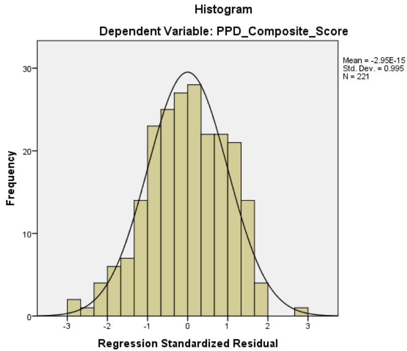
Figure 4-2: The histogram showing that data was normally distributed
