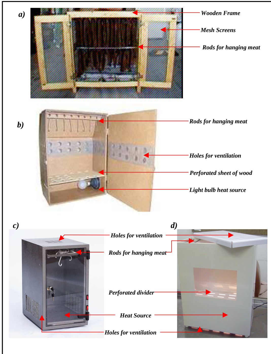
Figure 1.6: Biltong boxes commonly used for the drying of meats. a) Home-made enclosed cabinet (Anonymous, 2002), b) wooden home-made biltong box (Anonymous, 2002), c) commercially produced steel biltong dryer with a filament heat source (Anonymous, 2009e) and d) commercially produced perspex biltong dryer with a light bulb heat source.
