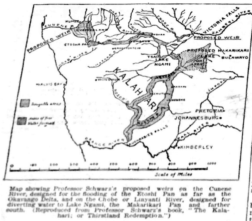
Figure 5.3.1.1: Map showing the proposed methodology of the Kalahari Scheme (After Moore, The Sunday Times , 11 August 1935).
