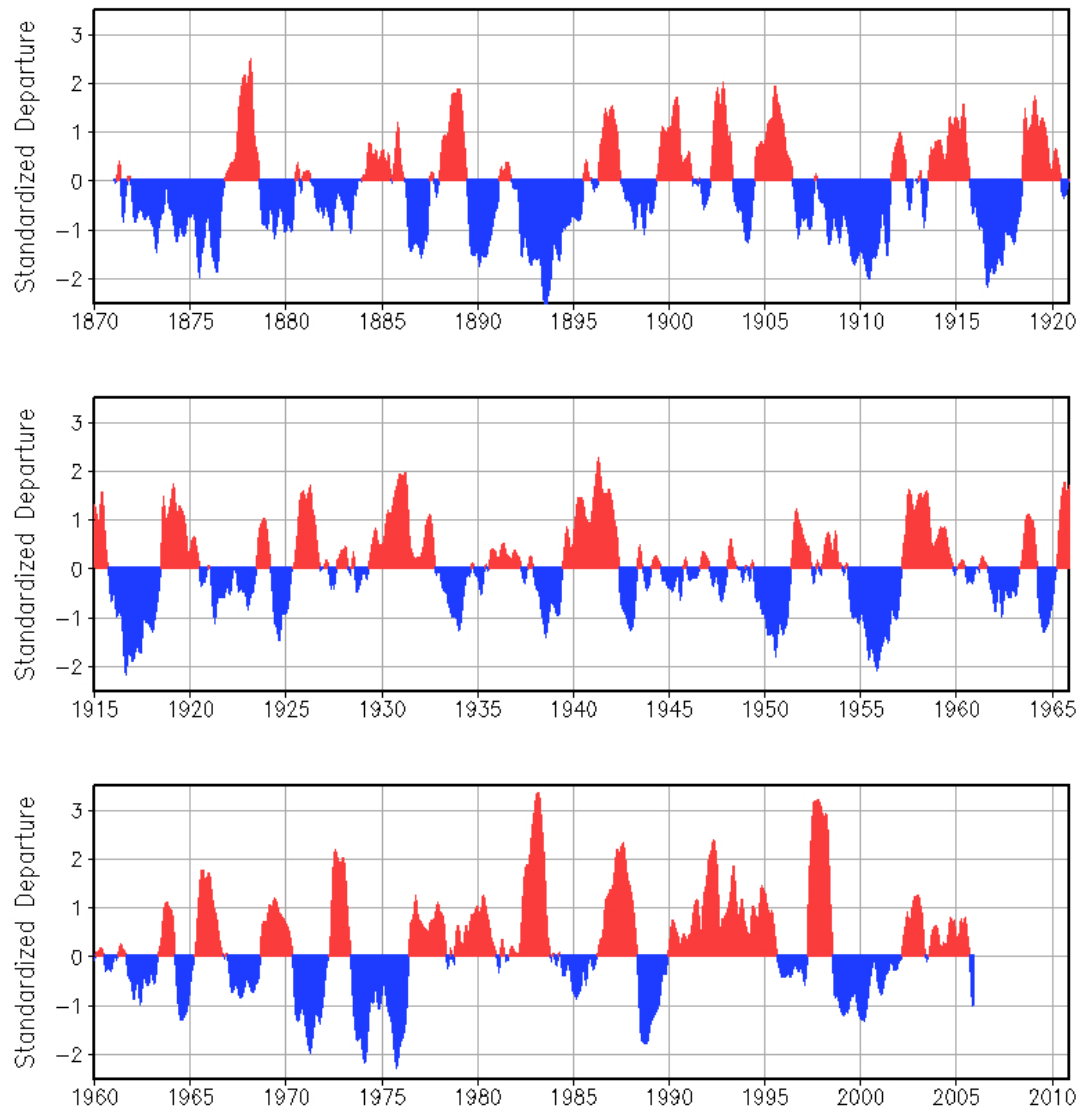
Figure 2.2.2: Extended Multivariate ENSO Index (MEI) (After Wolter and Timlin, 2011)
