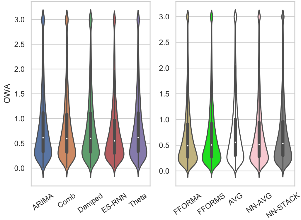
FIGURE 4.5: Yearly subset OWA distributions
