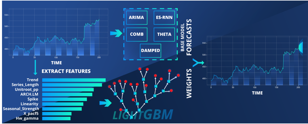
FIGURE 3.1: The proposed FFORMA forecasting pipeline.
