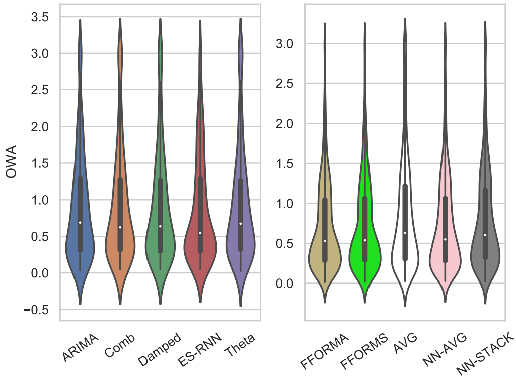
FIGURE 4.2: Weekly subset OWA distributions
