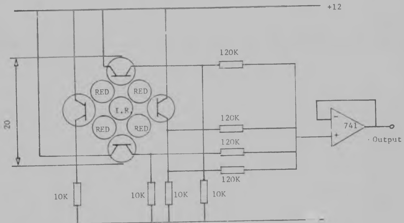
Figure 4.10 Transducer Using an Annulus of Detectors (Schematic)
