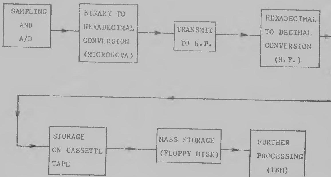
Figure A.4.1 The Data Handling Process
