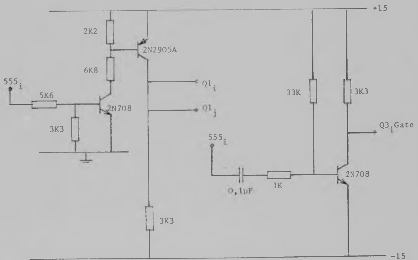
Figure 4.9 FET Drivers.
