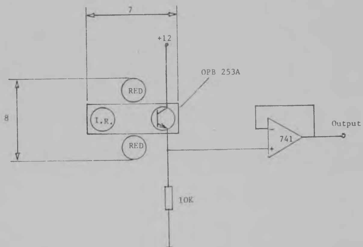
Figure 4.11 Schematic of Transducer Using an OPB 253A Reflective Sensor.
