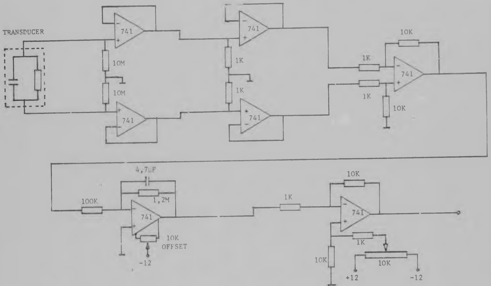
Figure 4.3 Circuit Diagram of Pulse Monitor.
