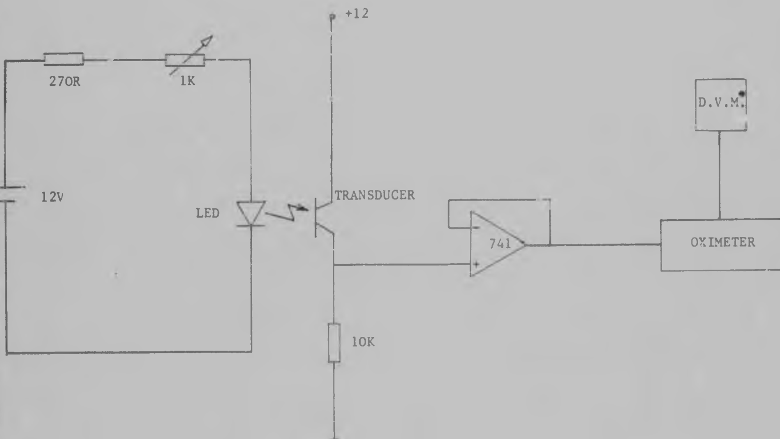
Figure 4.13 Experimental Setup for Checking Transducer Linearity.
