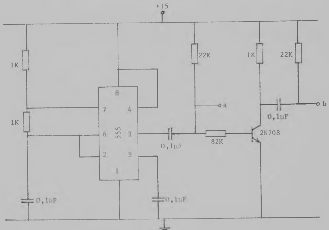
Figure 4.8 Oscillator.
