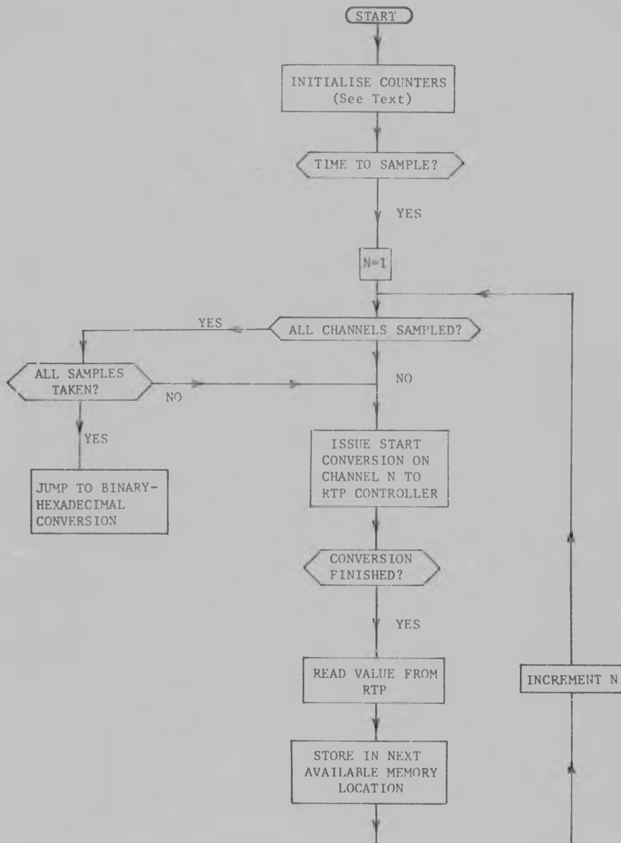
Figure A4.2 The Sampling Process.
