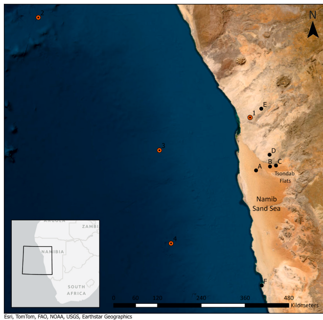
Fig. 1. Archaeological sites in the Namib Sand Sea and nearby, as discussed in the paper. A, Narabeb, B, Namib IV, C, Anibtanab (previously referred to as both Zebravlei and Mniszech's Vlei), D, Mirabib, E, Erb Tanks, F, Tsaui/Khaeb National Park (previously referred to as the Sperrgebiet). Also showing location of key palaeoenvironmental proxies for the region (used in Fig. 8), where: 1, Rössing Cave Speleothem (Geyh and Heine, 2014) and 2,3,4 are marine sedimentary cores containing proxies for terrestrial aridity: 2, MD98-2094 (Stuut et al., 2002), 3, MD08-3167 (Collins et al., 2014), 4, MD96-2098 (Daniau et al., 2023).
