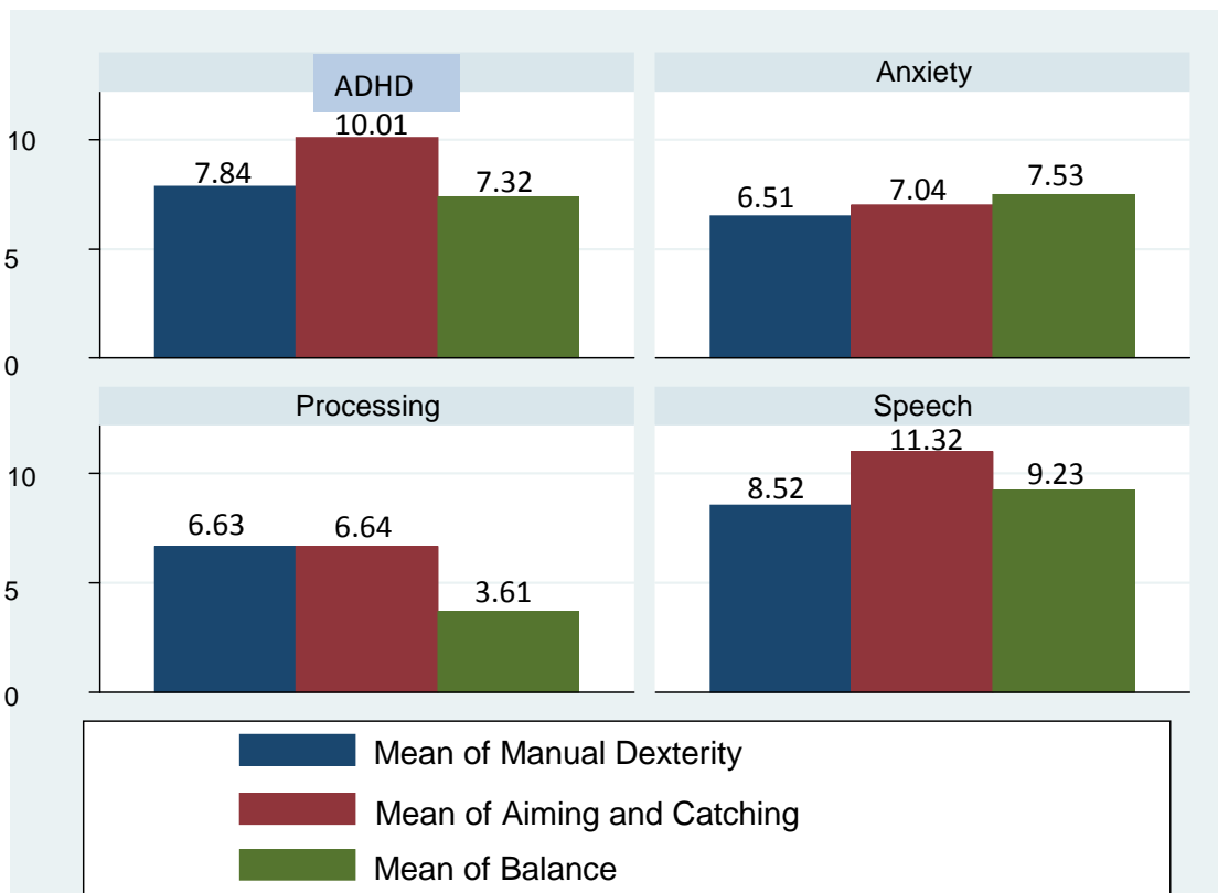
Figure 4.8 Bar graphs illustrating the mean standardise scores for each test component per each diagnosis
