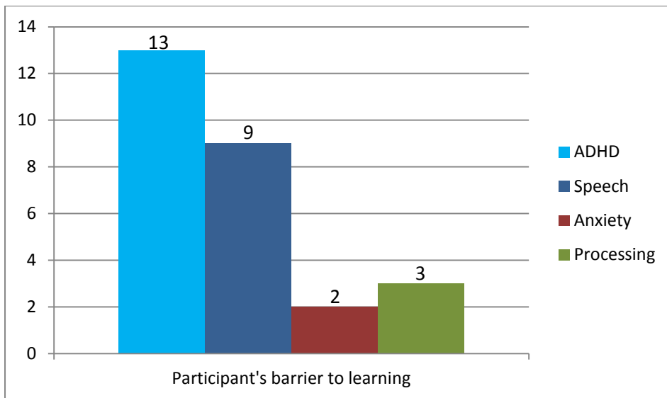
Figure 4.2 Bar graph children by diagnosis of intrinsic barriers to learning (n=27)
