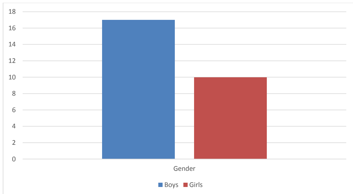
Figure 4.1 Bar graph illustrating the number of children by gender (n=27)
