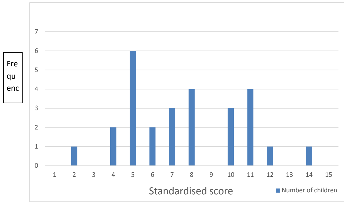
Figure 4.6 Histogram graph illustrating the frequency of standardise scores for Balance (n=27)
