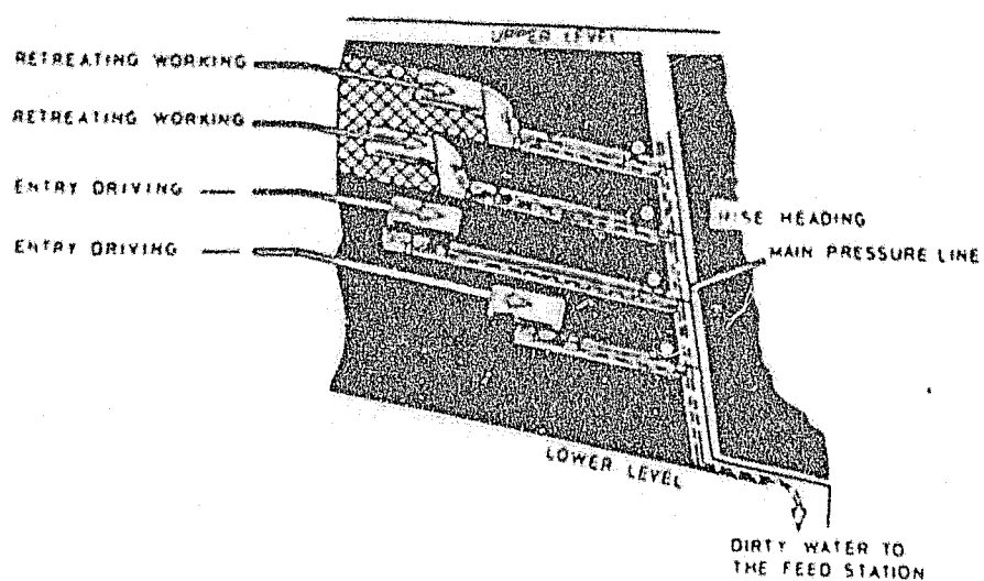
(c) Hydraulic mining (Milstein, 1979)
