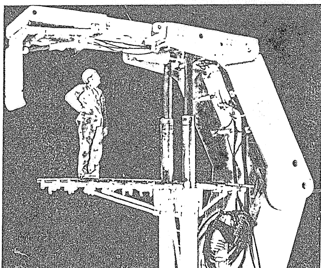
PLATE 2 Full face mechanised longwall support unit with elevated travelling way and face sprag.
