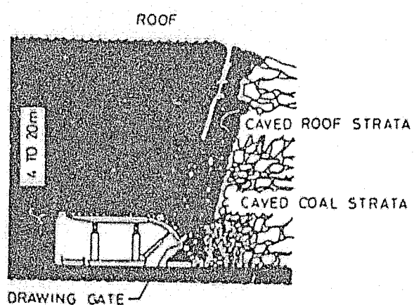
(a) Integrated mechanised longwall mining with sublevel caving (Barron, 1974)
