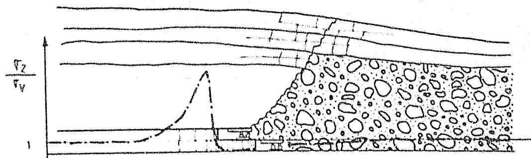
c) Simultaneous multi-slice longwall mining - faces in close proximity. The stress distribution profile at the upper floor strata horizon is almost identical to that associated with a single slice longwall operation. However, the lateral confinement offered to the floor strata of the upper longwall face is reduced significantly.
