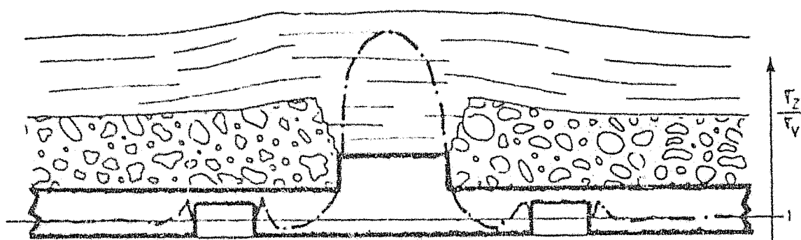
(b) Adjacent upper panels extracted. Panel entry development for adjacent lower slices. Upper slice interpanel pillar formed.
