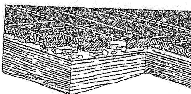
(b) Sublevel caving and drawing (Stoces, 1966)
