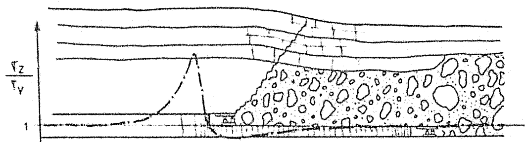
b) Simultaneous multi-slice longwall mining - faces far apart. The stress distribution profile at the upper floor strata horizon and the lateral confinement of the upper slice longwall face are almost identical to that associated with a single slice longwall operation.
