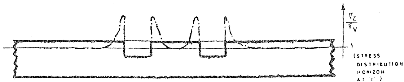
(a) Panel entry development for adjacent upper slices
