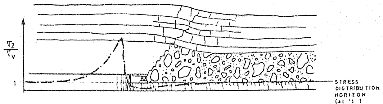
a) Single slice longwall mining - stress distribution profile at the floor horizon.
