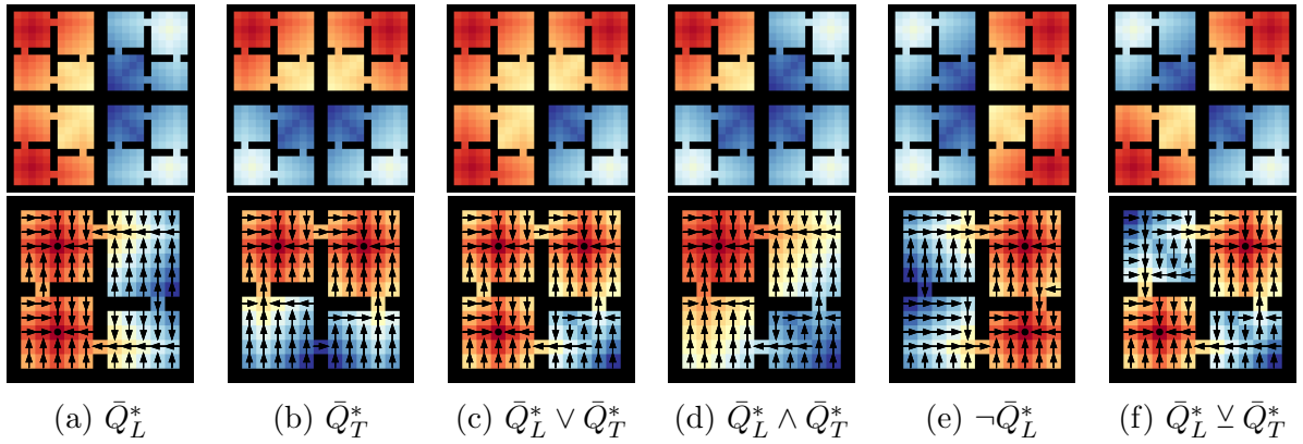
Figure 5.8: An example of Boolean algebraic composition using generated extended value functions of base deterministic shortest path tasks. Arrows represent the optimal action in a given state. (a–b) The generated optimal extended value functions for the base tasks. (c) Zero-shot disjunctive composition. (d) Zero-shot conjunctive composition. (e) Zero-shot negation. (f) Combining operators to model exclusive-or composition.
