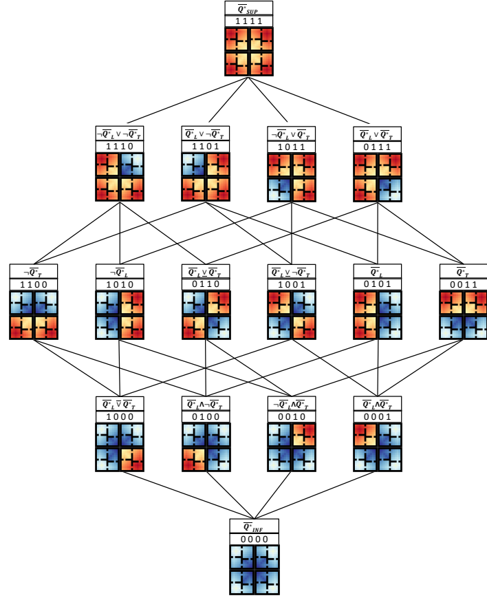
(b) Hasse diagram of the Boolean EVF algebra.
