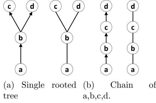
Figure 2.2: Example of a partial order and a well order. (a) Shows a partial order drawn as a directed graph and as a Hasse diagram. (b) Shows a well order also drawn as a directed graph and as a Hasse diagram. The Hasse diagram is drawn such that if a \leq b , then a \in \mathcal{L} is drawn below b \in \mathcal{L} . An edge is drawn between a and b if they are comparable and one covers the other. That is if say a \leq b and they are immediate neighbours.
