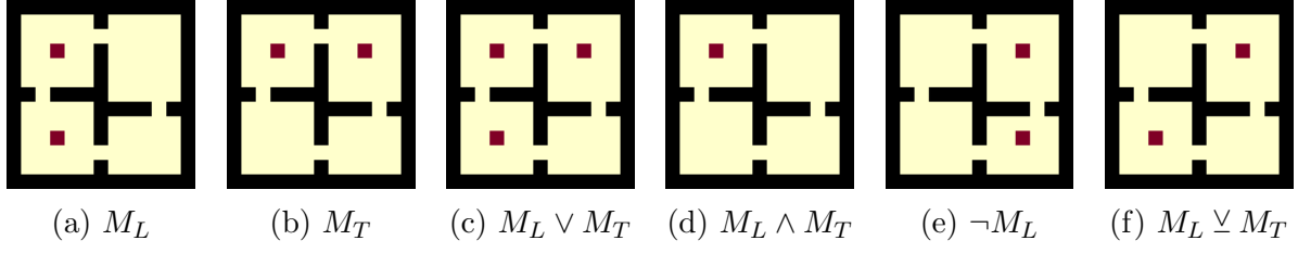
Figure 3.5: Showing task composition of base tasks in four-rooms domain. Figures (a)-(b) shows the rewards for the base tasks, (c)-(f) shows the rewards of the composed tasks. \oplus represents exclusive disjunction.
