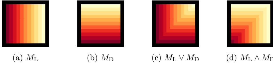
Figure 3.1: Rewards at terminal states for the disjunction and conjunction of tasks in gridworld domain (any position becomes terminal if the agent chooses to stay in it). All internal rewards are r_{\text{MIN}} . Figures (a)-(b) shows the dense goal rewards for the left and down tasks. (c) shows the rewards of their disjunction. (d) shows the rewards of their conjunction.
