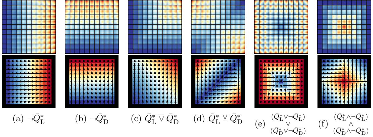
Figure 5.4: Showing the composition of EVFs learned from discounted tasks in gridworld domain. Figures (a)-(b) shows the values for the right and up EVFs, specified by the negation of the left and down EVFs respectively. (c)-(f) shows the values of the composed EVFs.
