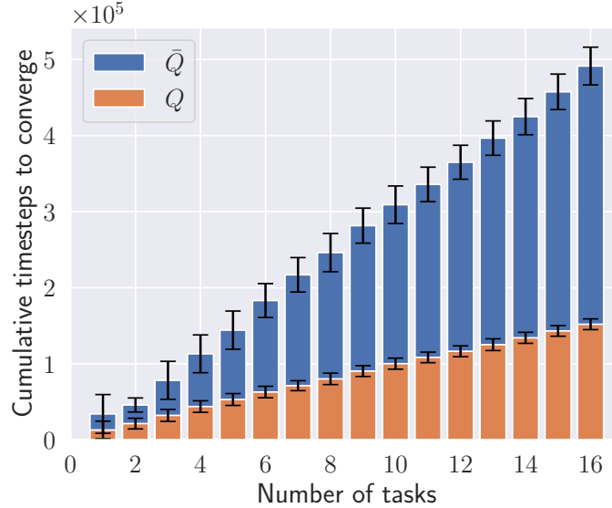
Figure 4.5: Cumulative number of samples required to learn optimal extended and regular value functions. Error bars represent standard deviations over 100 runs.
