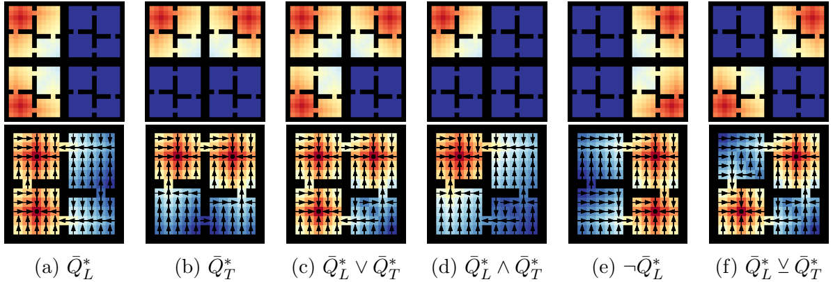
Figure 5.9: An example of Boolean algebraic composition using generated extended value functions of base discounted goal-reaching tasks. Arrows represent the optimal action in a given state. (a–b) The generated optimal extended value functions for the base tasks. (c) Zero-shot disjunctive composition. (d) Zero-shot conjunctive composition. (e) Zero-shot negation. (f) Combining operators to model exclusive-or composition.
