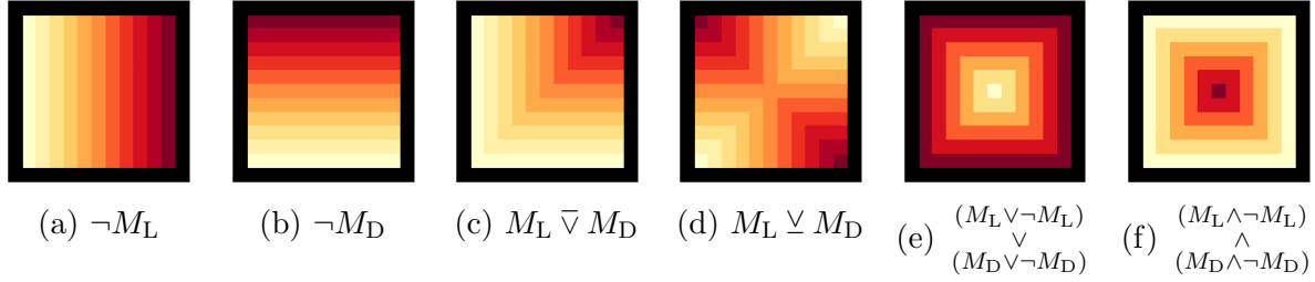
Figure 3.2: Rewards at terminal states for the composition of tasks in gridworld domain (any position becomes terminal if the agent chooses to stay in it). All internal rewards are r_{\min} . Figures (a)-(b) shows the rewards for the right and top tasks, specified by the negation of the left and down tasks respectively. (c) shows the rewards of the task specified by the negation of the disjunction of the left and down tasks— M_L \bar{\vee} M_D := \neg(M_L \vee M_D) . (d) shows the rewards of the task specified by the exclusive disjunction of the left and down tasks— M_L \vee M_D := (M_L \vee M_D) \wedge \neg(M_L \wedge M_D) . (e) shows the rewards of the task specified by the disjunction of the left, right, down and top tasks. (f) shows the rewards of the task specified by the conjunction of the left, right, down and top tasks.
