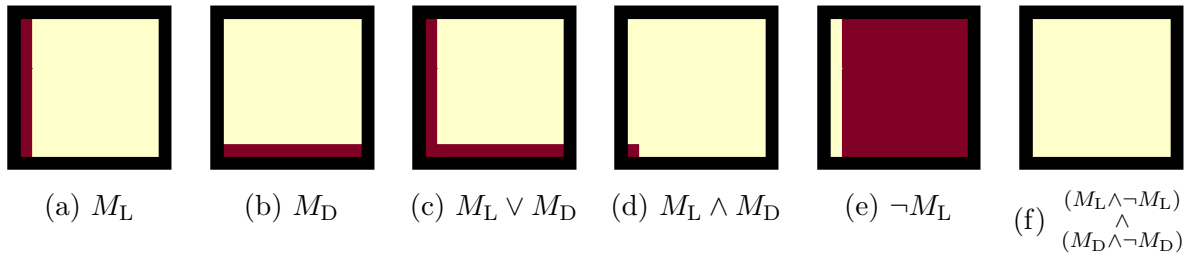
Figure 3.3: Showing composition of boolean tasks in gridworld domain. Figures (a)-(b) shows the Boolean goal rewards for the left and down tasks, (c)-(f) shows the rewards of the composed tasks.
