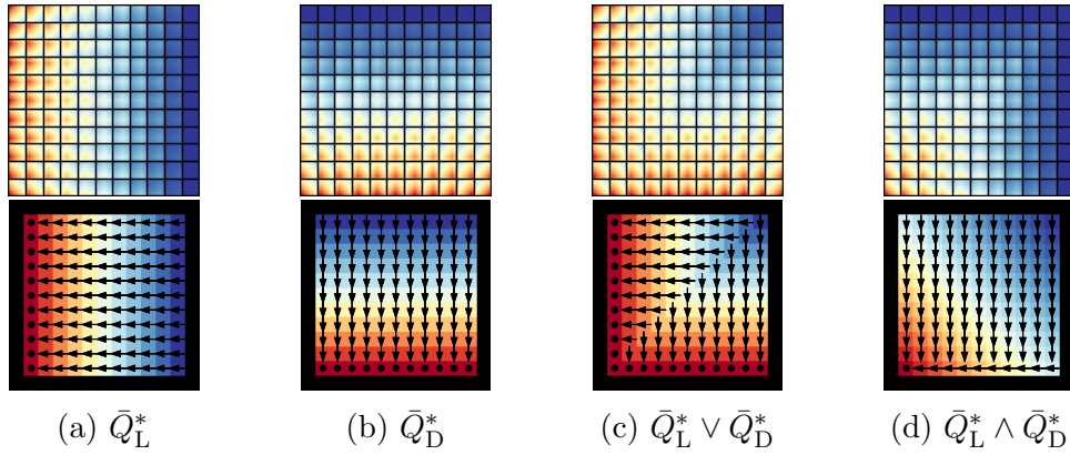
Figure 5.2: Showing the disjunction and conjunction of EVFs learned from discounted tasks in gridworld domain. Figures (a)-(b) shows the EVFs for the left and down tasks. (c) shows the EVF of their disjunction. (d) shows the EVF of their conjunction.
