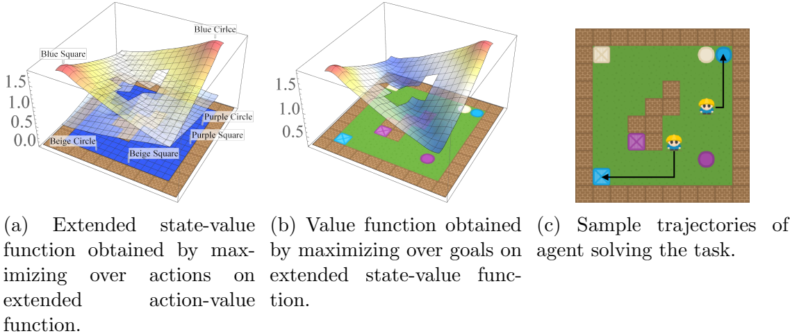
Figure 4.7: Learned EVF for the discounted goal reaching task of collecting blue objects in the video game domain. The EVF shows the value function with respect to each goal plotted on the same axis.
