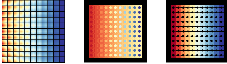
(a) Extended state-value function obtained by acting greedily over actions on extended action-value function. (b) Action-value function obtained by acting greedily over goals on extended action-value function. (c) State-value function and policy obtained by acting greedily over action-value function.
