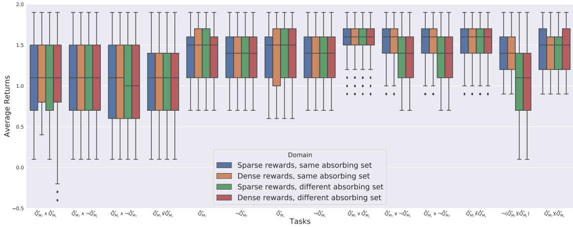
Figure 5.17: Box plots indicating returns for each of the compositional tasks, and for each of the four variations of the domain. Results are collected over 100000 episodes with random start positions.
