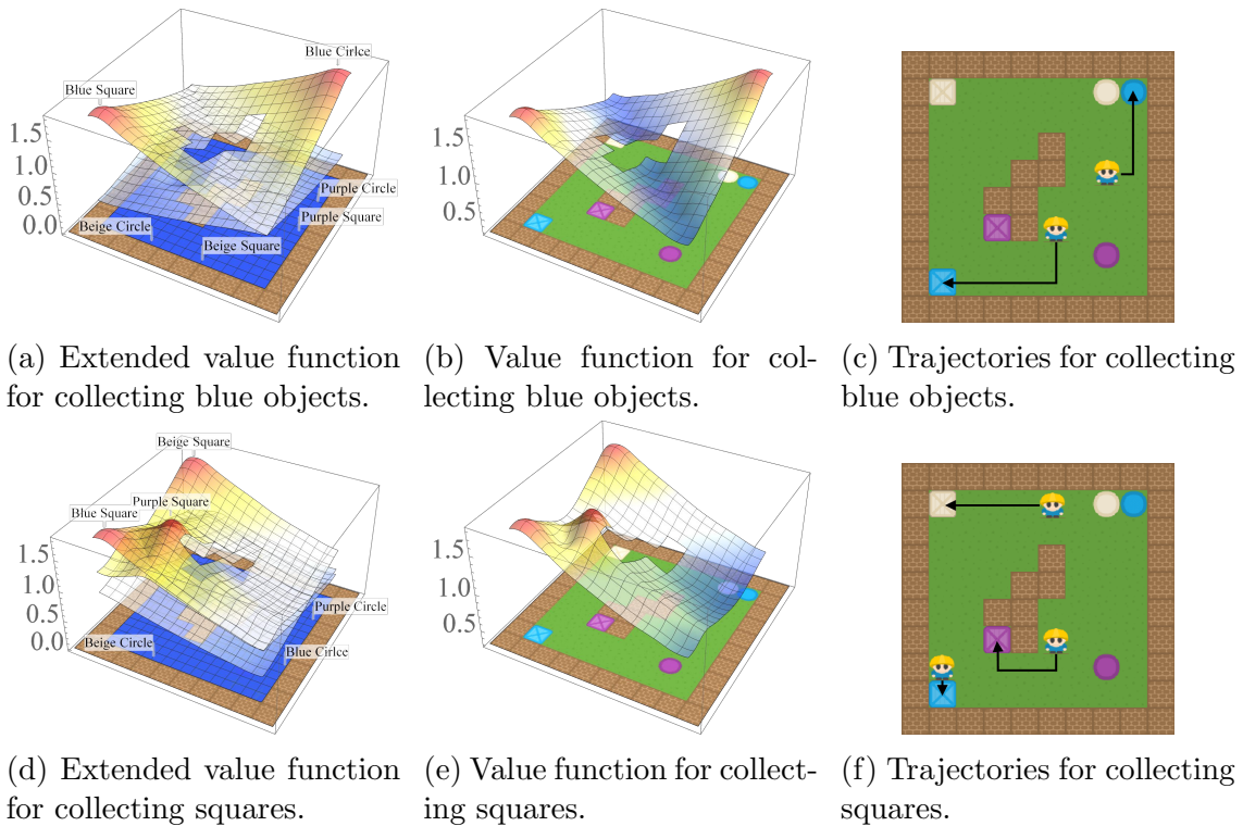
Figure 5.14: Base tasks for the video game environment in the discounted goal reaching setting. We show extended value functions learned for the blue, and square tasks.
