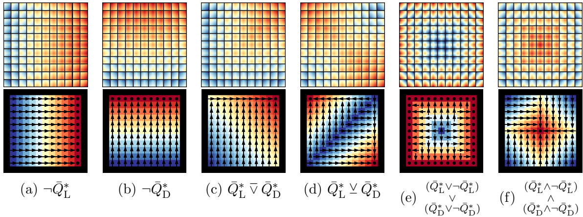
Figure 5.3: Showing the composition of EVFs learned from deterministic shortest path tasks in gridworld domain. Figures (a)-(b) shows the values for the right and up EVFs, specified by the negation of the left and down EVFs respectively. (c)-(f) shows the values of the composed EVFs.
