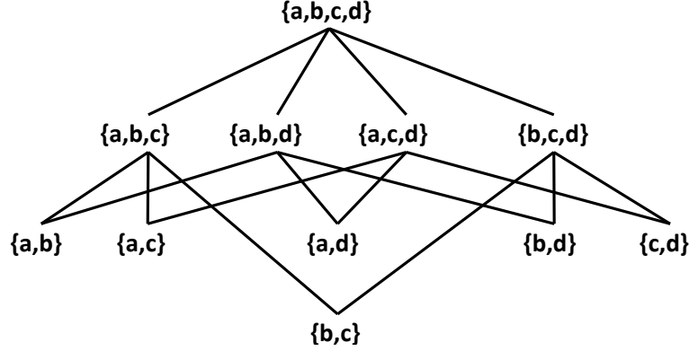
Figure 2.3: Join semi-lattice on subsets of \{a, b, c, d\} with at least 2 elements. The Hasse diagram is ordered by is a subset of .
