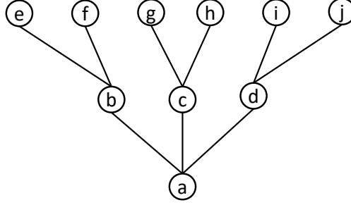
Figure 2.4: Meet semi-lattice induced by a tree with 10 nodes.
