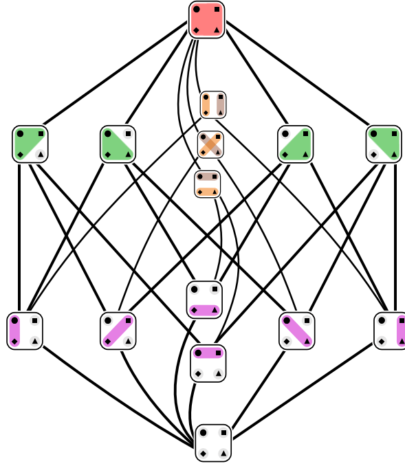
Figure 2.5: Hasse diagram of the partitions of a 4 element set.
