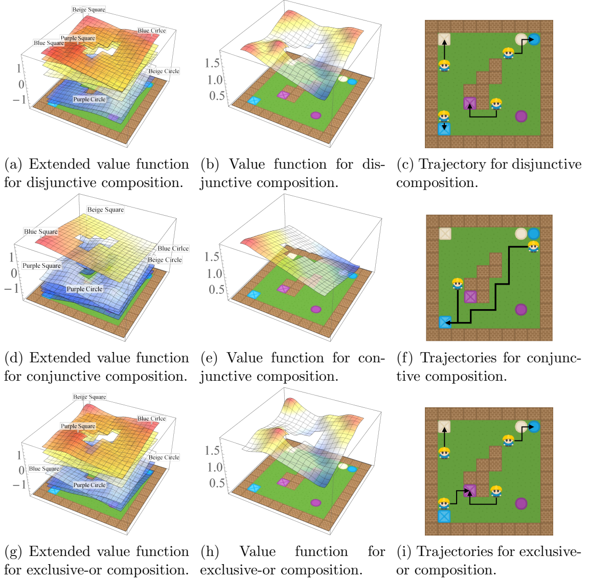
Figure 5.13: By composing extended value functions from the base deterministic shortest path tasks (collecting blue objects, and collecting squares), we can act optimally in new tasks with no further learning. The extended value functions shows the value function with respect to each goal plotted on the same axis. To generate this, we place the agent at every location and apply the element wise composition operators on the outputs of each network. We then compute the maximum over all actions for each goal. The points are interpolate between each other to smooth the graph. Any error in the visualisation is due to the use of non-linear function approximation.
