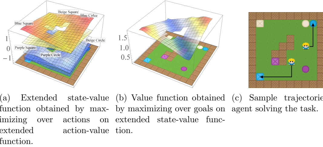
Figure 4.6: Learned EVF for the deterministic shortest path task of collecting blue objects in the video game domain. The EVF shows the value function with respect to each goal plotted on the same axis.
