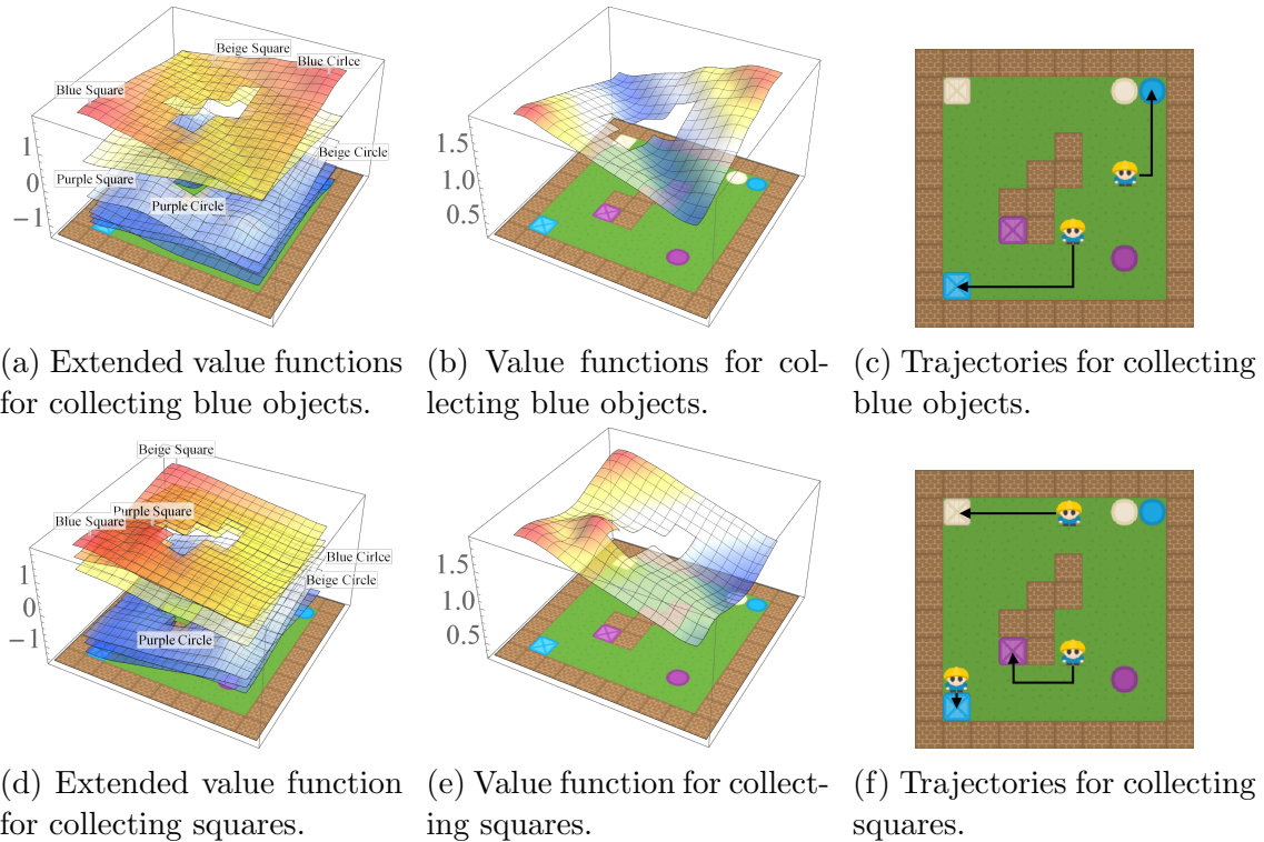
Figure 5.12: Base tasks for the video game environment in the deterministic shortest path setting. We show extended value functions learned for the blue, and square tasks.
