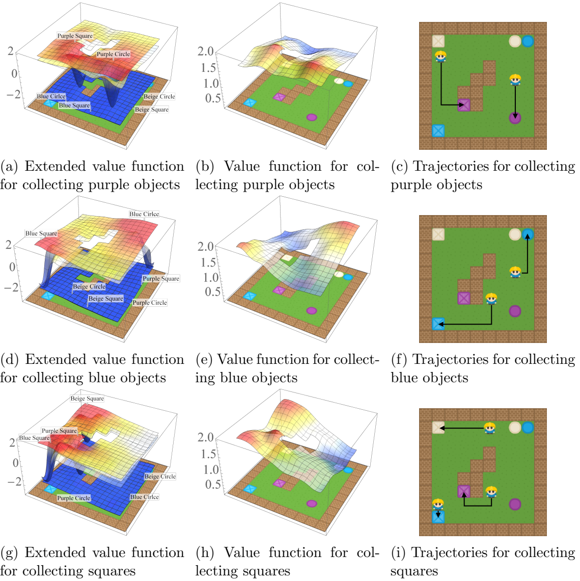
Figure 5.19: Base tasks for the video game environment with relaxed assumptions. We show extended value functions learned for the purple, blue, and square tasks.
