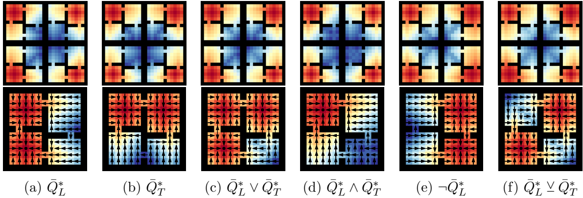
Figure 5.16: An example of Boolean algebraic composition using the learned extended value functions with dense rewards. Top row shows extended value functions while bottom one shows resulting value functions and policies obtained by maximizing over goals. Arrows represent the optimal action in a given state. (a–b) The learned optimal extended value functions and resulting value functions for the base tasks with dense rewards. (c) Disjunctive composition. (d) Conjunctive composition. (e) Negation. (f) Combining operators to model exclusive-or composition. We note that the resulting value functions are very similar to those produced in the sparse reward setting.
