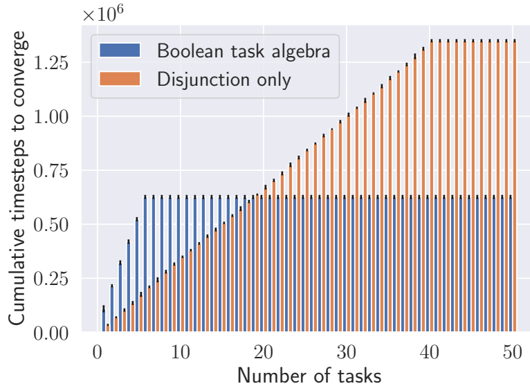
Figure 5.18: Cumulative number of samples required to solve tasks in a 40-goal Four Rooms domain. Error bars represent standard deviations over 100 runs.
