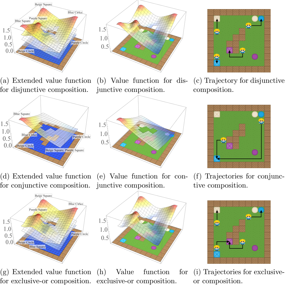
Figure 5.15: By composing extended value functions from the base discounted goal-reaching tasks (collecting blue objects, and collecting squares), we can act optimally in new tasks with no further learning. The extended value functions shows the value function with respect to each goal plotted on the same axis. To generate this, we place the agent at every location and apply the element wise composition operators on the outputs of each network. We then compute the maximum over all actions for each goal. The points are interpolate between each other to smooth the graph. Any error in the visualisation is due to the use of non-linear function approximation.
