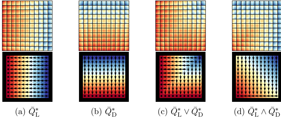
Figure 5.1: Showing the disjunction and conjunction of EVFs learned from deterministic shortest path tasks in gridworld domain. Figures (a)-(b) shows the EVFs for the left and down tasks. (c) shows the EVF of their disjunction. (d) shows the EVF of their conjunction.
