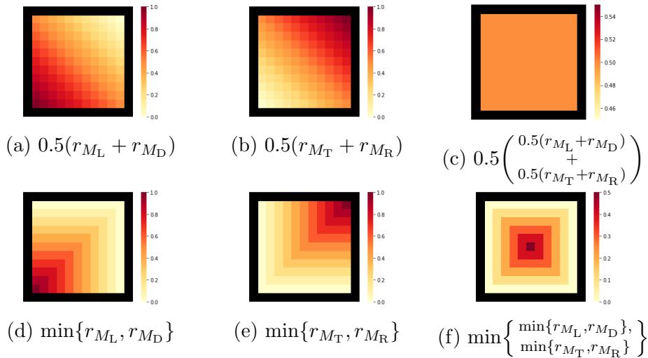
Figure 3.7: Consider 4 tasks, M_L , M_R , M_D , and M_T , in which an agent must navigate to the left, right, down, and top regions of an xy -plane respectively. The top row shows conjunctions approximated using average of rewards while the bottom one shows true conjunctions using the min of rewards. From left to right we plot the reward for entering a region of the goal space for the conjunction of M_L and M_D , conjunction of M_T and M_R , and conjunction of (M_L and M_D) and (M_T and M_R) . Note that by averaging reward, terminal states quickly become equally rewarded, losing the meaning of the true conjunction.
