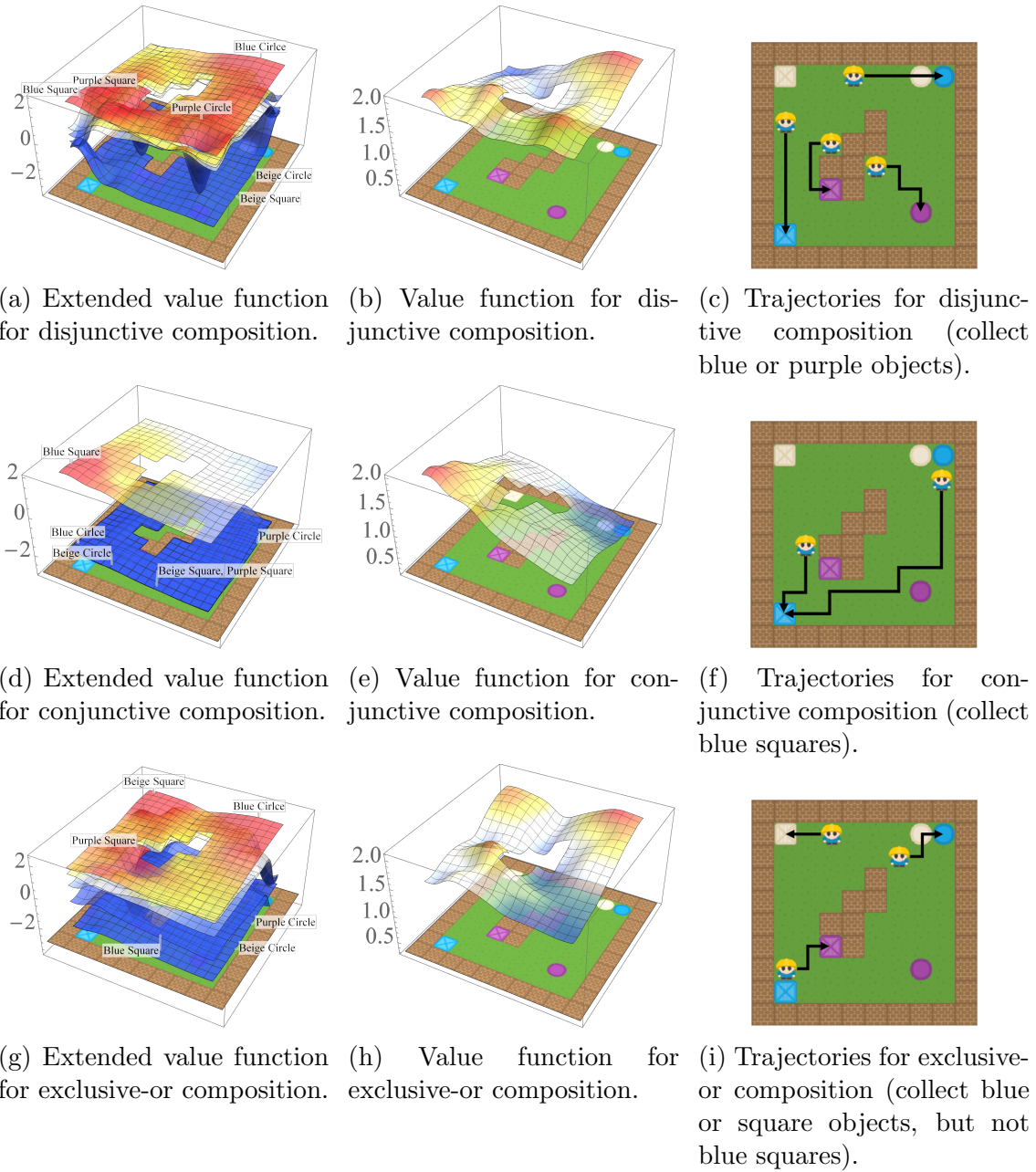
Figure 5.20: Results for the video game environment with relaxed assumptions. We generate extended value functions to solve the disjunction of blue and purple tasks, and the conjunction and exclusive-or of blue and square tasks. The extended value functions shows the value function with respect to each goal plotted on the same axis. To generate this, we place the agent at every location and apply the element wise composition operators on the outputs of each network. We then compute the maximum over all actions for each goal. The points are interpolate between each other to smooth the graph. Any error in the visualisation is due to the use of non-linear function approximation with the relaxed assumptions.
