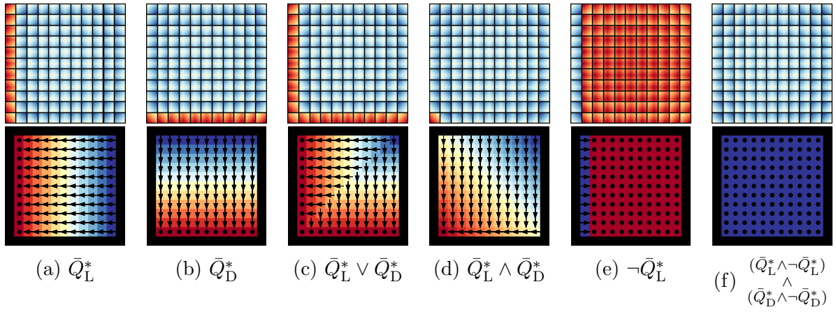
Figure 5.6: Showing composition of Boolean EVFs in gridworld domain. Figures (a)-(b) shows the Boolean goal rewards for the left and down tasks, (c)-(f) shows the rewards of the composed tasks.
