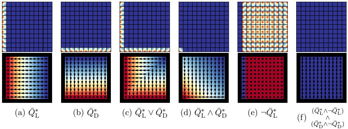
Figure 5.7: Showing composition of Boolean tasks in gridworld domain. Figures (a)-(b) shows the Boolean goal rewards for the left and down tasks, (c)-(f) shows the rewards of the composed tasks.
