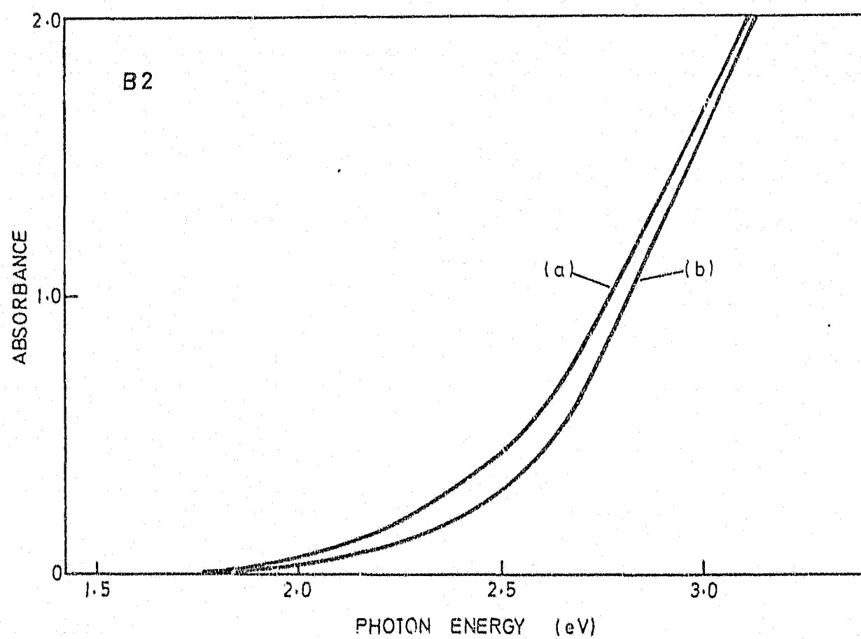
FIG. 4.11 The room temperature optical absorption spectrum of a natural type Ib diamond (B2) (a) after cooling from 400°C and (b) after bleaching with 2.5 eV light.
