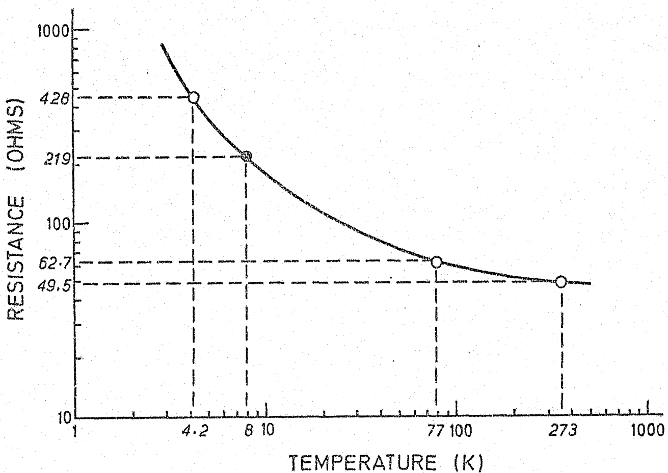
FIG. 3.8 The variation of resistance with temperature of the Allen-Bradley resistor used for temperature measurement in the helium cryostat. The open circles indicate calibration points and the solid line is the universal curve of Clement et al (1956) fitted to these points. Resistance and temperature in the sample position is indicated by the closed circle.
