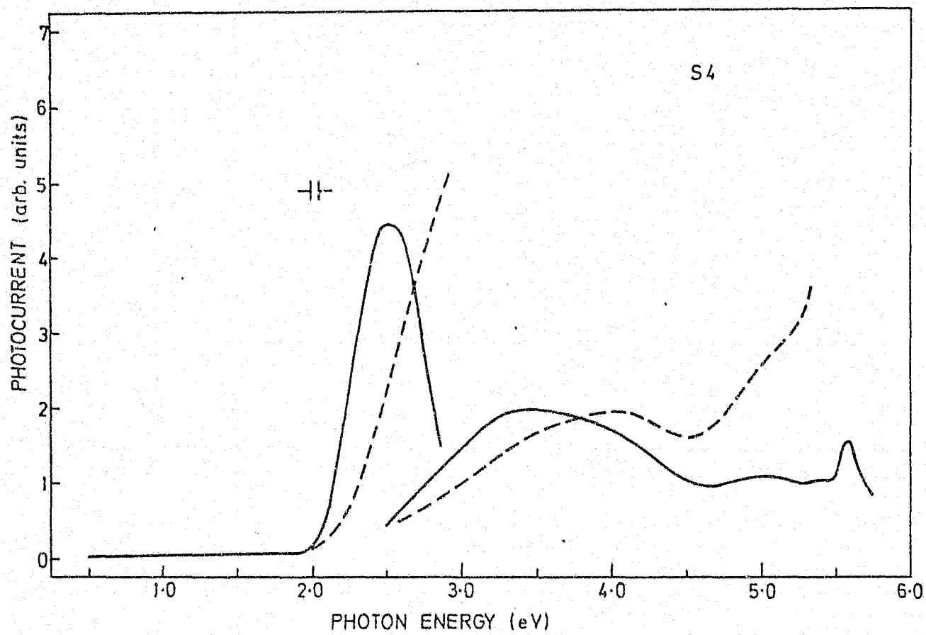
FIG. 4.15 The room temperature photoconduction spectrum of synthetic sample S4. The solid line is the unnormalized spectrum; the broken line is the normalized spectrum.
