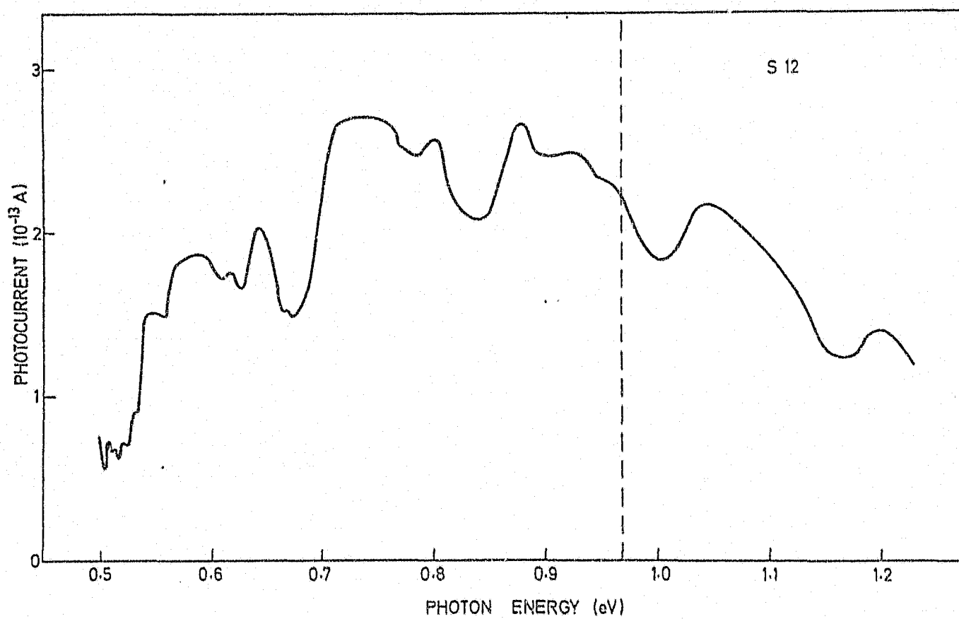
FIG. 4.20 The infrared photoconductivity spectrum of sample S12 at 80K. See Fig. 4.21 for the spectrum to the right of the broken line.
