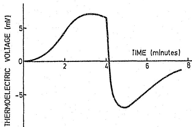
FIG. 4.10 The thermoelectric effect observed under identical experimental conditions in (a) a p-type semiconducting diamond (see Fig. 3.12) and (b) in diamond B3, which is clearly n-type.
