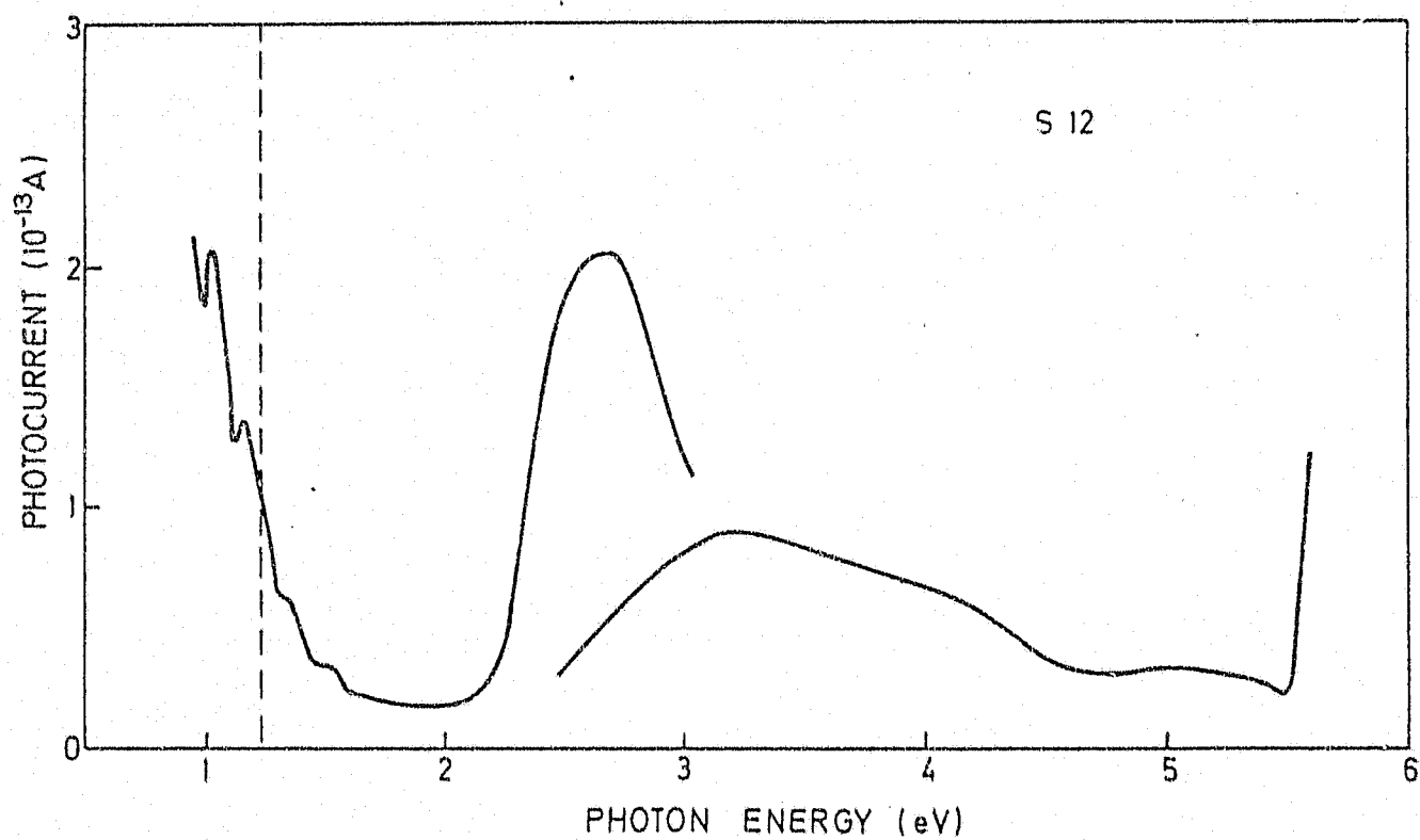
FIG. 4.21 The photoconduction spectrum of sample S12 at 80K. See Fig. 4.20 for the spectrum to the left of the broken line.
