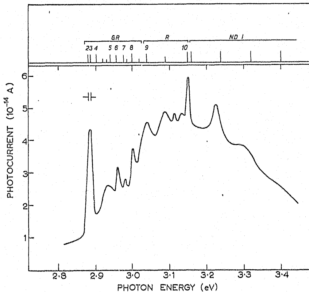
FIG. 4.3 The photoconduction spectrum at 80K of an electron-irradiated type Ia diamond in the neighbourhood of the GR2 to GR8, R9 and R10 lines, and the ND1 absorption system. At the top of the figure are shown the positions of the GR2 to GR8, R9 and R10 lines, as given by Clark, Ditchburn and Dyer (1956), and the absorption lines of the ND1 system (Dyer and du Preez, 1965). The tungsten lamp of the monochromator was used.
