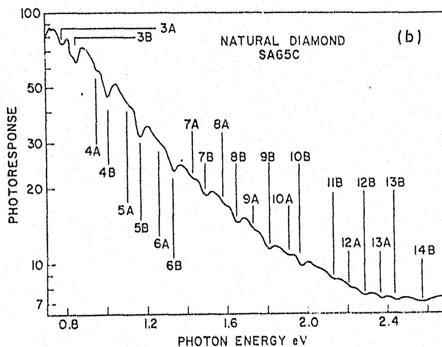
FIG. 2.4 The photoconductivity spectrum of a type IIb diamond (a) in the one-, two-, and three-phonon region above the acceptor ionization threshold, and (b) at higher energies, showing the minima associated with the multiphonon cascade process. Both spectra are from Collins, Lightowers and Dean (1969).
