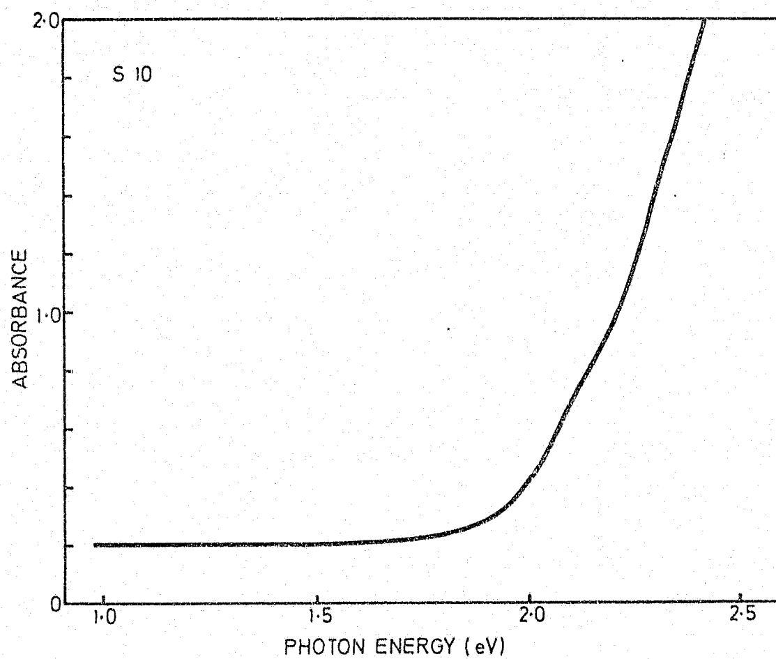
FIG. 4.14 The visible-ultraviolet spectrum of synthetic diamond S10.
