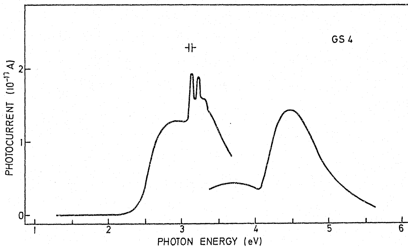
FIG. 5.1 The photoconduction spectrum at 80K of a type Ia gem sand diamond. The ND1 system, centred at 3.3 eV, is extremely prominent
