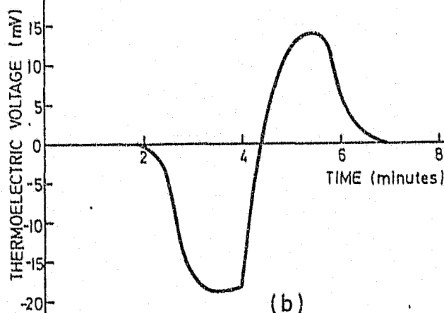
FIG. 4.10 The thermoelectric effect observed under identical experimental conditions in (a) a p-type semiconducting diamond (see Fig. 3.12) and (b) in diamond B3, which is clearly n-type.
