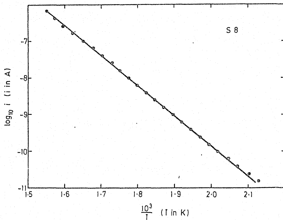
FIG. 4.18 The current i through synthetic diamond S8 as a function of temperature T , with a fixed applied voltage of 90V.
