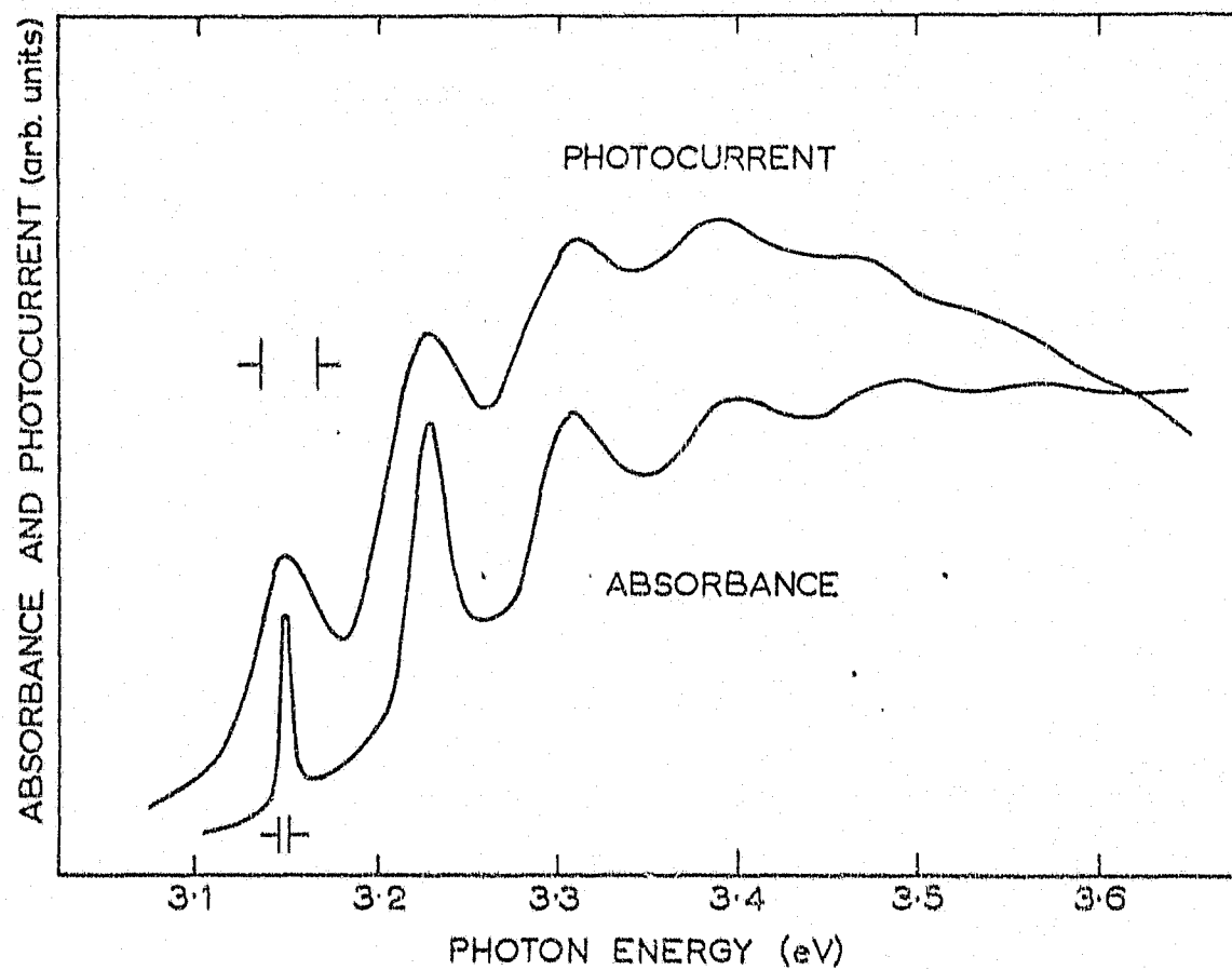
FIG. 4.4 Photoconduction and optical absorption spectra at 8K in the neighbourhood of the ND1 system in an electron-irradiated type Ia diamond. The deuterium lamp was used with the monochromator.
