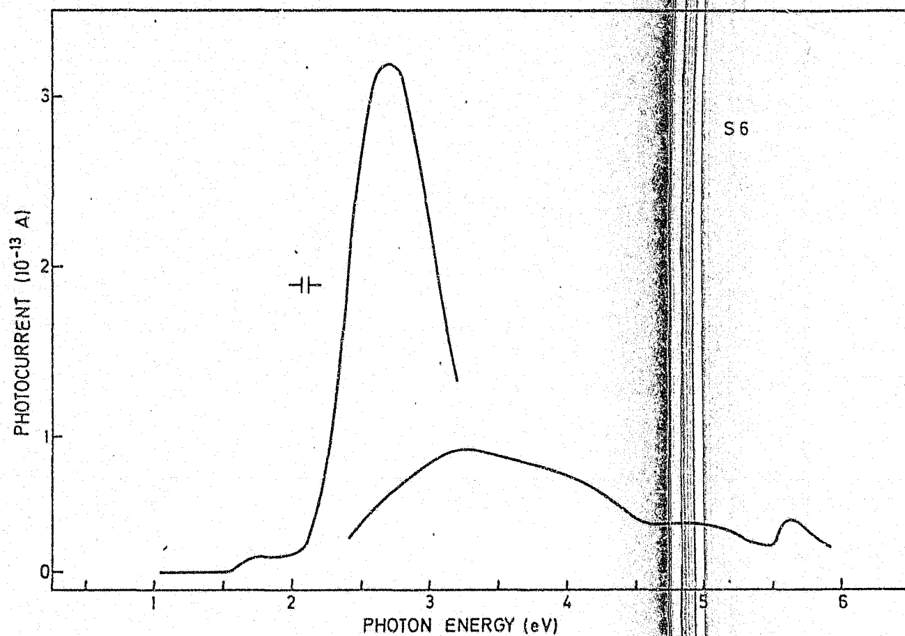
FIG. 4.16 The room temperature (unnormalized) photoconduction spectrum of synthetic diamond S6.
