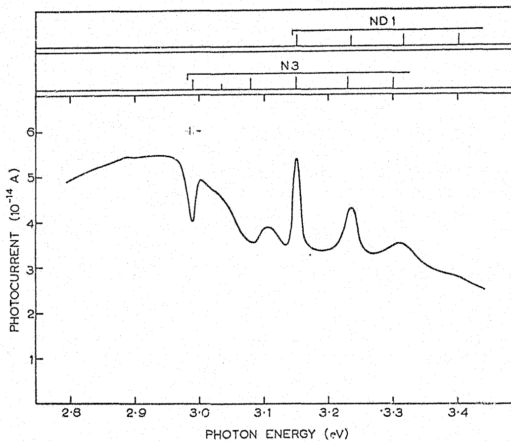
FIG. 4.6 The photoconductivity spectrum at 80K in an irradiated type Ia diamond which contains both the N3 and ND1 systems. The first two lines of the N3 system appear as minima followed by maxima at the positions of the ND1 maxima. The tungsten lamp was used with the monochromator.
