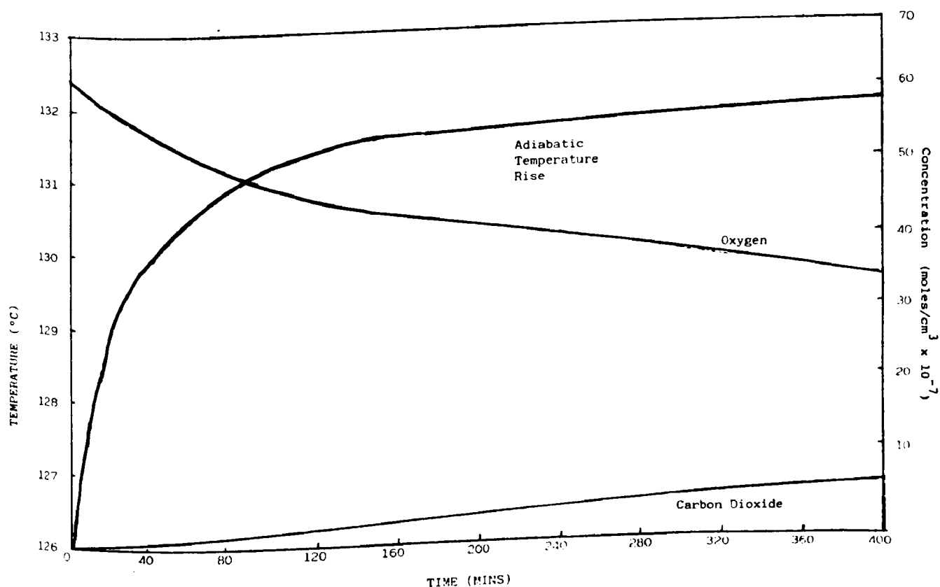
Figure 1.1 Temperature, Oxygen and Carbon Dioxide Versus Time
