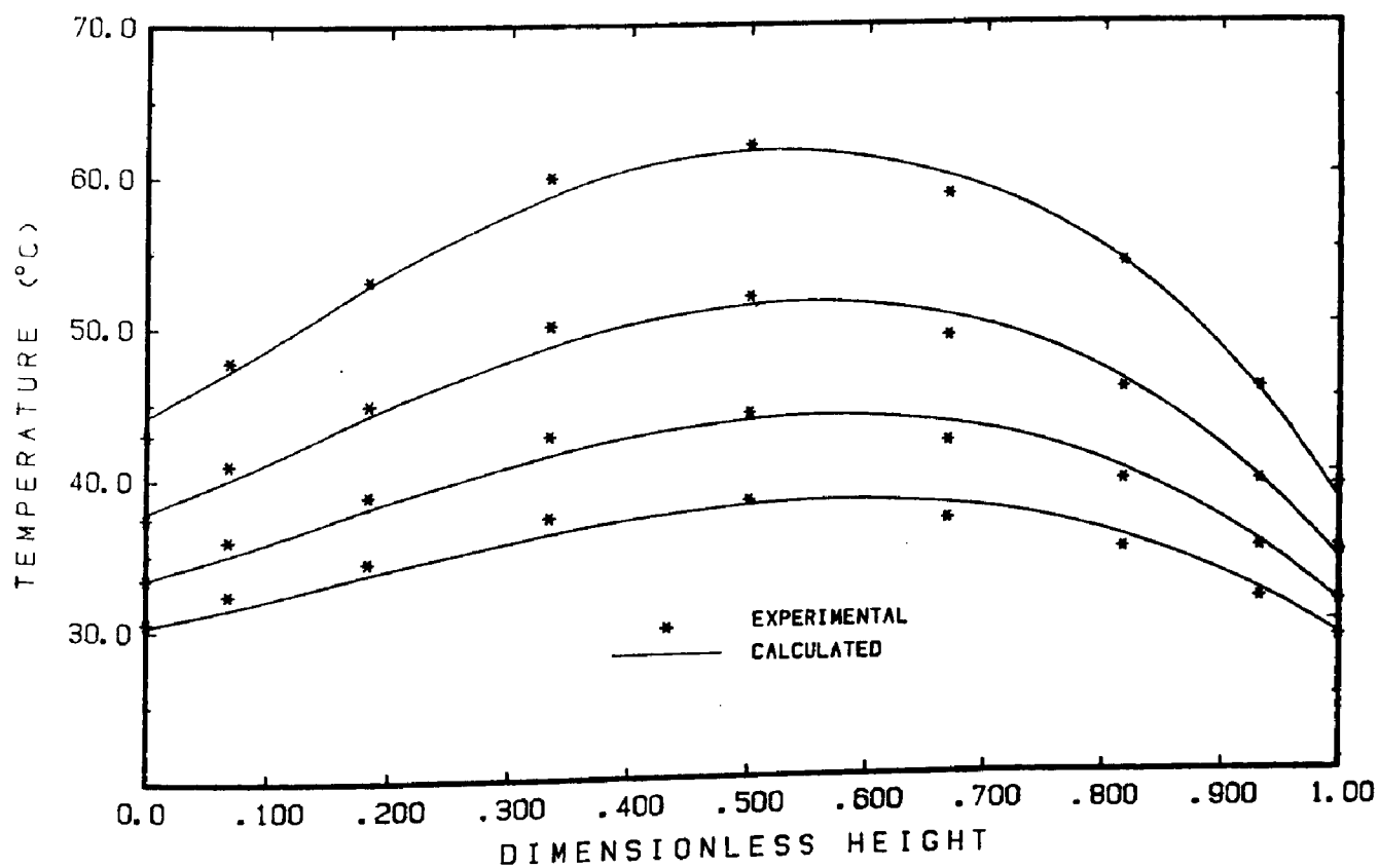
Figure 7.2 Chimney experiment - Fitting heat transfer coefficients Profiles plotted every 30 minutes
