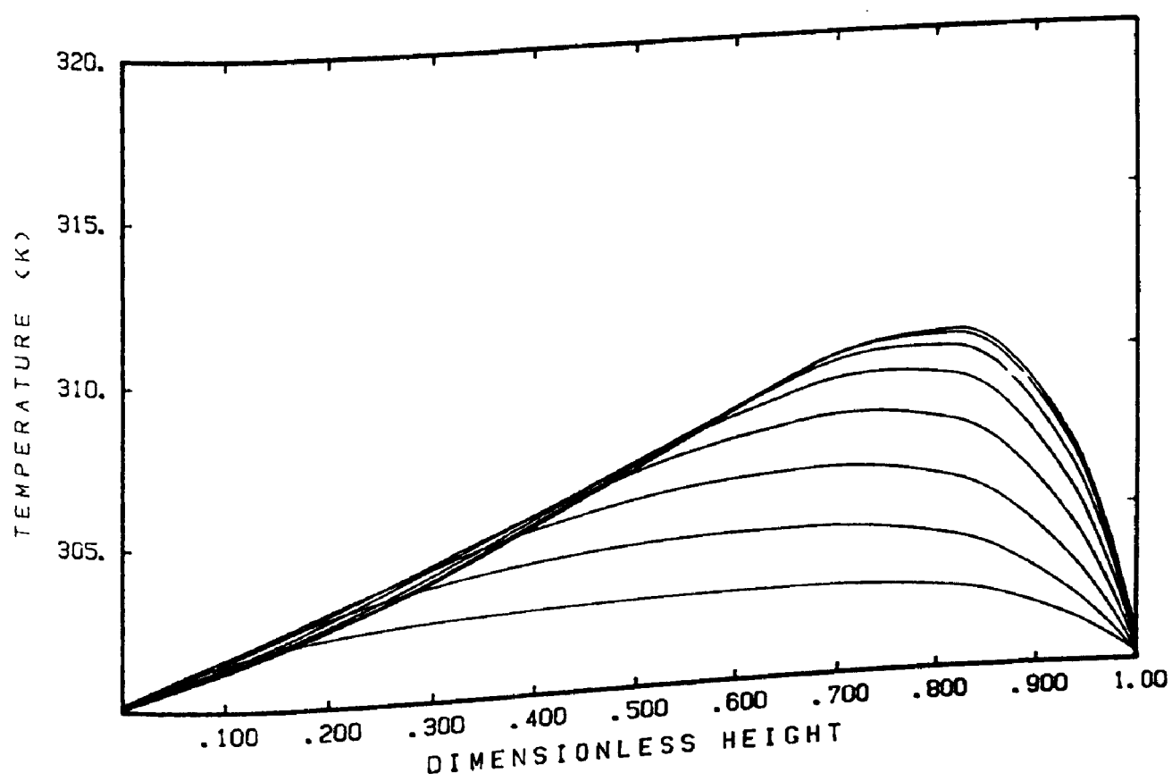
Figure 8.15 Temperature profiles in a coal bed Particle size 10 mm - Numerical Method
