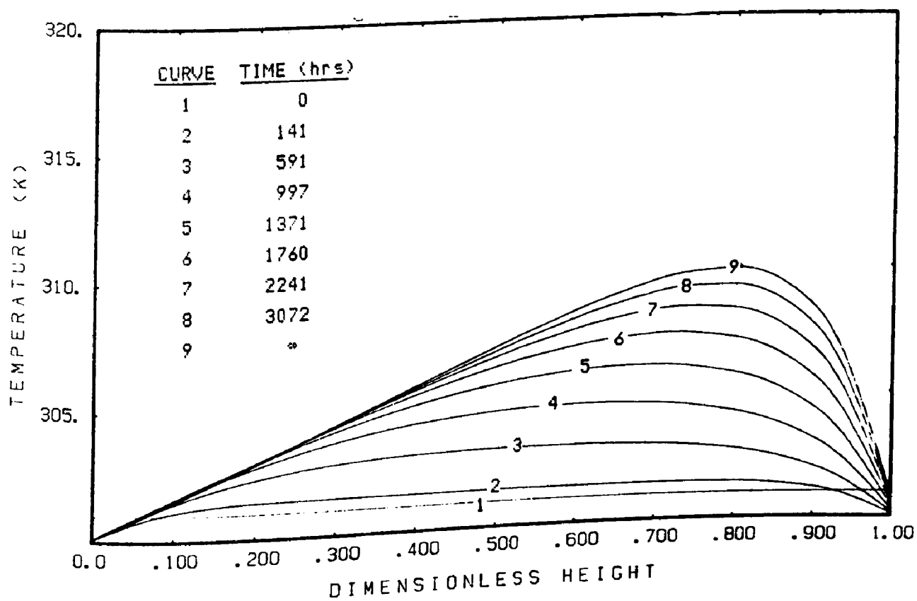
Figure 8.13 Temperature profiles in a coal bed
