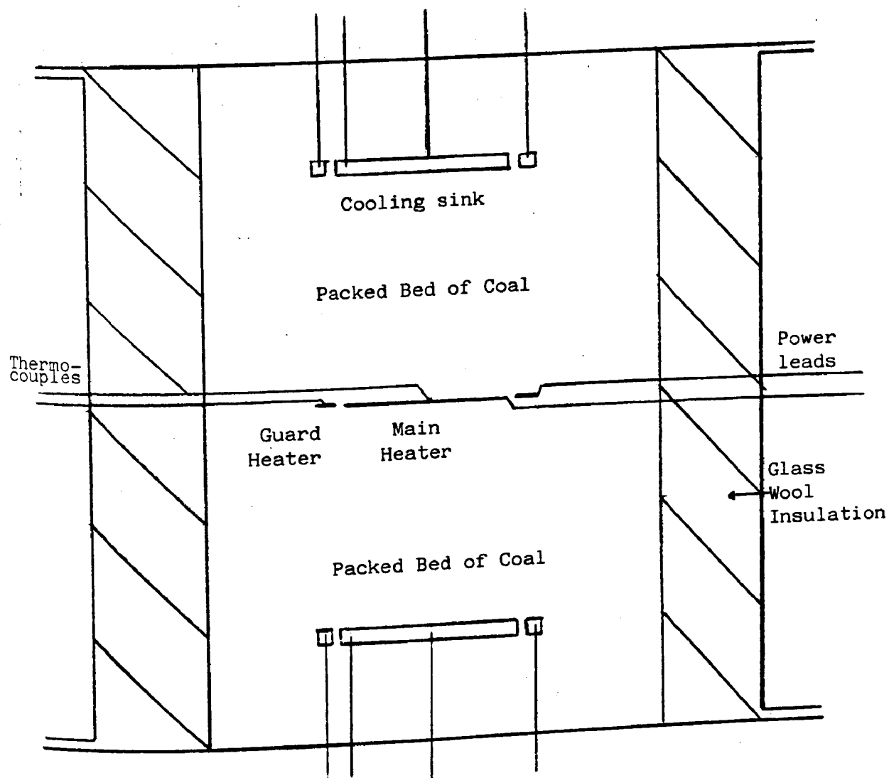
Figure 4.2 Guarded hot ring apparatus - Assembled apparatus
