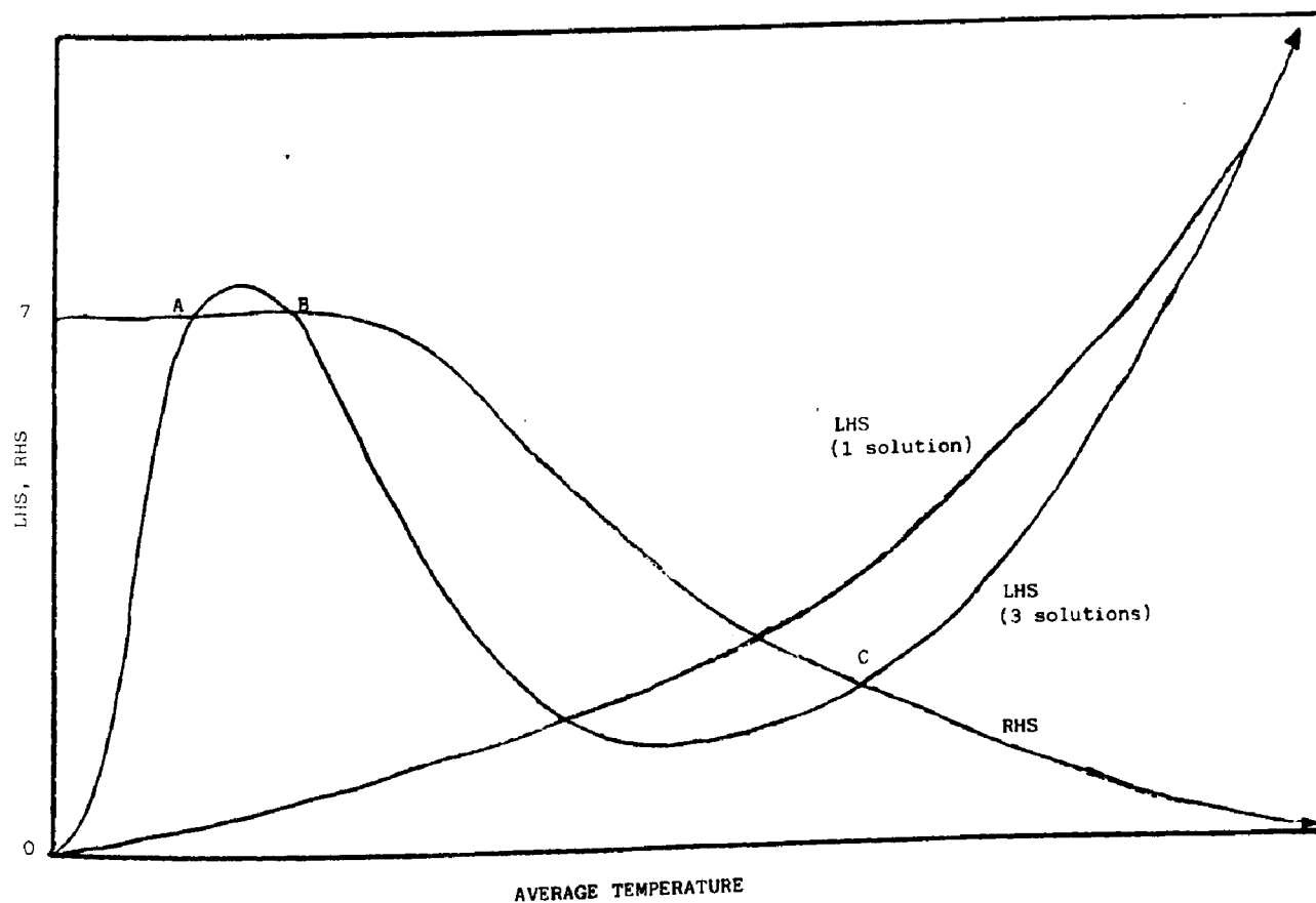
Figure 8.1 LHS and RHS of equation 8.2 as a function of \theta
