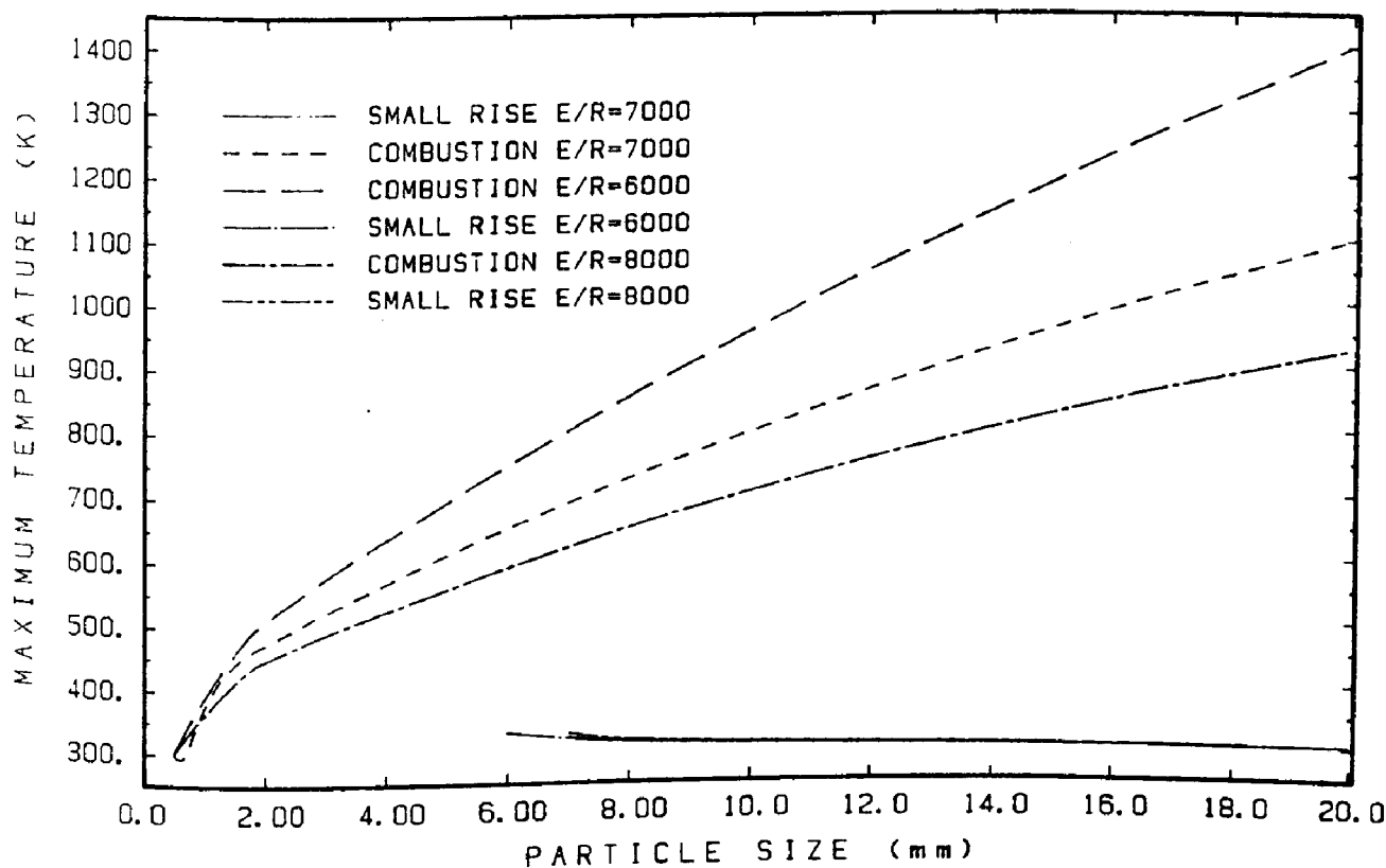
Figure 8.6 Effect of varying the activation energy on the maximum temperature
