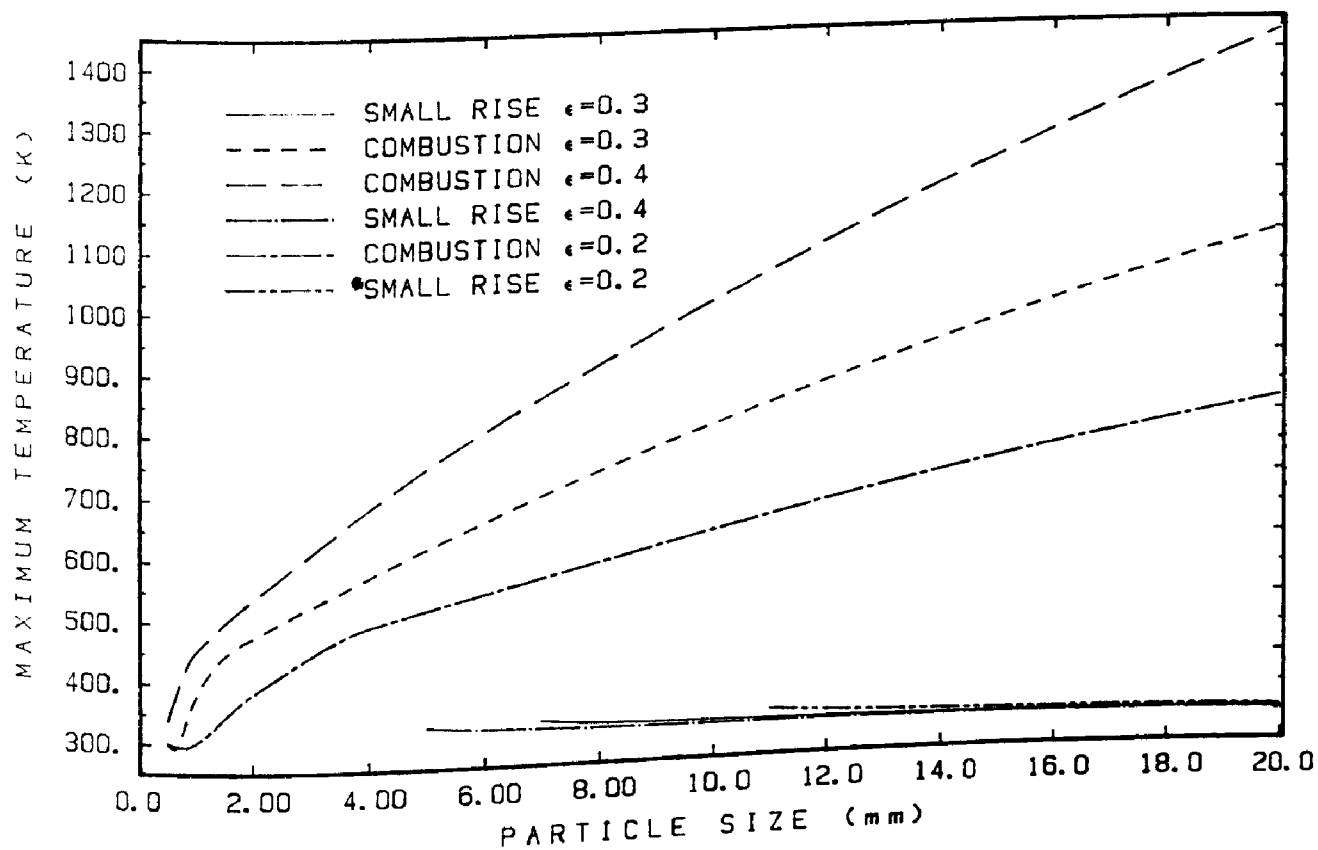
Figure 8.4 Effect of varying voidage on the maximum temperature
