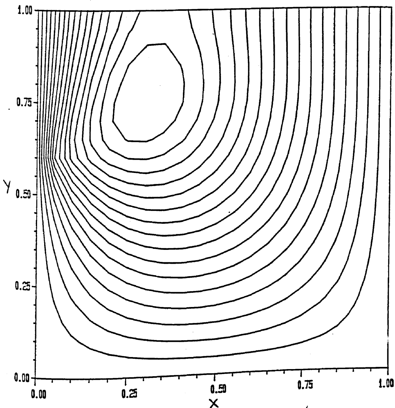
Figure 5.1 Streamlines in a Packed Bed Containing a Line Source (From Young, 1985)
