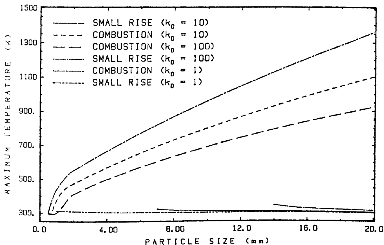
Figure 8.5 Effect of varying the pre-exponential factor on the maximum temperature
