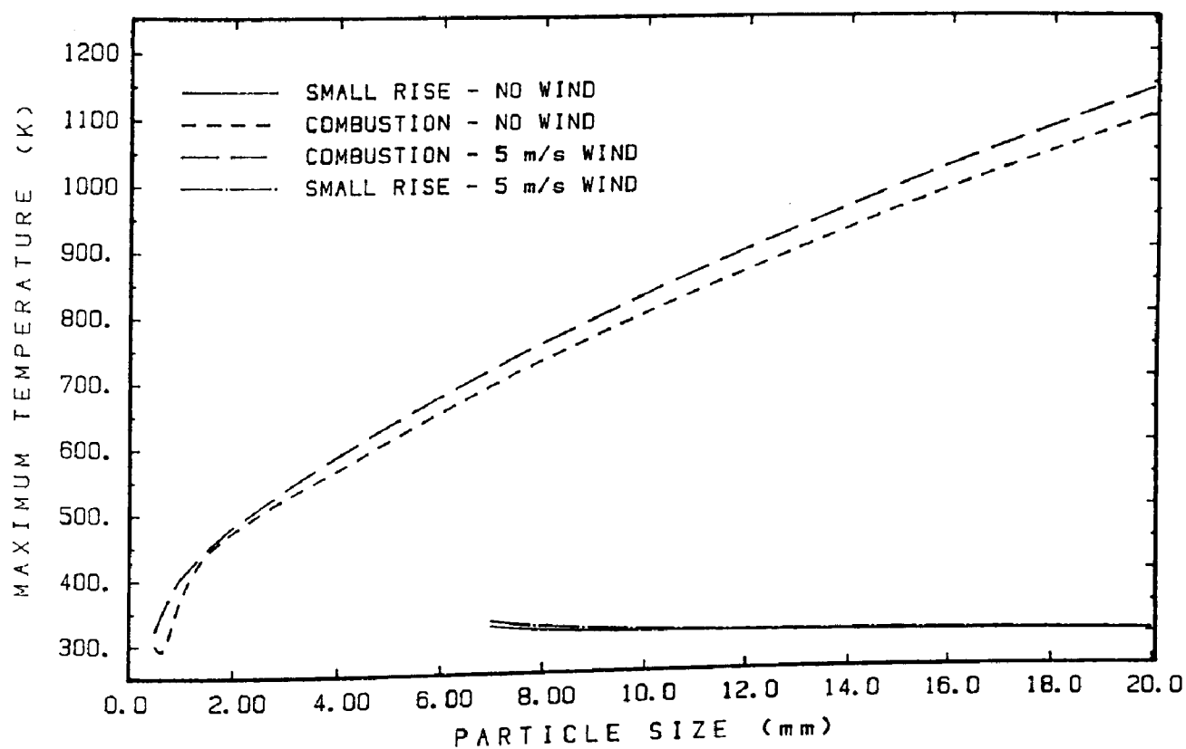
Figure 8.9 Effect of wind on the maximum temperature
