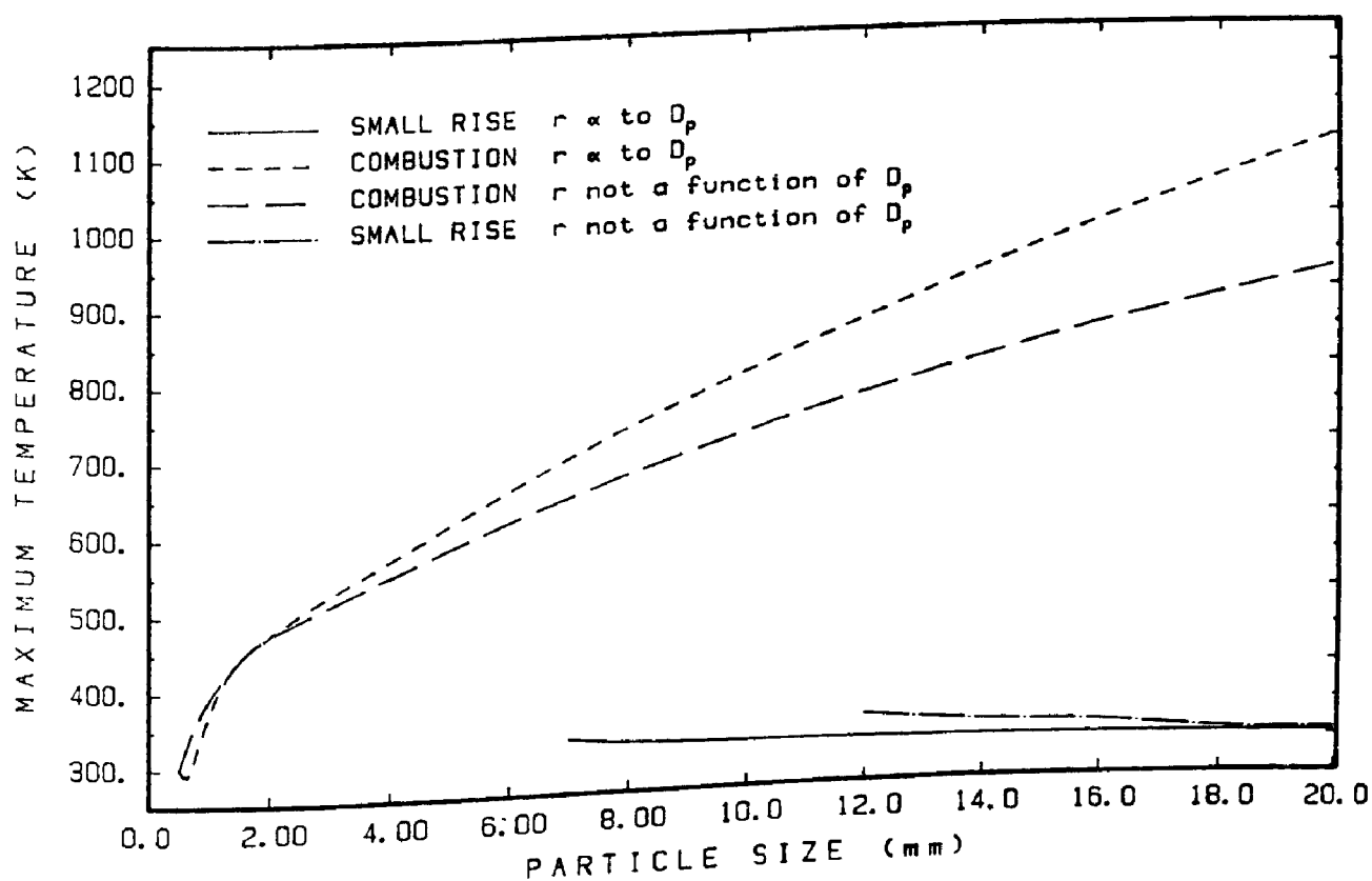
Figure 8.8 Effect of different assumptions about surface area on the maximum temperature
