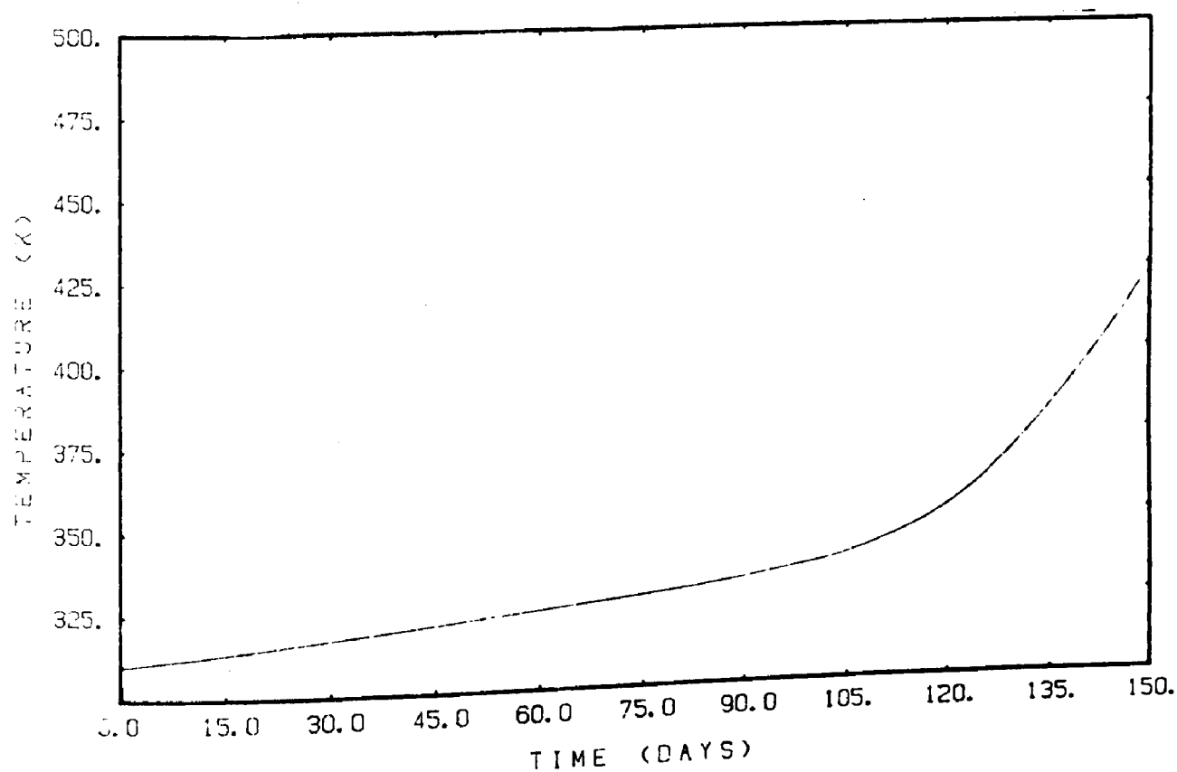
Figure 8.14 Temperature-time behaviour at bed centre Particle size 6 mm - Analytical solution
