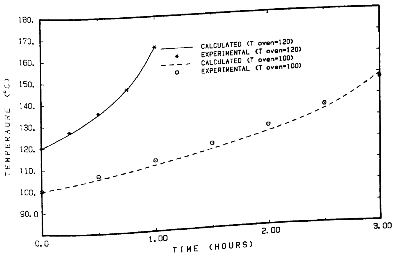
Figure 7.5 Chimney experiment - Fitting ignition runs
