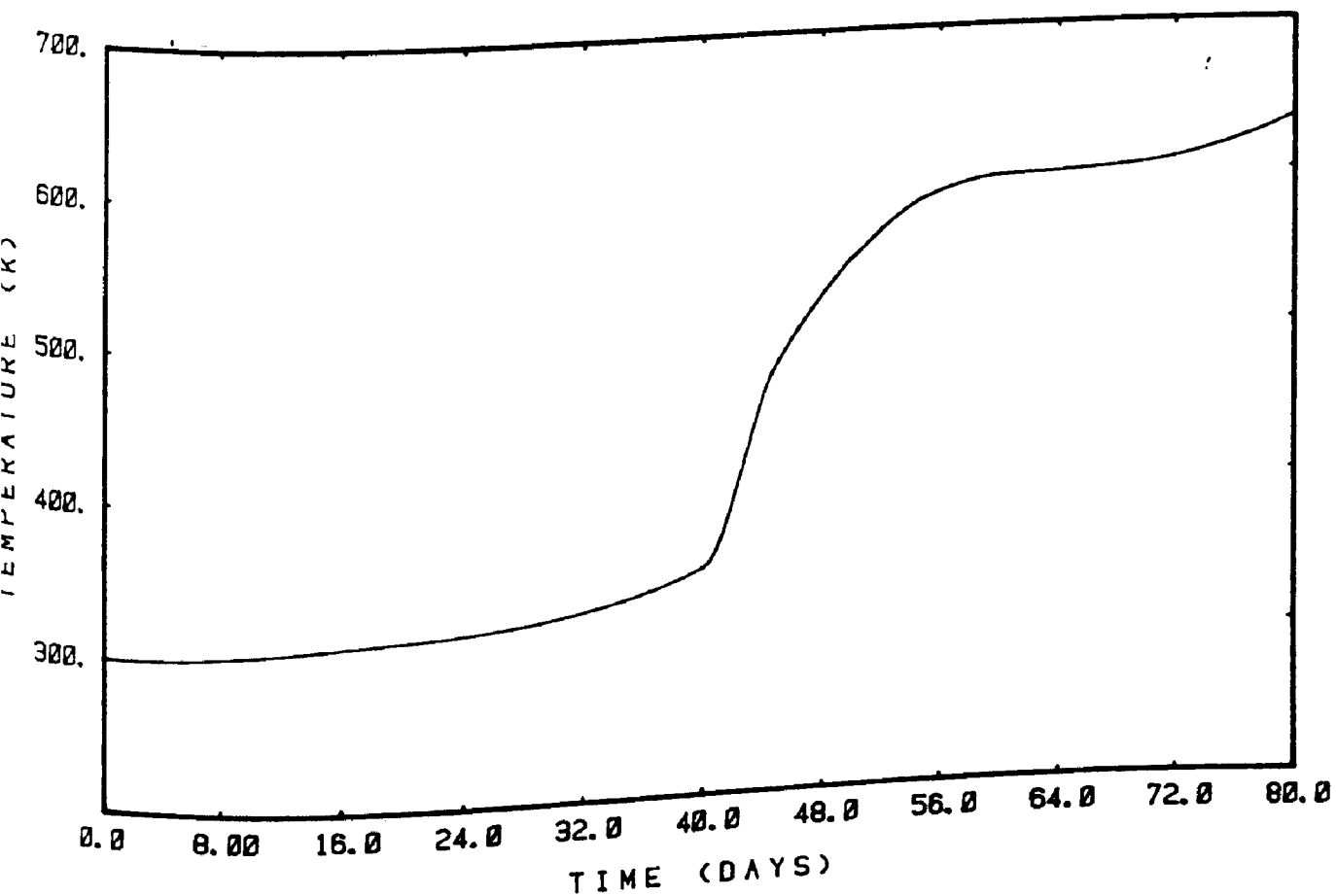
Figure 8.16 Temperature profiles with ignition Particle size 2 mm - 5 m/s wind - Numerical method First three curves 20 days apart Subsequent curves 5 days apart
