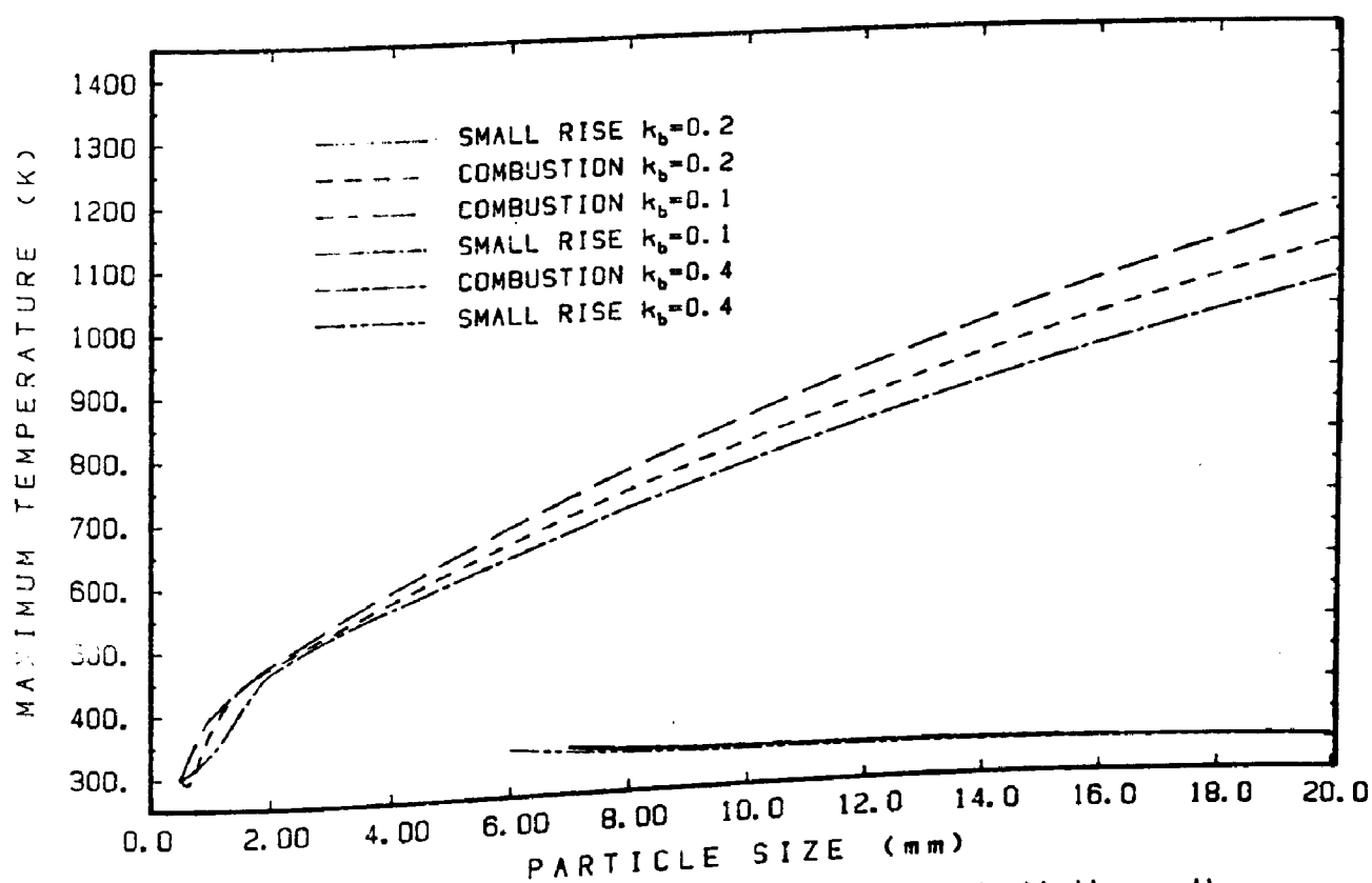
Figure 8.10 Effect of varying bed thermal conductivity on the maximum temperature
