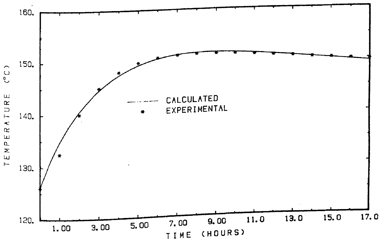
Figure 7.3 Chimney experiment - Fitting ageing run 1
