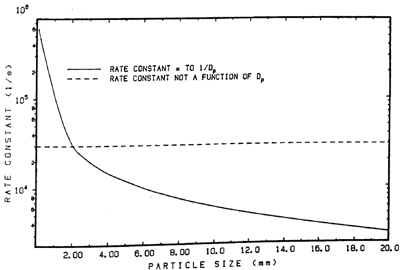
Figure 8.7 Pre-exponential factor versus particle size for the two cases considered
