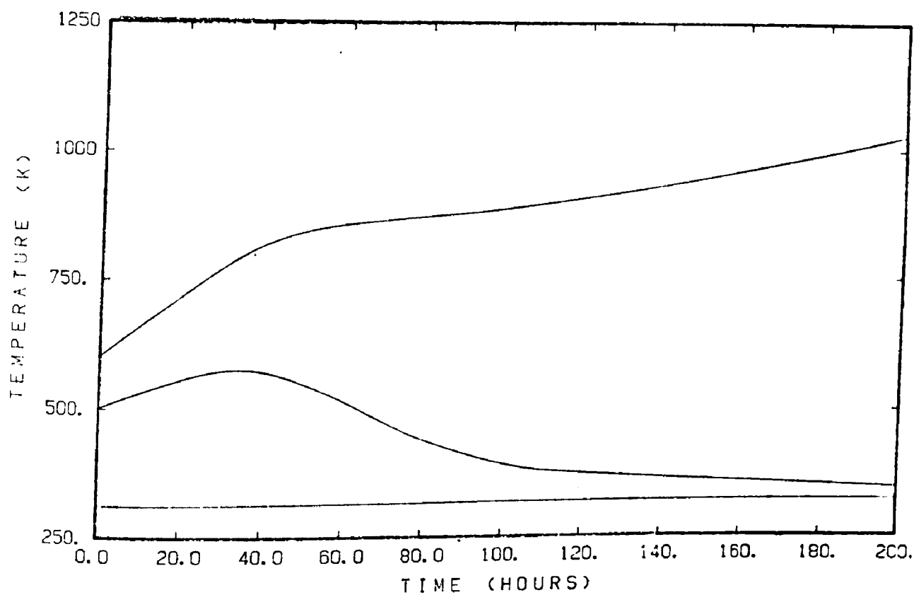
Figure 8.12 Temperature-time curves in the centre of a coal bed for different initial temperatures
