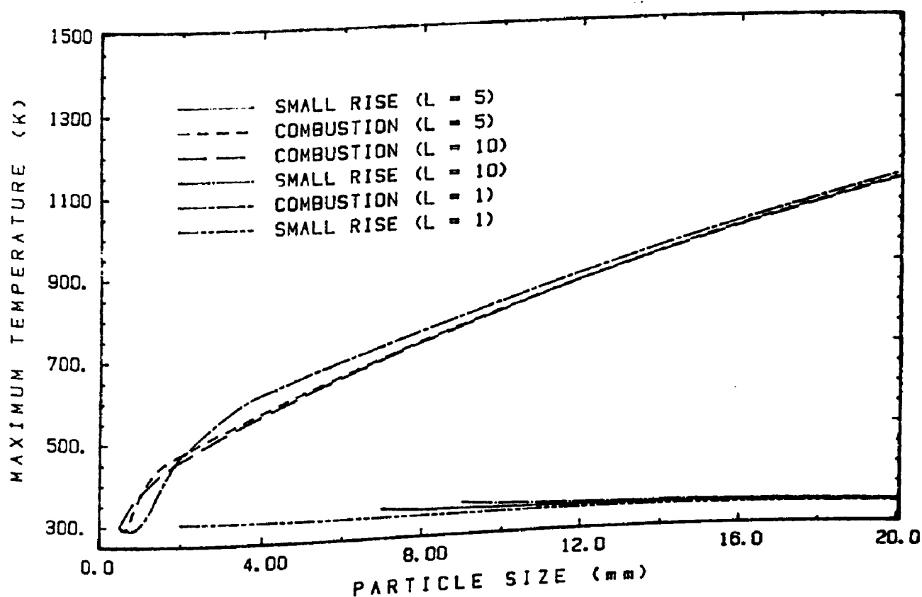
Figure 8.11 Effect of varying bed length on the maximum temperature
