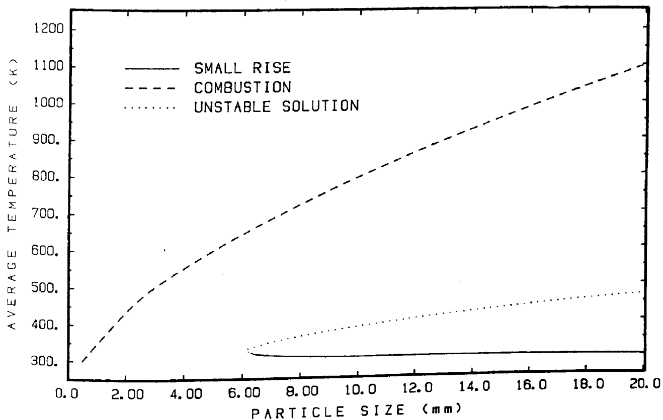
Figure 8.3 Stable and unstable solutions for the base-case
