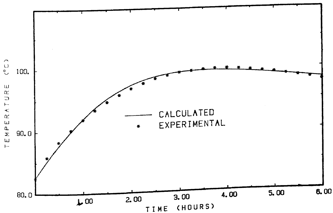
Figure 7.4 Chimney experiment - Fitting ageing run 2
