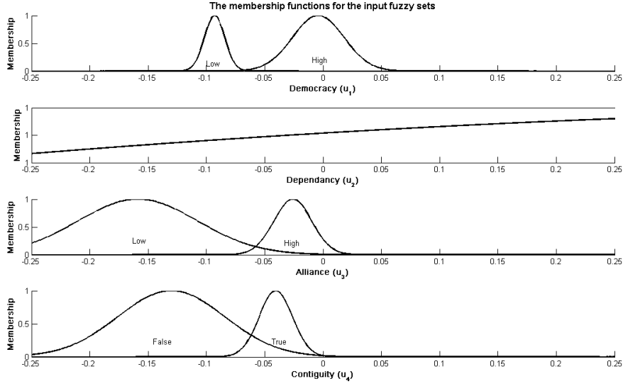
Figure 5.3: The graphs illustrate how the input variables have been partitioned. The membership functions for dependancy have not been partitioned effectively since the one set is seen to be a subset of the other. This allows us to remove this variable and therefore reduce the complexity of the resulting fuzzy statements.
