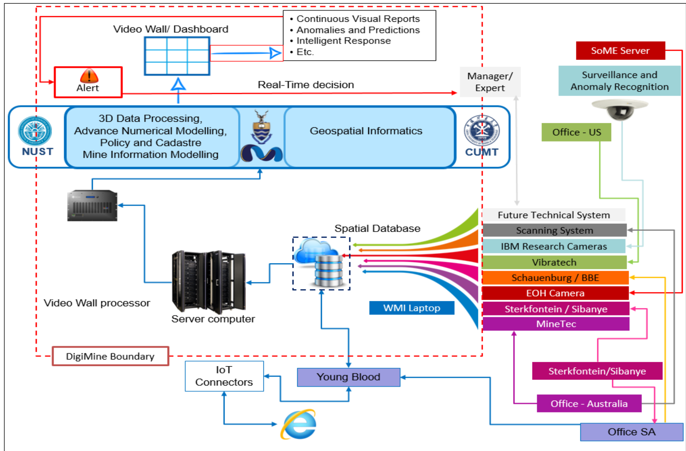
Figure 4.20 Architecture of systems installed in the Mockup-mine (Source: WMI)
