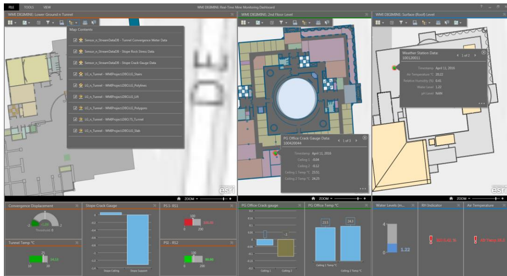
Figure 4.21 Dashboard-display of data sent from sensors housed in displayed sections of WMI's building which were converted to simulate different levels of a mine (Opiti, 2017)
