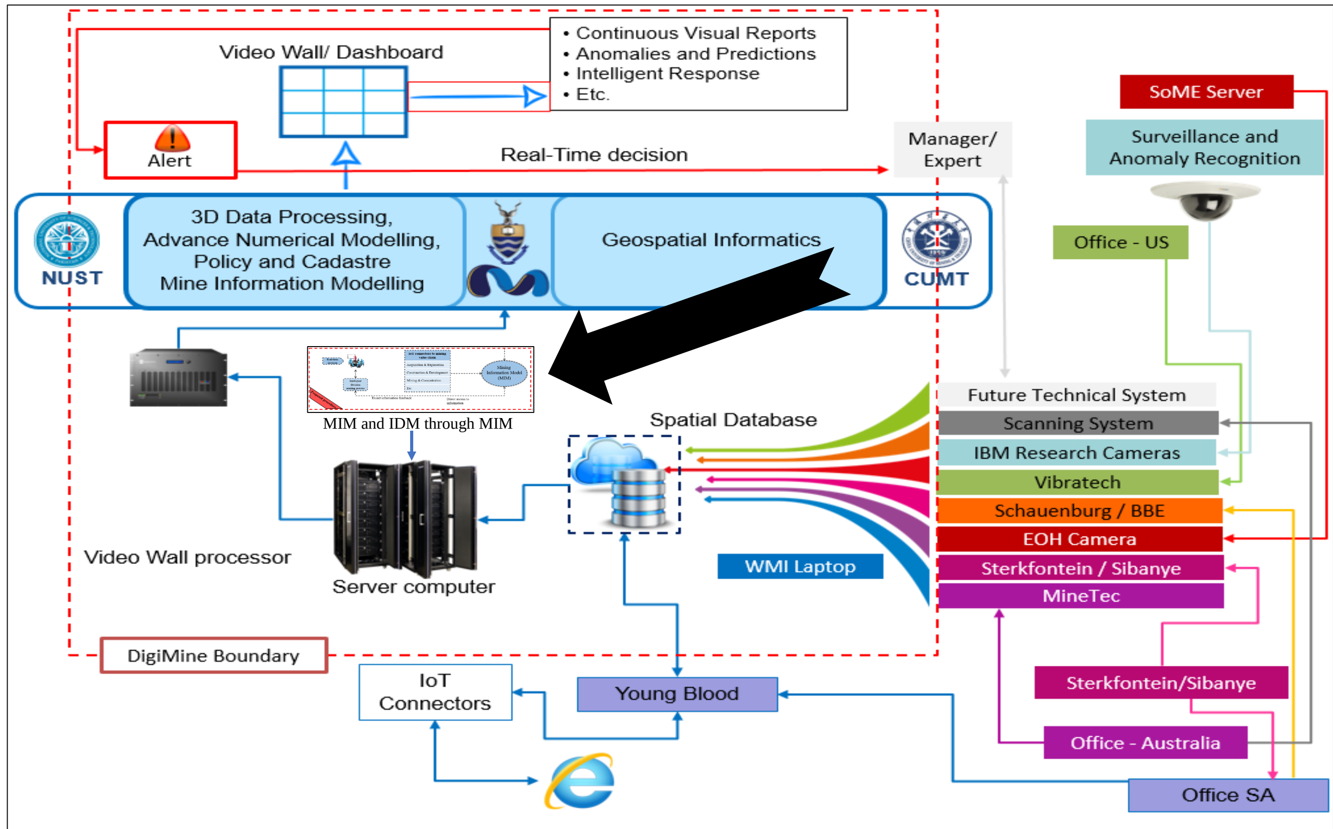
Figure 5.1 Architecture of Wits Mockup-mine with the addition of MIM and IDM through MIM (Source: WMI)
