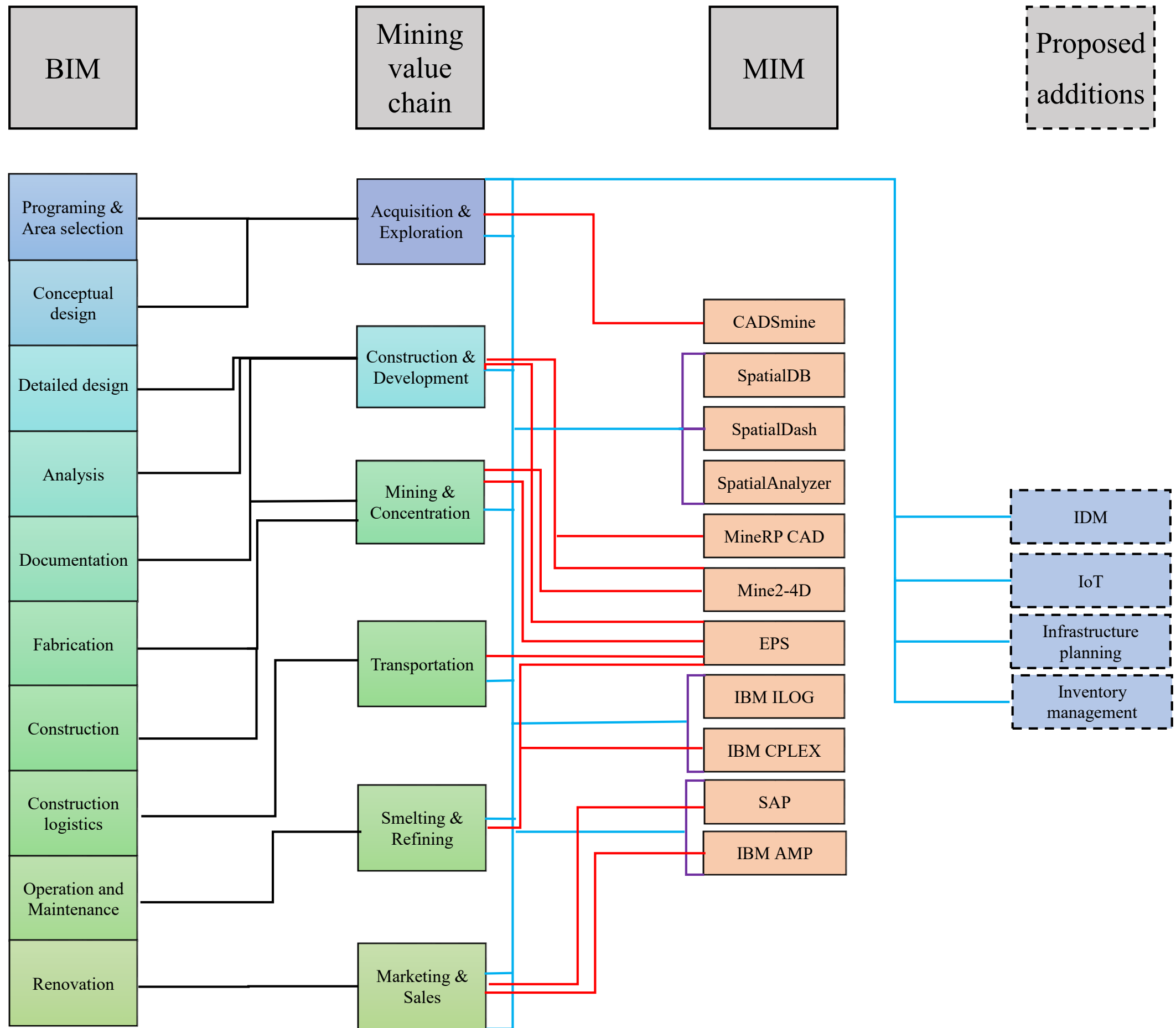
Figure 4.9 MIM architecture across the mining value chain (Source: Author)
