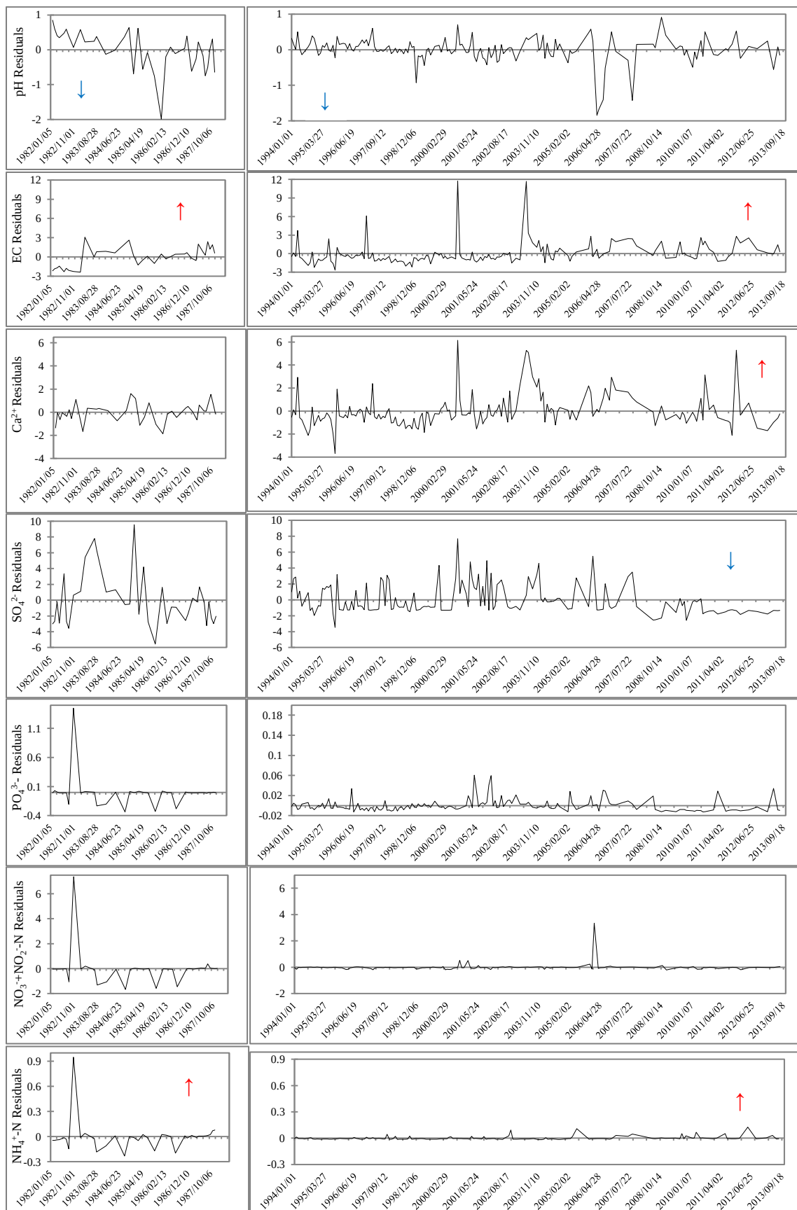
Figure 2.13: Post-LOWESS WQ residuals versus time for the Sterkstroom river (A4H008).
