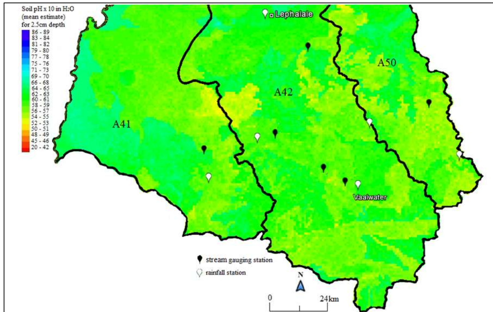
Figure 1.14: Soil pH map for tertiary catchments A41, A42 and A50 (ISRIC 2013).
