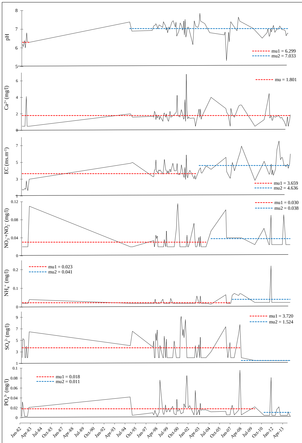
Figure 2.9: Water quality trends in the Palala (A5H004), based on Pettitt's homogeneity tests on monthly medians.
