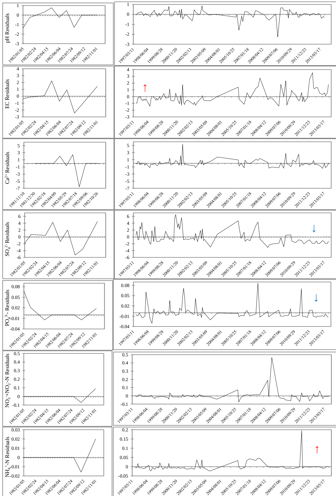
Before ( T_1 ) After ( T_2 ) Figure 2.12: Post-LOWESS WQ residuals versus time for the Palala river (A5H004).* Due to missing WQ data from 1983 to mid-1997, T_1 represents the year 1982 only whilst T_2 included data from between June 1997 and June 2013.
