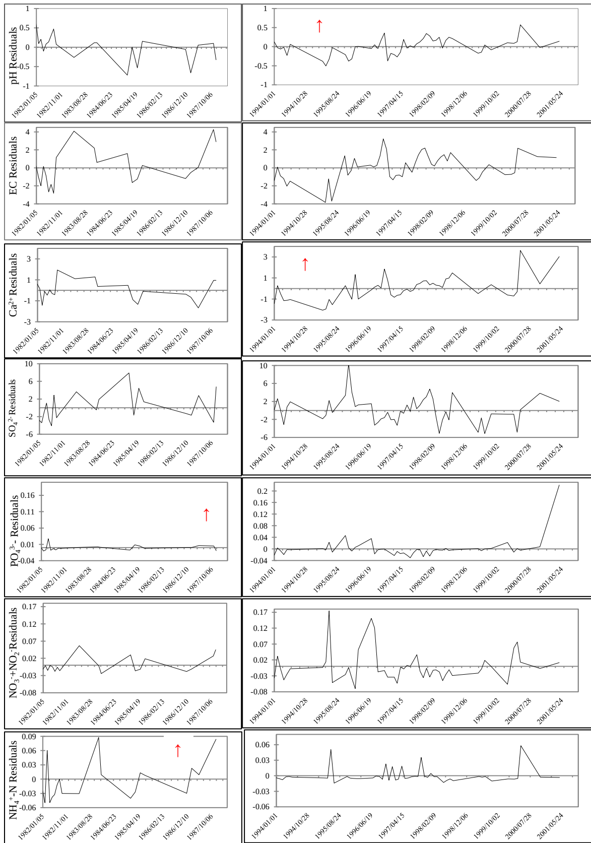
Figure 2.10: Post-LOWESS WQ residuals versus time for the Middle Mokolo river (A4H005). *Due to missing data for more than a decade after 2001, T_2 in this case was between January 1994 and May 2001.
