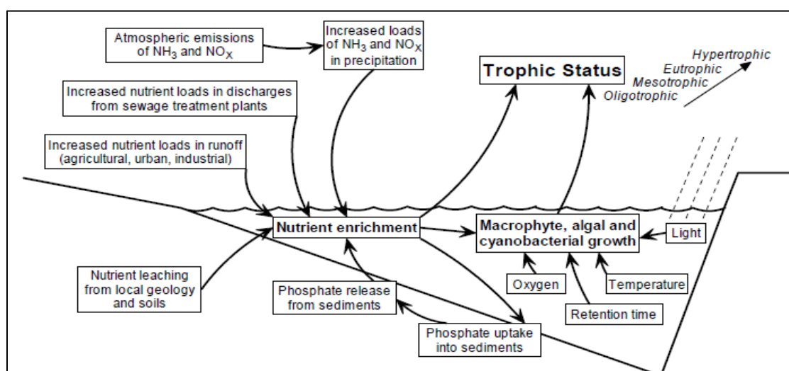
Figure 1.2: Natural and anthropogenic factors and processes which collectively determine the trophic status of waterbodies (Source: DWAF 2002).
