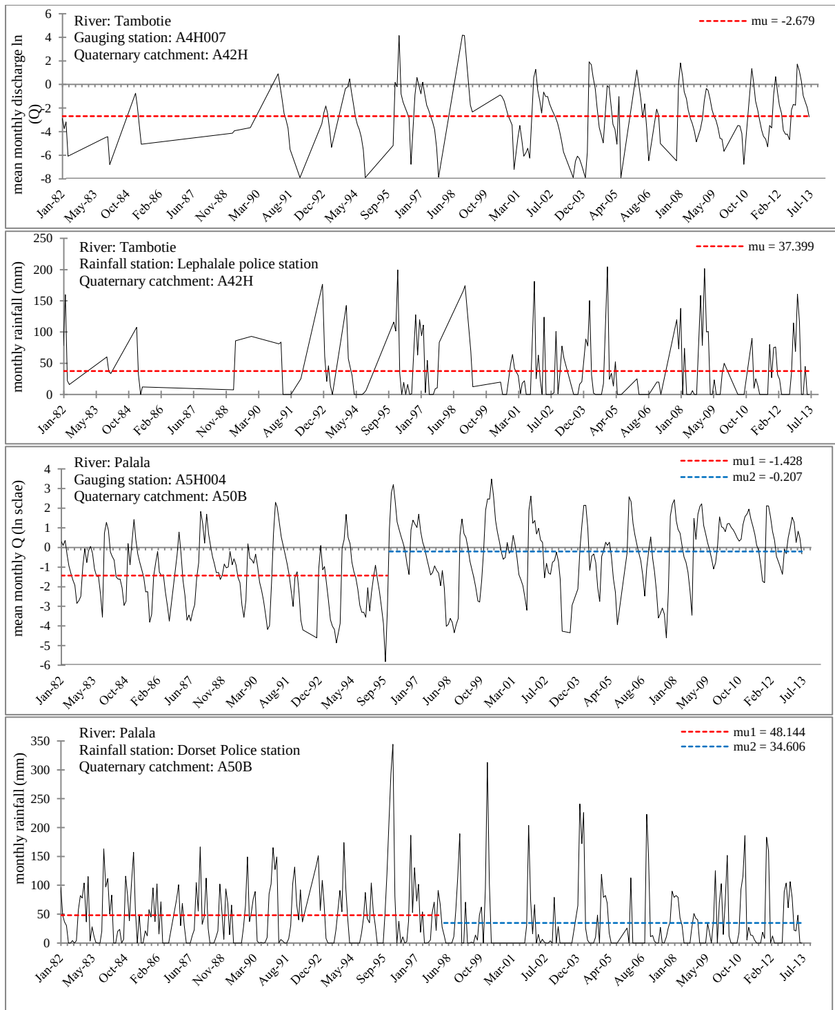
Figure 2.3: Monthly discharge and rainfall trends in the Tambotie and Palala, based on Pettitt's homogeneity tests.
