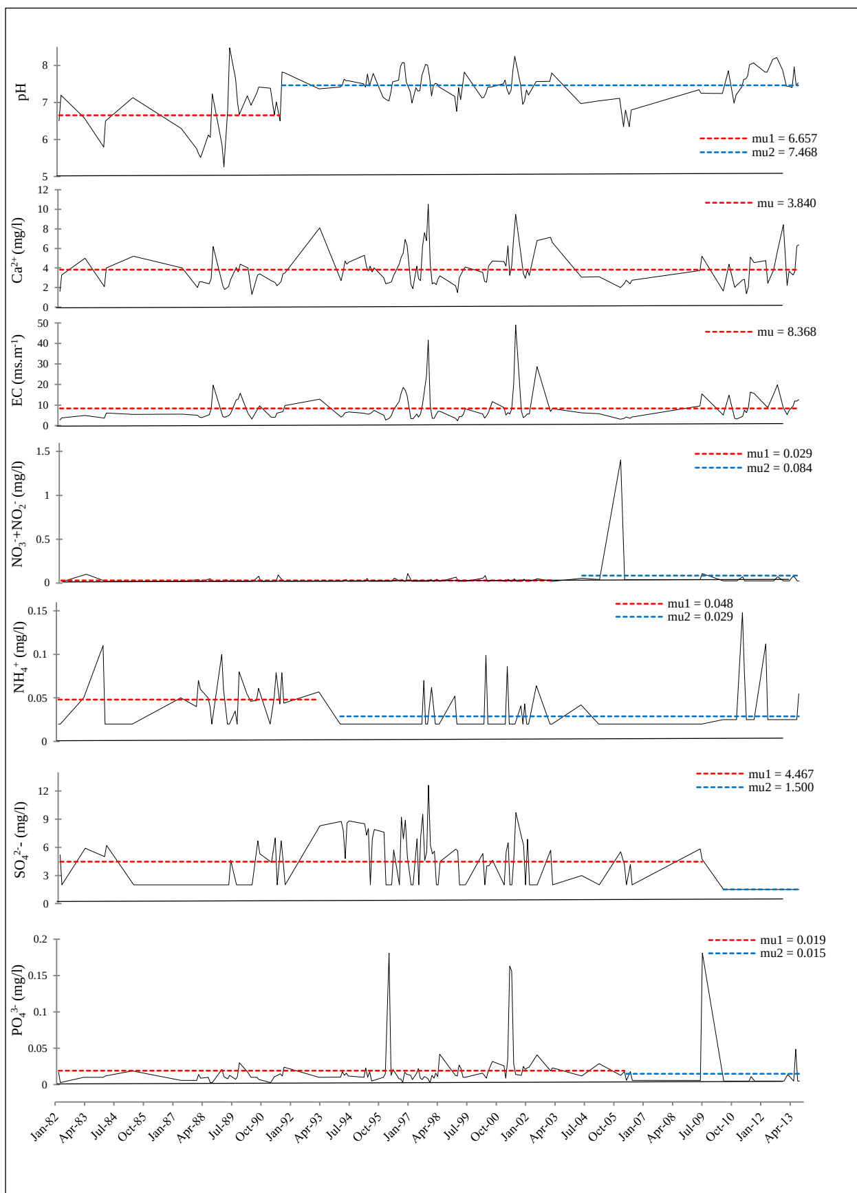
Figure 2.4: Water quality trends in the Matlabas (A4H004), based on Pettitt's homogeneity tests on monthly medians.
