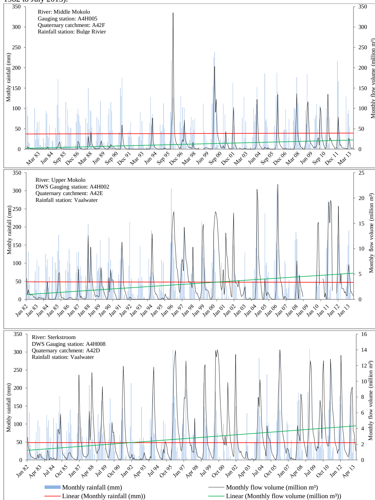
A1: Long-term monthly flow volume and rainfall trends in 4 ry catchments A42F, A42D and A42E (January 1982 to July 2013).
