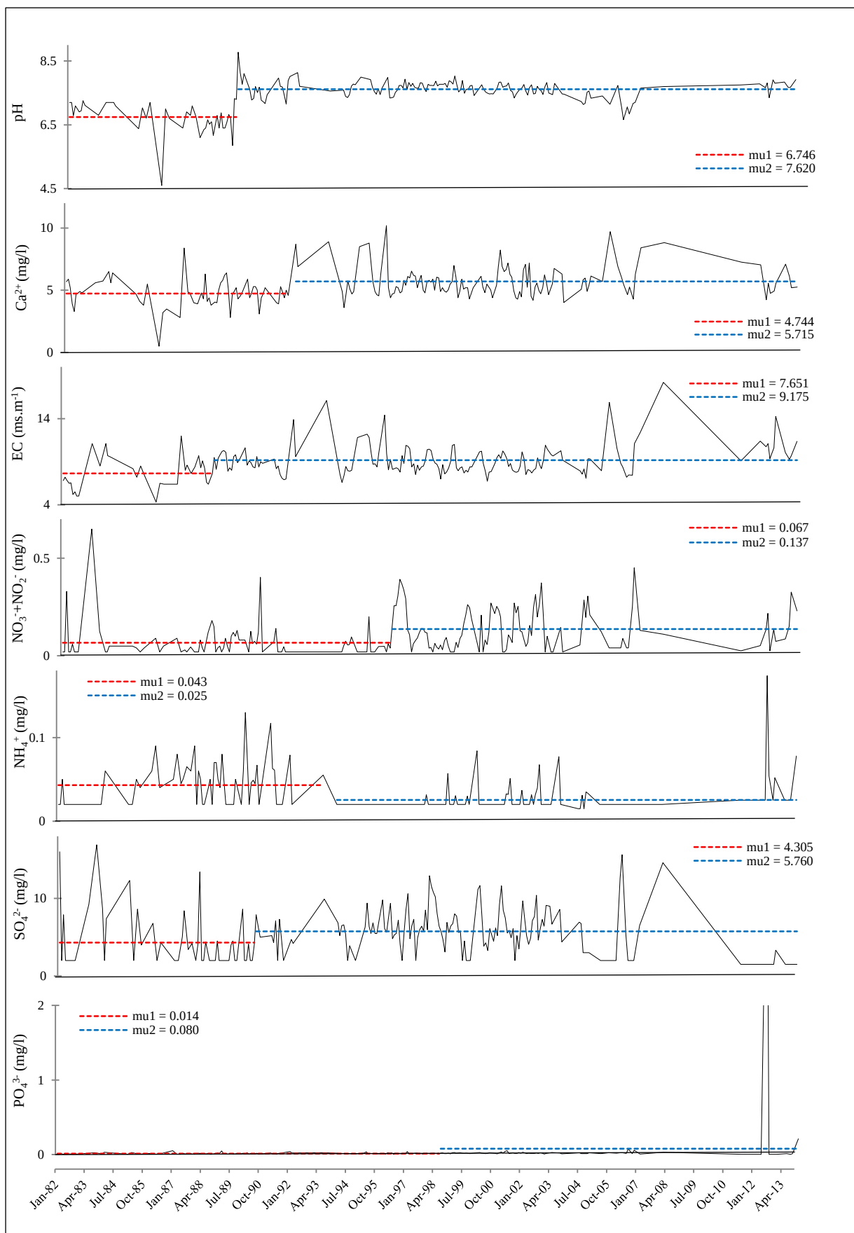
Figure 2.6: Water quality trends in the Upper Mokolo (A4H002), based on Pettitt's homogeneity tests on monthly medians.
