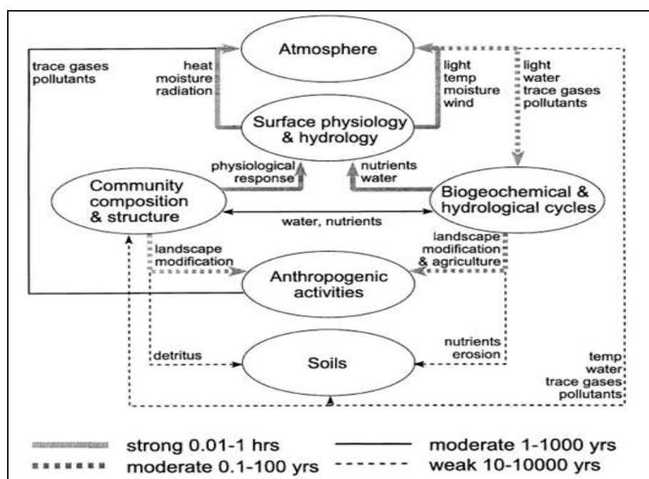
Figure 1.1: General overview of hydrobiogeochemical interactions and pathways, at various temporal scales. (adapted from Hutjes et al., 1998).
