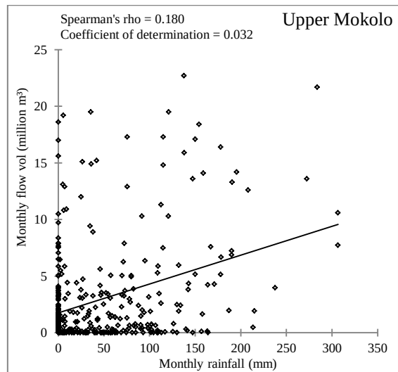
A4: Correlation scatterplots for monthly rainfall totals vs monthly stream flow volumes.
