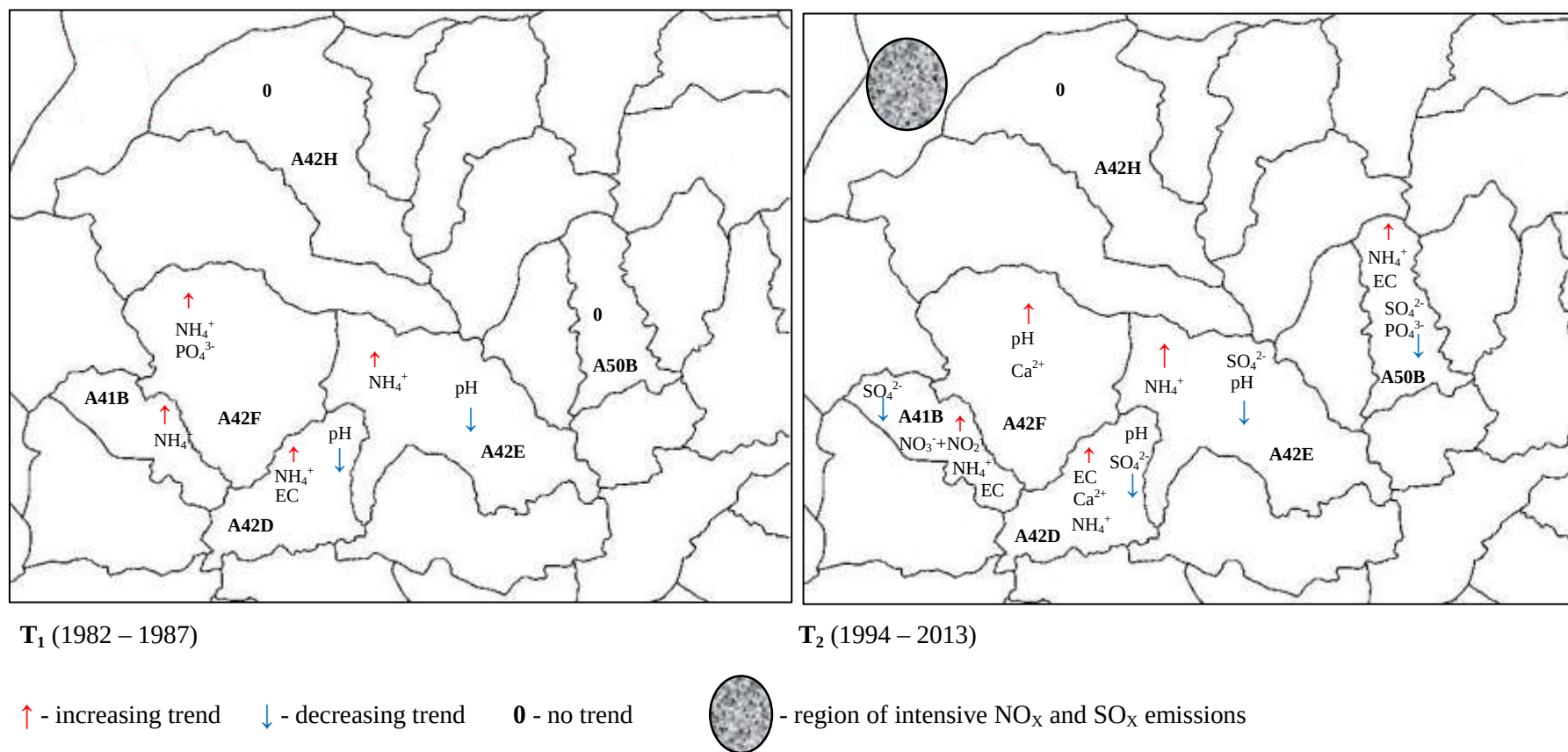
Figure 2.16: Before and after trend directions in the quaternary catchments of the Waterberg (on LOWESS residuals). Only variables with increasing or decreasing trends are shown. Detrending the effects of Q was achieved using the LOWESS method. Deseasonalisation was accomplished by the Seasonal M-K test, which represented the final stage of the overall trend analysis that was performed in addition to the M-K trend test.
