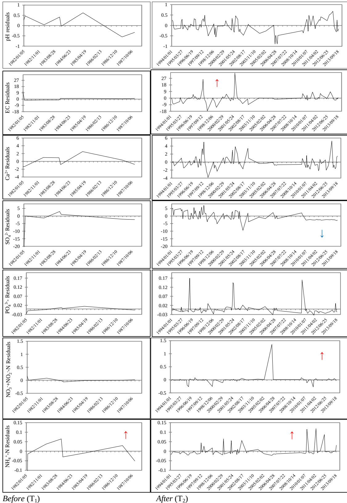
Figure 2.11: Post-LOWESS WQ residuals versus time for the Matlabas river (A4H004).
