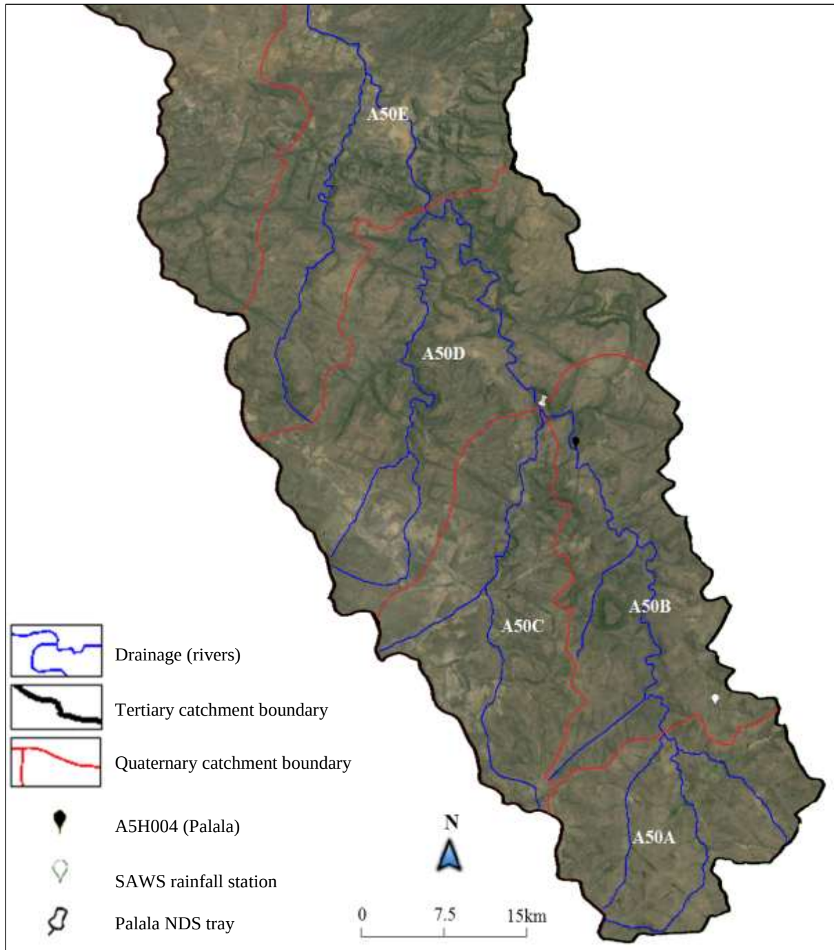
Figure 1.6: Tertiary catchment A50 showing drainage and location of sampling sites.
