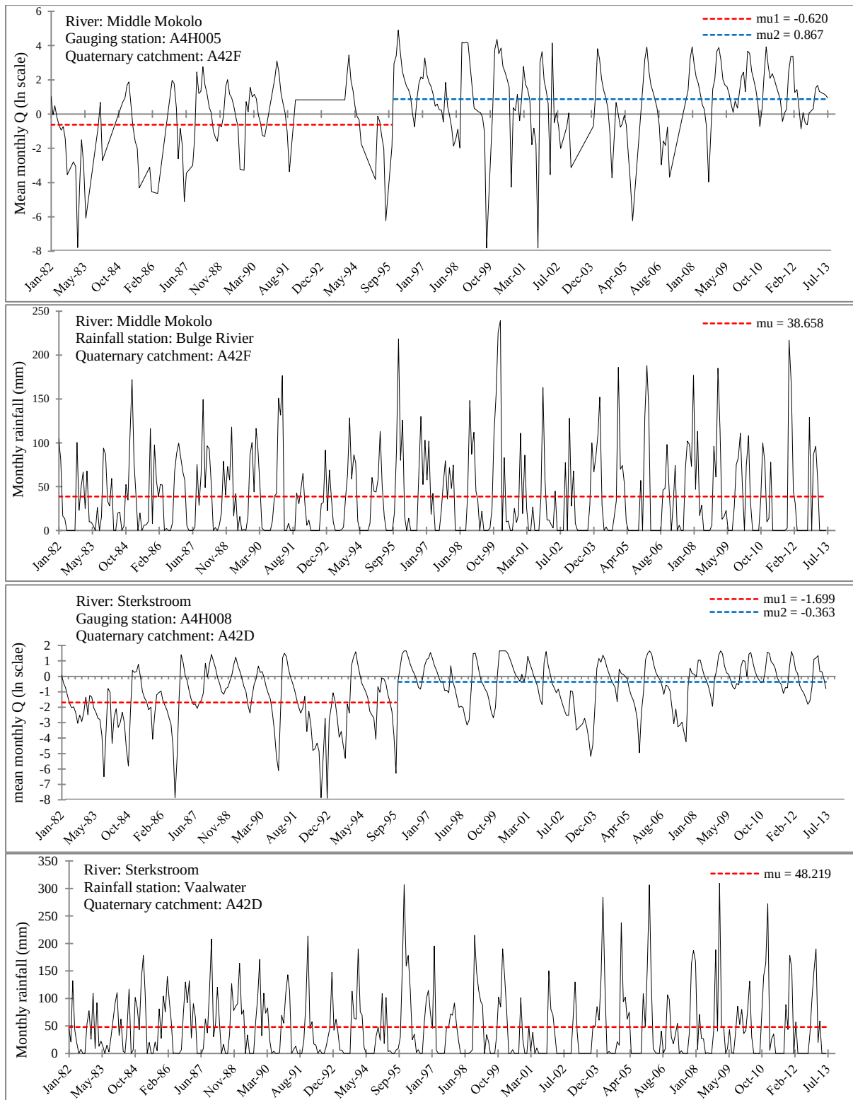
Figure 2.1: Monthly discharge and rainfall trends in the Middle Mokolo and Sterkstroom, based on Pettitt's homogeneity tests.
