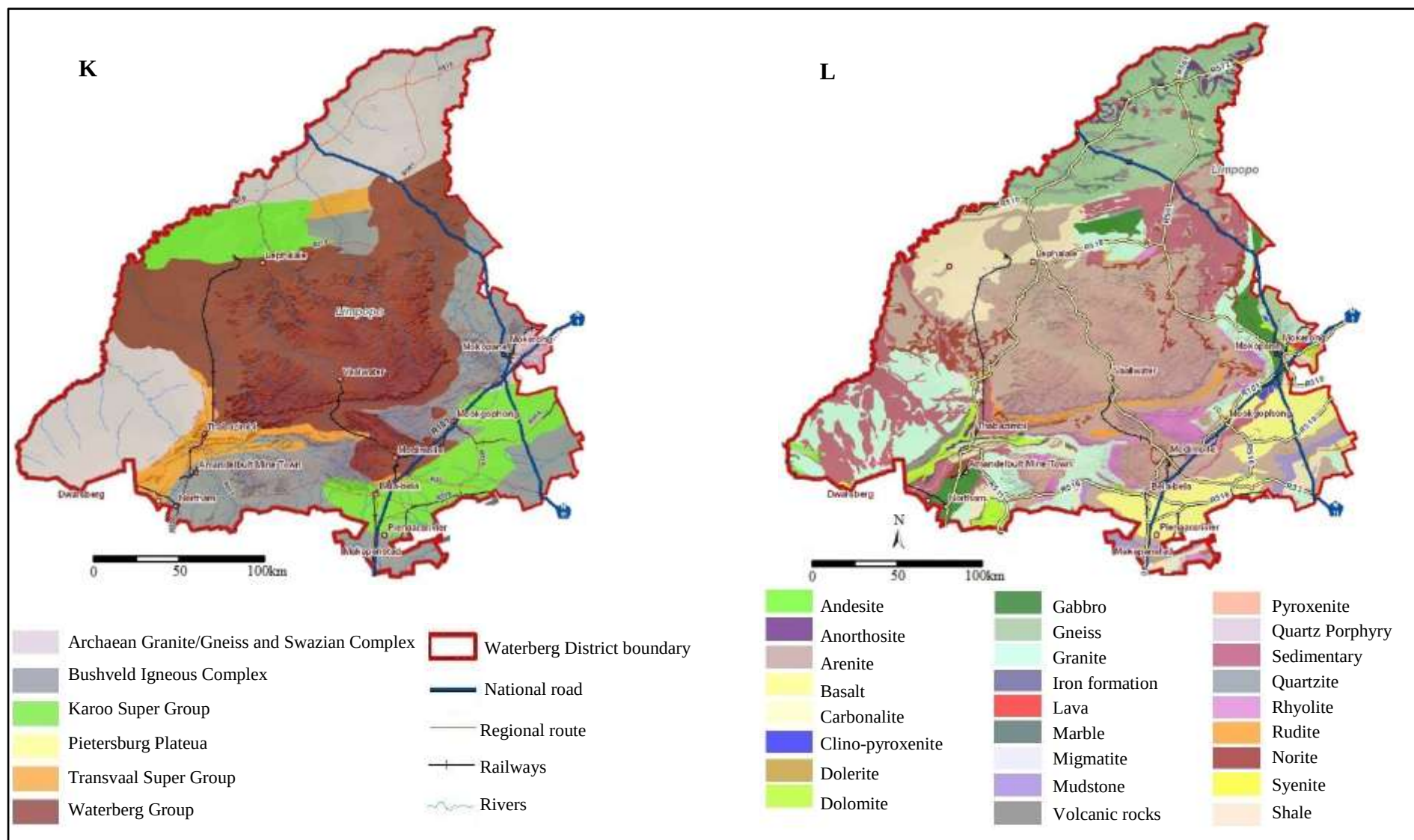
Figure 1.13: Simplified geological map (K) and dominant rock types (L) (Source: Waterberg EMF 2010).
