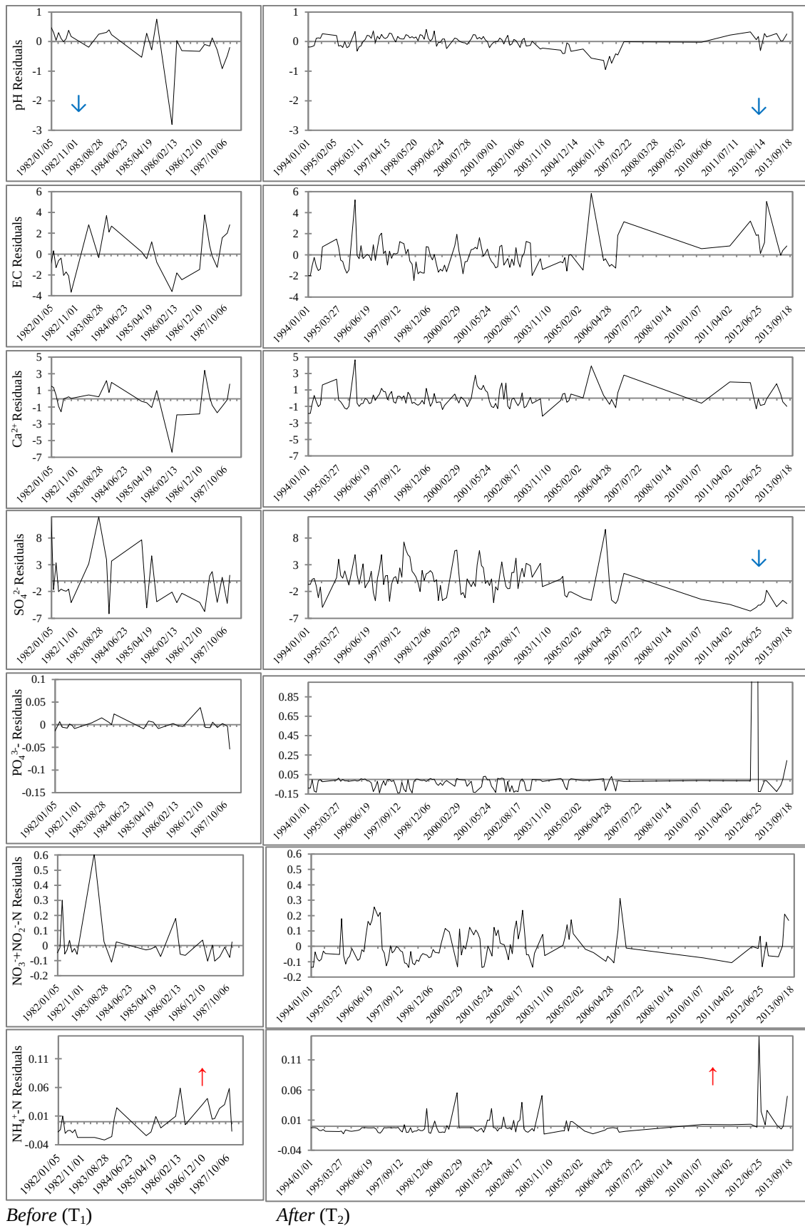
Figure 2.14: Post-LOWESS WQ residuals versus time for the Upper Mokolo river (A4H002).
