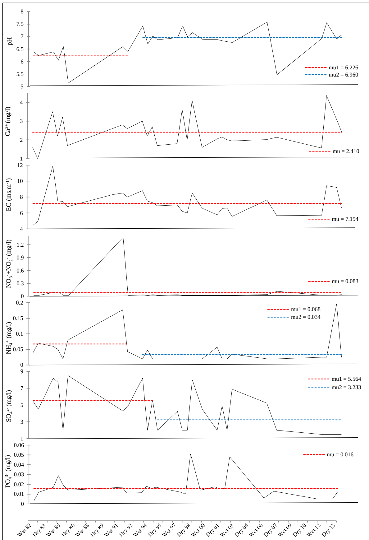
Figure 2.8: Water quality trends in the Tambotie (A4H007), based on Pettitt's homogeneity tests on seasonal medians.
