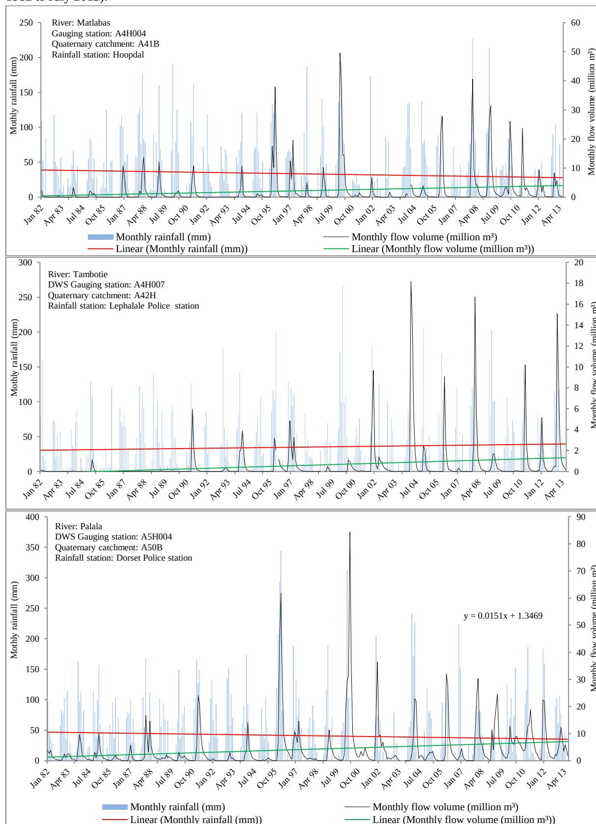
A2: Long-term monthly flow volume and rainfall trends in 4 ry catchments A41B, A42H and A50B (January 1982 to July 2013).
