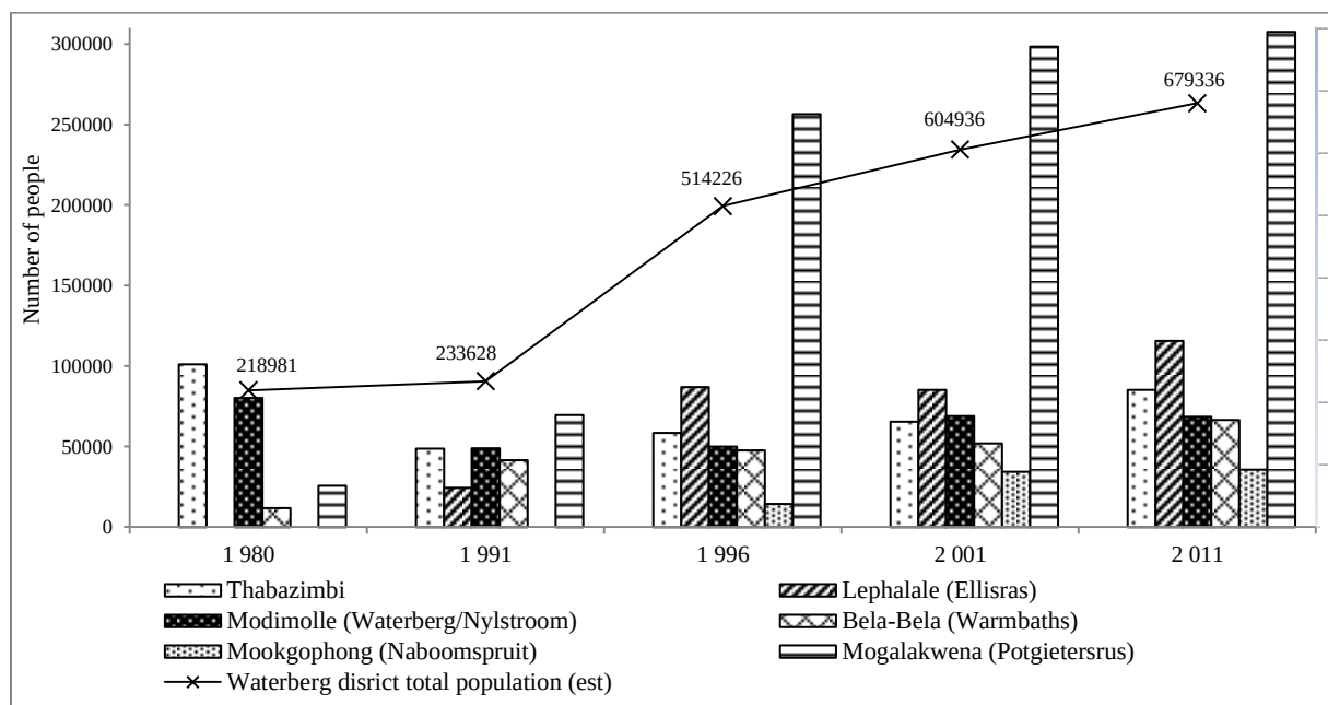
Figure 1.7: Historical human population estimates for what is today the Waterberg District Municipality, comprising 6 local municipalities. The former municipal names are included in parentheses. The 1980 and 1991 census estimates do not include the former homelands of Lebowa and Bophuthatswana. (Source: Stats SA http://www.statssa.gov.za/?page_id=964 ).
