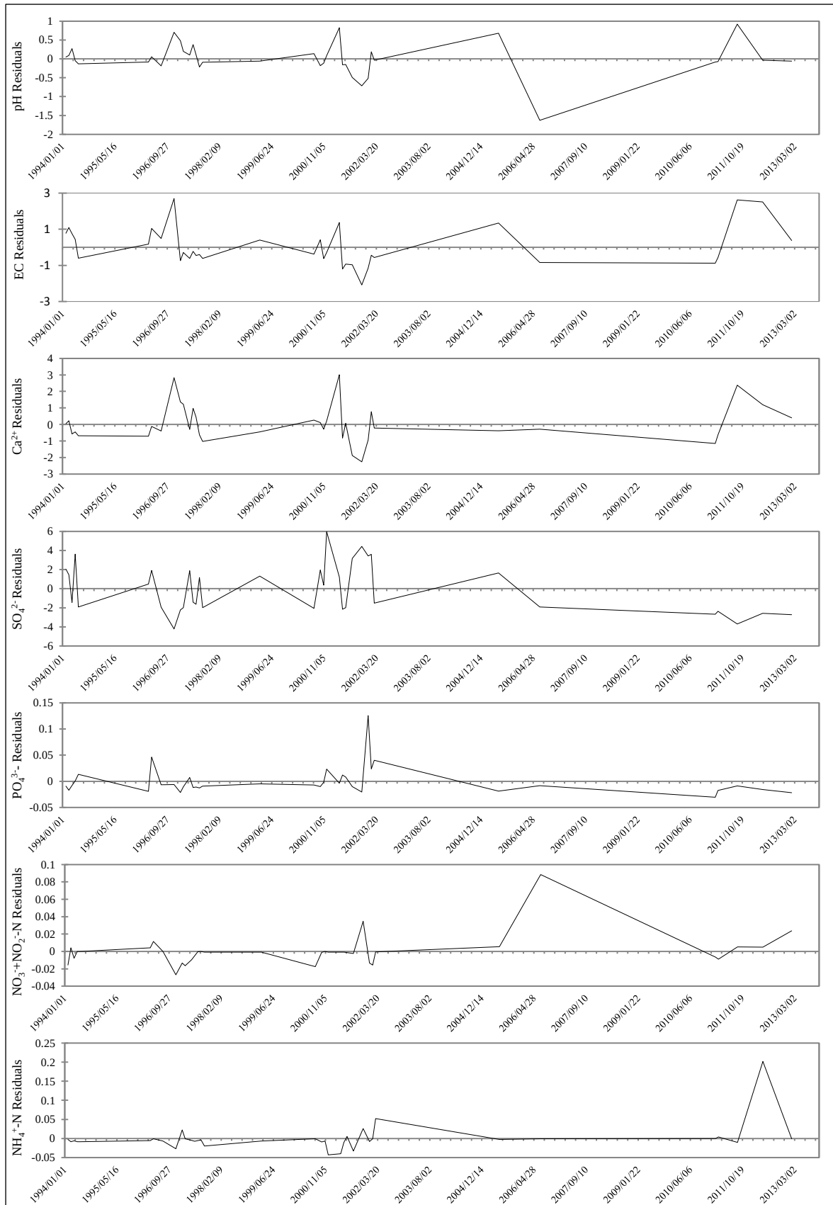
Figure 2.15: Post-LOWESS WQ residuals versus time for the Tambotie river (A4H007). There was insufficient data for a pre-LOWESS regression and trend tests for T_1 (only 6 observations between 1982 and 1987).
