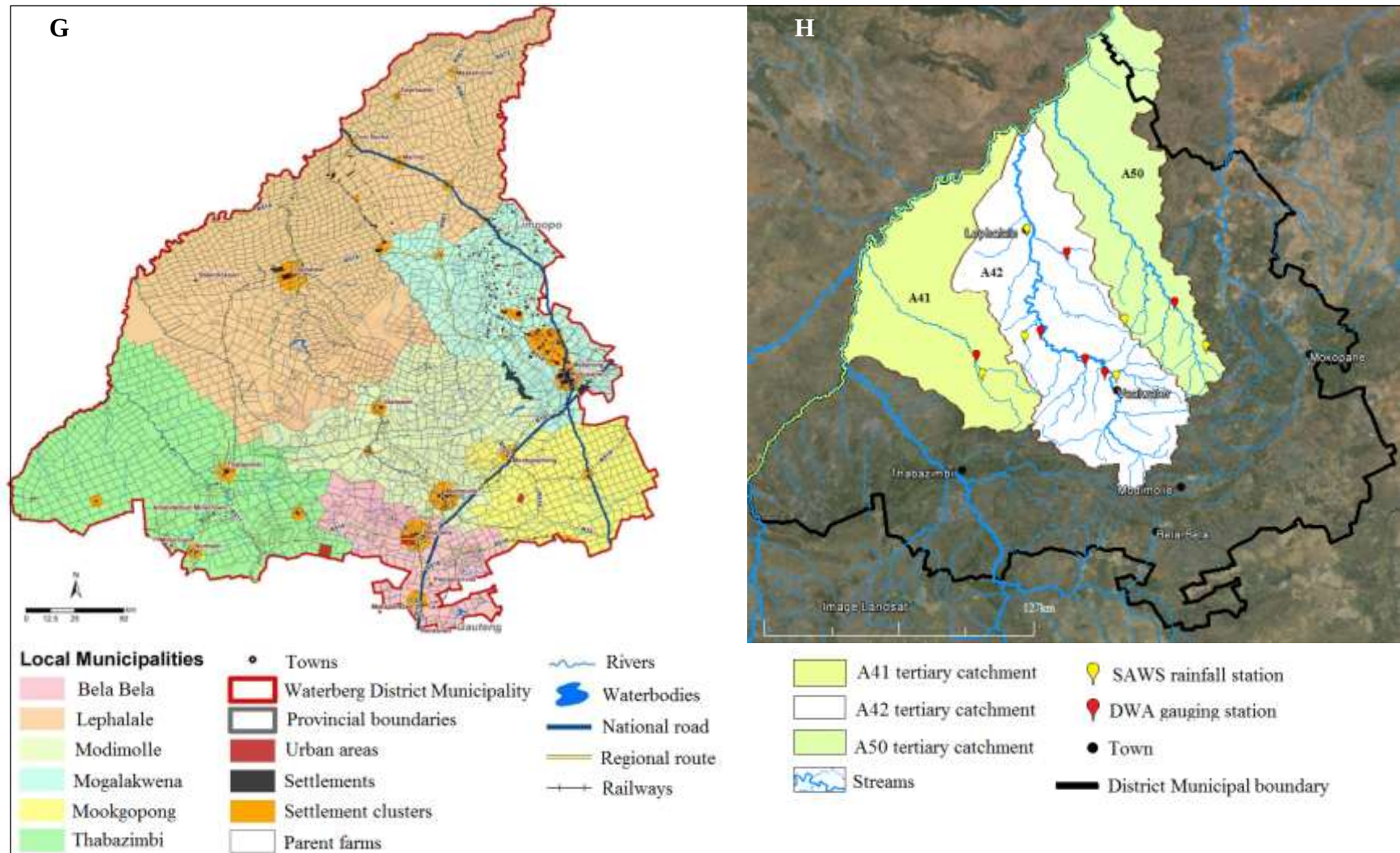
Figure 1.8: Waterberg district municipality (G) showing human population settlement clusters (Source: Waterberg EMF 2010) and study sites showing tertiary catchment boundaries (H).
