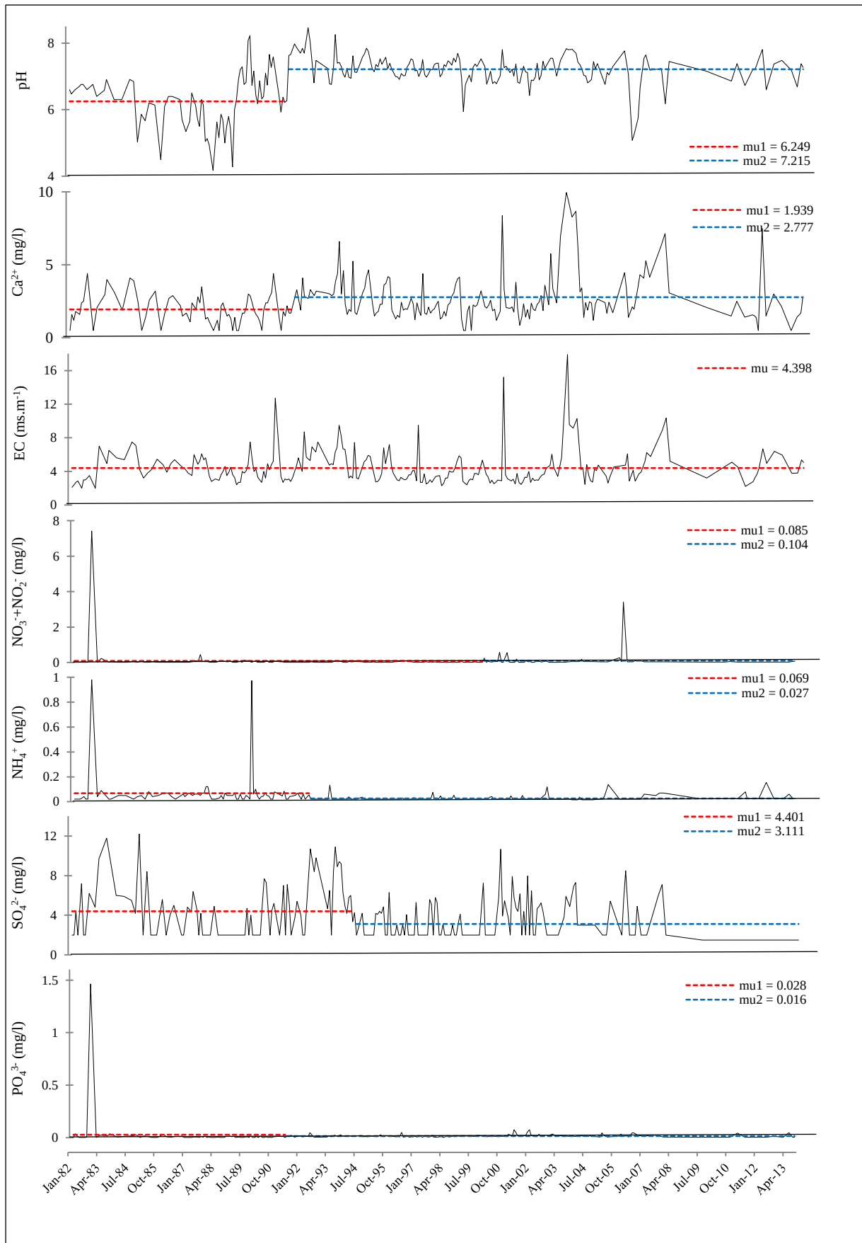
Figure 2.7: Water quality trends in the Sterkstroom (A4H008), based on Pettitt's homogeneity tests on monthly medians.
