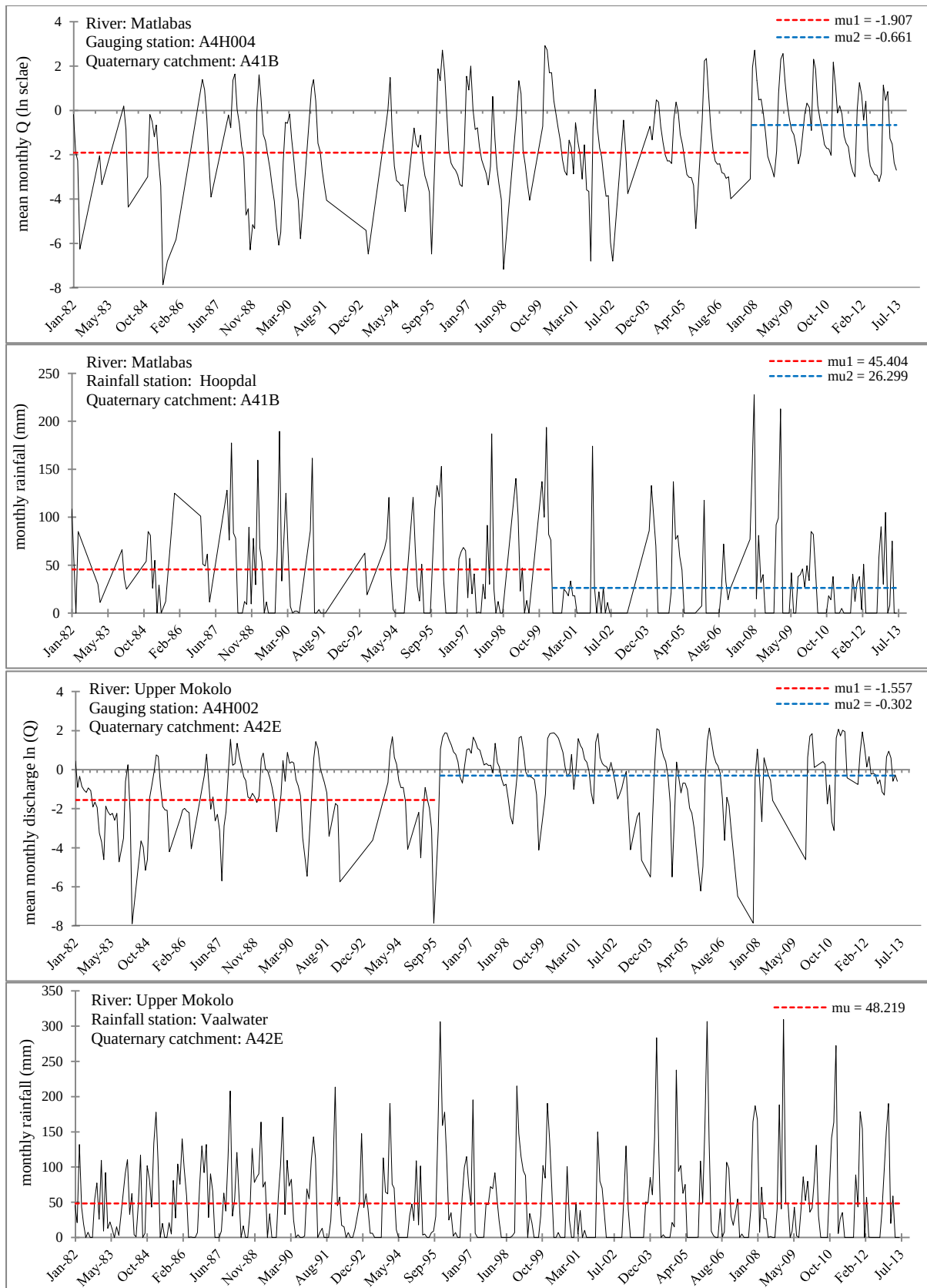
Figure 2.2: Monthly discharge and rainfall trends in the Matlabas and Upper Mokolo, based on Pettitt's homogeneity tests.
