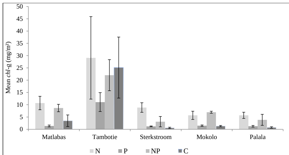
Figure 3.2: Periphyton growth, measured as mean chl- \bar{a} , after 9 days incubation period. Standard deviation shown as Y-error bars.
