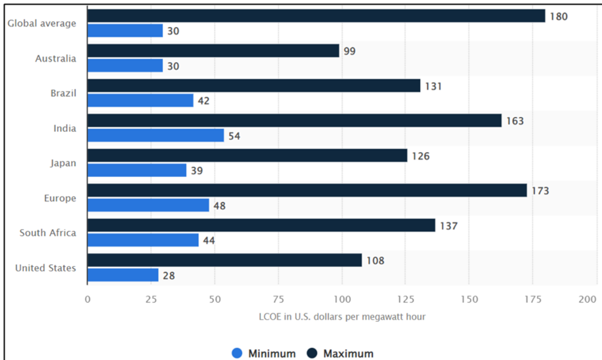
Figure 2.3: Global Levelised Cost for Solar Photovoltaic as of 2021 (USD/Megawatt) (Source: IRENA, 2020b, p 4)
