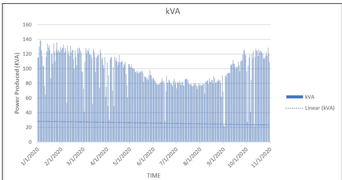
Figure 4.2: Performance data for Kempton Park Solar PV in 2020 (Source: CoE Metering on-line system obtained from CoE officials).
