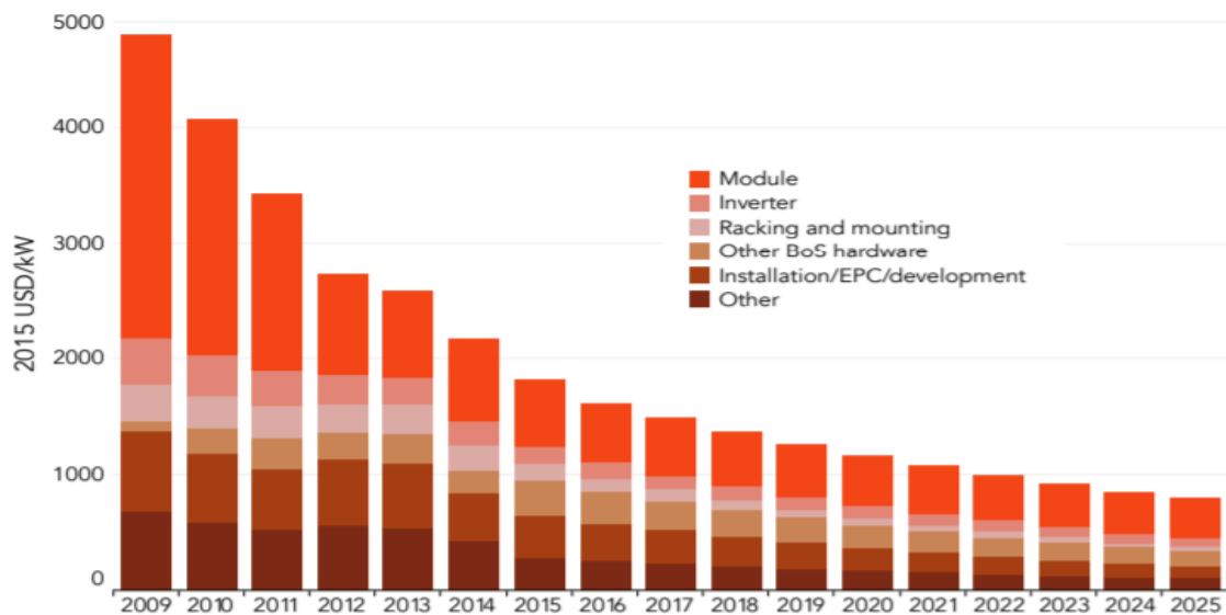
Figure 4.14: Projected decrease in Solar PV costs to 2025 (Source: Eskom, 2018, p 19)
