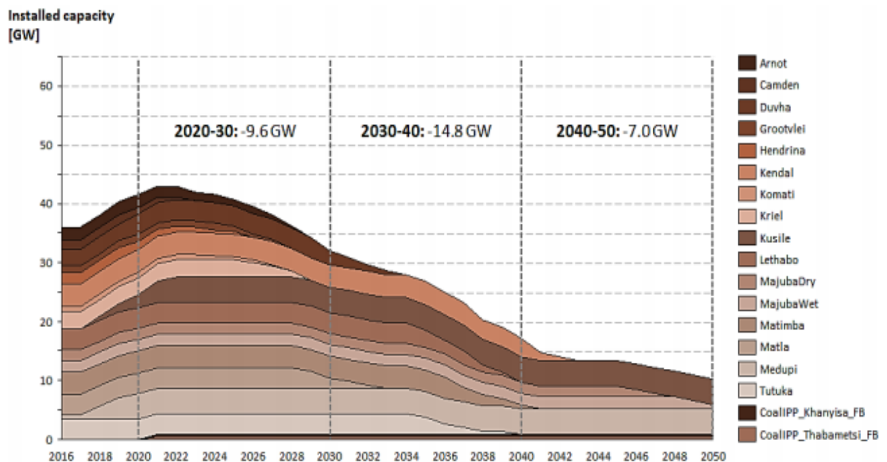
Figure 2.6: Decommissioning schedule for coal-fired power plants (Source, ERC, CSIR and IFPRI, 2017, p 14)
