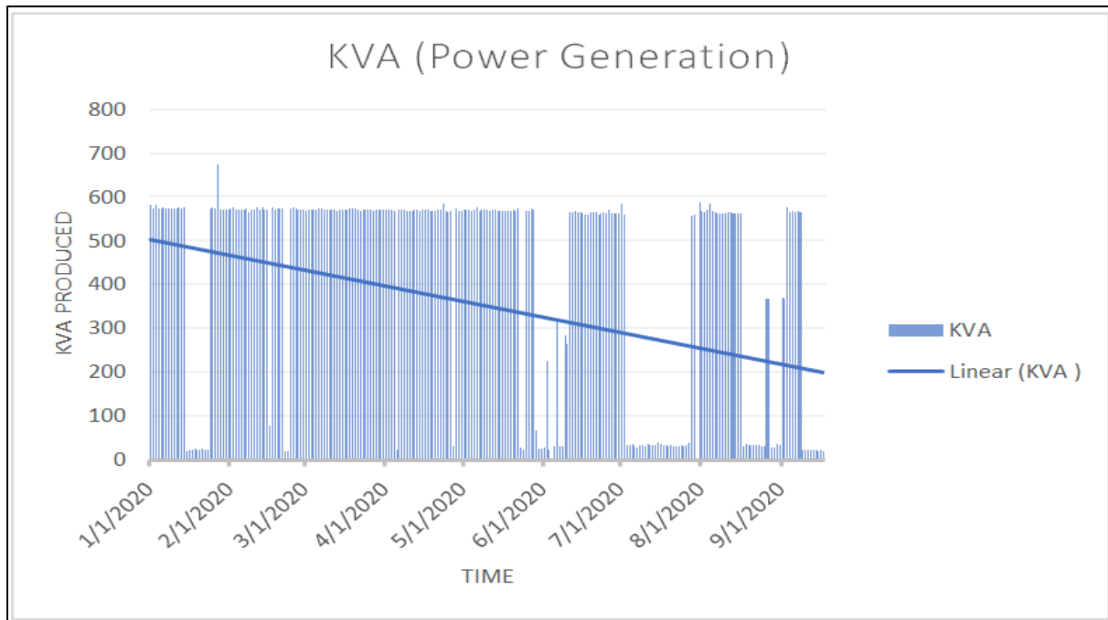
Figure 4.4: Performance data for Simmer and Jack Landfill Gas Plant (Source: Source: CoE Metering on-line system, obtained from CoE officials, 2020).
