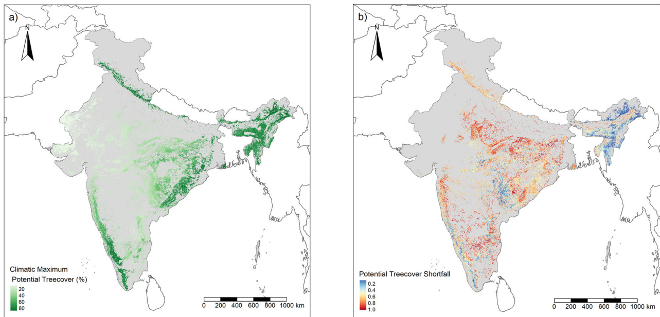
Fig. 2 | Climatic maximum potential tree cover (%) and Potential tree cover shortfall. The climatic maximum potential tree cover is the maximum tree cover based on the maximum climate water deficit (MCWD), fitted with 95th percentile smooth additive quantile regression model. It is the highest in north-eastern India and the stretch of the Western Ghats along the western coast of peninsular India (a). Potential tree cover shortfall is a measure of the convergence/ divergence of the current tree cover with the climatic maximum potential tree cover. It has a range of 0–1, where values close to 1 indicate divergence of current tree cover from the climatic maximum potential tree cover (or there is 0% current tree cover) (shades of
