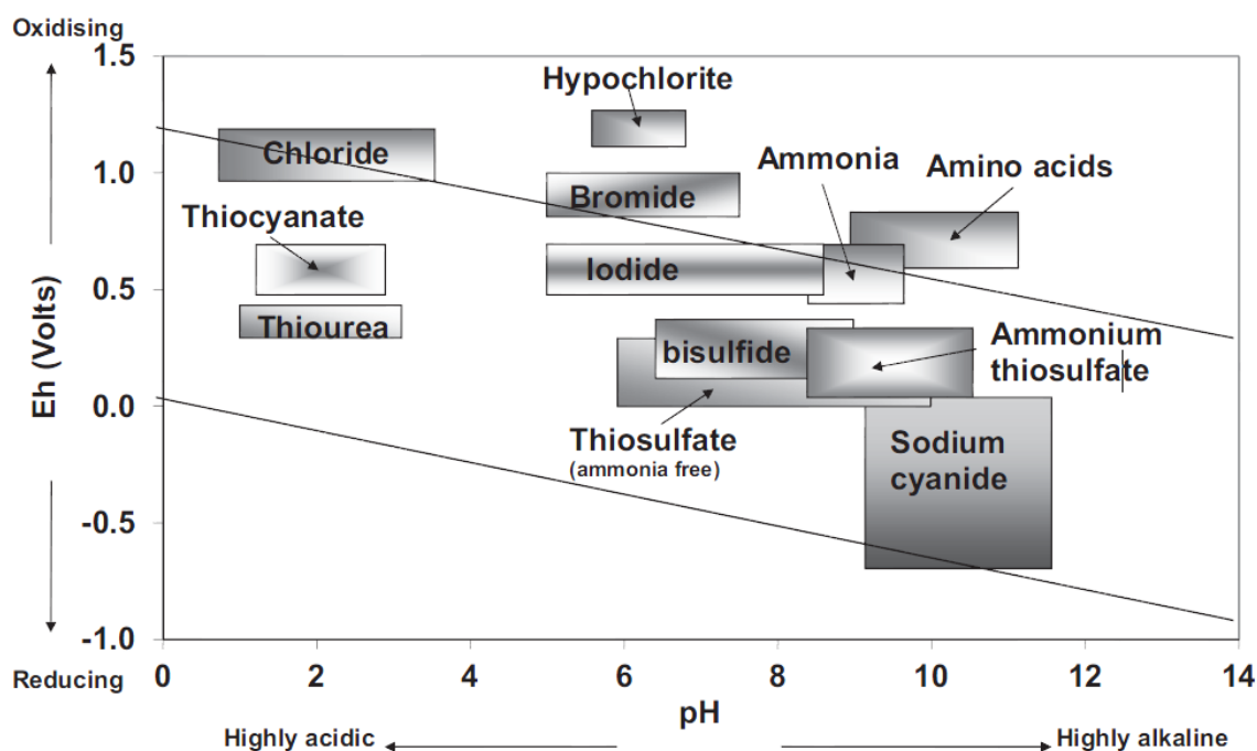
FIGURE 3 Stability fields (Eh and pH) of various gold lixiviants (Aylmore, 2016a). Note- the sodium cyanide operating conditions are significantly larger than any alternative lixiviant
