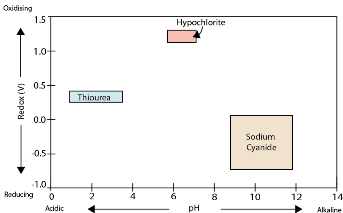
Figure 1 Stability fields (Eh and pH) of various gold lixiviants (Aylmore, 2016a). Note- the sodium cyanide operating conditions are significantly larger than any alternative lixiviant.
