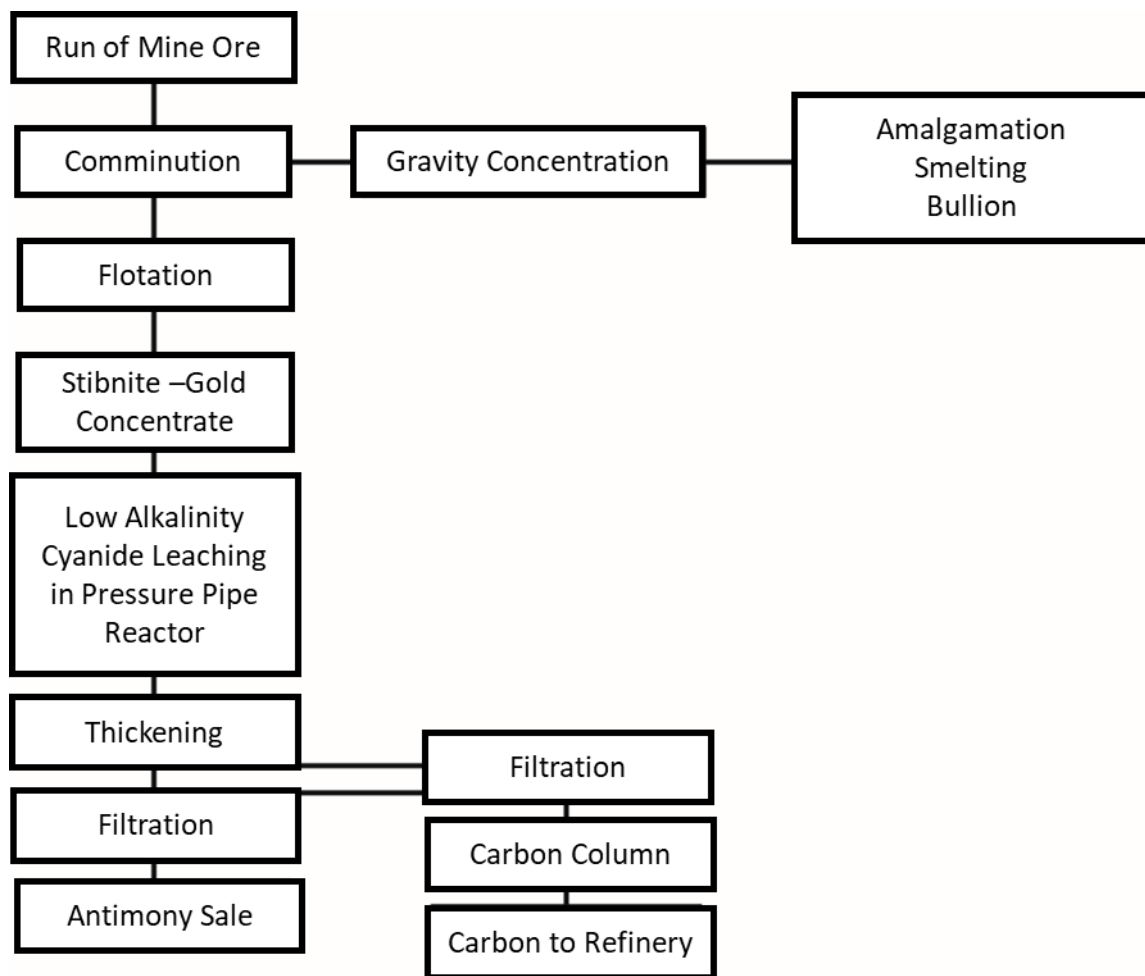
Figure 2-15 Processing flow chart for Consolidated Murchison, a simplified diagram (Davis, 1986; Marsden and House, 2006). Low alkalinity pressure leaching of this ore has been used to deal with the highly refractory nature of this ore.
