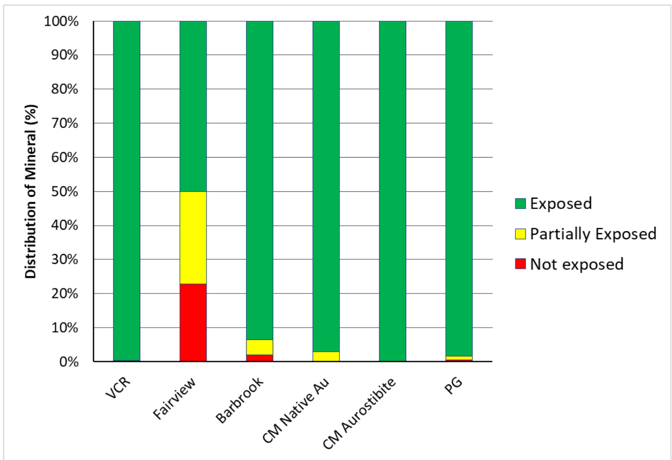
Figure 6-14 Gold mineral exposures for each sample, subdivided into not exposed, partially exposed, and exposed. The Fairview sample has notably moderate exposure while the remaining samples have excellent exposure. CM – Consolidated Murchison, PG – Pilgrim’s Rest.
