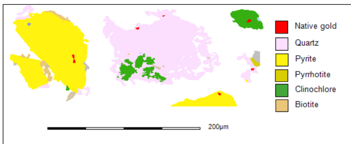
Figure 2 False colour images, produced by MLA, of the remaining gold grains in the residue from the chlorite-hypochlorite leach.
