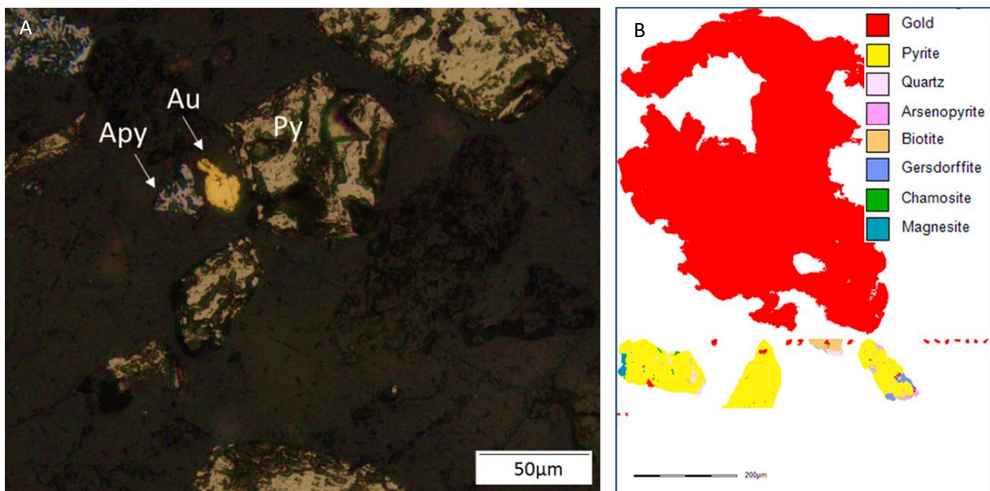
FIGURE 5 Fairview ore minerals A) Example of mineralisation, including arsenopyrite (Apy), pyrite (Py) and gold (Au). The gold grain has an equivalent circular diameter of 46.5 \mu\text{m} . B) The range in size of gold grains at Fairview is evident in this false colour MLA-generated image of polished blocks of panned concentrate.
