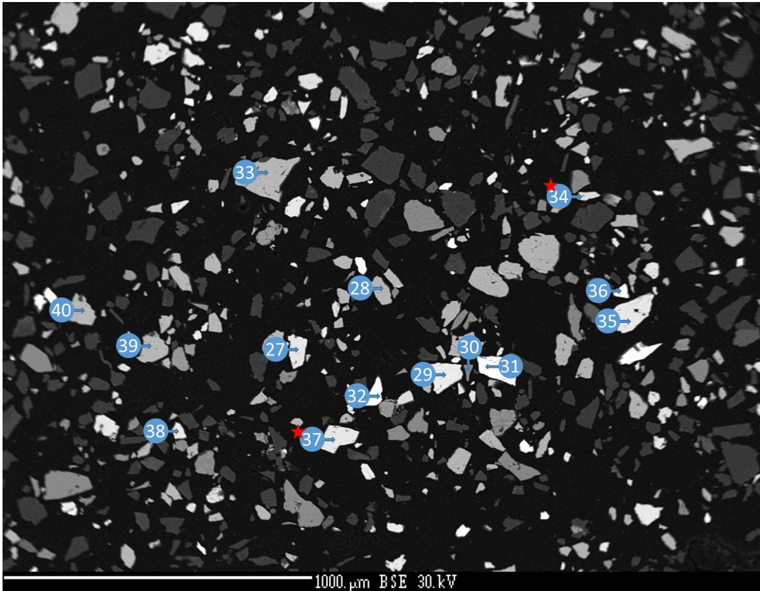
Figure 6-18 The points of analyses for the Consolidated Murchison material. Points with gold detected have been marked in red. Each point correlates with the data found in Table 6-6 and have the chemical composition of stibnite.
