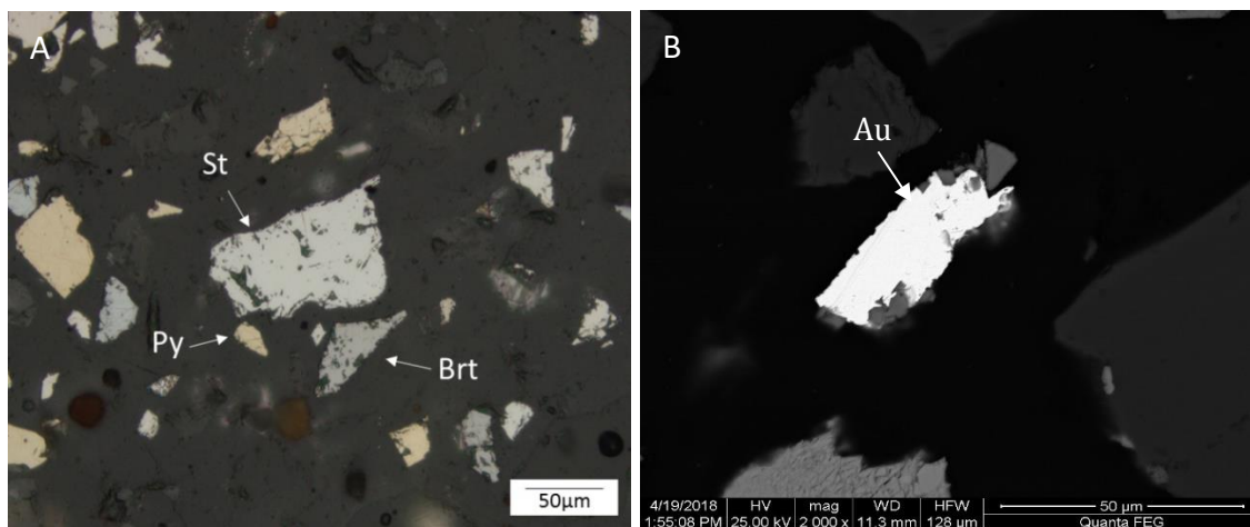
Figure 5 A) An example of mineralisation at Consolidated Murchison including stibnite (St), pyrite (Py) and berthierite (Brt). B) Gold grain associated with arsenopyrite, gold is well liberated and exposed, with an ECD of 25.5 \mu\text{m} .
