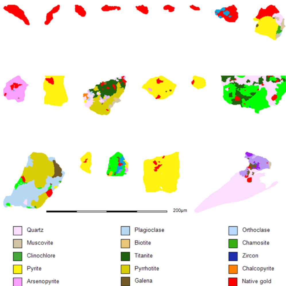
Figure 1 False color MLA images of gold grains (red) and their associated minerals found in the VCR thiosulfate glycine residue
