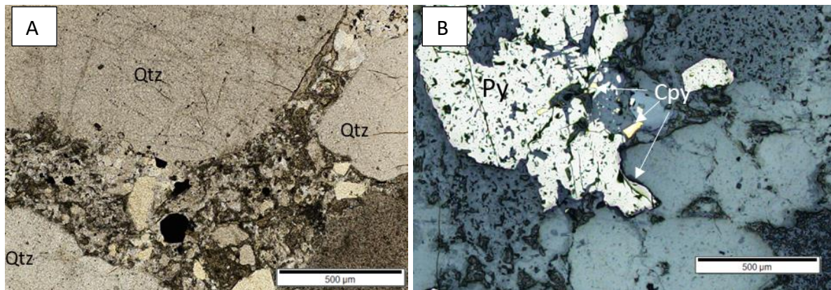
Figure 4-2 Microphotographs from Ventersdorp Contact Reef thin sections. A) A PPL transmitted light image showing the abundant quartz (Qtz) pebbles, interacting with a fine-grained matrix of quartz, chlorite and sericite, pyrite was also present within the matrix (present as black grains in transmitted light). B) A reflected light image of a pyrite (Py) grain associated with chalcopyrite (Cpy) at the margins as is typical for the VCR material.
