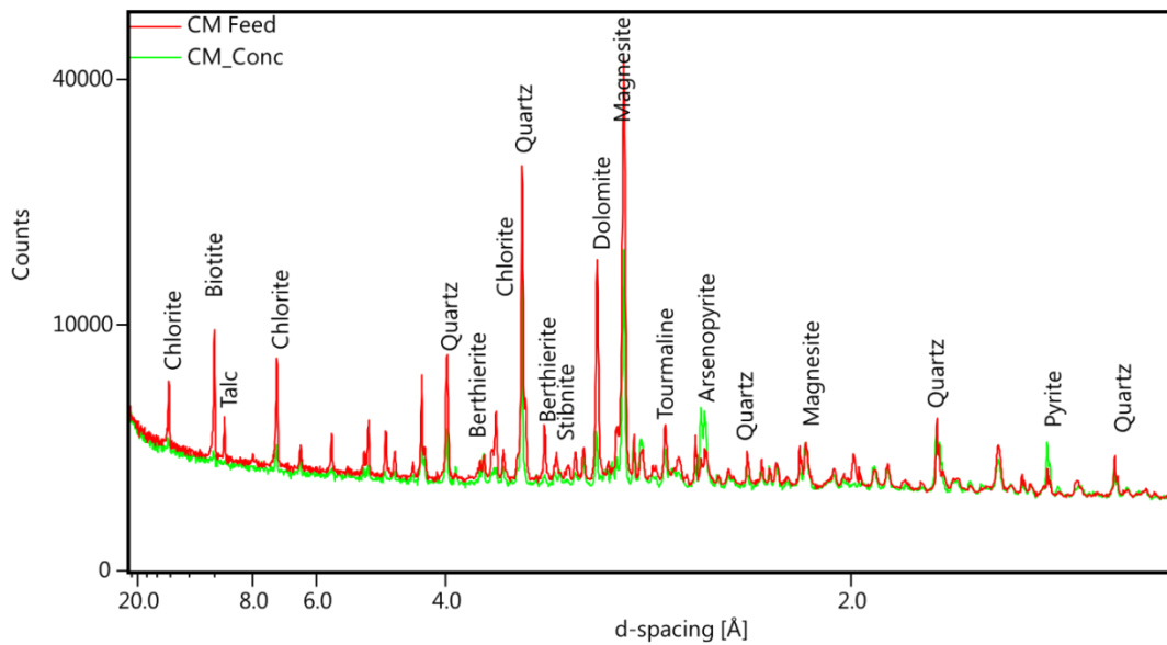
Figure 5-4 X-Ray diffractograms for Consolidated Murchison feed (red) and gravity concentrate (green). The diffractogram shows the increase in arsenopyrite and pyrite in the gravity concentrate.
