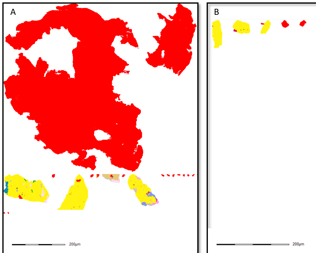
Figure 4 A) An example of the vast range in sizes of gold grains in Fairview, evident in this false colour MLA-generated image, where gold is represented by red. B) All the Barbrook ore gold grains, with pyrite association represented.
