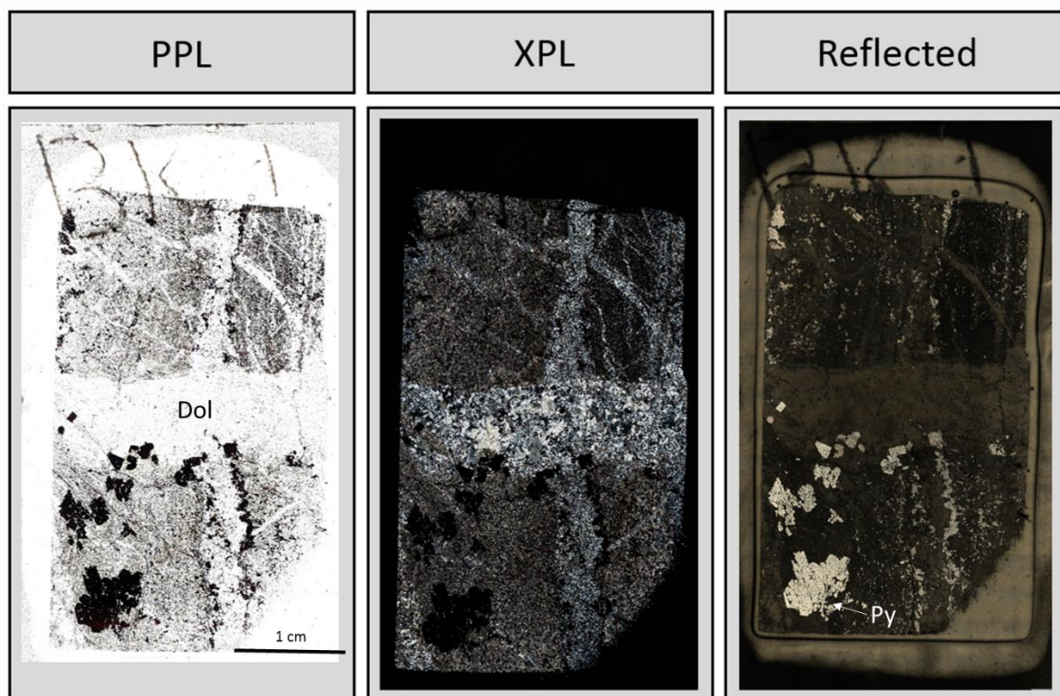
Figure 4-5 Transmitted (PPL and XPL) and reflected light images highlighting the overall mineralogy and texture of the Barbrook sample. The fine-grained groundmass common in this sample is evident, comprised of quartz, chlorite and muscovite. Dolomite (Dol) was abundant in the cross-cutting veins. Pyrite (py) is also present.
