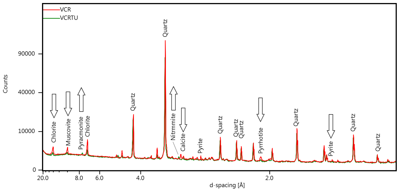
Figure 10-3 XRD pattern for Ventersdorp Contact Reef (VCR) feed (red) and residue (green) overlain to highlight the mineralogical similarities before and after thiourea leaching. As is evident no mineralogical changes took place during leaching.
