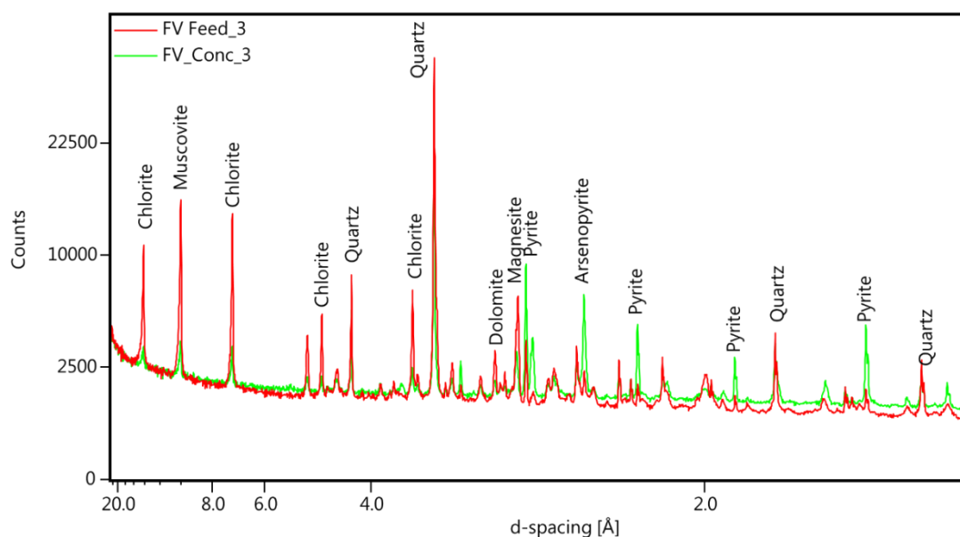
Figure 5-2 X-Ray diffractograms for Fairview feed (red) and gravity concentrate (green). The minerals that were upgraded in the gravity concentrate include pyrite and arsenopyrite.
