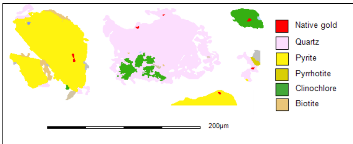
Figure 10-2 False colour images of the remaining gold grains in the Ventersdorp Contact Reef residue from the chlorite-hypochlorite leach. These gains have little to no exposure and are consistently less than 10 µm.
