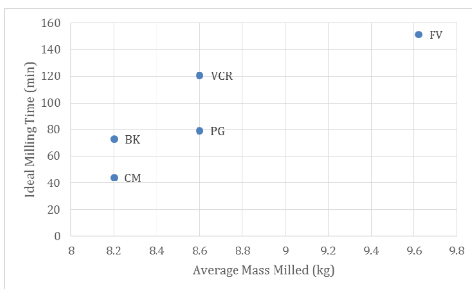
Figure 3-3 Graph representing the relationship between the mass of the material being milled and the time required to obtain a grind of 80% passing 75 \mu\text{m} . This graph highlights that the milling time is not only related to the mass of the milling material.
