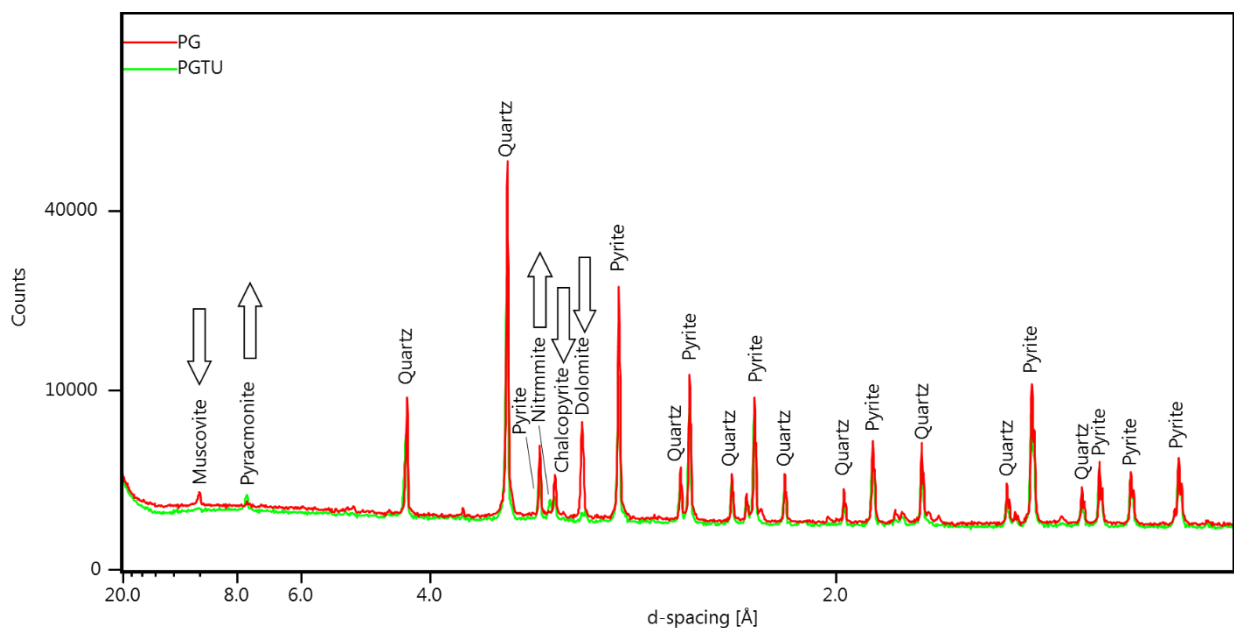
Figure 10-4 XRD pattern for Pilgrim's Rest feed (red) and residue (green) overlain to highlight the mineralogical nature before and after thiourea leaching. The mineralogy was unaffected during this leach
