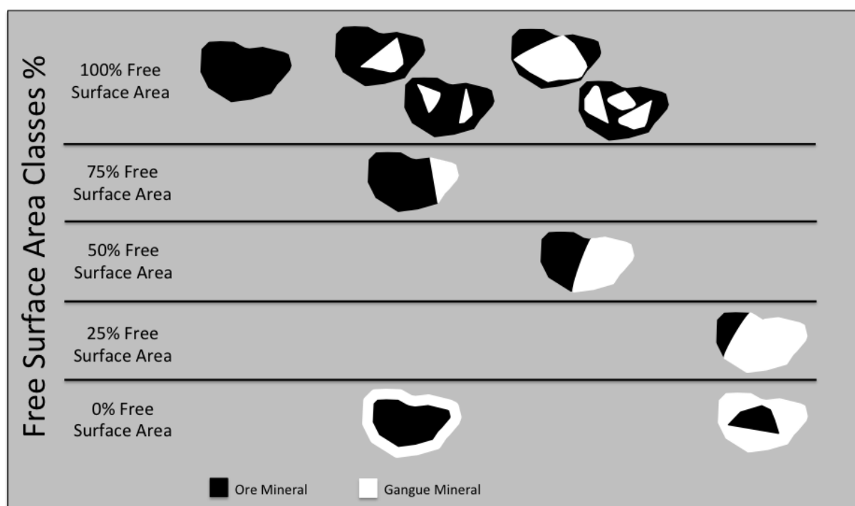
Figure 6-13 The range of classes of free surface area/exposure. Ranging from 100% free surface exposure to 0% free surface exposure (Crop, 2013). The 100% free surface area highlights the difference between liberation and exposure. All of the grains in the top row have 100% exposure, while liberation varies from 100% of the left to less than 25% on the right.
