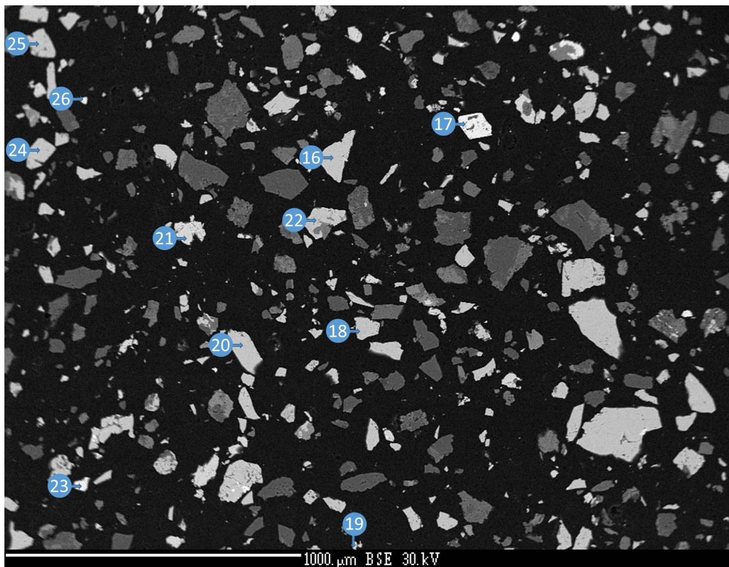
Figure 6-17 The points of analyses for the Barbrook material. Unfortunately, no gold was detected within the sulphides in this sample. Each point correlates with the data found in Table 6-5.
