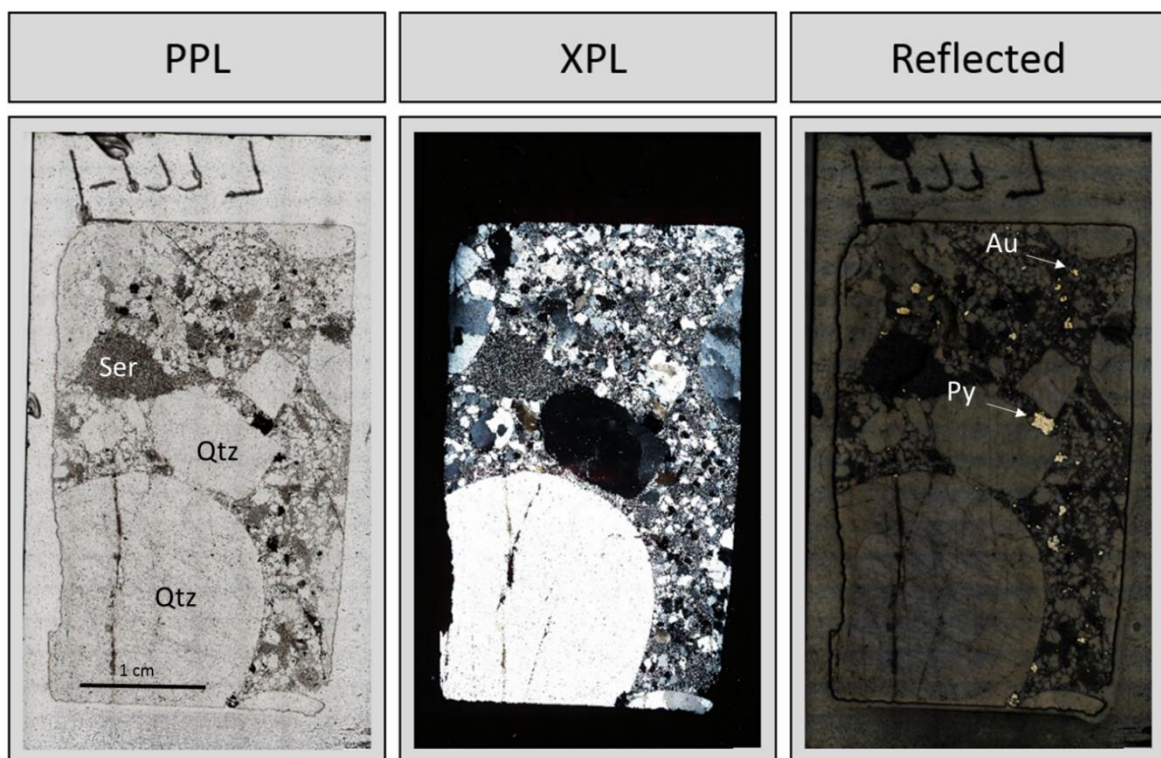
Figure 4-1 Overview photomicrographs of transmitted (PPL and XPL) and reflected light images, these highlight the overall mineralogy and texture of the sample. As is evident in the image, the Ventersdorp Contact Reef sample was a matrix-supported conglomerate. The PPL and XPL images highlight the presence of predominantly quartz (Qtz) clasts. The abundant matrix contained fine-grained quartz, chlorite (Chl) and sericite (Ser). The thin section in reflected light highlights the abundant pyrite (Py) as well as minor gold (Au).
