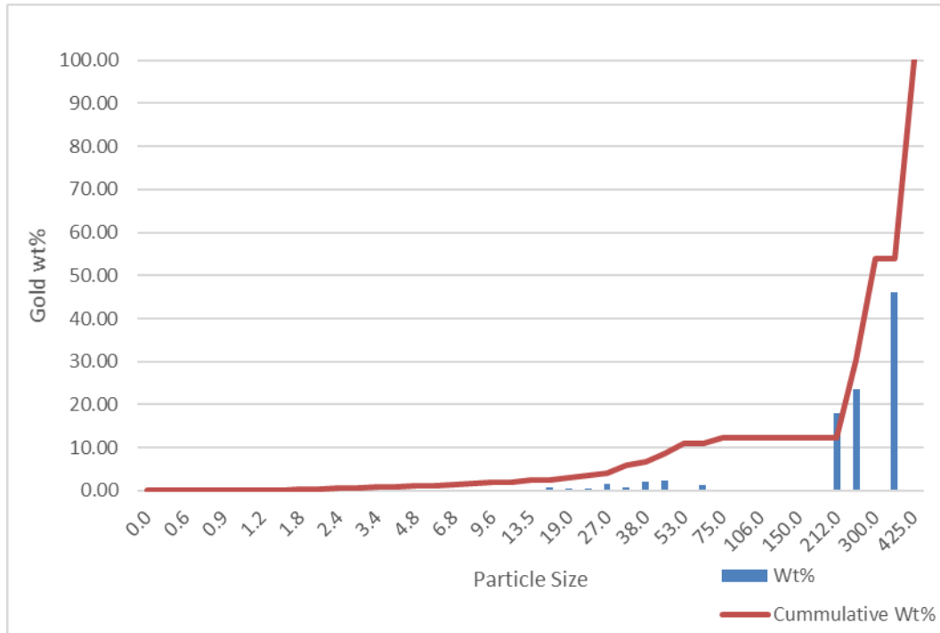
Figure 6-1 The gold grain size distribution for the Ventersdorp Contact Reef sample, with a bar graph representing weight percent contribution for certain size fractions, and line graph representing cumulative weight percent. The gold in the Ventersdorp Contact Reef sample ranged in grain size from 0.5 \mu\text{m} to 425 \mu\text{m} with the majority of gold weight percent occurring in the coarser grained fraction (200 -425 \mu\text{m} )
