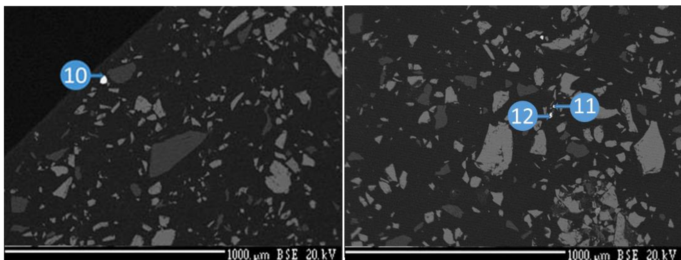
Figure 6-19 Gold grains analysed for Au/Ag content from the Ventersdorp Contact Reef sample (points labelled 1-7) and the Pilgrim's Rest sample (labelled 8-12). Most of the grains analysed were native gold with between 5% and 10% silver.
