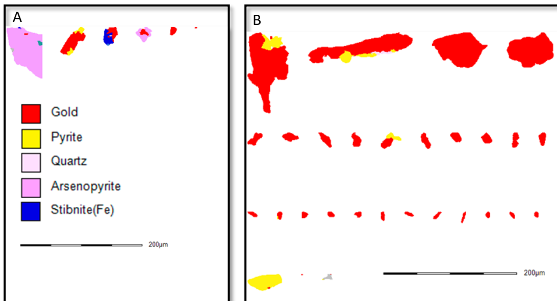
Figure 6-7 False colour MLA images A) Consolidated Murchison sample gold grains, highlighting the grain size distribution, limited number of grains and the lower degree of liberation. The native gold had a limited grain size distribution from 2 \mu\text{m} to 27 \mu\text{m} . B) Pilgrim's Rest sample gold grains, highlighting the range in size, excellent liberation and exposure.
