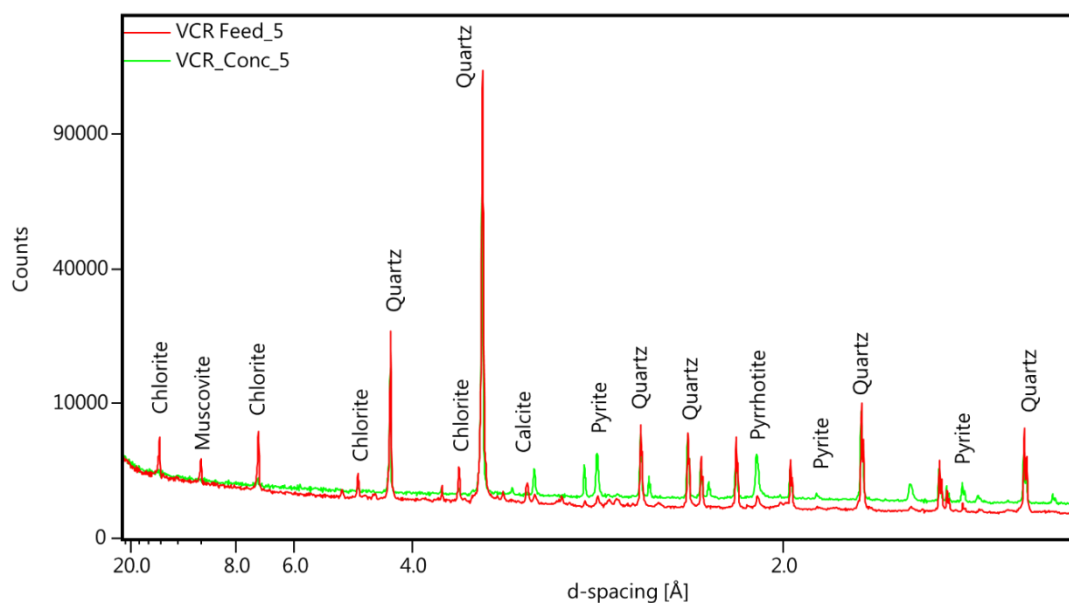
Figure 5-1 X-Ray diffractograms for the Ventersdorp Contact Reef feed (red) and gravity concentrate (green). The gravity concentration process increased the amount of pyrite and pyrrhotite from the feed to the concentrate.
