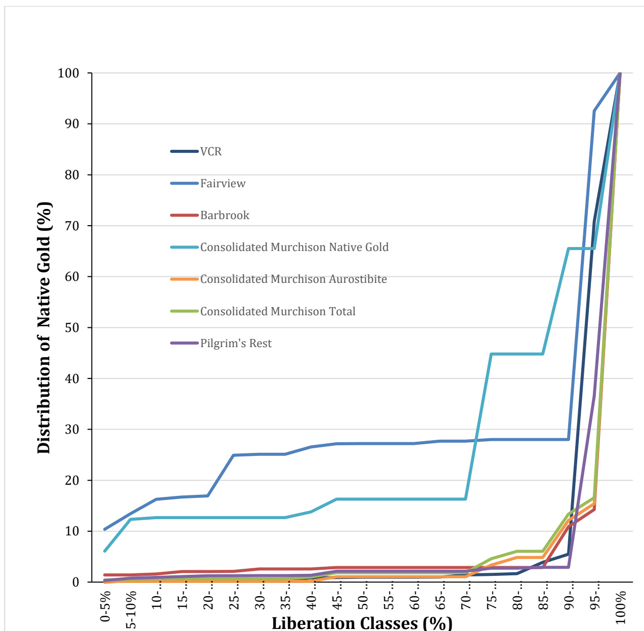
Figure 6-12 Graph representing the cumulative gold liberation by particle composition for the deposits of interest. The lower degree of liberation associated with the Fairview and Consolidated Murchison Native gold is clearly evident. The Ventersdorp Contact Reef, Barbrook and Pilgrim's Rest samples all have good liberation.
