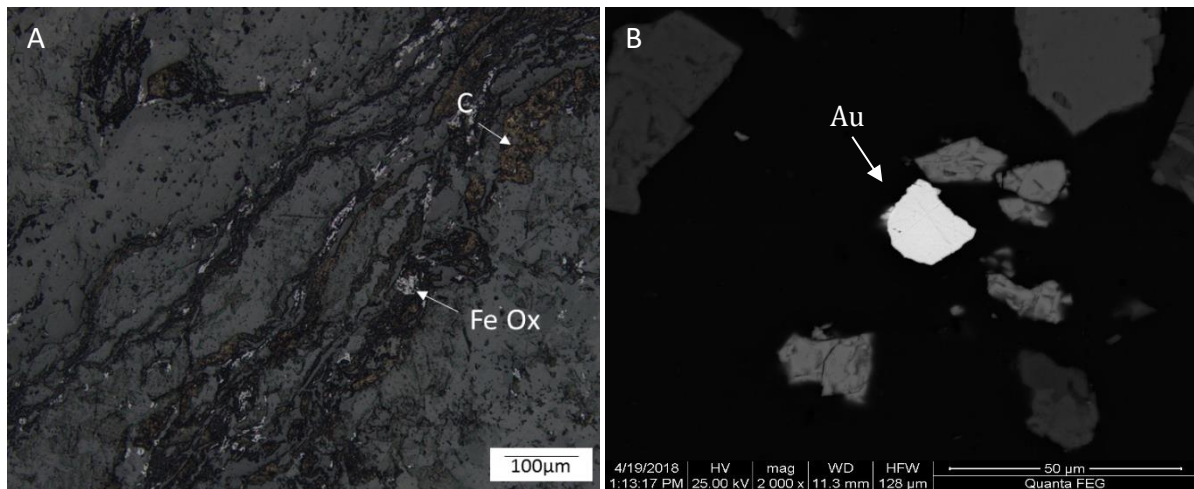
Figure 3 A) Example of carbon found in Barbrook, associated with various iron oxides. B) One of the larger Barbrook gold grains found using the MLA (BSE image) with an ECD of 16.9 μm.
