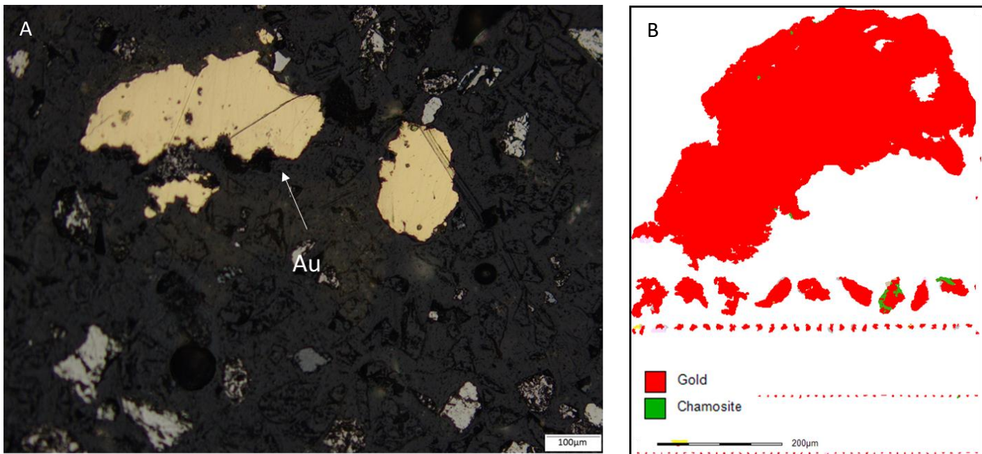
FIGURE 4 VCR gold mineralisation A) Gold grains with several surface exposures of gold, the largest of the gold grains (top left) has an equivalent circular diameter of greater than 250 \mu\text{m} . B) False colour image of a subset of gold grains found in the VCR, with excellent liberation and minor mineral associations.
