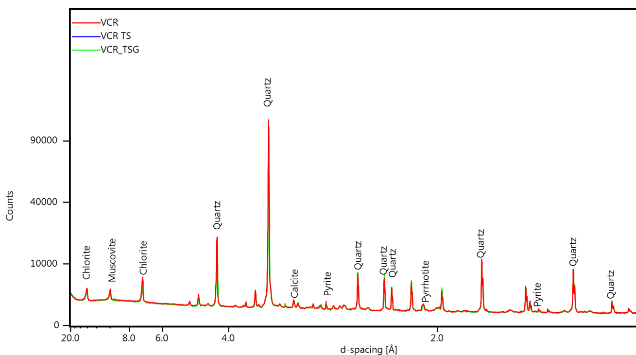
Figure 10-5 The XRD patterns for the Ventersdorp Contact Reef feed material (VCR) and the residue for thiosulphate (VCR TS) and thiosulphate + glycine (VCR TSG) leaching. These patterns are barely differentiable, highlighting the absence of mineralogical change throughout thiosulphate leaching.
