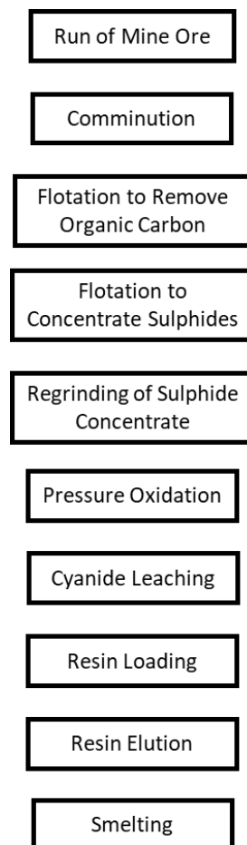
Figure 2-9 Processing flowchart for Barbrook, a simplified diagram generated from Caledonia Mining Resources Annual Reports. Organic carbon in this system is removed using flotation. The sulphides are also concentrated using flotation, after which they undergo further comminution, pressure oxidation and cyanide leaching.
