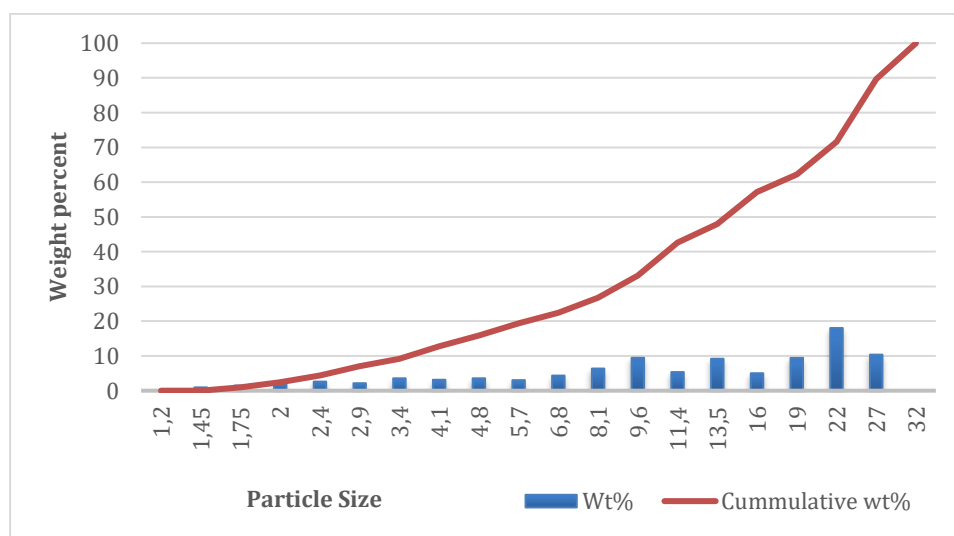
Figure 10-8 Gold grain size distribution from thiosulphate glycine leached Ventersdorp Contact Reef residue.
