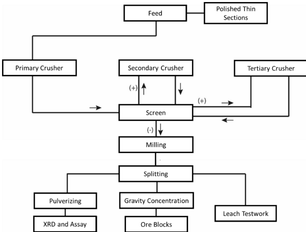
Figure 3-1 Flowsheet for sample preparation for XRD, assay, ore blocks for gold characterisation and leaching. Crushing, milling and splitting were required for the leaching test work, while subsequent pulverisation was needed for XRD and assay. Gravity concentration was used to prepare ore blocks for gold characterisation.
