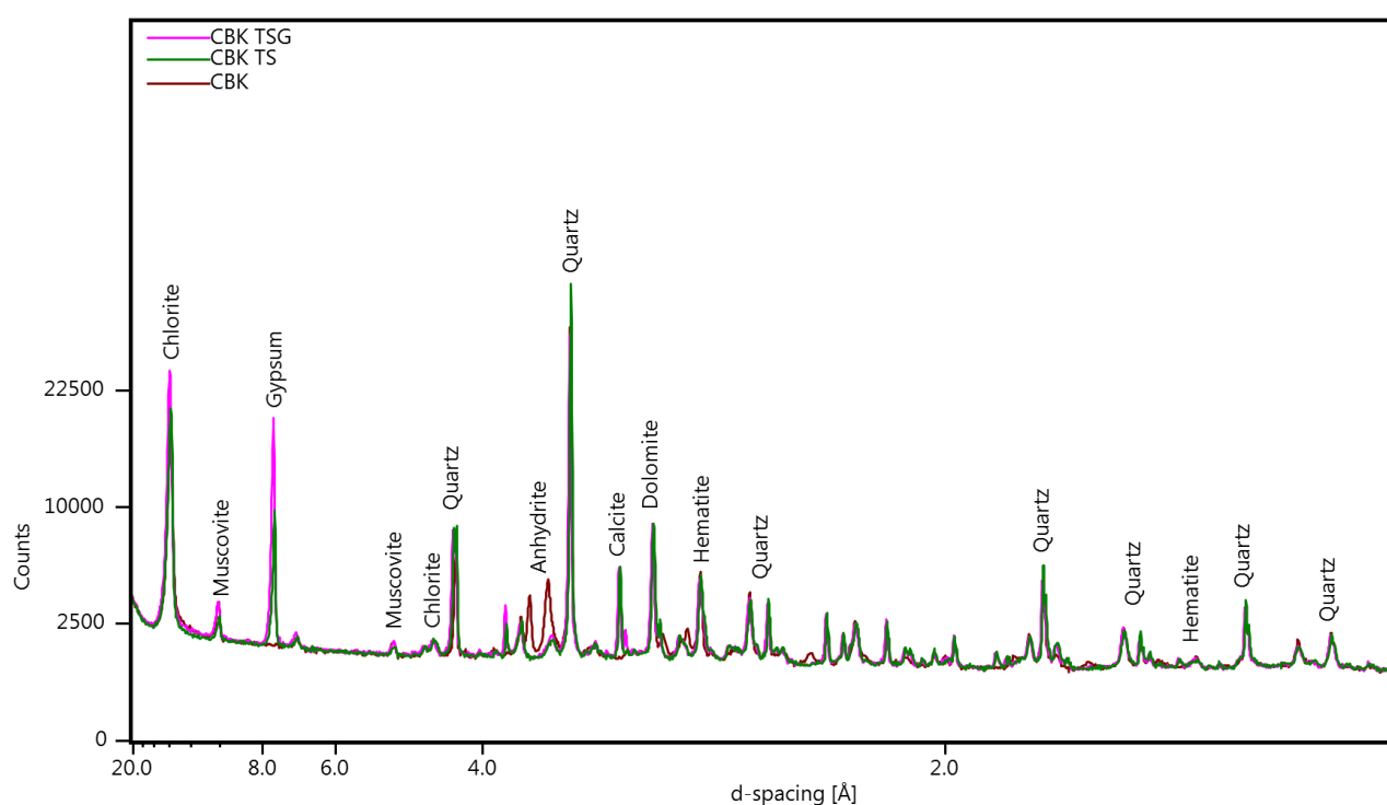
Figure 10-6 XRD pattern for calcined Barbrook material showing very little mineralogical variation from the feed to the residue with the exception of the change from anhydrite to gypsum. CBK- Calcined Barbrook feed, TS- Thiosulphate leach residue, TSG – Thiosulphate + glycine leach residue.
