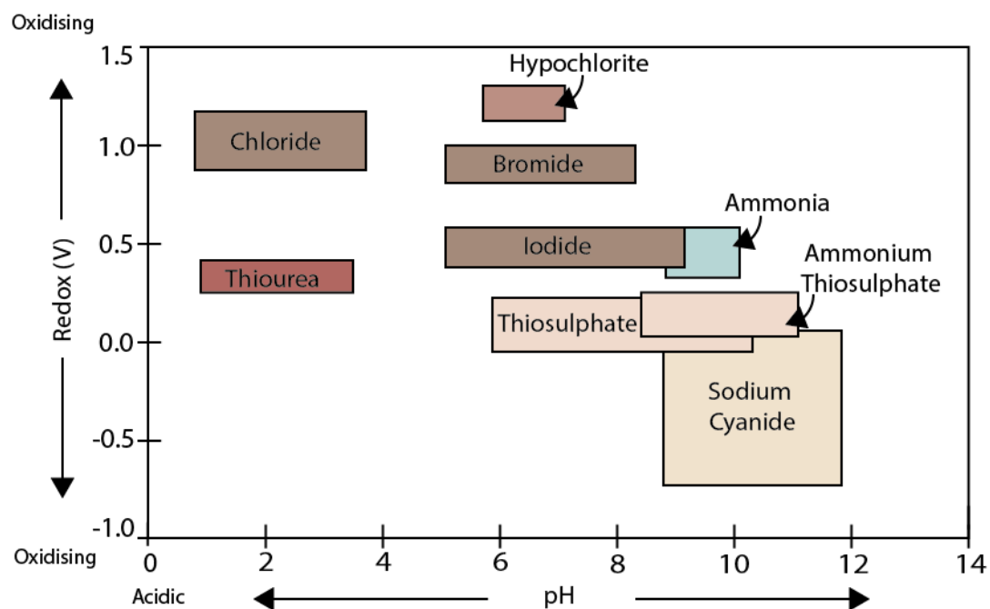
Figure 1-2 Stability fields (Redox and pH) of several gold lixiviants (After Aylmore, 2016a). Note that the sodium cyanide operating conditions are significantly larger than for any alternative lixiviant. Alternative lixiviants of interest to this study is the hypochlorite, thiourea and thiosulphate.
