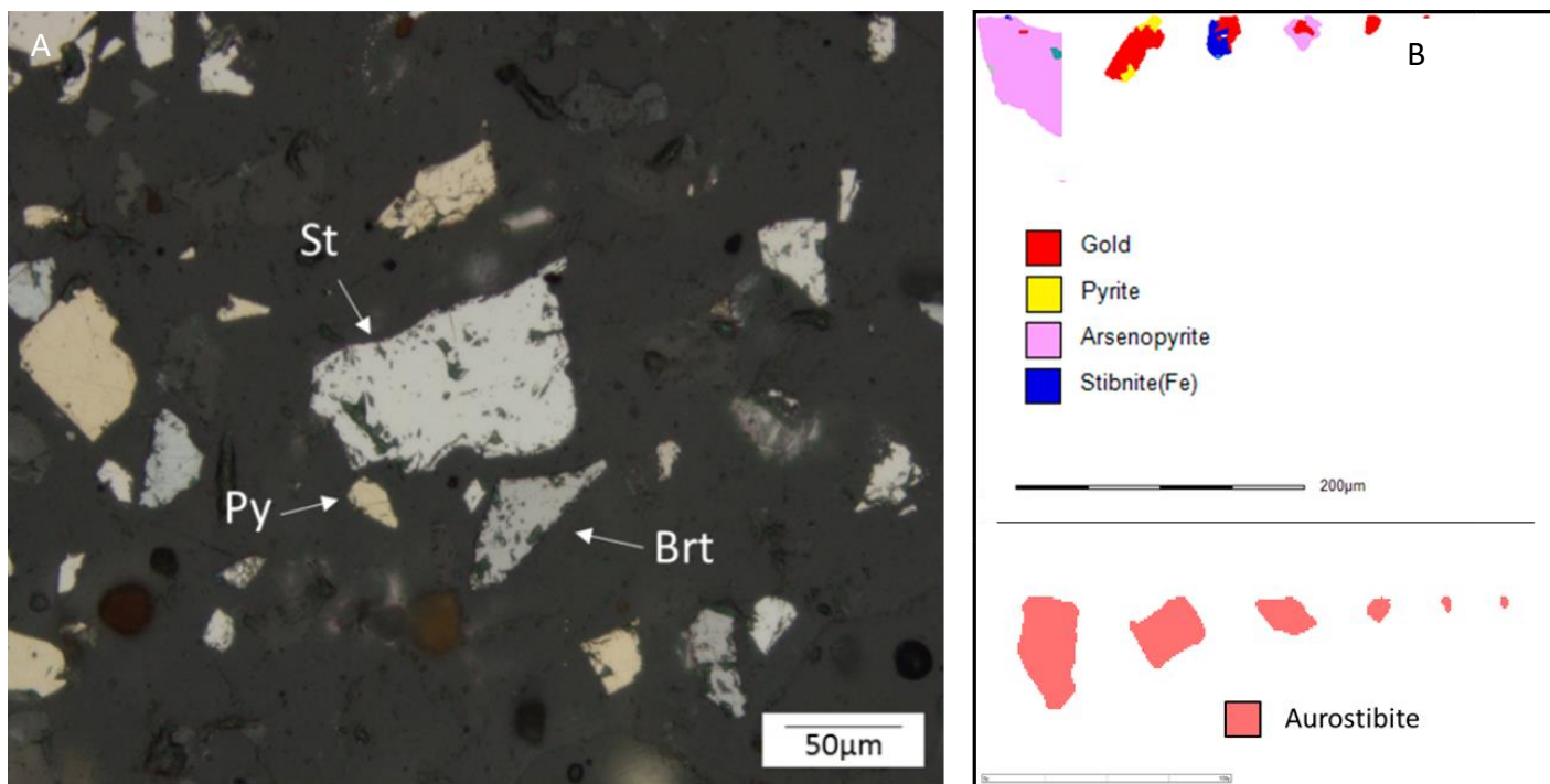
FIGURE 7 Mineralisation at Consolidated Murchison A) An example of mineralisation that includes stibnite (St), pyrite (Py), and berthierite (Brt). B) Gold and aurostibite grains, highlighting the lower degree of liberation in native gold, while aurostibite grains have excellent liberation and exposure.
