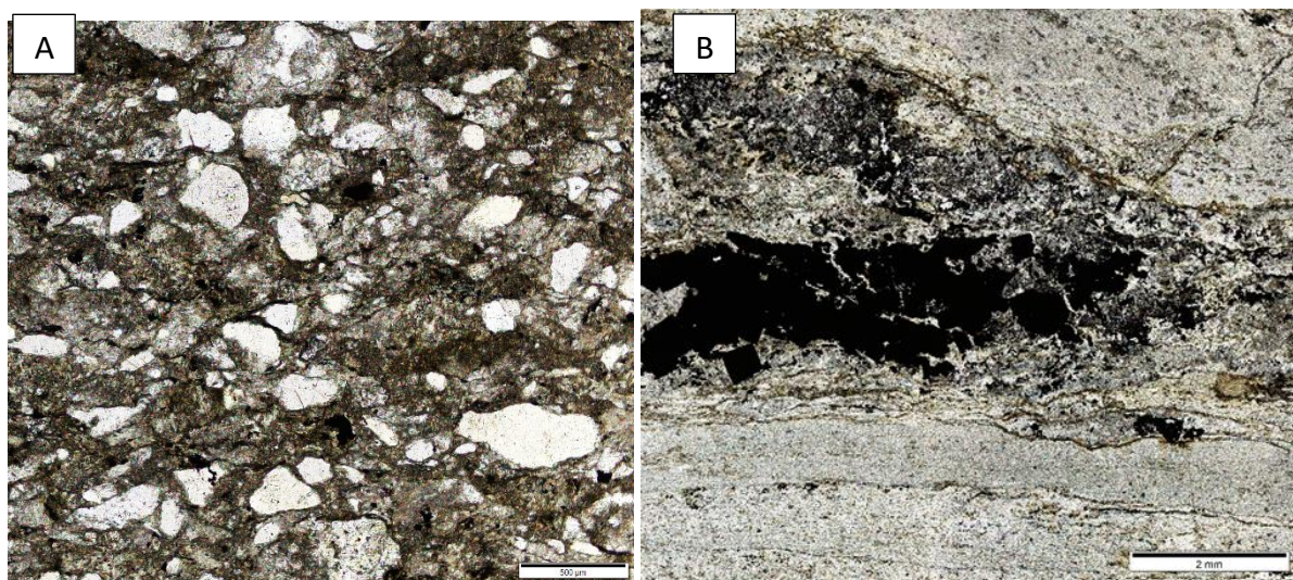
Figure 4-4 Transmitted light (PPL) images of Fairview material. A) Lithic quartz fragments with a fine-grained matrix of quartz, chlorite, dolomite, magnesite and to a lesser extent muscovite. B) Quartz and calcite vein crosscutting the fine grained micaceous schist. Subhedral to euhedral pyrite occurs within the vein (evident in transmitted light as the black mineral).
