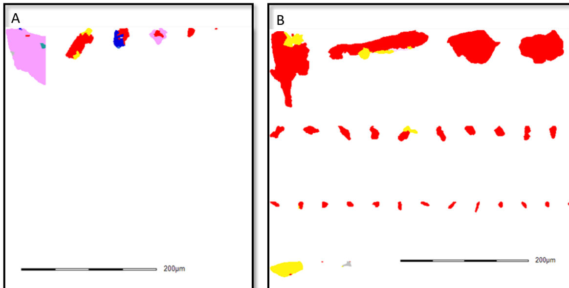
Figure 6 A) Consolidated Murchison gold grains, highlighting the lower degree of liberation. B) Pilgrim's Rest gold grains, highlighting the range in size, excellent liberation and exposure.
