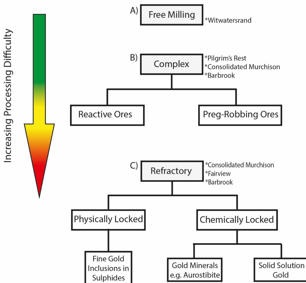
FIGURE 2 A diagram outlining the three main types of gold deposit types; 1) Free Milling, 2) Complex and 3) Refractory (in increasing order of processing difficulty). While the deposits of study and their respective mineralogy will be outlined, the deposits have been grouped with their respective deposit types.
