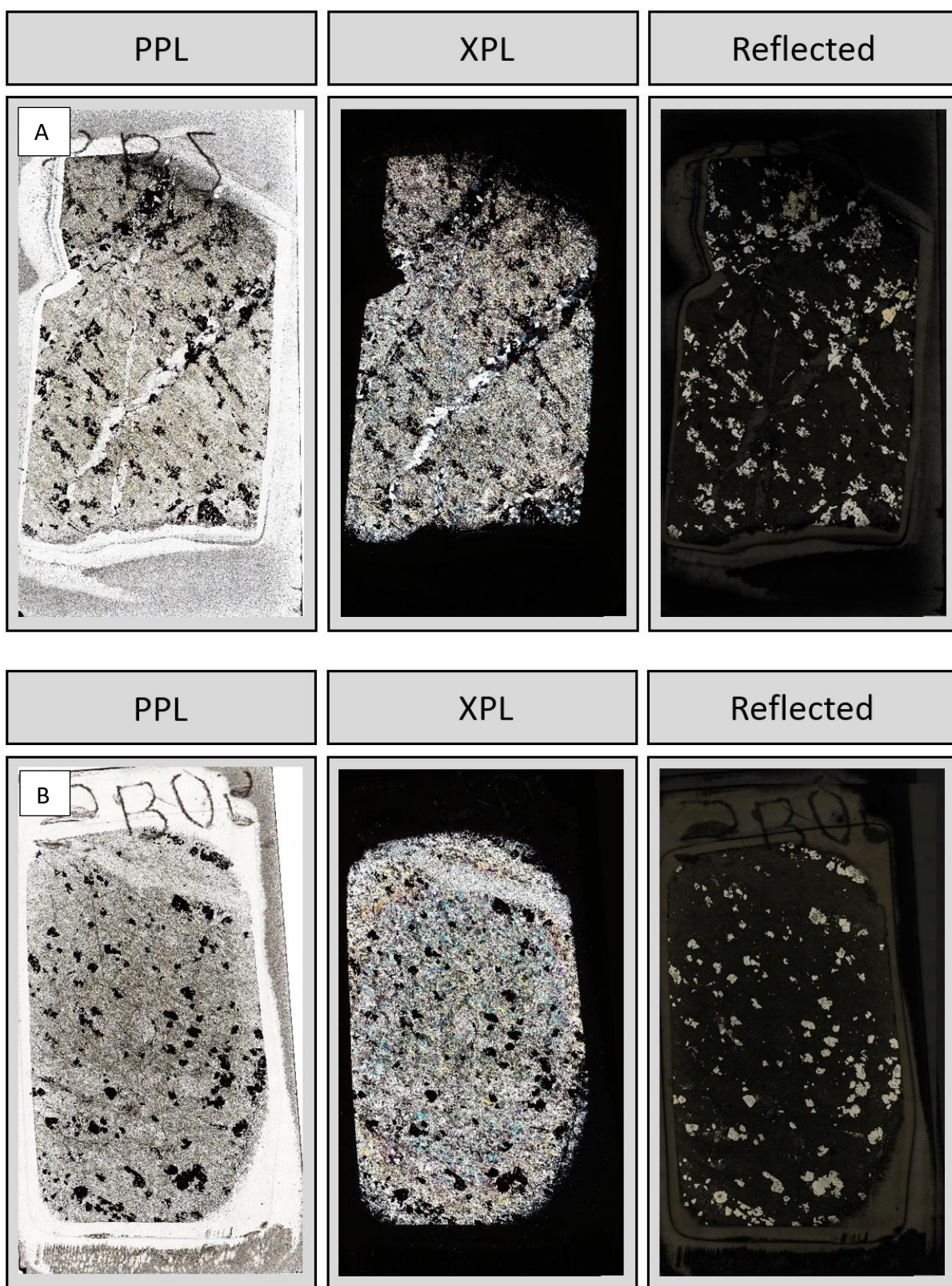
Figure 4-7 Transmitted (PPL and XPL) and reflected light images highlight the overall mineralogy and texture of Consolidated Murchison. A) Photomicrograph of the schist that is commonly host to the mineralisation B) Less prominent alignment of the micas found in this sample. The majority of the minerals comprising these samples cannot be determined at an overview scale due to its fine-grained nature. Pyrite is visible in reflected light, distributed homogeneously across much of the sample.
