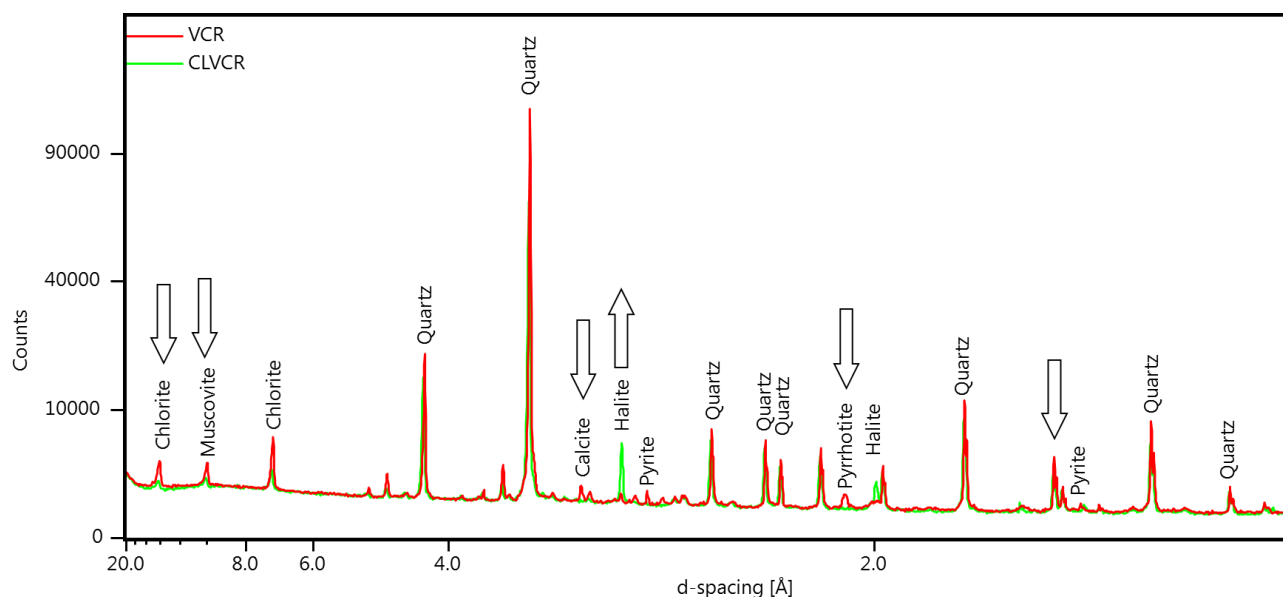
Figure 10-1 XRD pattern for the Ventersdorp Contact Reef (VCR) feed (red) and residue (green) overlain to highlight mineralogical differences after chloride-hypochlorite leaching. The arrows represent the increasing or decreasing abundance from feed to residue. Consumption of chlorite, calcite, pyrrhotite and pyrite is evident.
