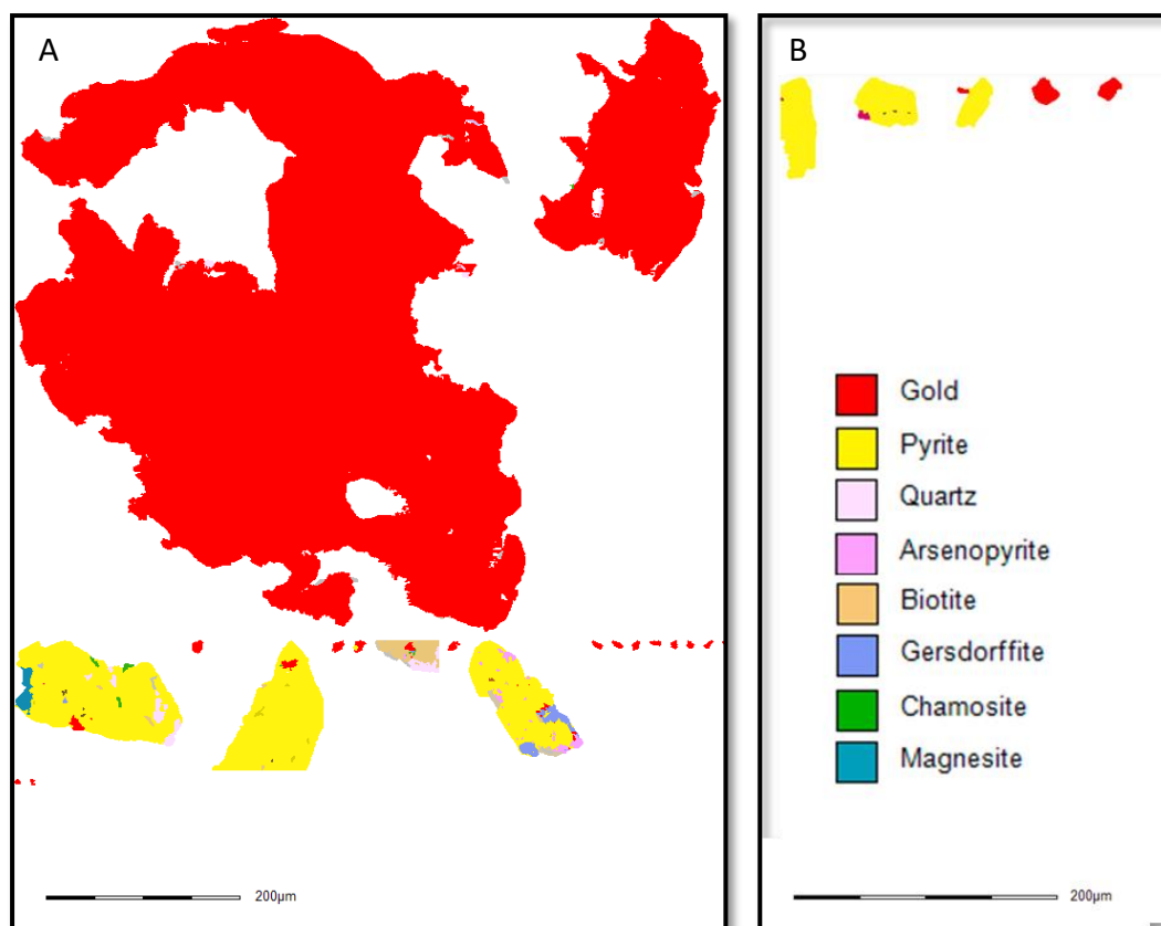
Figure 6-4 False colour MLA images from the Barberton samples (Fairview and Barbrook) A) An example of the vast range in sizes of gold grains in the Fairview sample, from 0.5 \mu\text{m} to 425 \mu\text{m} . B) The Barbrook sample gold grains, with pyrite association represented. The Barbrook sample gold grains ranged in size from 1 \mu\text{m} to 53 \mu\text{m} .
