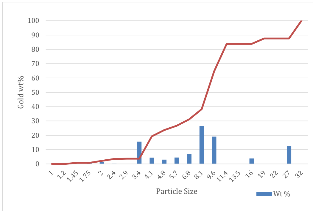
Figure 6-6 Graph representing the native gold grain size distribution for the Consolidated Murchison sample, with a bar graph representing weight percent contribution from certain size fractions, and a line graph representing cumulative weight percent. The native gold had a limited grain size distribution from 2 \mu\text{m} to 27 \mu\text{m} with much of the gold occurring predominantly in the range from 3-10 \mu\text{m} .
