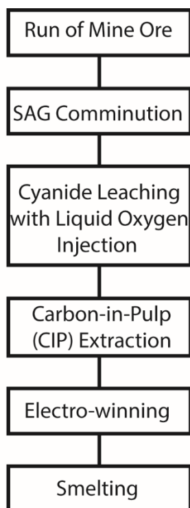
Figure 2-5 Processing flowchart for Mponeng Mine, important steps in this processing include cyanide leaching with Liquid Oxygen Injections and Carbon-in-Pulp extraction. .
