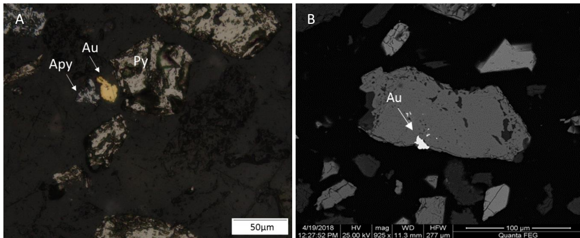
Figure 2 A) Example of the mineralisation found in Fairview, including arsenopyrite (Apy), pyrite (Py) and gold (Au). The gold grain has an equivalent circular diameter (ECD) of 46.5 μm. B) Example of a gold grain at Fairview (BSE), with limited liberation due to association with pyrite, but good exposure and an ECD of 10.7 μm.
