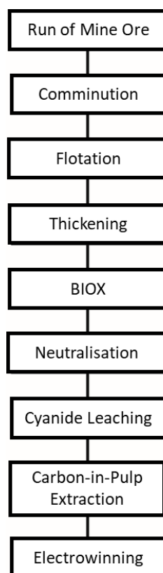
Figure 2-8 Processing flowchart for Fairview mine, in which it is evident that flotation, thickening and BIOX processes are implemented before cyanide leaching and carbon in pulp extraction.
