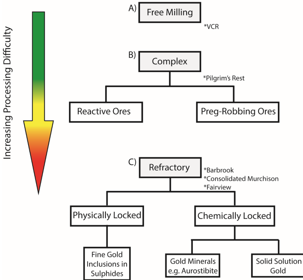
Figure 1-1 Three main types of gold deposit types exist, based on their response to recovery; 1) Free Milling, 2) Complex and 3) Refractory. While the deposits of study and their respective mineralogy will be outlined in subsequent chapters, the deposits have been grouped with their respective deposit types. Ventersdorp Contact Reef is free milling, Pilgrim's Rest is complex, Barbrook is refractory but also contains a complex component, Fairview and Consolidated Murchison are both refractory.
