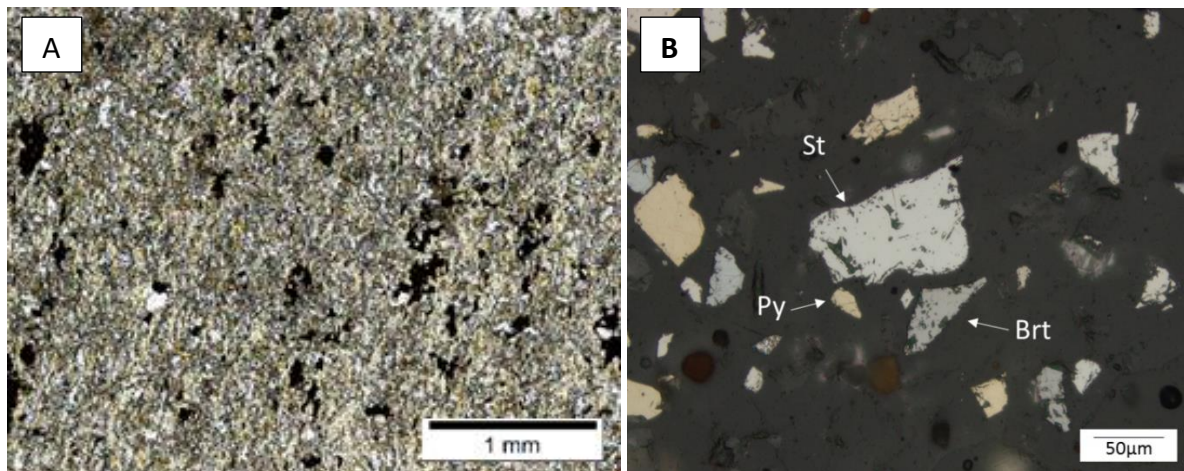
Figure 4-8 Microphotographs of typical components of the Consolidated Murchison sample. A) Fine grained quartz carbonate schist, with chlorite, biotite and magnesite. B) An example of mineralisation at Consolidated Murchison including stibnite (St), pyrite (Py) and berthierite (Brt).
