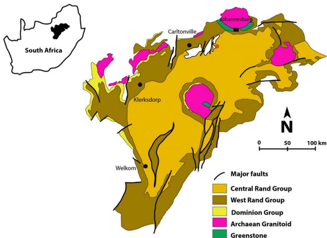
Figure 2-3 Schematic geological map of the Witwatersrand Basin (Mngadi et al., 2019). The Mponeng gold mine is the source of the Ventersdorp Contact Reef sample for study. The Mponeng mine is found within the Carletonville Goldfield, and the precise locality of the mine marked in red.
