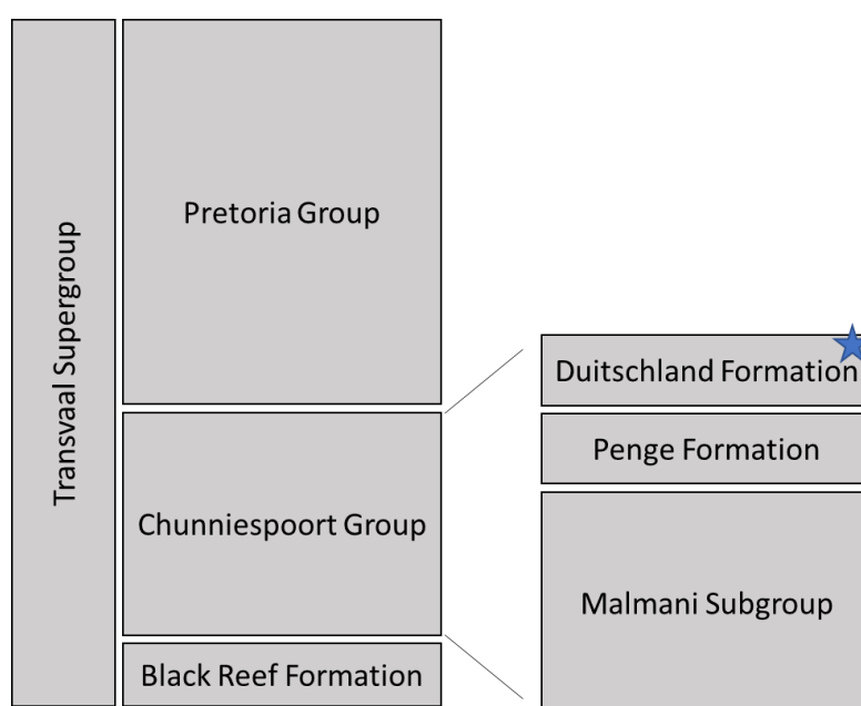
Figure 2-11 A portion of the stratigraphic sequence of the Transvaal Supergroup, is host to the Chuniespoort Group and subsequently the Duitschland Formation. Pilgrim's Rest mineralisation occurs within the Duitschland Formation (demarcated with a blue star). This stratigraphic sequence is based on Tyler and Tyler, (1996).
