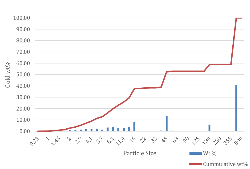
Figure 6-3 Graph representing the gold grain size distribution for the Fairview sample, with a bar graph representing weight percent contribution from certain size fractions, and a line graph representing cumulative weight percent. The gold in the Fairview sample had a large range in grain sizes, from 0.5 \mu\text{m} to 425 \mu\text{m} . There were inconsistencies in distribution due to the absence of gold grains between sizes of 16 \mu\text{m} and 45 \mu\text{m} , between 45 \mu\text{m} and 180 \mu\text{m} , and 180 \mu\text{m} and 355 \mu\text{m} .
