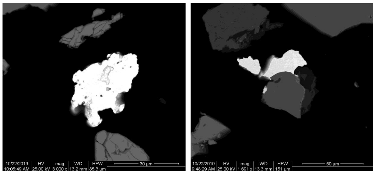
Figure 10-9 BSE images of gold (white) found in calcined, thiosulphate glycine leach of the Ventersdorp Contact Reef residue. The compact nature of the gold, along with the embayments along the margins would suggest that these grains underwent incomplete dissolution.
