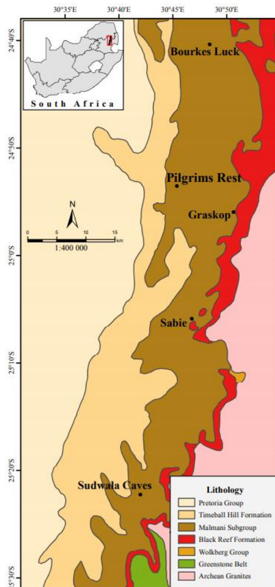
Figure 2-10 Schematic geological map of the Sabie-Pilgrim's Rest region, host to the Pilgrim's Rest gold deposit. Map produced from Jaguin et al., (2012).
