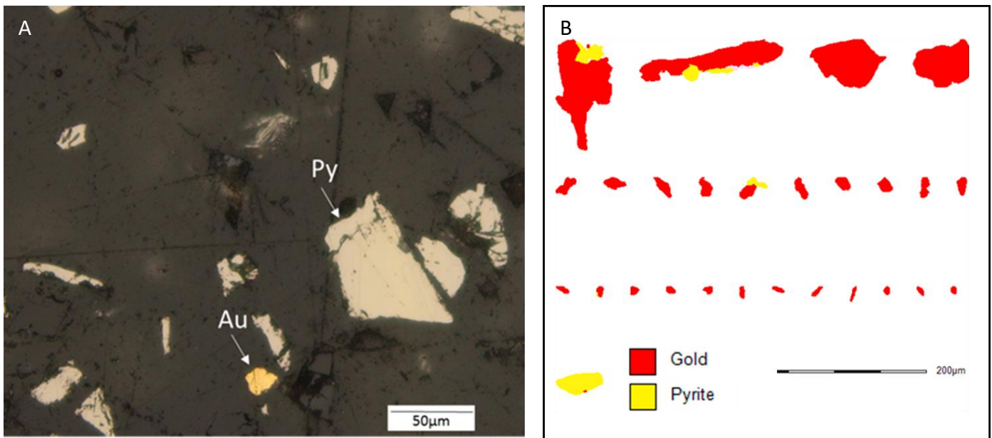
FIG 8 Pilgrim's Rest mineralisation A) A gold grain with an equivalent circular diameter of 16 \mu\text{m} . Significant pyrite mineralisation is also evident. B) MLA images of Pilgrim's Rest gold grains, highlighting the range in size, and excellent liberation and exposure.
