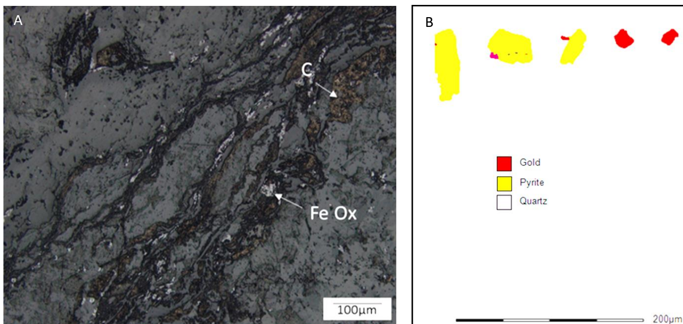
FIGURE 6 Features of interest from Barbrook ore A) Example of carbon associated with various iron oxides. B) Barbrook gold grains, with pyrite and minor quartz association represented.
