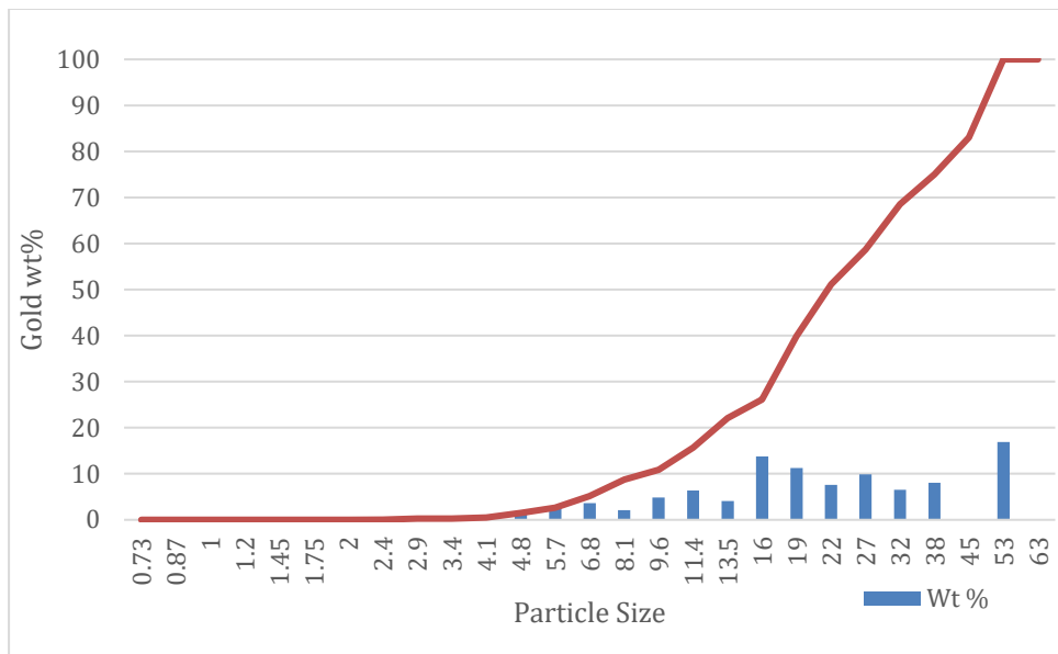
Figure 6-8 Graph representing the aurostibite grain size distribution for Consolidated Murchison, with a bar graph representing weight percent contribution from certain size fractions, and a line graph representing cumulative weight percent. Aurostibite grains tended to be significantly larger than the native gold grains, with a range in size from 0.73 \mu\text{m} to 53 \mu\text{m}
