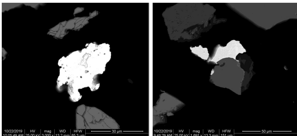
Figure 2 BSE images of gold remaining in the residue of the calcined, thiosulfate glycine leached material with embayments suggesting incomplete dissolution.
