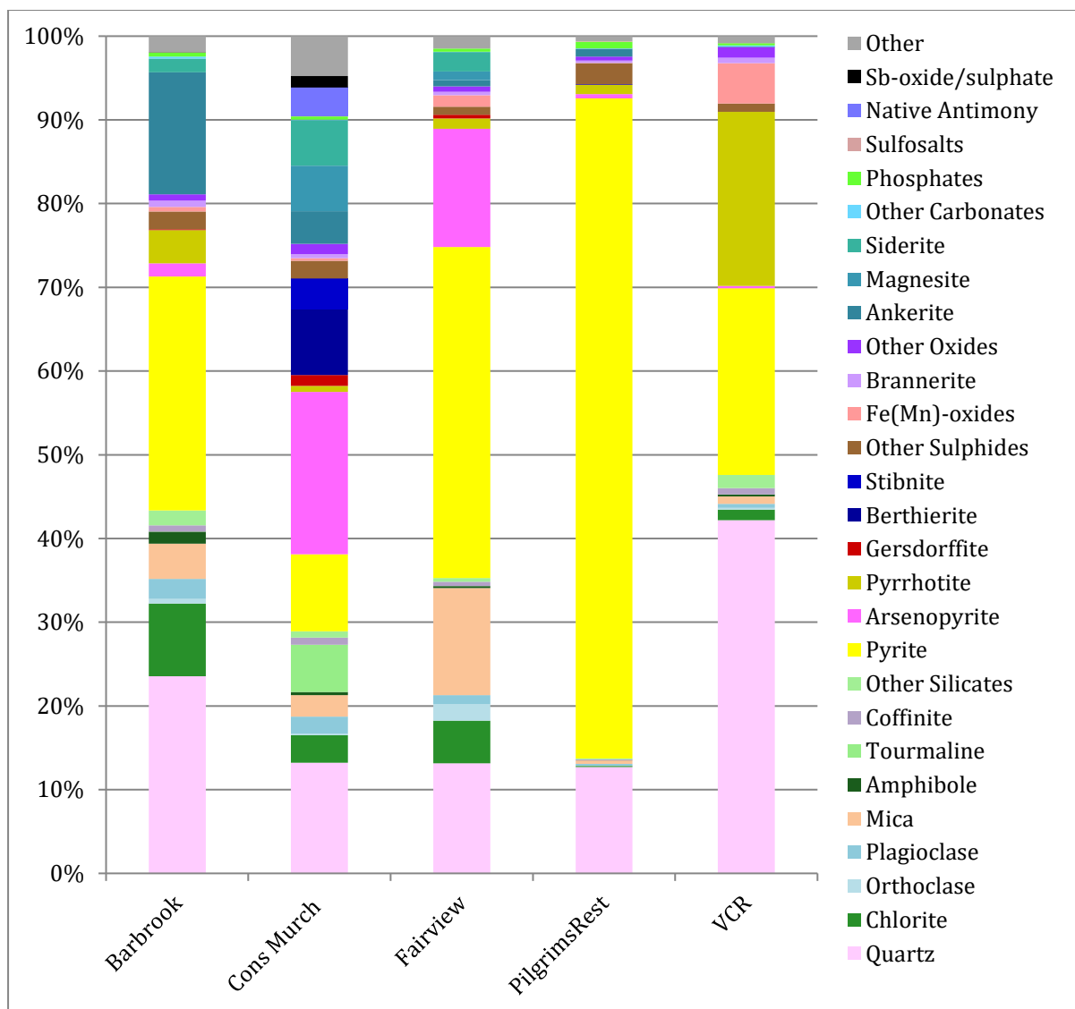
Figure 6-15 Normalised modal mineralogy summarised for the ore deposits of interest. All the samples have abundant quartz and to a lesser extent pyrite. With the exception of Pilgrim's Rest, all samples also have feldspars, chlorite and mica.
