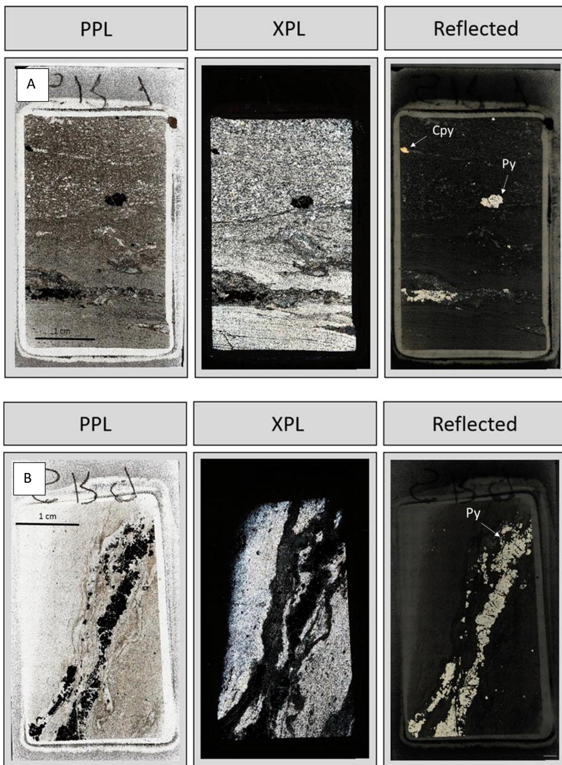
Figure 4-3 Transmitted (PPL and XPL) and reflected light images highlight the overall mineralogy and texture of the Fairview sample. A) The PPL and XPL images depict a matrix of quartz, chlorite, and dolomite. Individual minerals grains were typically not differentiable at low magnification. B) Veins are common in Fairview and are predominantly quartz with minor calcite. The reflected light image highlights the pyrite (py) found in veins and fractures.
