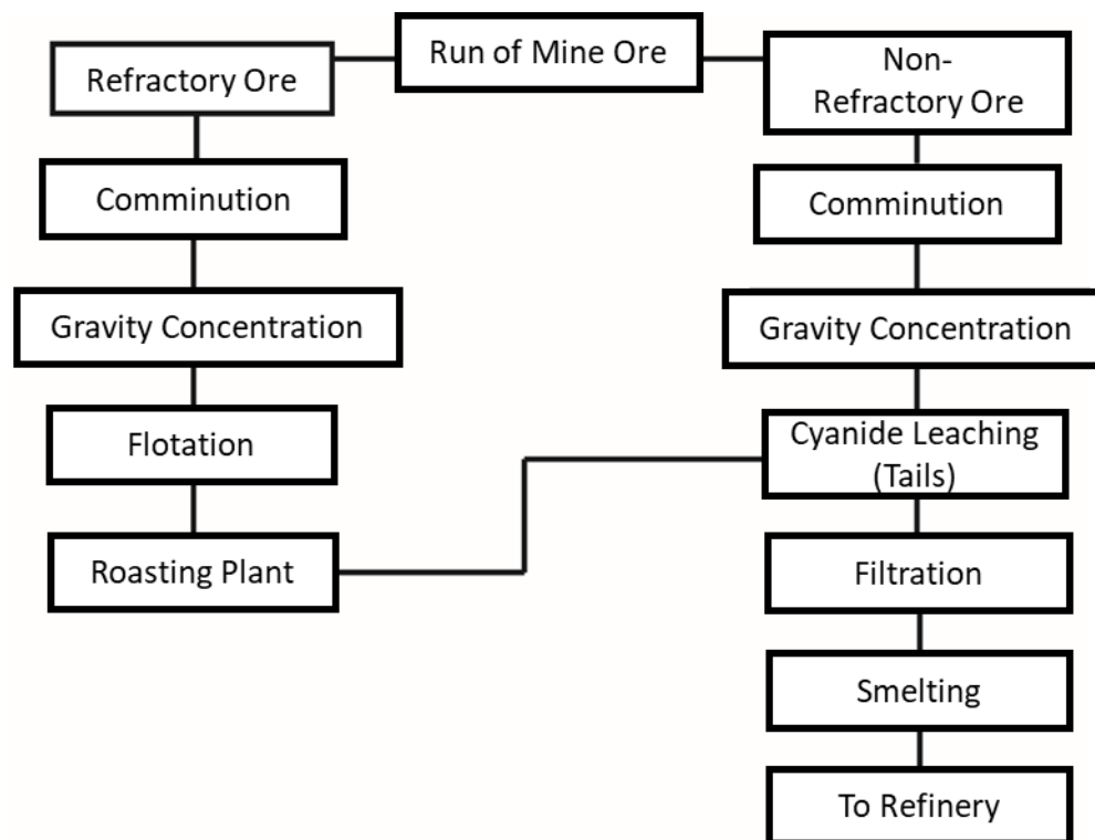
Figure 2-12 Processing flow chart for Pilgrim's Rest, a simplified diagram from 7th Commonwealth Mining and Metallurgical Congress, (1961). Discrete processes were applied for the two ore types, refractory and non-refractory.
