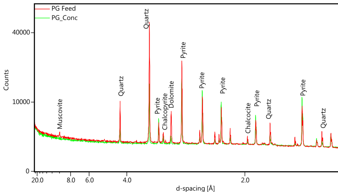
Figure 5-5 – X-Ray diffractograms for Consolidated Murchison feed (red) and gravity concentrate (green). There is a significant increase in the amount of pyrite present in the concentrate relative to the feed.
