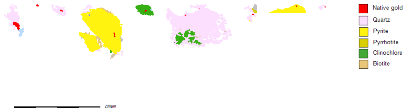
False colour images of gold found in leach residue
