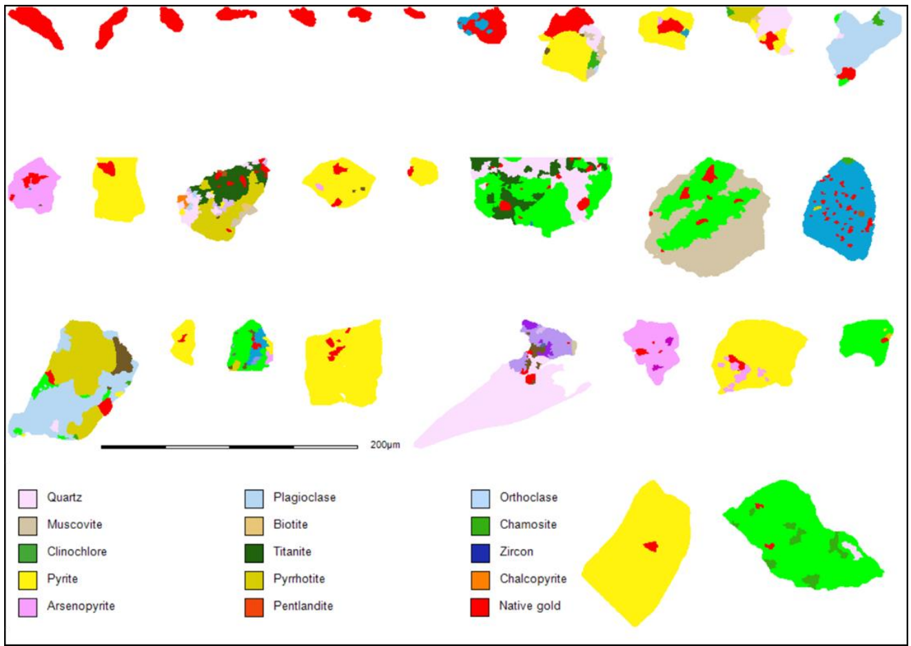
Figure 10-7 False colour images from MLA of gold grains (red) and their associated minerals found in the Ventersdorp Contact Reef thiosulphate glycine residue. This image emphasises the number of fine grained (less than of 27 µm equivalent circular diameter) gold particles in the residue.
