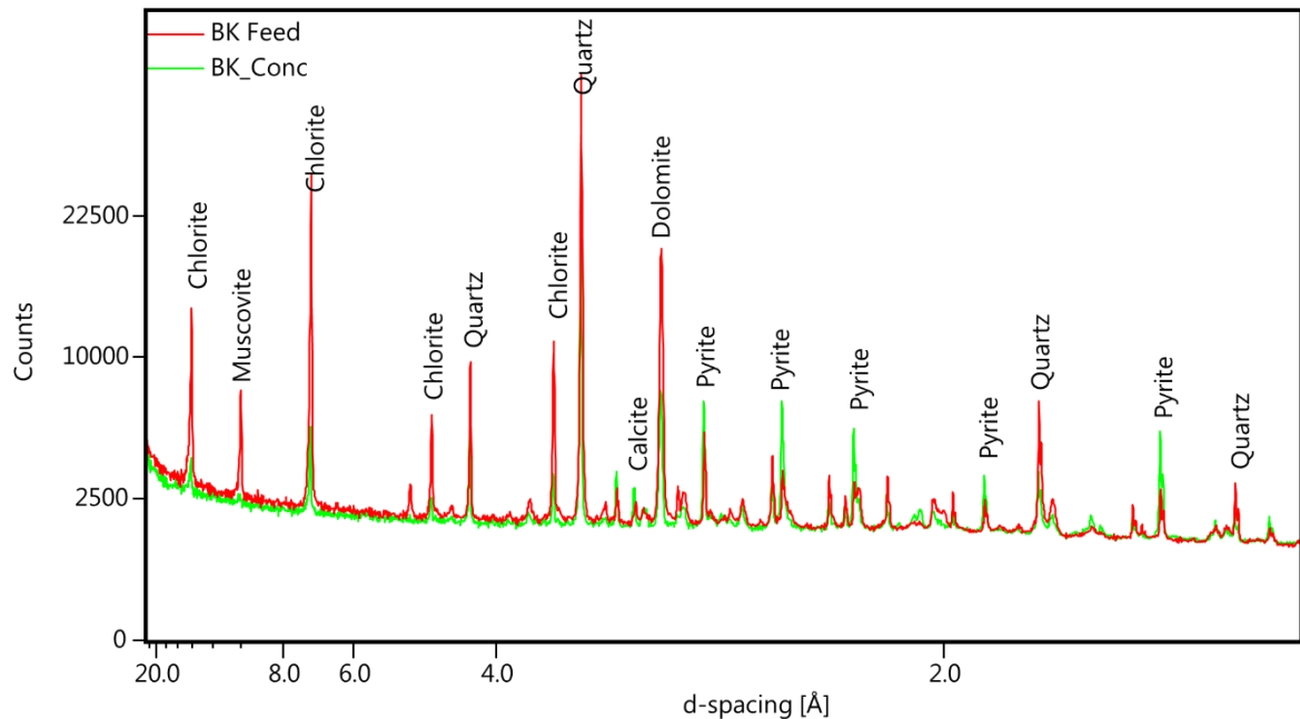
Figure 5-3 X-Ray diffractograms for Barbrook feed (red) and gravity concentrate (green). The amount of pyrite present has increased from the feed to the concentrate.
