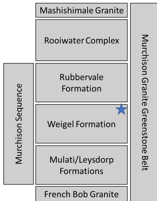
Figure 2-14 The stratigraphy of the Murchison Greenstone Belt, with the Weigel Formation, host to the Antimony Line and the Monarch deposit from which the studied samples were obtained. This column is based on the work in Poujol, (2001).
