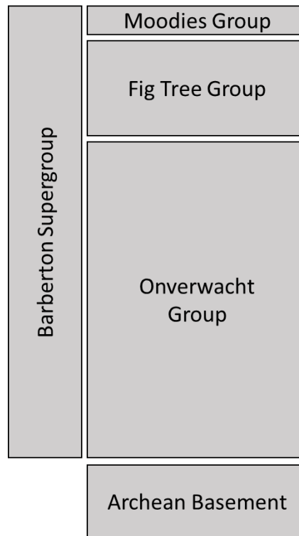
Figure 2-7 The stratigraphic sequence found in the Barberton Supergroup, with the Onverwacht, Fig Tree and Moodies Groups all of which are host to mineralisation in the Fairview locality. The Fig Tree Group is exclusively host to mineralisation in the Barbrook locality. The stratigraphic column was compiled from Lowe and Byerly, (2007).
