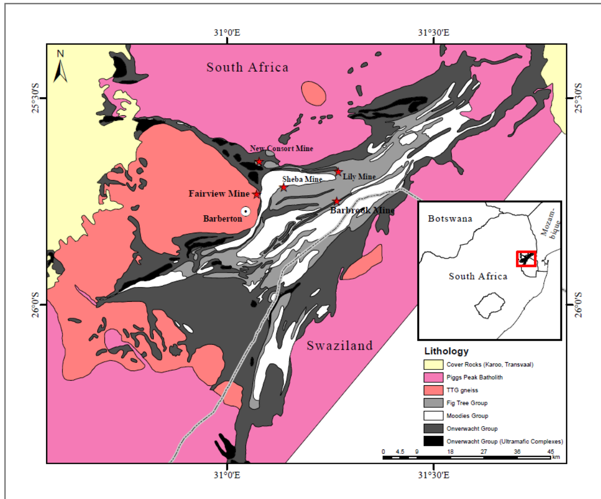
Figure 2-6 The geology of the Barberton Greenstone Belt with both Fairview and Barbrook mines marked in red (after Dirks et al., 2013).
