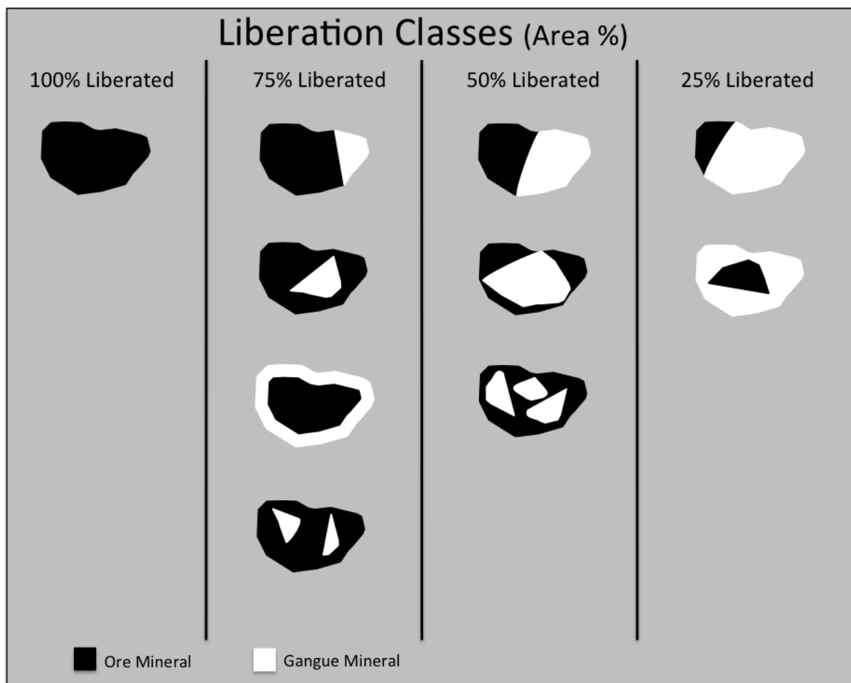
Figure 6-11 The range of liberation classes, e.g. 100% liberated, where the ore mineral is 100% of the area of the particle containing the ore mineral to 25% liberation, where the gold only comprises 25% of the area of the host particle (Crop, 2013).
