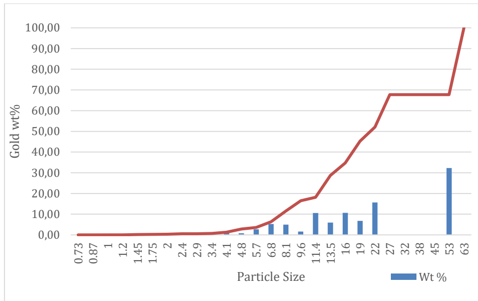
Figure 6-5 Graph representing the gold grain size distribution for the Barbrook sample, with a bar graph representing weight percent contribution from certain size fractions, and a line graph representing cumulative weight percent. The gold grains ranged in size from 1 \mu\text{m} to 22 \mu\text{m} , with a single exception of one larger grain at 53 \mu\text{m} .
