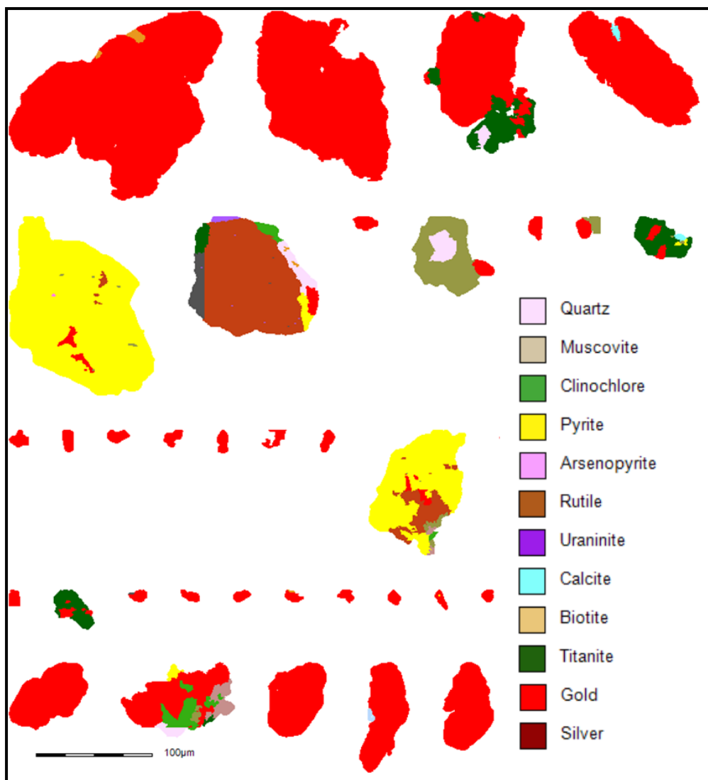
Figure 6-2 False colour images from the MLA of gold found in the Ventersdorp Contact Reef sample. This image highlights the range in grain size of gold from 0.5 \mu\text{m} to 425 \mu\text{m} , with the majority of gold weight percent occurring in the coarser grained fraction (200 -425 \mu\text{m} ).
