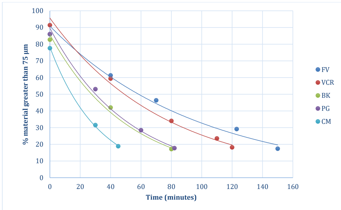
Figure 3-2 Milling curves produced for the milling masses of Ventersdorp Contact Reef (VCR), Fairview (FV), Barbrook (BK), Pilgrim's Rest (PG), and Consolidated Murchison (CM). Each curve shows an initially rapid decrease in grain size (evident in a steep gradient) before a moderate tapering out (a more shallow gradient) of grain size reduction.
