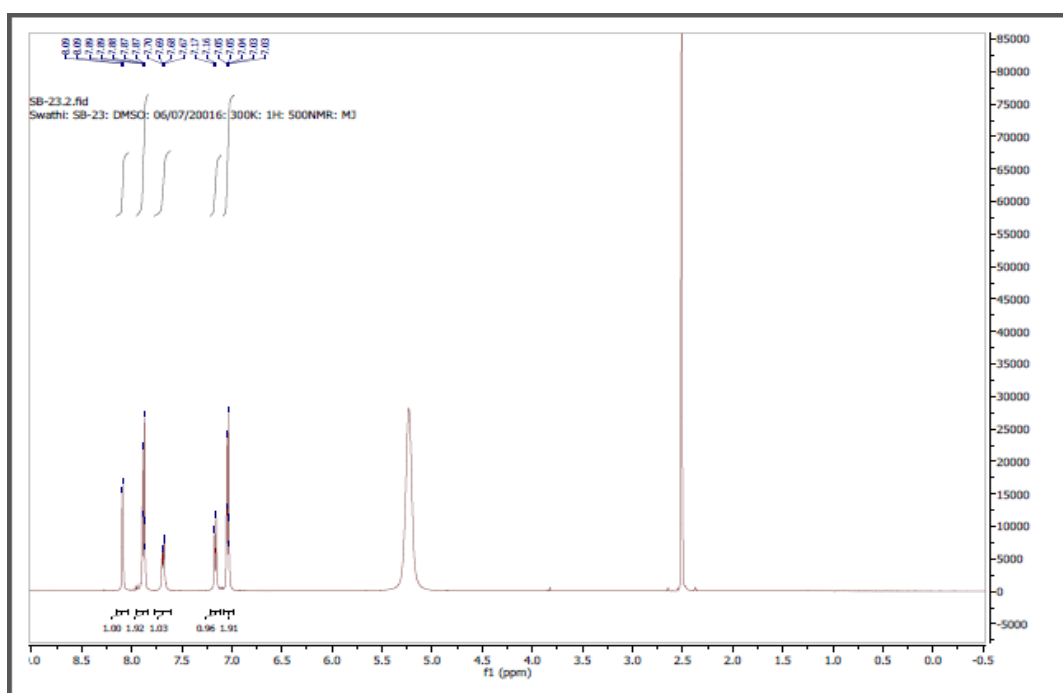
Figure C3 (d): ^1\text{H} NMR Spectra of SPPSU at 20°C
