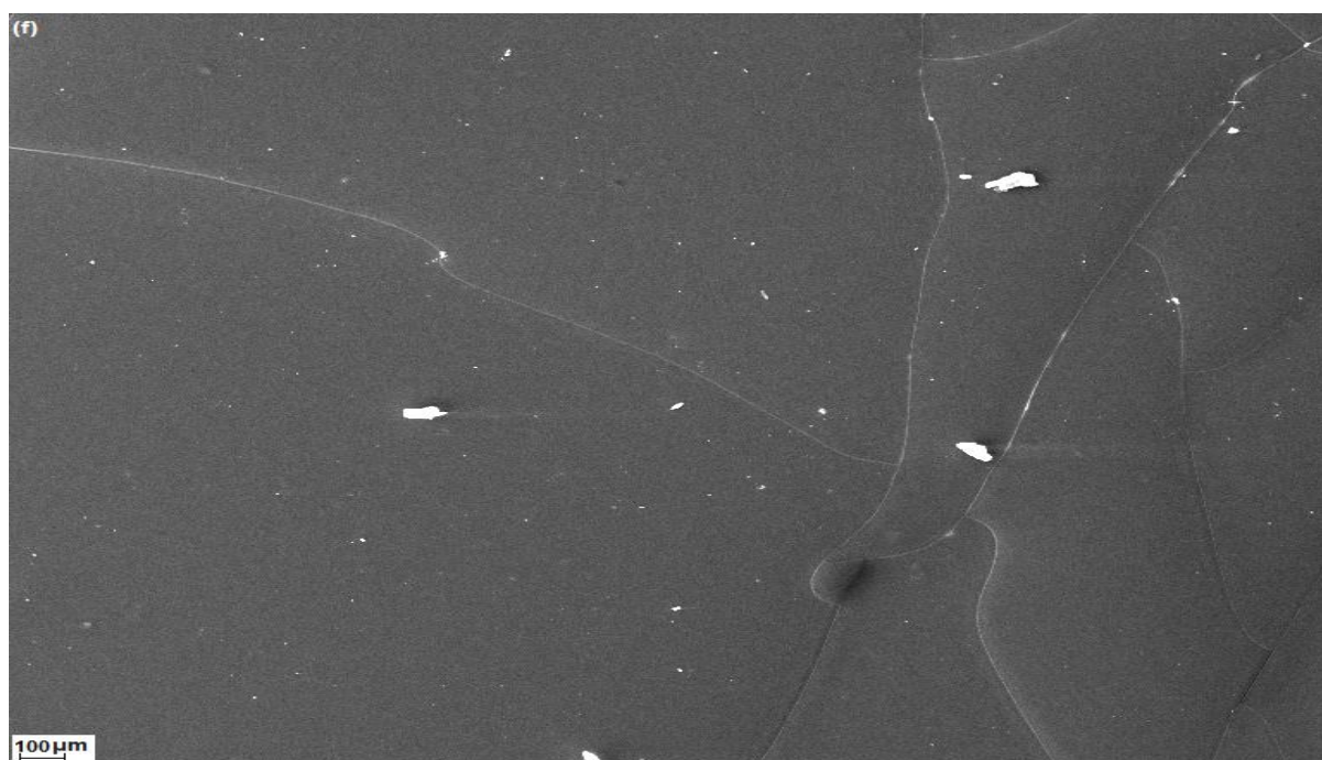
Figure 4.9 C: SEM images (e) 1 wt% CNB loaded IEM at 75% sonication amplitude (f) 4 wt% CNB loaded IEM at 75% sonication amplitude
