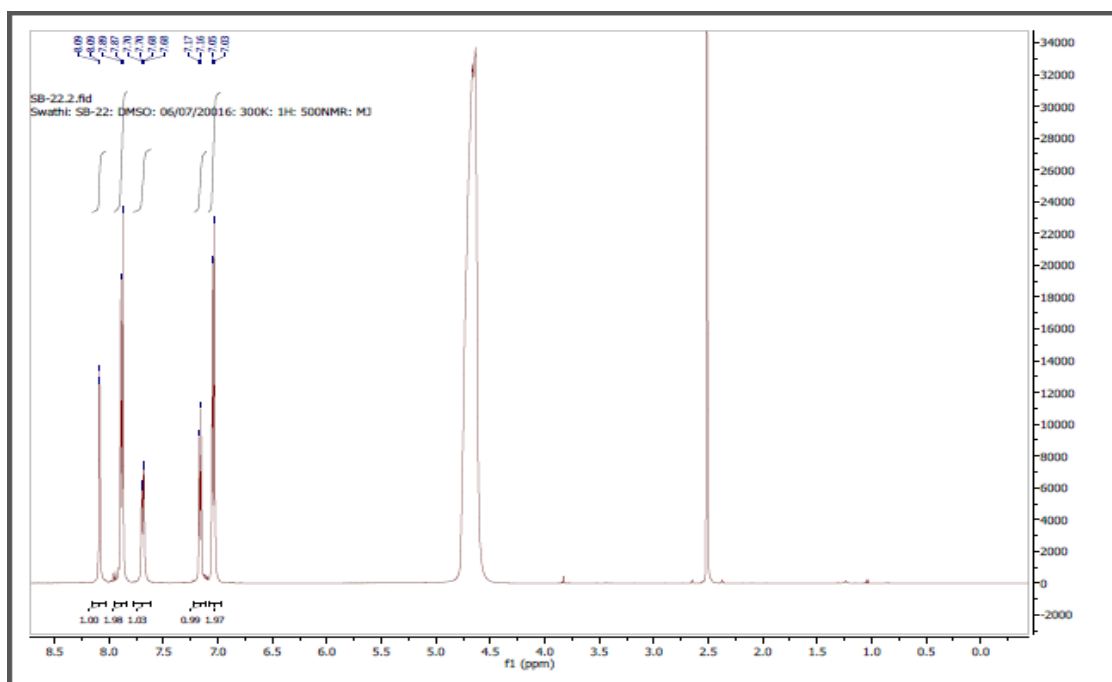
Figure C3 (a): ^1\text{H} NMR Spectra of SPPSU at -10^\circ\text{C}
