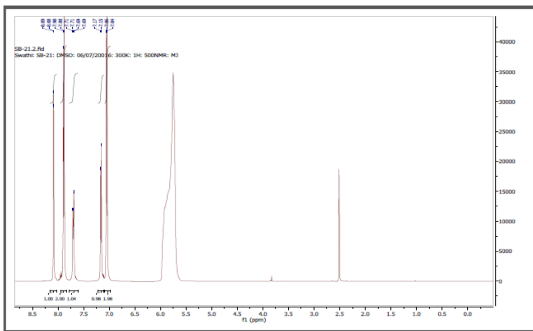
Figure C3 (c): ^1\text{H} NMR Spectra of SPPSU at 10°C
