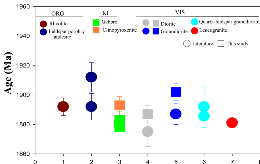
Figure 12. Compilation of ages for the Orange River Group (ORG), Kokerboom Intrusion (KI) and Vioolsdrif Intrusive Suite (VIS). The data for the ORG and VIS are taken from Meng et al. (2020).
