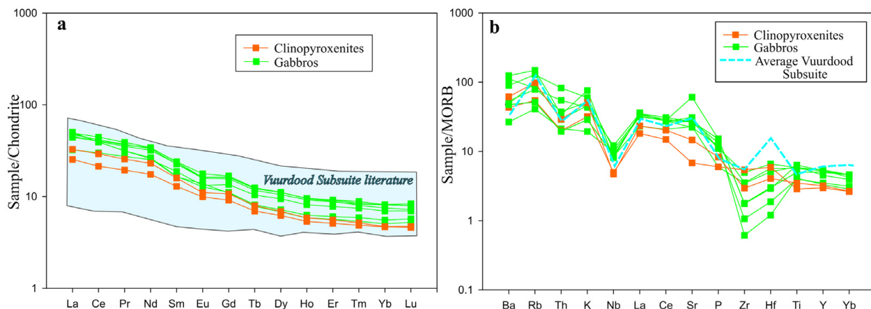
Figure 9. (a) Chondrite-normalised (Anders and Grevesse, 1988) REE patterns for the various rock types of the mafic-ultramafic intrusion: clinopyroxenites have relatively flat patterns, whereas the gabbros show LREE enrichment and minor Eu anomalies, both rock types have very similar patterns, Eu anomalies are identical within uncertainties. (b) Mid ocean ridge basalt (MORB)-normalised (White, 2005) multi-element patterns for the various rock types constituting the mafic-ultramafic intrusion and the average Vuurdood Subsuite. The MORB-normalised multi-element patterns for the mafic-ultramafic intrusion and average Vuurdood Subsuite overlap.
