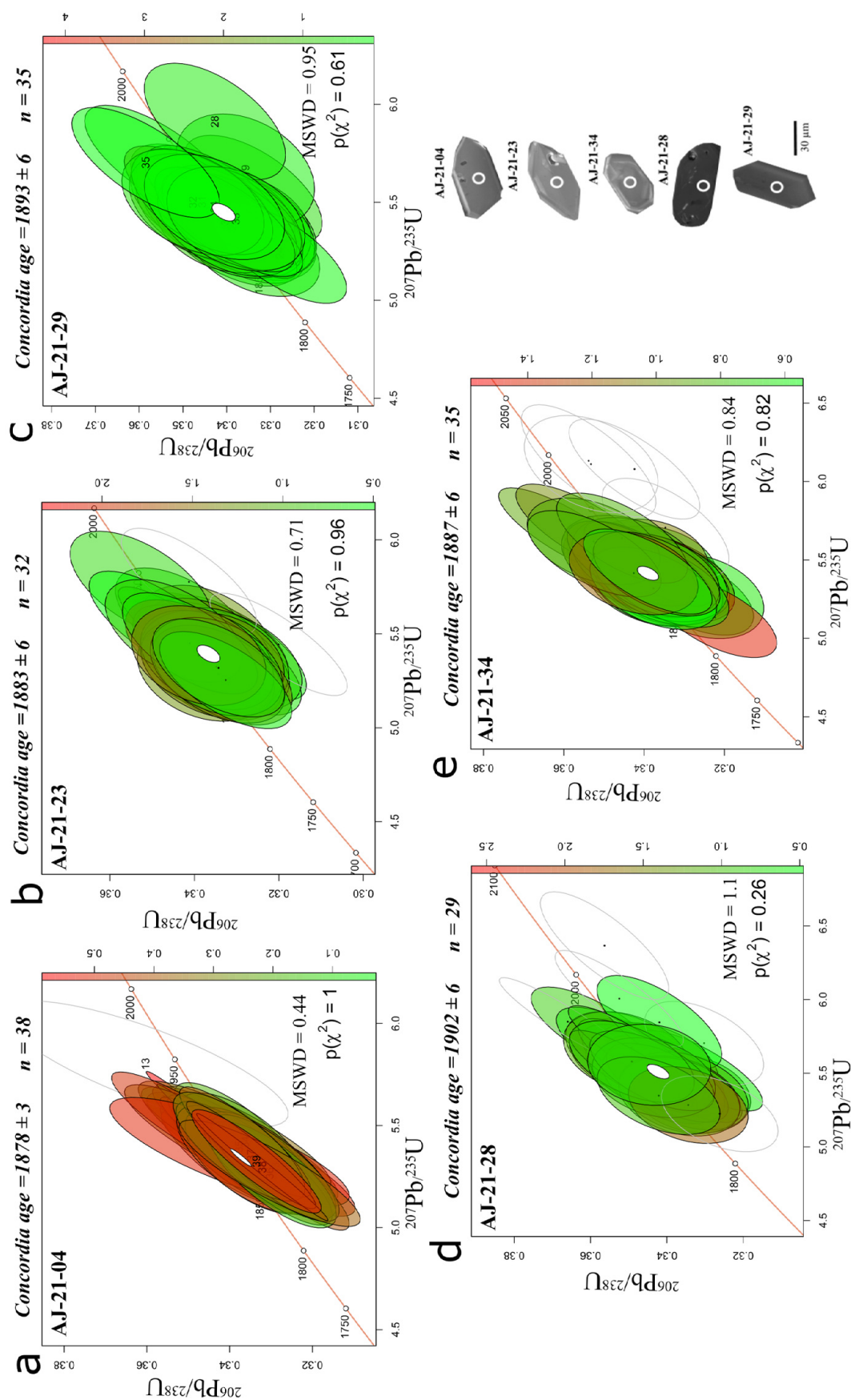
Figure 11. Wetherill Concordia diagrams illustrating the results from the U-Pb geochronological analyses. The red colours on the diagram indicate discordance and the green colours indicate concordance. Uncertainties on individual isotope ratios are 2\sigma (standard error; absolute). The circles indicate laser ablation spots. (a) 38 analyses on zircons from the gabbro sample (AJ-21-04) provide a concordia age of 1878 \pm 3 Ma. (b) 32 analyses on zircons from the additional gabbro sample (AJ-21-23) yielded a concordia age of 1883 \pm 6 Ma. (c) 35 analyses on zircons from the clinopyroxenite sample (AJ-21-29) yielded a concordia age of 1893 \pm 6 Ma. (d) 29 analyses on zircons from the granodiorite in contact with the gabbroic intrusion (AJ-21-28) provided a concordia age of 1902 \pm 6 Ma. (e) 35 analyses conducted on the diorite sample (AJ-21-34) yielded a concordia age of 1887 \pm 6 Ma. A full compilation of CL and BSE images can be found in the Supplementary Information 5.
