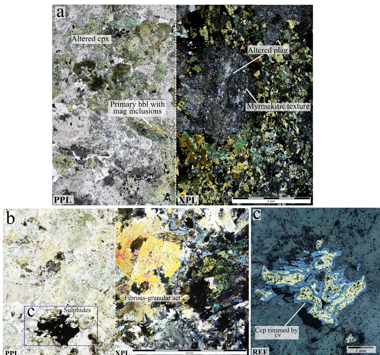
Figure 5. Plane polarised light (PPL) and cross polarised light (XPL) photomicrographs of gabbro (a), and clinopyroxenite (b) of the mafic-ultramafic intrusion. (a) Primary stubby prisms of clinopyroxene are altered to bornblende (bbl), chlorite and epidote whereas plagioclase is pervasively altered to sericite and epidote and displays a myrmekitic texture. (b) Sulphides in the clinopyroxenite. Fibrous-granular actinolite is evident. Primary clinopyroxene is altered to actinolite with minor chlorite and epidote and has inclusions of magnetite (mag). Opaque material is prevalent in the reflected (REF) light image. (c) Chalcopyrite (ccp) is being replaced by covellite (cv) and are rimmed by haematite-magnetite-ilmenite assemblages.
