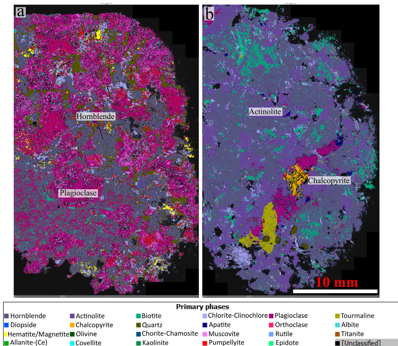
Figure 6. False-colour maps produced using the Tescan Automated Mineral Analyser (TIMA) of representative thin sections for the gabbros (a), and clinopyroxenites (b). Modal abundances of plagioclase decrease from the gabbros to clinopyroxenites. From the mineral liberation maps the non-cotectic proportions of dominant mineral phases are clear.
