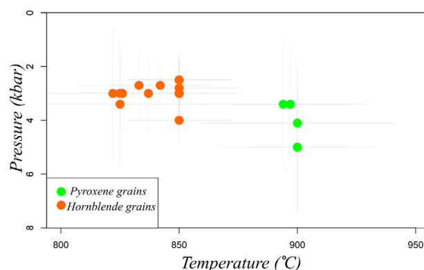
Figure 10. P-T graph showing the results from the machine learning geothermobarometry conducted on pyroxenes and hornblende grains from the Vuurdood Subsuite pyroxenites. Pressure and temperature, when including procedural uncertainty, ranges, from ~1.5 to 7 kbar and ~800 to 900°C, respectively.
