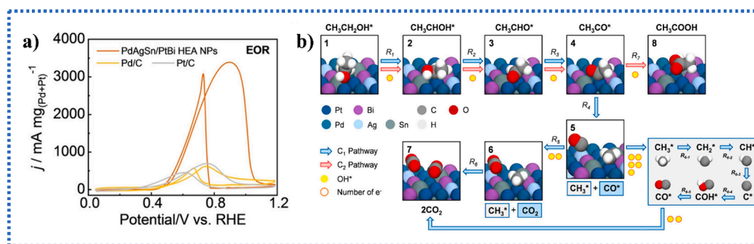
Fig. 3. a) CV polarization for EOR on PdAgSn/PtBi HEA Nps, Pd and Pt, b) DFT calculation: scheme of intermediate and major products involved in EOR, Reprinted with Ref. [86] Copyright (2023) Wiley-VCH GmbH.
