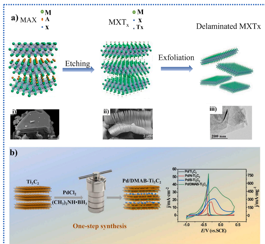
Fig. 9. a) Shows the synthesis of MXenes from a precursor MAX phase by etching using HF. Some layers are removed and replaced by surface terminals T x such as –O, –OH, and/or –F to form multilayered MXenes. Exfoliation of multilayered MXene into 2D flakes becomes possible through sonication or intercalation of cations and organic molecules. (i) SEM micrographs of bulk Mo 2 CT x flake, (ii) SEM micrograph of Ti 3 C 2 T x after etching, (iii) TEM image of Ti 3 C 2 T x flake after exfoliation. Image (i) and (7ii) adapted from Ref. [122], with permission from ACS Nano, Copyright (2012). TEM image (iii) of isolated Ti 3 C 2 T x adapted from Ref. [123], with permission from Elsevier Copyright (2019). b) One-step hydrothermal procedure for co-doping and reducing Pd to make Pd/DMAB-Ti 3 C 2 . Reprinted from Ref. [124], with permission from Elsevier. Copyright (2023).
