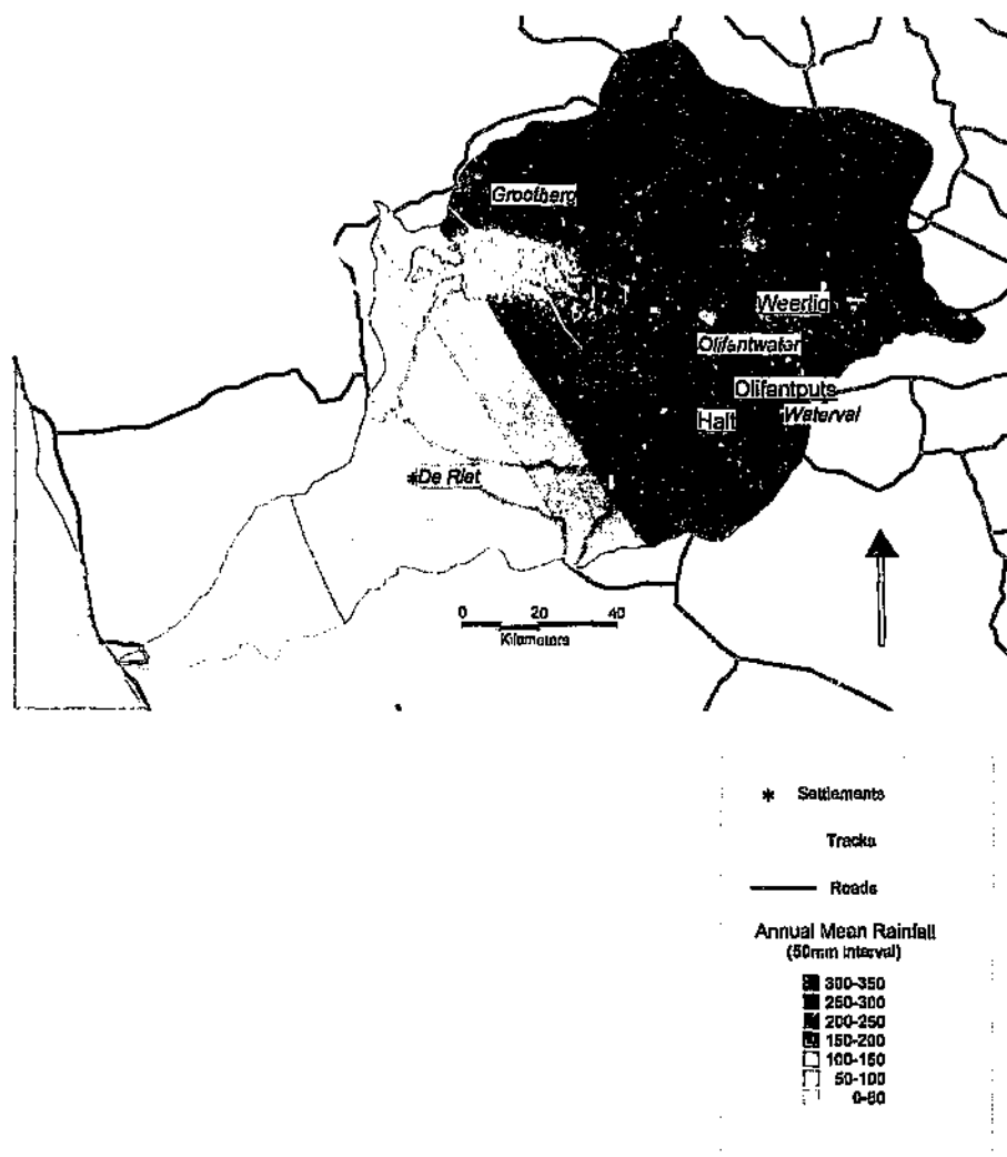
Figure 2.5: Huab Catchment - annual mean rainfall, interval 50mm
