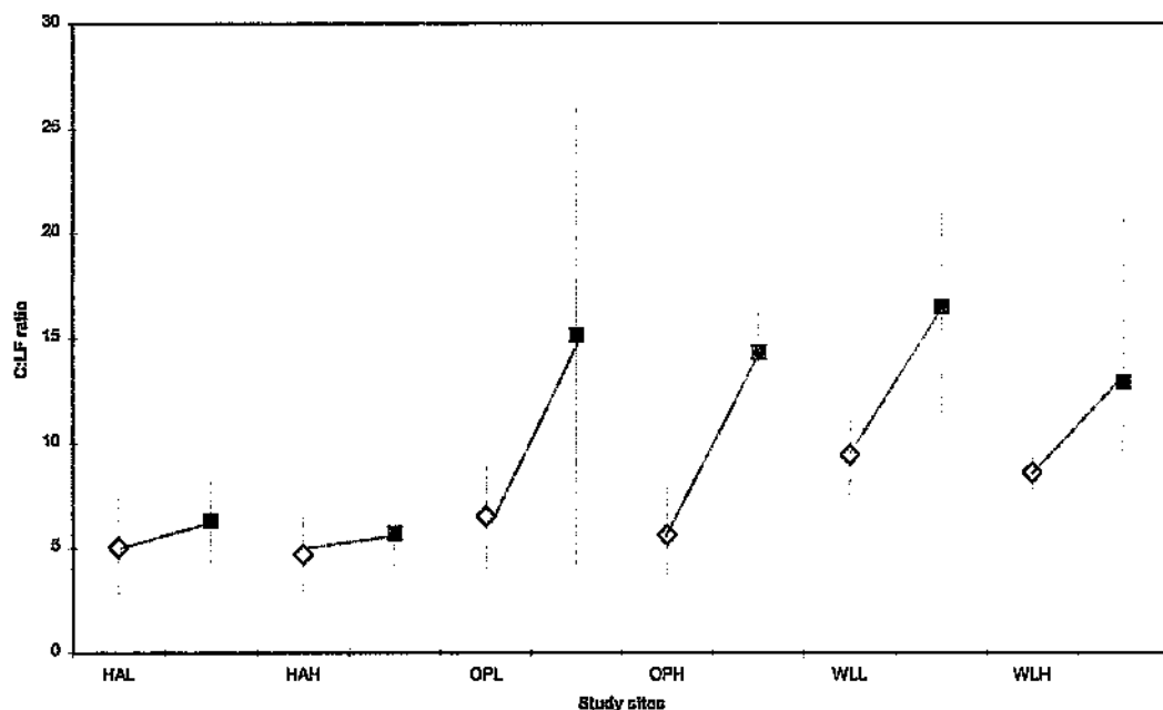
Figure 8.5: Mean C:LF and standard deviation calculated for each study site in March'98 (◊) and October'98 (■).
