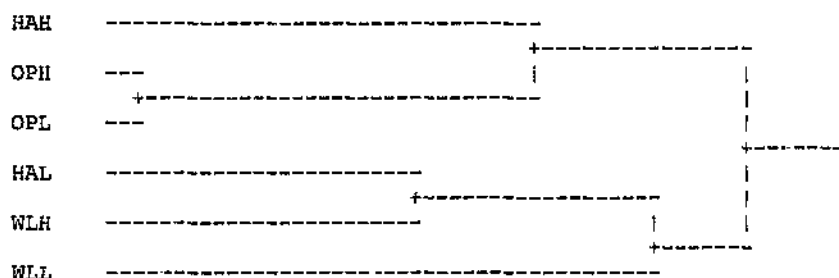
Figure 8.6: Dendrogramme of the cluster analysis performed on the termite presence/absence matrix for taxa found at transects and during searches at the six study sites. The average linkage method was used measuring Euclidean distance.
