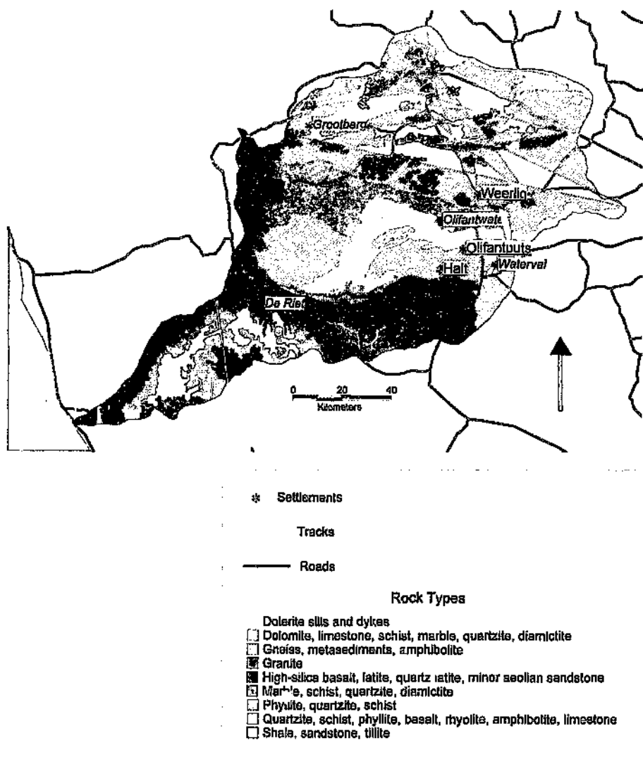
Figure 2.4: Huab Catchment : Geology
