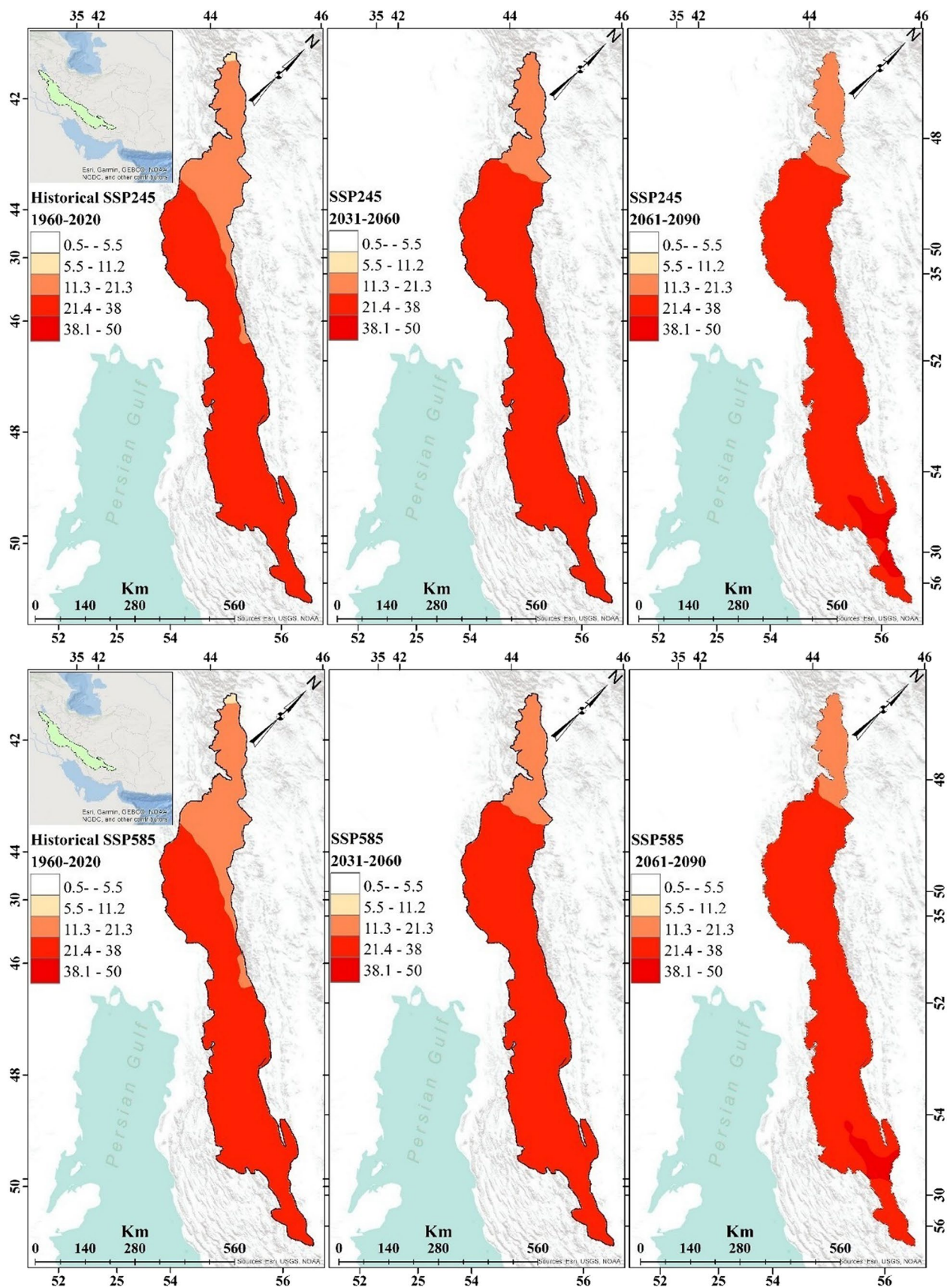
Fig. 5 Spatial distribution of the annual average FWI considering the reference period and future data series
