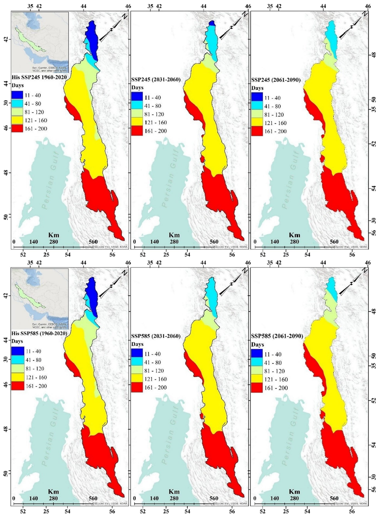
Fig. 7 Comparison of the spatiotemporal distribution of the average number of days per year with FWI > 38 for the reference and future periods
