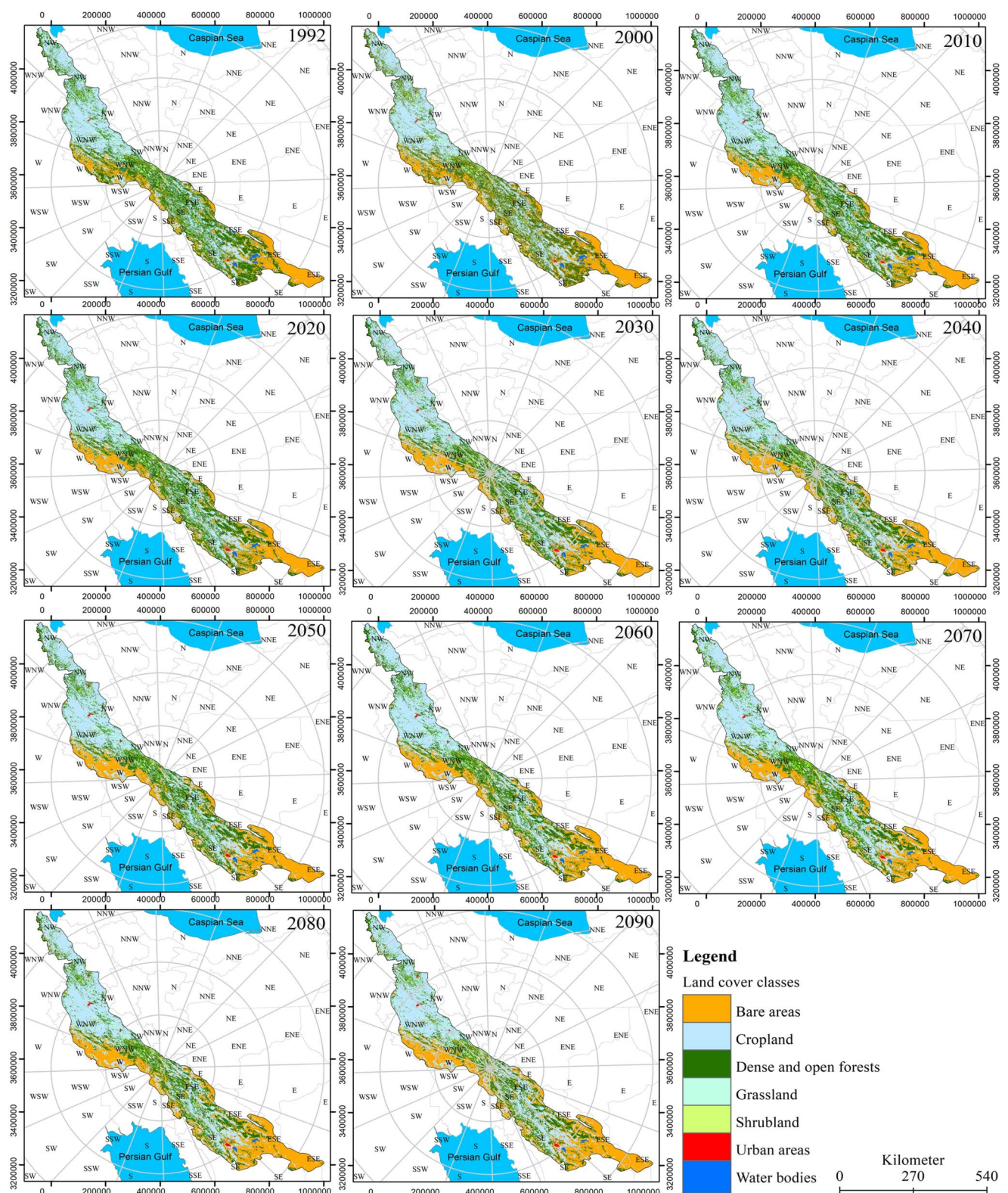
Fig. 9 Spatiotemporal changes in land use across the Zagros region during the study period: 1992–2090
