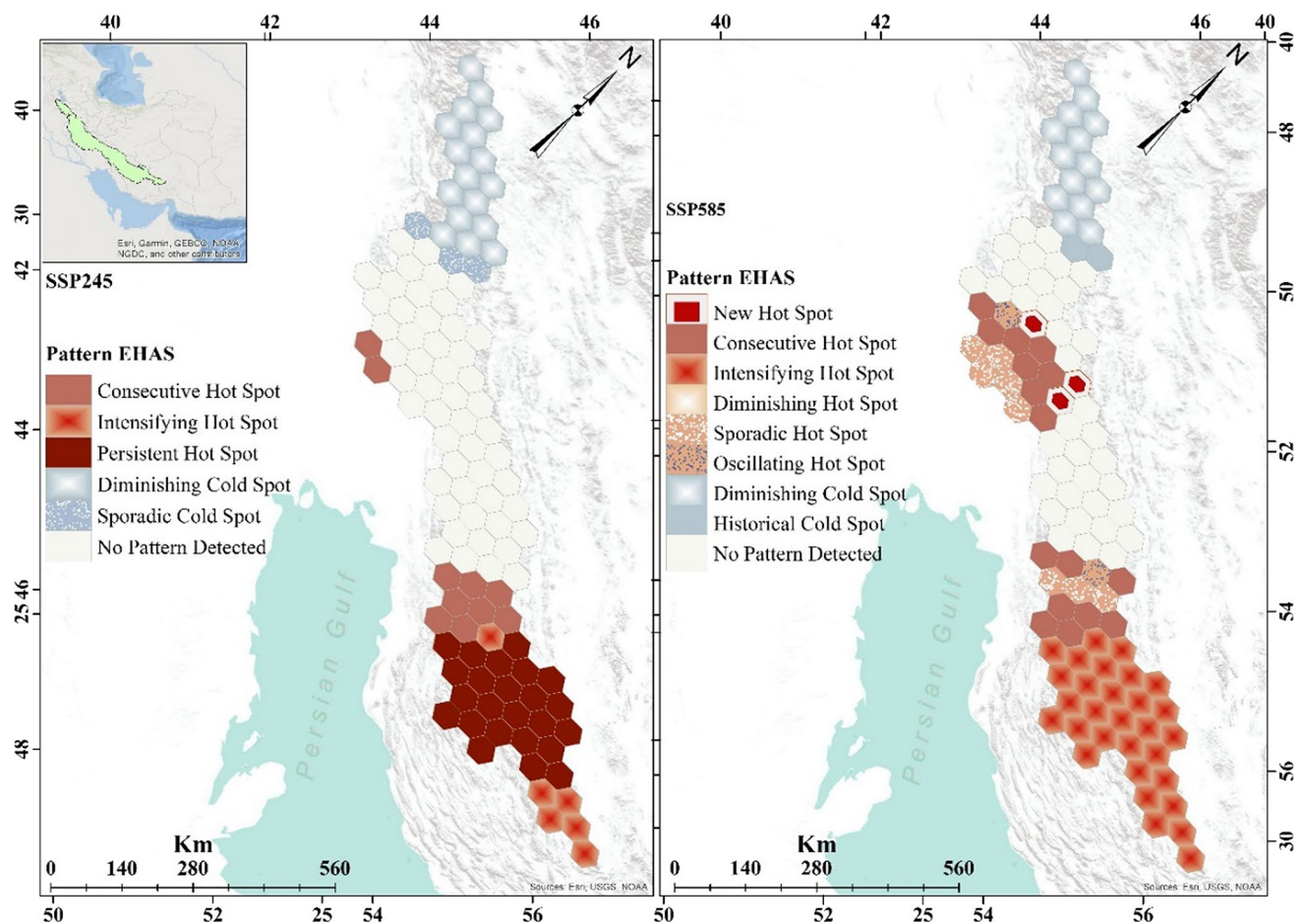
Fig. 15 Spatiotemporal anomalies of FWI (> 38) over the Zagros Mountains using EHSA analysis
