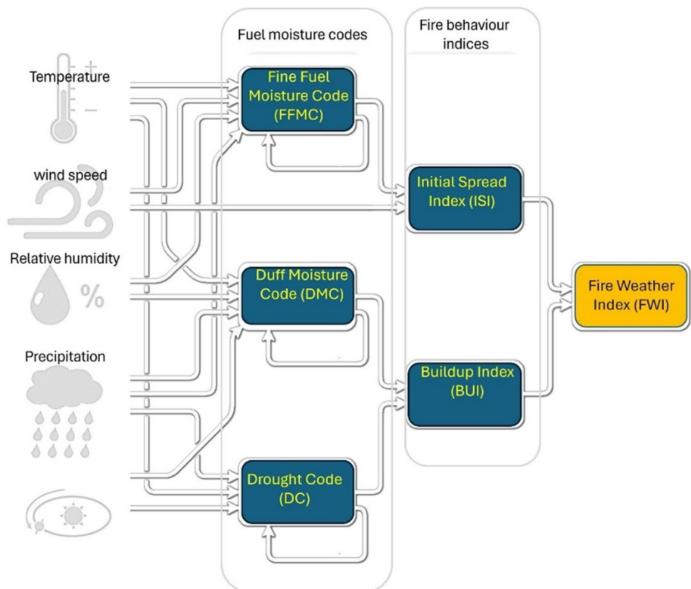
Fig. 2 Structure of the Canadian Forest fire weather index system (after De Groot 1987; de Rigo 2016)
