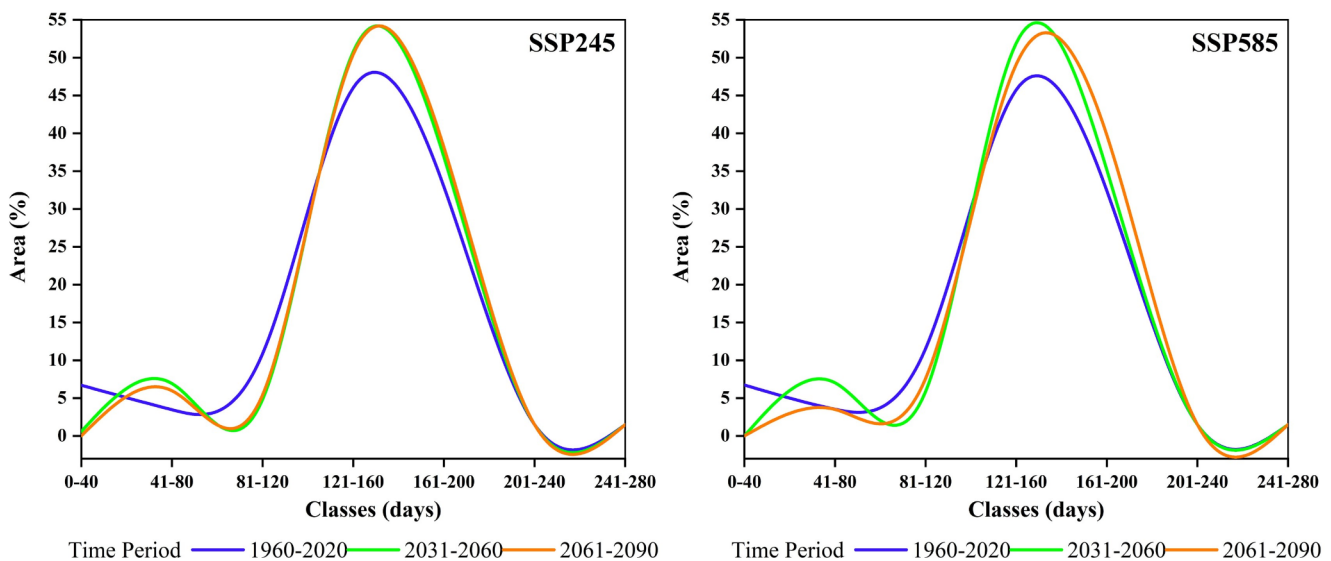
Fig. 6 Comparison of the area corresponding to the average annual frequency of FWI > 38 based on the time series of the reference period and future data in scenarios SSP245 and SSP585
