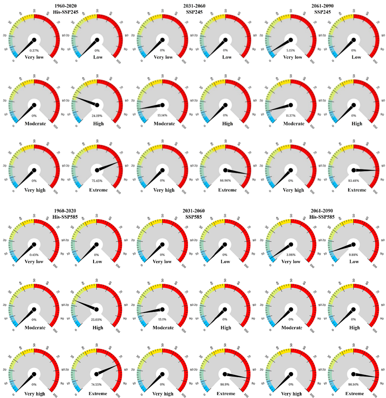
Fig. 4 Comparison of the area corresponding to the annual average of different FWI classes based on the temporal series of the reference period and future data
