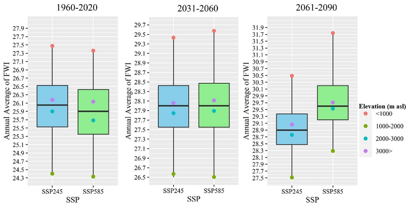
Fig. 12 The mean annual FWI for elevation classes from < 1000 m asl to > 3000 m asl considering the reference period and future data series
