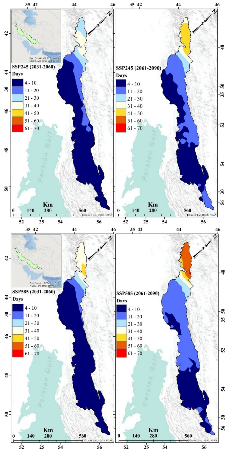
Fig. 8 Daily frequency (average number of days per annum) of FWI > 38 values for future decades, relative to the reference period
