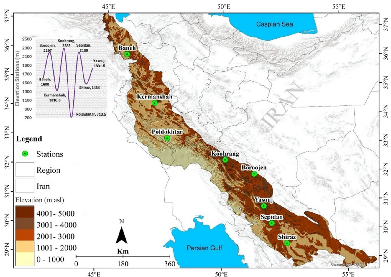
Fig. 1 The Zagros Mountain study region
