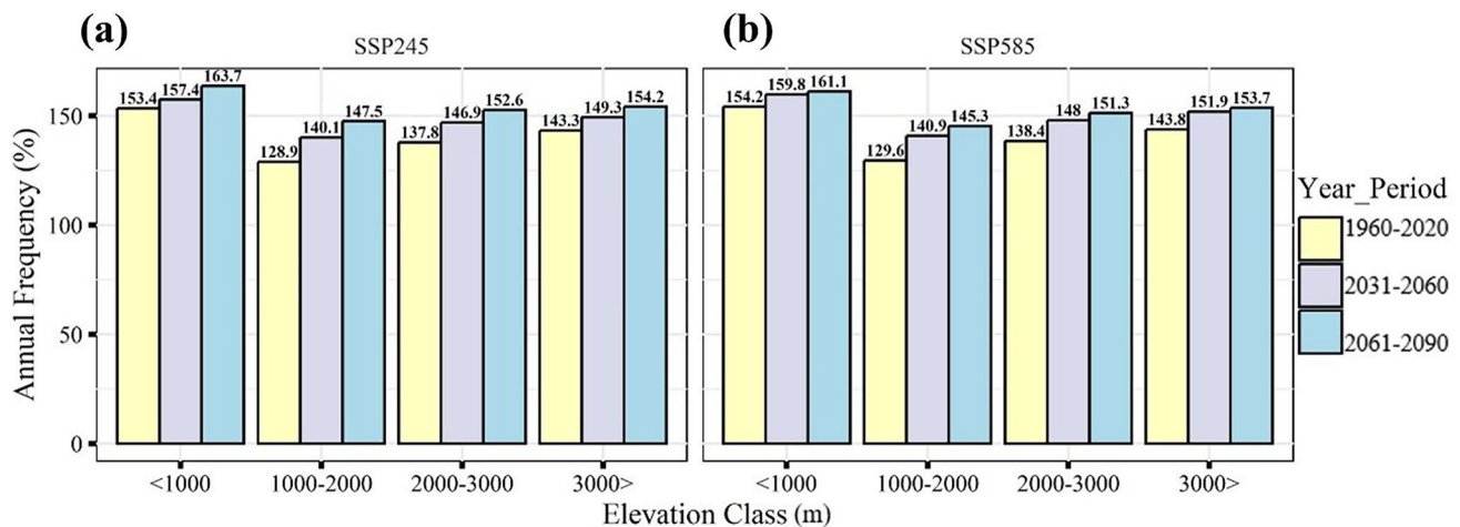
Fig. 13 The percentage annual frequency of FWI > 38 based on different elevation classes for a SSP245 and b SSP585
