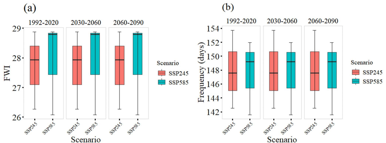
Fig. 11 a Comparison of annual average FWI and b average frequency of days per year with FWI > 38 values based on time series of dense and open forests land use areas
