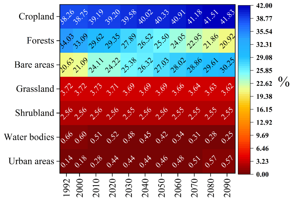
Fig. 10 Percentage land use cover for different periods of time
