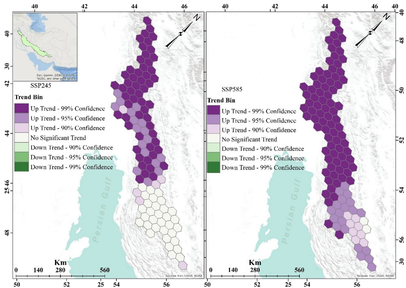
Fig. 14 Changes in FWI (>38) over the Zagros Mountains using the Mann–Kendall method
