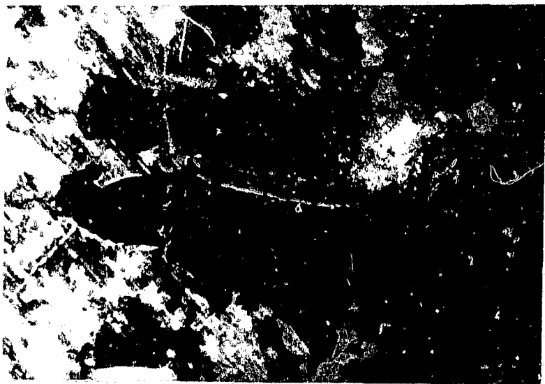
Micrograph of graphic granite showing an ex-solution rim of quartz (a), at the quartz (black mineral) microcline-microperthite border. A 60. Crossed nicols. Slide X 4653.
