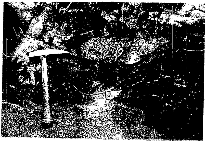
Aplite vein cutting granite (mottled), and enclosing a xenolith of granite. Xenolith is parallel to the aplite strike indicated by the direction of the hammer.
