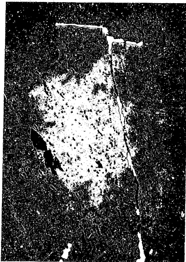
Micrograph of a polished section showing gold (white) in magnesite (grey). The gold has formed along cleavage planes in the magnesite. Shabanie Mine. X 70.
