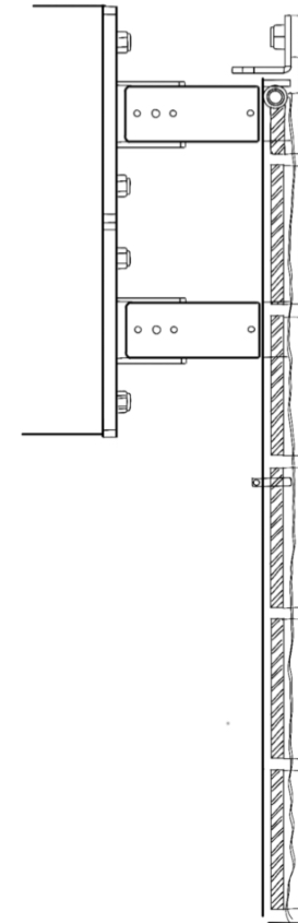
Figure 9.36: Example of a wind system anchor detail (Sarrablo, 2017).
