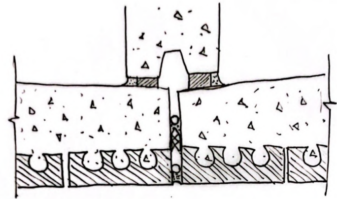
Figure 9.28: Author's plan drawing indicating how brick is casted into concrete panels
