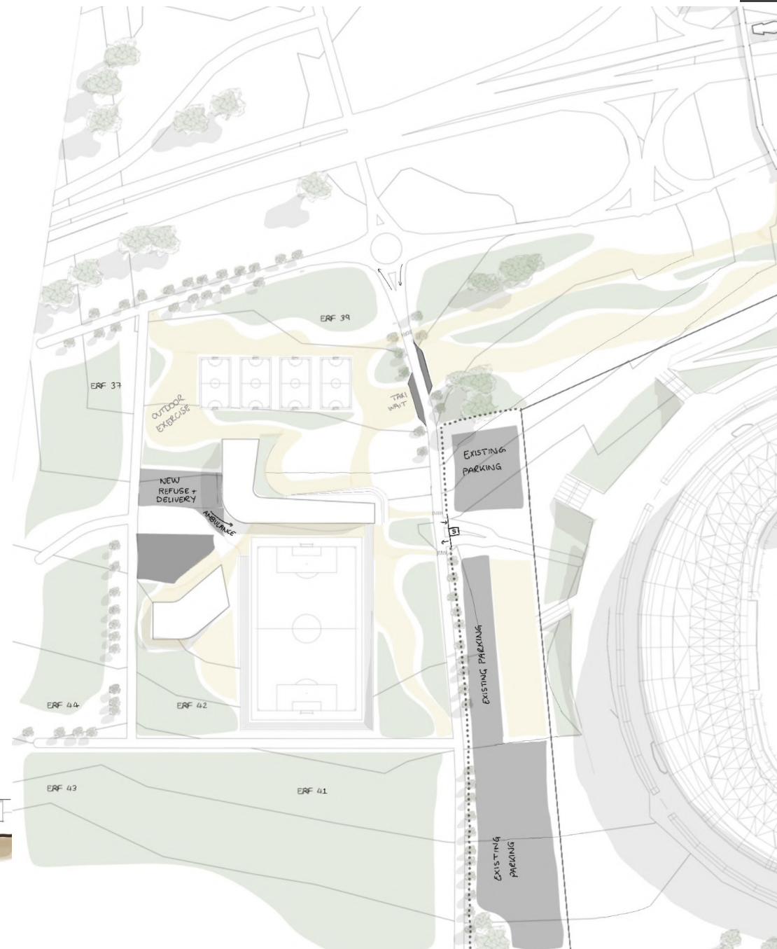
Figure 9.17: Author's drawing of revision 2 site plan
