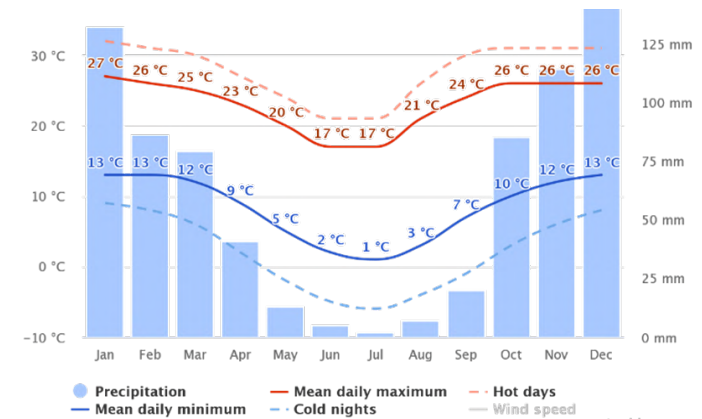
Figure 6.28: Average rainfall and temperatures in Nasrec, Johannesburg (Meteoblue, 2023)
