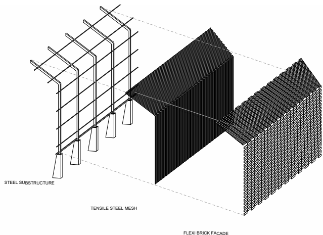
SCREEN AXONOMETRIC EXPLORATION
