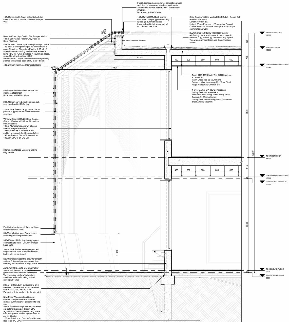
SCREENING PERIMETER SECTION
