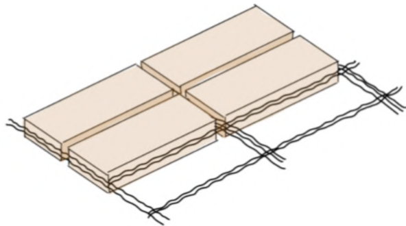
Figure 9.32: Author's drawing of how the wire mesh attaches to the ceramic tile
