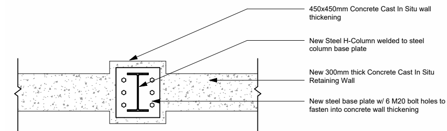
Figure 9.30: Author's technical plan detail of steel column connection
