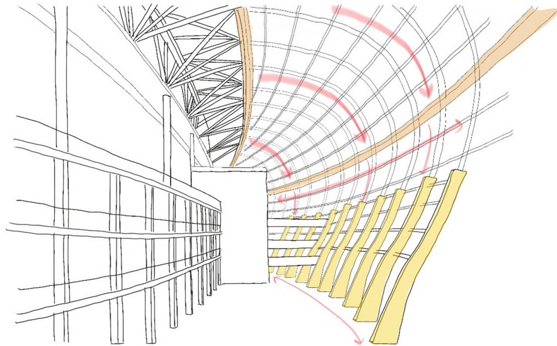
Figure 7. 16: Diagram illustrating the facade structure connection to the inclined concrete columns (Author's drawing)
