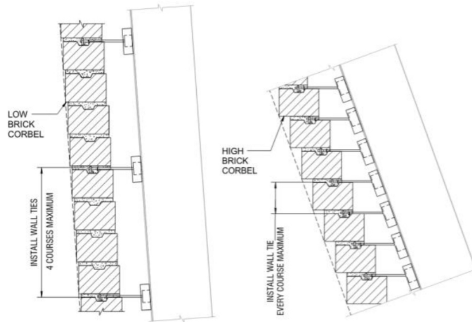
Figure 9.25: Image of wall sections showing tie arrangements (Inglis, 2020)
