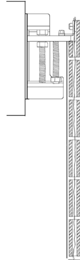
Figure 9.37: Example of a weight system anchor detail (Sarrablo, 2017).
