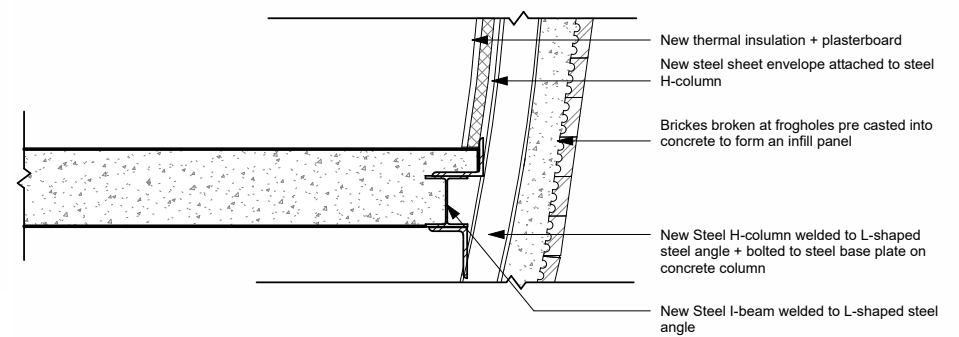
Figure 9.31: Author's technical sectional detail of steel column connection
