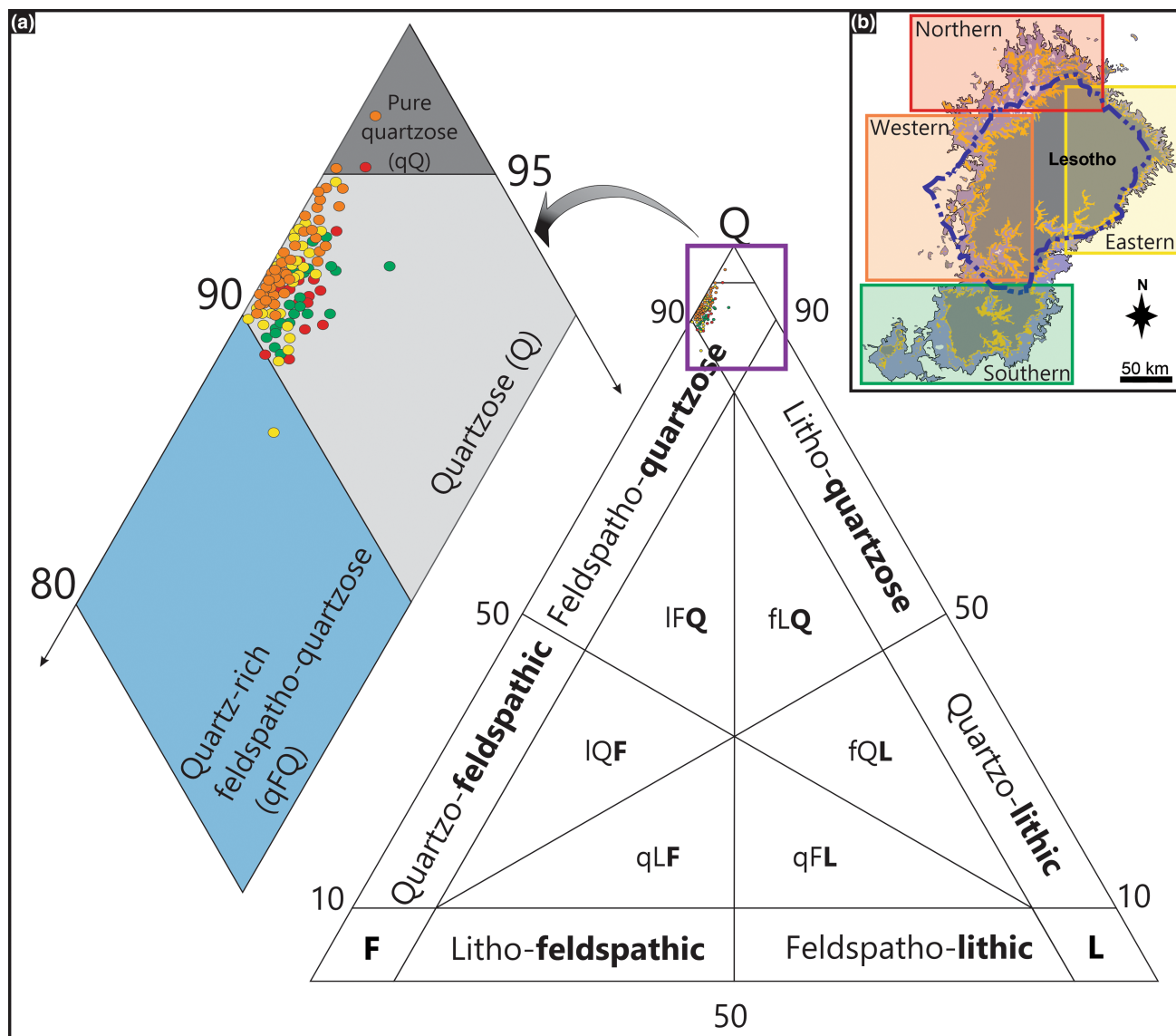
FIGURE 5 Sandstone composition of Clarens Formation samples (using the classification of Garzanti, 2019) (a). For regional sample locations, see colour coded map inset in (b). F, K-feldspar and plagioclase; L, Lithic fragments including chert; Q, total quartz. Note that the samples taken from the northern (red), eastern (yellow) and southern (green) sampling areas contain relatively more lithics than the western (orange) samples.
