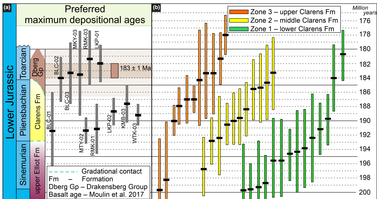
FIGURE 11 Detrital zircon geochronology of the Clarens Formation. (a) Preferred maximum depositional ages. (b) Distribution of all zircon dates younger than 200 Ma. Zones are lithostratigraphic intervals as defined by Beukes (1969, 1970) and refined by Head (2022). Bar heights (yellow, green, orange, and grey) depict 2 SE uncertainty. In addition to Moulin et al. (2017), the 183 \pm 1 Ma age of the Drakensberg Group is also based on Duncan et al. (1997) and Svensen et al. (2012).
