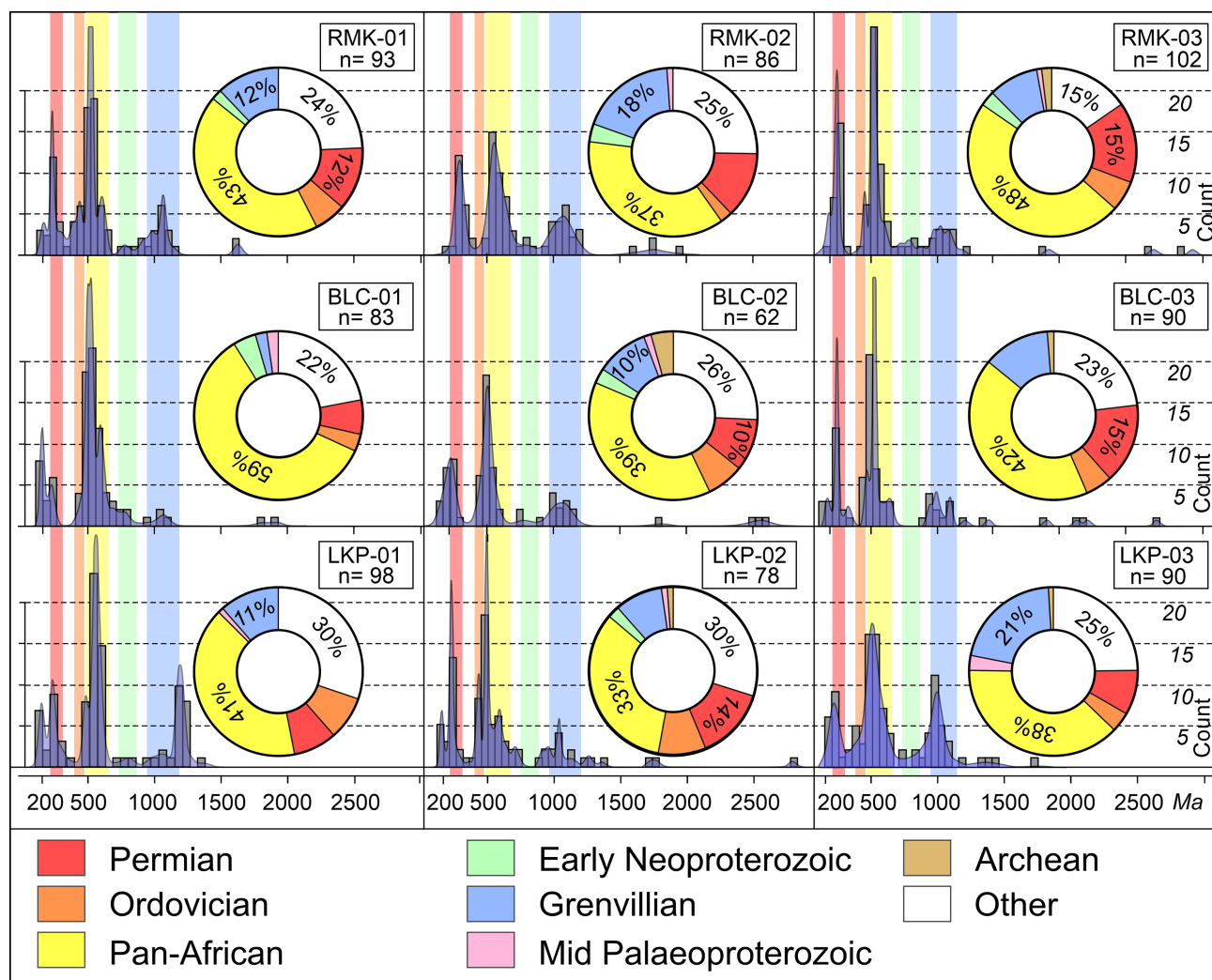
FIGURE 8 Kernel density estimates (KDEs) of nine samples from the southern half of the outcrop area combined with donut plots depicting the percentage of each age fraction that can be attributed to the large-scale tectonic events during time periods listed in the legend. The white boxes show the sample label and the number of concordant dates plotted in each diagram. See Figure 2 for sample locations and Figure 3 for the relative stratigraphic position of the samples within each sampled section (01: bottom, 02: middle, 03: top).
