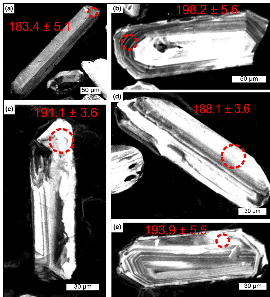
FIGURE 9 CL images of zircons with youngest dates of samples BLC-02-28, BLC-01-96, RMK-01-32, RMK-02-85 and BLC-01-38, respectively. (a–e) Zircons with oscillatory zoning typical of igneous origin, with euhedral to subhedral shape. Red circles represent ablation spots; ^{206}\text{Pb}/^{238}\text{U} concordant dates (Ma) \pm 2 SE uncertainty. Error propagation using zircon involves combining excess uncertainty (from “pseudosecondary standards”) with internal errors for each analysis (Paton et al., 2010).
