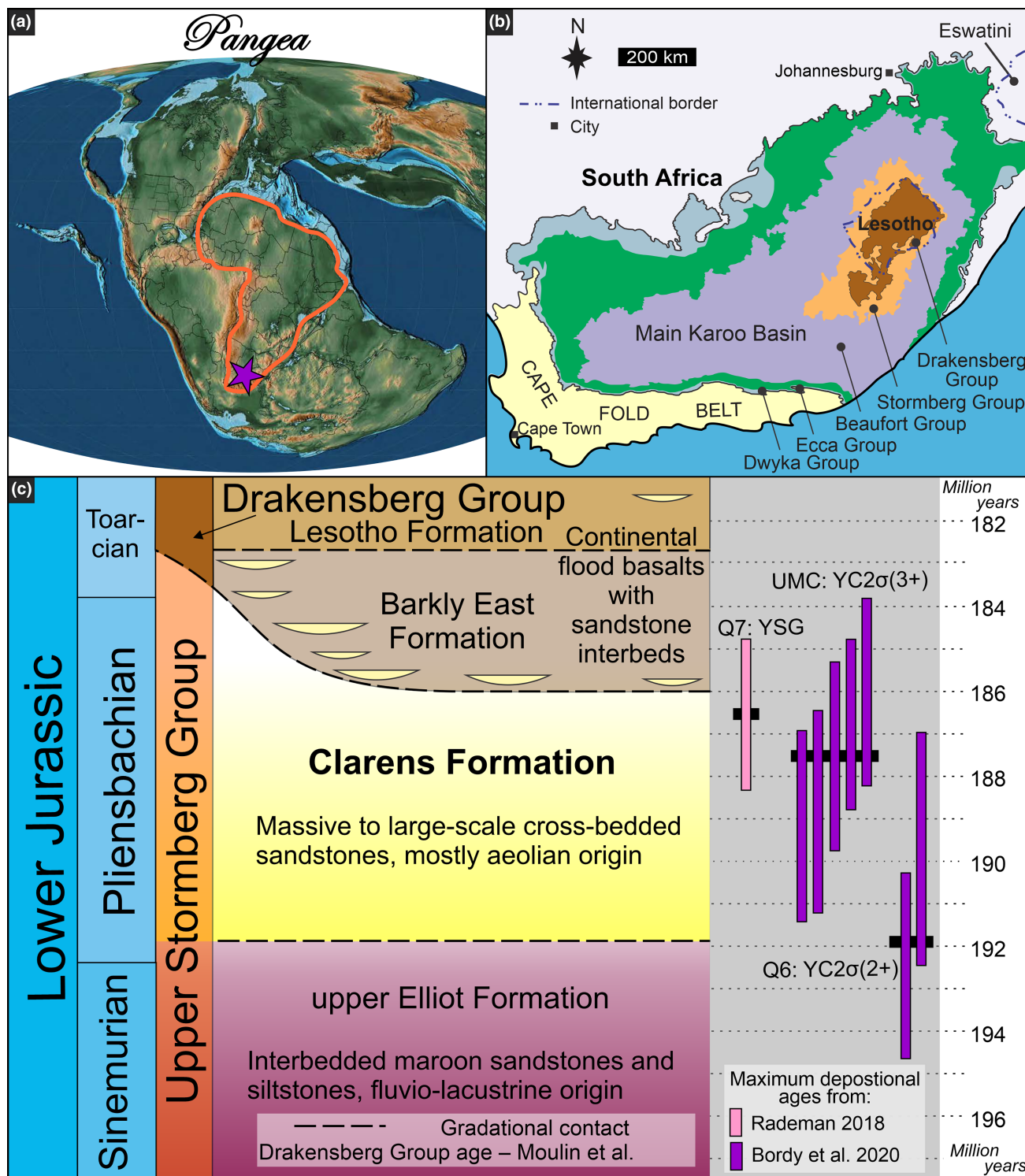
FIGURE 1 Geological context of the Clarens Formation. (a) Palaeo-geographic location of the Clarens Formation within Pangea in the Early Jurassic (base map modified after Scotese, 2014). (b) Geographical distribution of the stratigraphic groups in the Karoo Supergroup in the MKB of South Africa and Lesotho. (c) Abbreviations Q6, Q7, and UMC are sample numbers of previously published studies of the upper Karoo Supergroup, which includes the upper Stormberg (Elliot and Clarens formations) and Drakensberg groups (Bordy, Abrahams, et al., 2020; Bordy, Rampersadh, et al., 2020; Moulin et al., 2017; Rademan, 2018). YSG, youngest single grain, YC2 \sigma (2+), youngest cluster of 2 or more zircon dates that overlap at 2SE.
