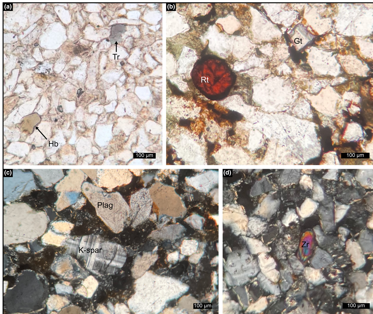
FIGURE 4 Photomicrographs of common and accessory minerals in the Clarens Formation. (a) Yellow-brown hornblende (Hb) and tourmaline (Tr) in a quartz-dominated sandstone—PPL. (b) Rutile (Rt) and garnet (Gt) amongst quartz grains in PPL. (c) K-feldspar (K-Spar) and plagioclase (Plag) amongst quartz grains in XPL. (d) Zircon (Zr) amongst grains in XPL. Note that the moderately to well-sorted sand grains are subrounded to subangular.
