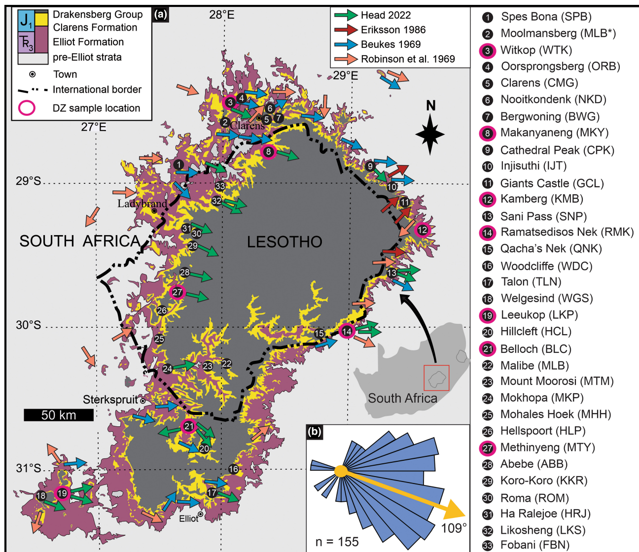
FIGURE 2 Spatial distribution of palaeo-current data and rock samples from the Clarens Formation. (a) Geological map of the upper Karoo Supergroup with sample locations of this study shown in numbered circles. DZ/magenta circles—samples used for detrital zircon U–Pb dating; coloured arrows – subregional palaeo-current directions from various studies. (b) Summary rose diagram for the Clarens Formation in the MKB from palaeo-current measurement of this study. n —total number of measurements; yellow arrow—the main palaeo-current vector.
