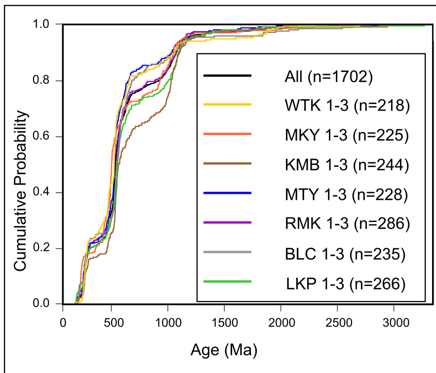
FIGURE 10 Cumulative probability plots for all samples combined and grouped per sample location.
