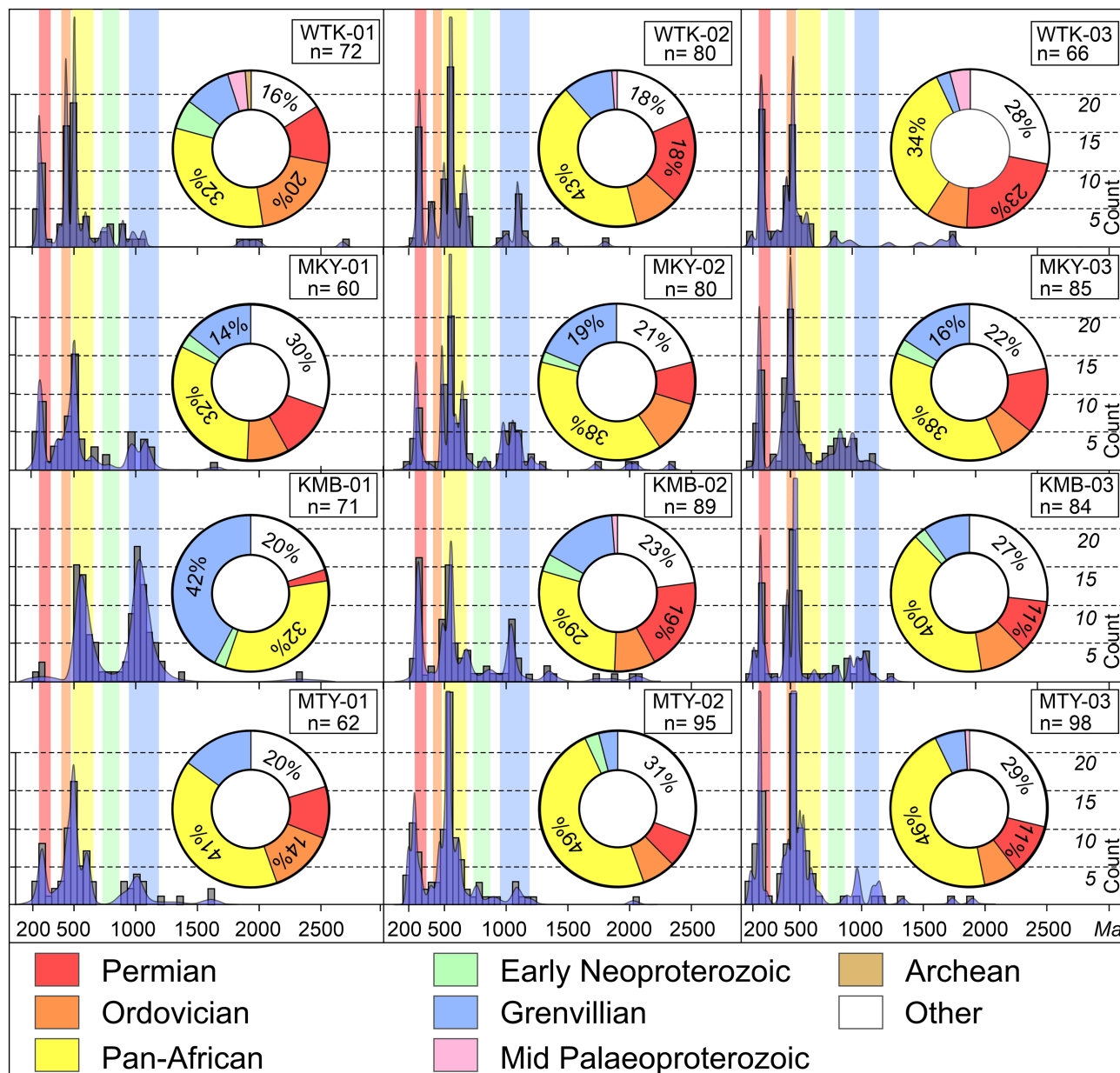
FIGURE 7 Kernel density estimates (KDE) of 12 samples from the northern half of the outcrop area combined with donut plots depicting the percentage of each age fraction that can be attributed to the large-scale tectonic events listed in the legend. The white boxes show the sample label and the number of concordant dates plotted in each diagram. See Figure 2 for sample locations and Figure 3 for the relative stratigraphic position of the samples within each sampled section (1: bottom, 2: middle, 3: top).
