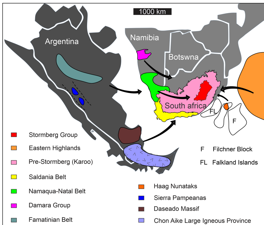
FIGURE 12 Source rock distribution of the Clarens Formation in southern Gondwana during the Early Jurassic (map compiled and modified after Bial et al., 2015; Bordy & Head, 2018; Casquet et al., 2008; Foster et al., 2015; Frimmel et al., 2013; Jacobs et al., 2008; Muir et al., 2020; Pankhurst et al., 2000; Pankhurst et al., 2006 and Ryan & Whitfield, 1979).
