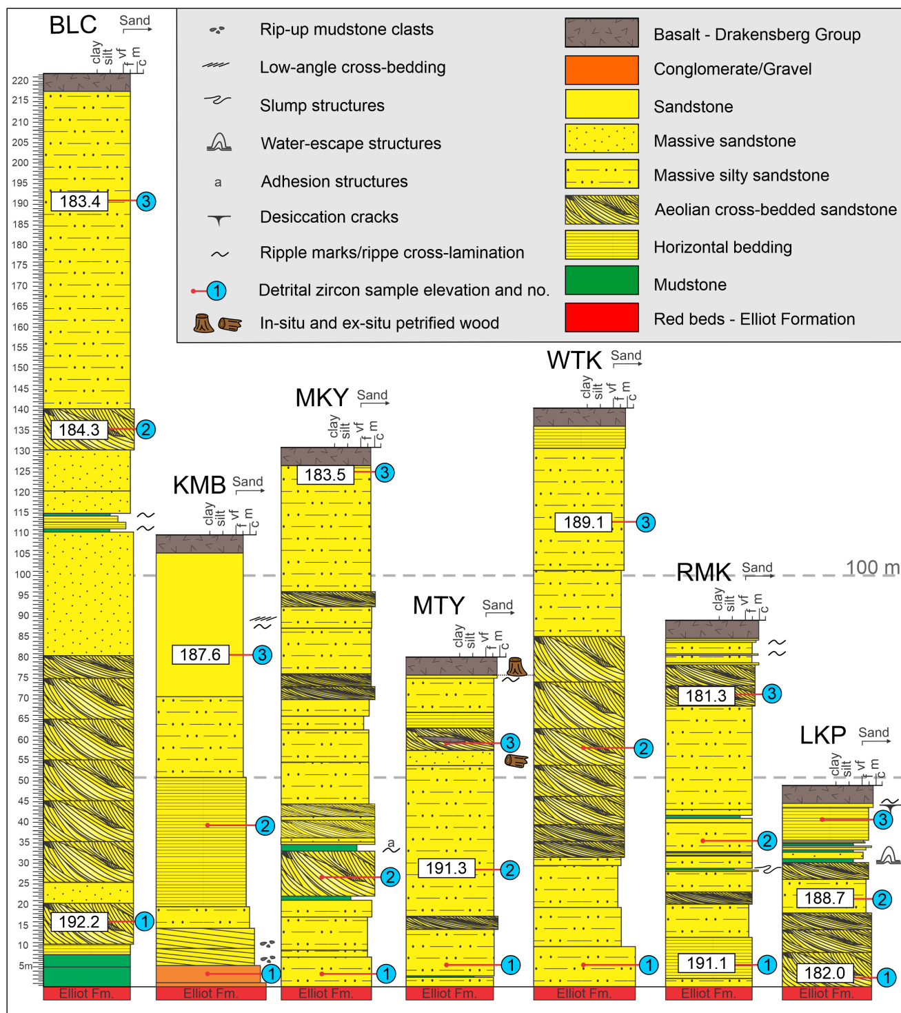
FIGURE 3 Sedimentary logs from this study with stratigraphic locations of detrital zircon samples and preferred MDAs in the Clarens Formation as detailed in Table 1. Note that the overlying 3-letter code refers to the location name, while samples labelled '1', '2' and '3' are from the three different stratigraphic intervals ('zones') of the Clarens Formation, and when combined, give the various sample names—e.g., BLC-01. See Figure 2 for log abbreviations and locations within the study area. For associated 2 SE uncertainty, see Table 1.
