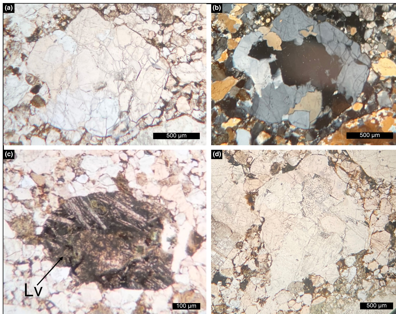
FIGURE 6 Photomicrographs of rare lithic fragments in the Clarens Formation. (a, b) Polycrystalline quartz in PPL (a) and XPL (b). (c) Volcanic lithic fragment (Lv: basalt grain) with jagged outline in the uppermost part of the Clarens Formation at Talon—PPL. (d) Polycrystalline quartz in the lowermost Clarens Formation at Kamberg. See Figure 2 for sample locations.
