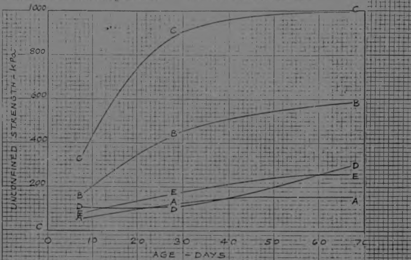
FIGURE 3b STRENGTH-AGE CURVES FOR AN 80%:20% GRANITE SAND:GRANULATED SLAG MIX CONTAINING 5% OF VARIOUS ACTIVATORS EACH EXPERIMENTAL POINT IS THE MEAN OF 3 DETERMINATIONS.
