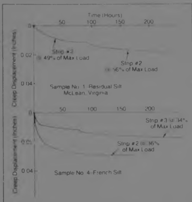
Fig 34: Creep Tests-Ribbed Strips
