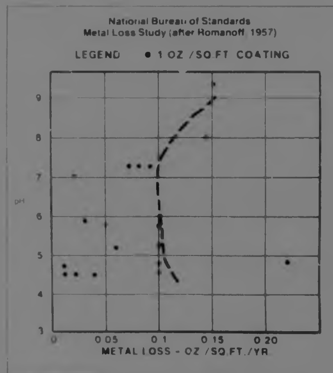
Fig 39 Metal Loss versus pH-Well Drained Sites Only
