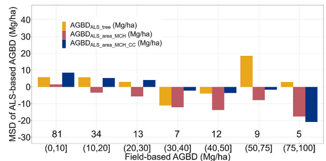
Fig. 10. Histogram of Mean Systematic Deviation of yellow: AGBD_{25m\_ALS\_tree} ; red: AGBD_{25m\_ALS\_area\_MCH} ; blue: AGBD_{25m\_ALS\_area\_MCH\_CC} vs. field estimated AGBD_{25m\_field\_25m} values were binned at 10 Mg/ha increments up to 50 Mg/ha, and in increments of 25 Mg/ha from 50 Mg/ha to 100 Mg/ha. The bottom row of numbers represents bin counts.
