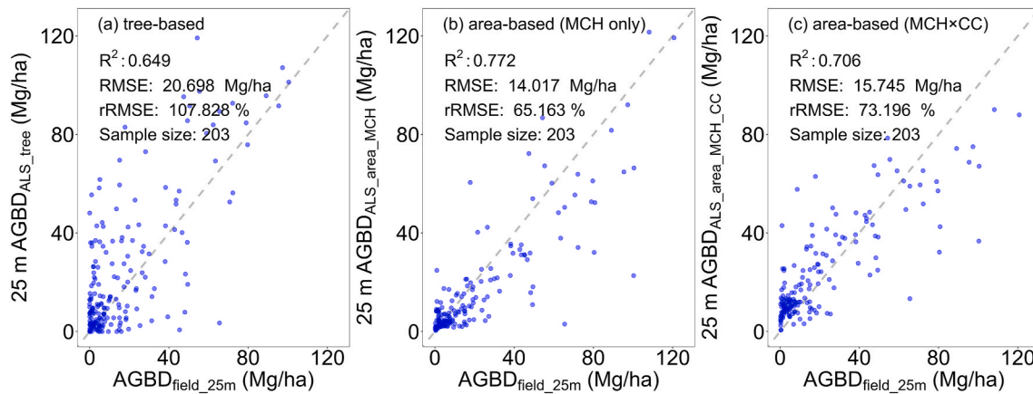
Fig. 8. Scatterplots of ALS-based AGBD vs. AGBD field measurements at 25 m level. a: tree-based method; b: area-based method (MCH); c: area-based method (MCH \times CC).
