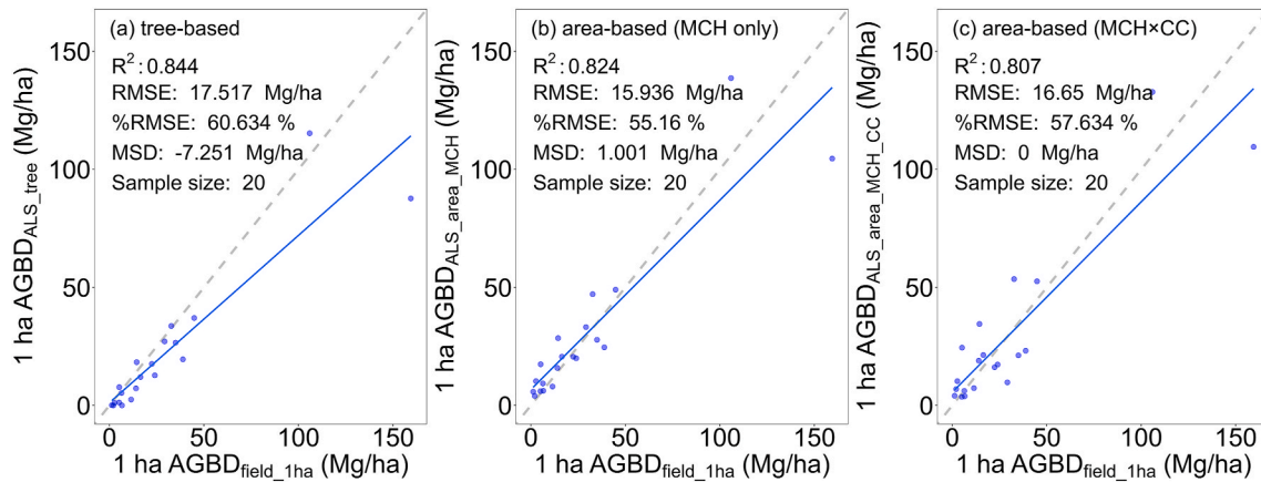
Fig. 7. Scatterplots of ALS-based AGBD vs. AGBD field measurements at 1 ha level. a: tree-based method; b: area-based method (MCH only); c: area-based method (MCH \times CC).
