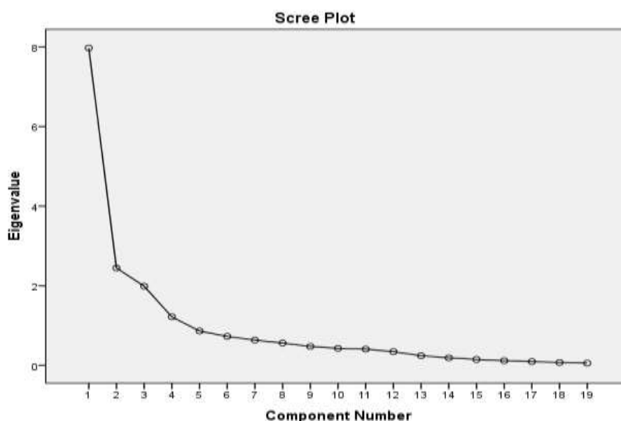
Figure 13: Scree plot.
