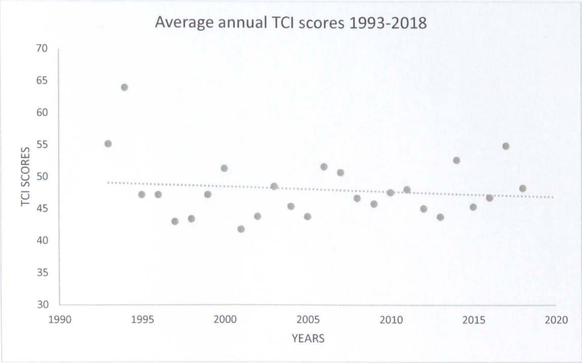
Figure 5.5: Annual average TCI score for the year 1993 to 2018
