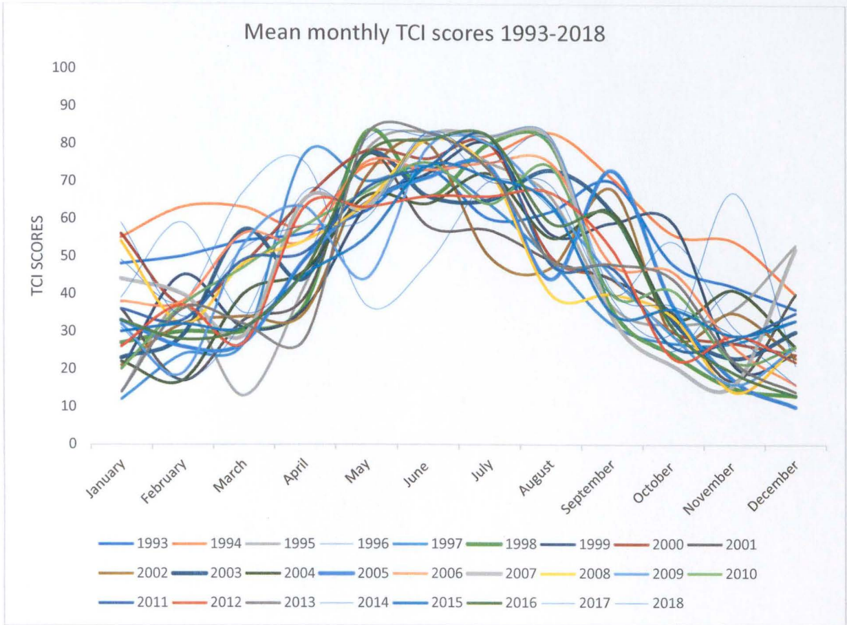
Figure 5.6: Scott and Mc Boyle’s (2001) classification of a winter peak seasonal variability for the 25-year period in Polokwane Limpopo, South Africa.
