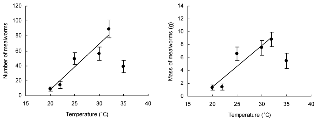
Fig. 3 The effect of temperature on appetite in terms of the number of mealworms eaten ( left ), and of temperature on the mass of mealworms eaten ( right ) for C. m. melanotus (regression analysis; number: y = 6.15x - 114.86 , R^2 = 0.91 , P = 0.01 ; mass: y = 0.65x - 11.55 , R^2 = 0.89 , P = 0.02 ; Mean \pm SE; N = 20 , 10 male 10 female for all temperature treatments). Measurements at 35 °C were not included in the regression analysis because lizards showed distress and the trial was aborted after only 3 days
