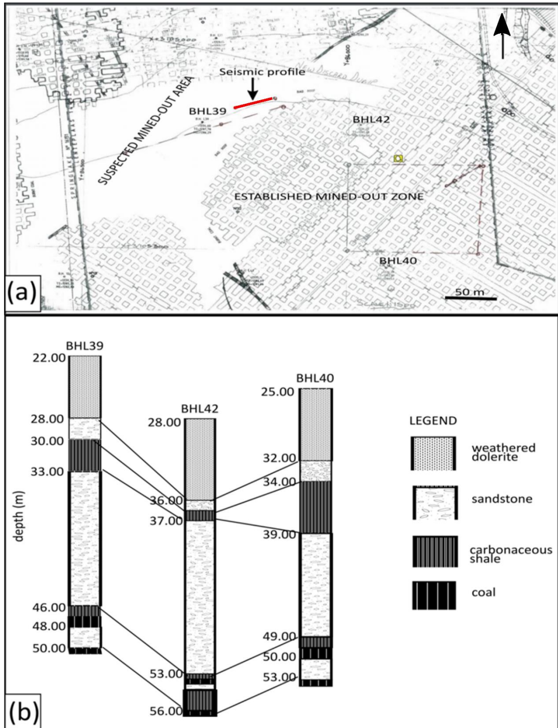
Figure 3.4: (a) Underground mine plan of the Springlake mine showing the seismic profile acquired across the suspected mined-out zone. (b) Boreholes from the Springlake mine showing the subsurface stratigraphy.
