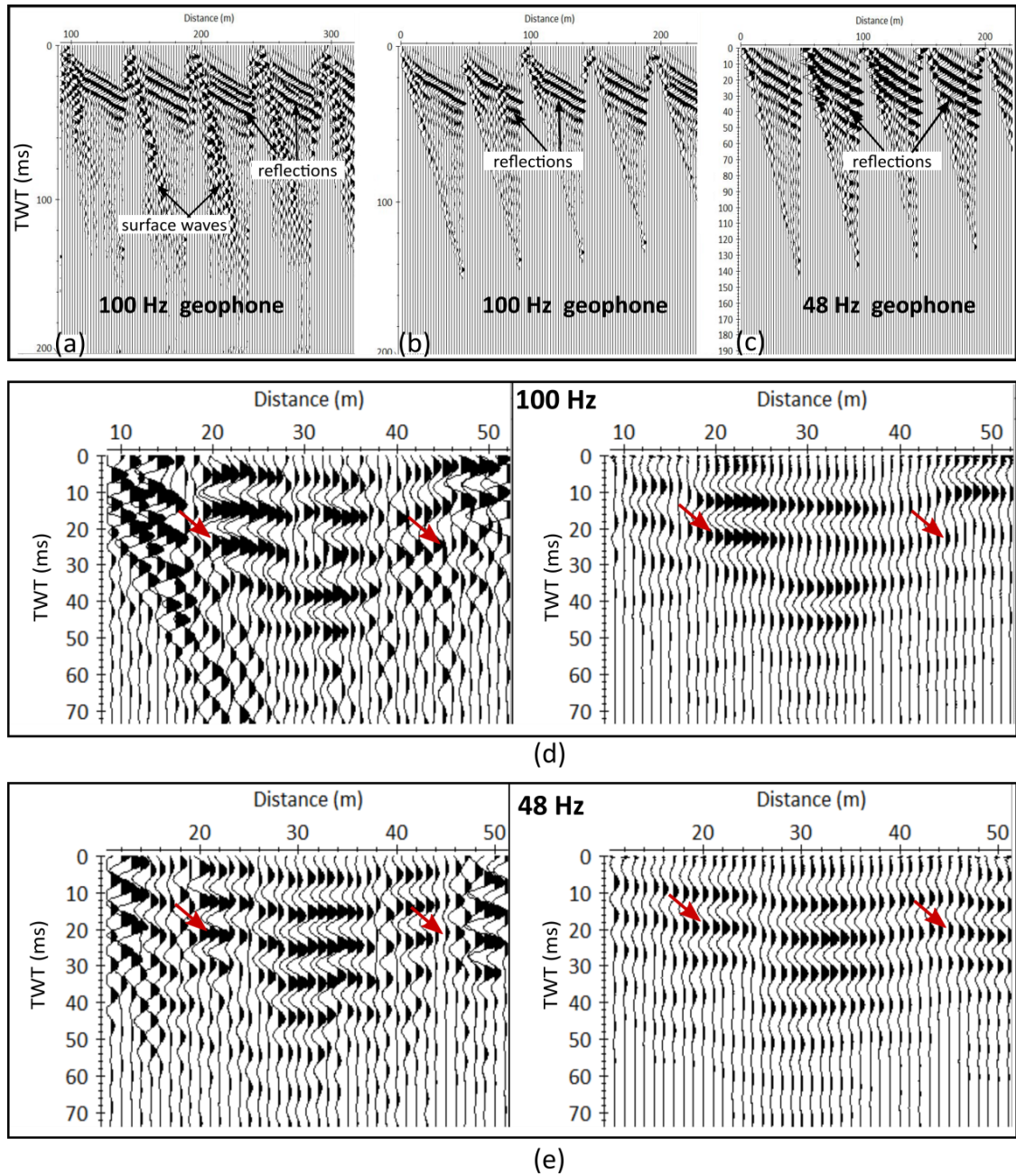
Figure 3.13: Pre-stack and the corresponding stacked sections obtained for the two geophone types along LN1. (a) Shot gathers from the 100 Hz geophone with visible reflection events after applying a bandpass Butterworth filter. Trace normalized gain is applied for display, (b) The same shot gathers from the 100 Hz geophone after applying a surgical bottom mute at 330 m/s. Note the muting of the surface air waves, (c) Shot gathers from the 48 Hz geophone showing visible reflection events after applying a bandpass Butterworth filter and a surgical bottom mute. Trace normalized gain is applied for display, (d) Stacked and the corresponding migrated section (without AGC) obtained with the 100 Hz geophone type, and (e) Stacked and the corresponding migrated section (without AGC) obtained with the 48 Hz geophone type. The top of the dolerite layer is indicated by the red arrow.
