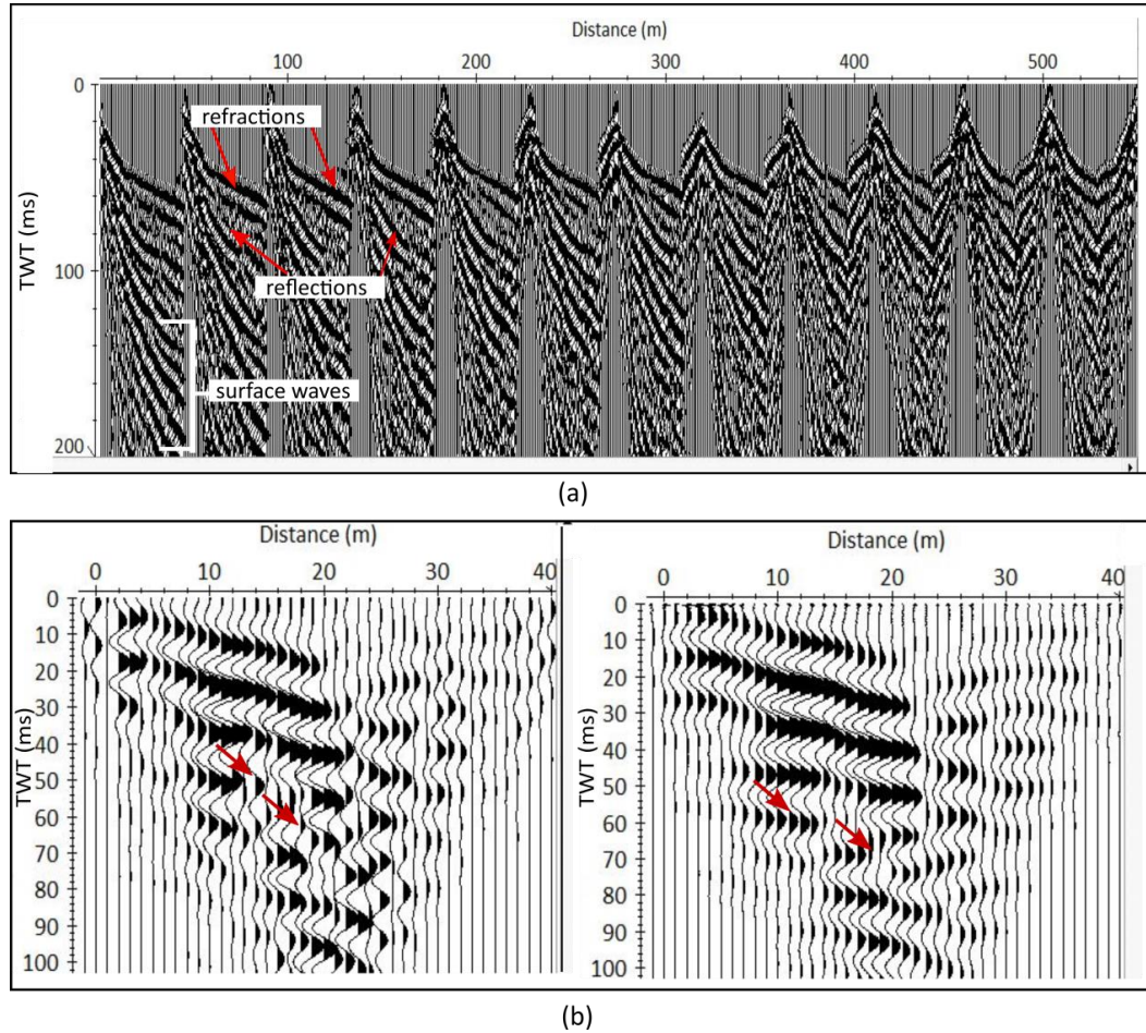
Figure 3.17: (a) Pre-stack shot gathers along the Springlake profile showing visible reflection events after applying a bandpass Butterworth filter, and (b) Stacked and migrated section (with AGC applied). Note the disrupted zone indicated with the arrows below \sim 40 ms.
