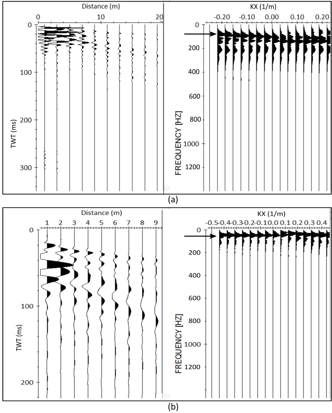
Figure 3.8: Selected traces and the corresponding amplitude spectra for (a) the Benoni datasets and (b) the Springlake datasets. The arrow indicates the largest amplitude corresponding to the frequencies of the surface waves.
