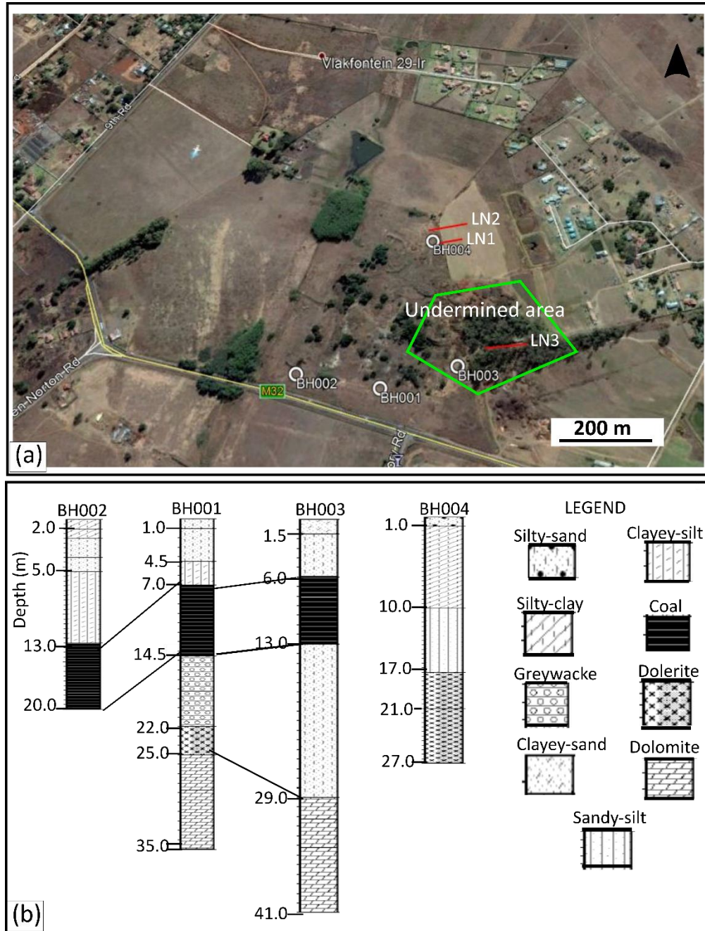
Figure 3.3: (a) Satellite image of Benoni study area showing the location of the boreholes and the seismic lines acquired in the area. (b) The stratigraphical correlation of the geology encountered in the boreholes shows that the coal seam deepens towards the west of the study area. Note the undermined area within the polygon.
