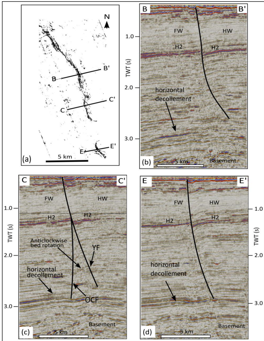
Figure 4.4: Interpreted perpendicular sections along the strike of the AK Fault. (a) Cross-sections along the different segments of the fault. (b) Sigmoidal fault plane geometry along the fault's bends. (c) Evidence of reactivation of the AK Fault revealed by the cross-cutting of the Early Cretaceous fault (OCF) by the Late Cretaceous, Cenozoic fault (YF) and the anticlockwise rotation of beds caused by the freeboard failure of the hanging-wall along a horizontal decollement. (c) Listric geometry of the AK Fault with its base along a horizontal decollement above the underlying crystalline basement. FW- footwall, HW- hanging wall.
