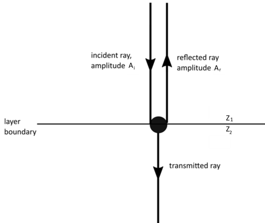
Figure 2.5: Reflected and transmitted rays associated with a ray arriving at normal incidence on an interface with appreciable impedance contrast ( Z_2 > Z_1 ) (modified after Kearey et al., 2002)
