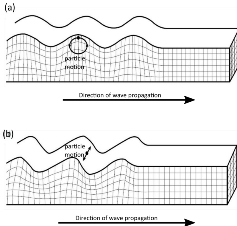
Figure 2.2: Elastic deformations and ground particle motions associated with the passage of surface waves. (a) Rayleigh wave. (b) Love wave. (modified after Kearey et al., 2002)
