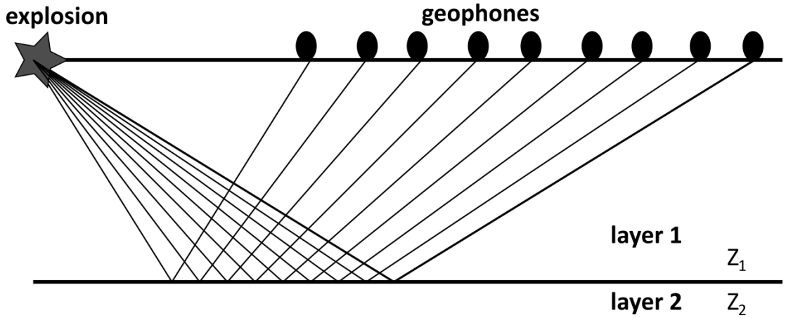
Figure 2.4: An illustration of the principle of reflection seismic method. Z_1 and Z_2 are the acoustic impedance of layers 1 and 2 respectively, ( Z_2 > Z_1 ).
