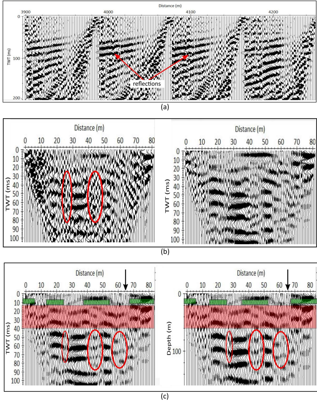
Figure 3.16: (a) Pre-stack shot gathers along LN3 with visible reflections after applying a bandpass Butterworth filter, with trace normalized gain applied for display (b) Stacked and the corresponding migrated section obtained along LN3. Note the alternating chaotic reflection zones (circled region) in the stacked section and the enhanced resolution in the migrated section, (c) Interpreted time and depth migrated section. The green colour highlights the coal seam zone within the un-mined pillars (note the coherent negative reflection amplitude characterizing the coal seam zone), while the highlighted region in red shows the disrupted bedding planes due to near-surface subsidence caused by the collapse of the overburden strata into dissolution cavities (circled region) within the underlying dolomite. The arrow indicates the location of the leaning structure in the undermined area.
