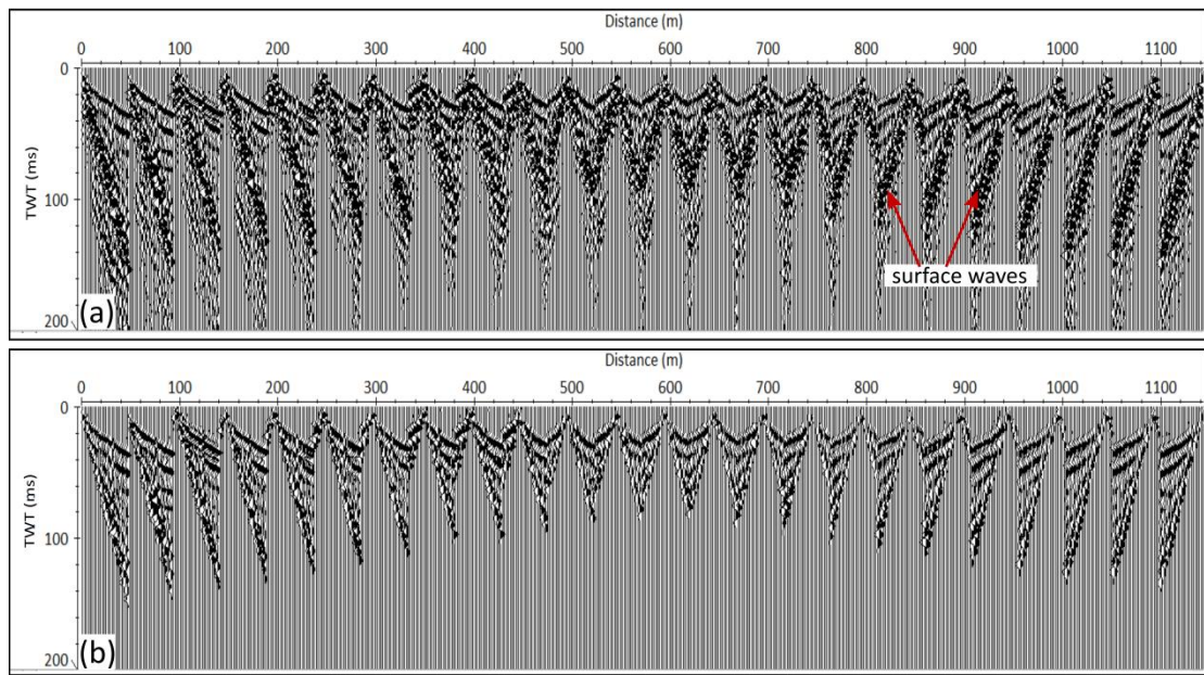
Figure 3.10: Pre-stack shot gathers before (a) and after surgical muting (b). Note the muting of the surface waves that occur in the form of air waves.
