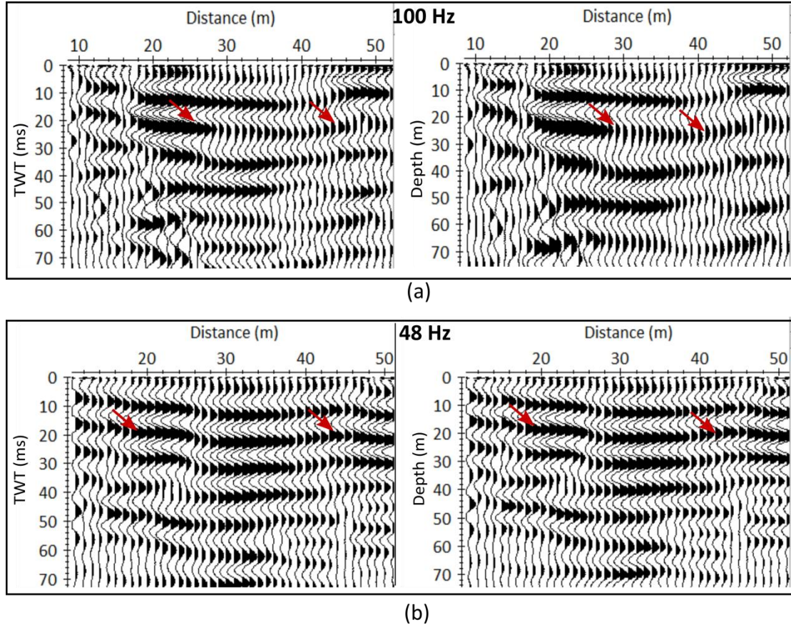
Figure 3.14: TWT migrated section (with AGC applied) and the corresponding depth sections obtained along LN1 (a) 100 Hz geophone type (b) 48 Hz geophone type. The arrow indicates the top of the dolerite layer.
