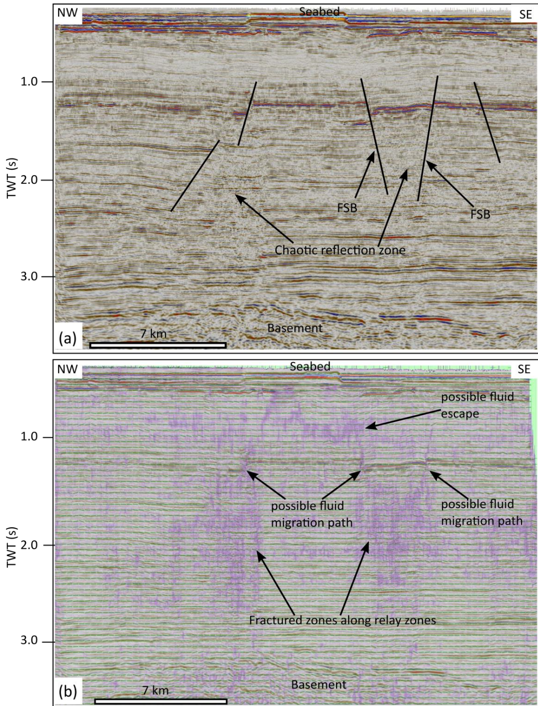
Figure 4.9: Edge attributes analysis to detect possible fluid migration pathways along the boundaries of the fault segments. (a) Interpreted inline section (see details in Fig. 8) showing the boundaries of the fault segments (FSB) and the chaotic reflection zones. (b) Edge attribute section revealing the fractured zones (in purple) where fluid may accumulate, and possible fluid migration paths through which fluid escape may occur.
