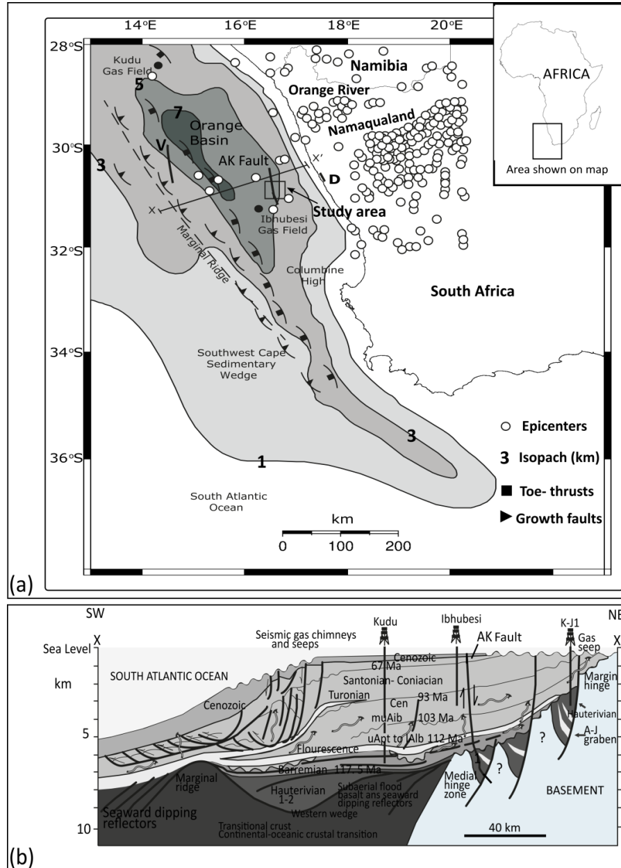
Figure 4.1: (a) Isopach map of the post-rift sedimentary succession in the offshore Orange Basin (modified from Jungslager, 1999). The outline of the AK Fault in the study area is shown along with the other two faults, “V” and “D” previously investigated by Viola et al., (2005) and De Beer (2012) respectively. The overlaid seismological data downloaded from the International Seismological Centre (2017) covers the region around southern Namibia and the Northern Cape, and shows the evidence of seismic activity within the vicinity of the AK Fault. (b) Geological cross-section across the central Orange Basin showing the AK Fault and other half-graben bounded faults (modified after Jungslager, 1999).
