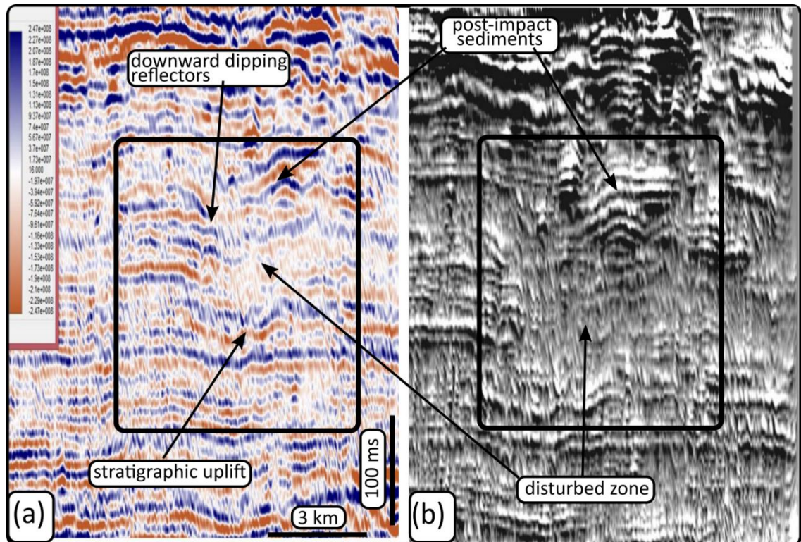
Figure 5.3: Cross-section across the crater with possible deformational features. (a) Amplitude section. (b) Shaded relief section with the crater appearing as low relief zone.
