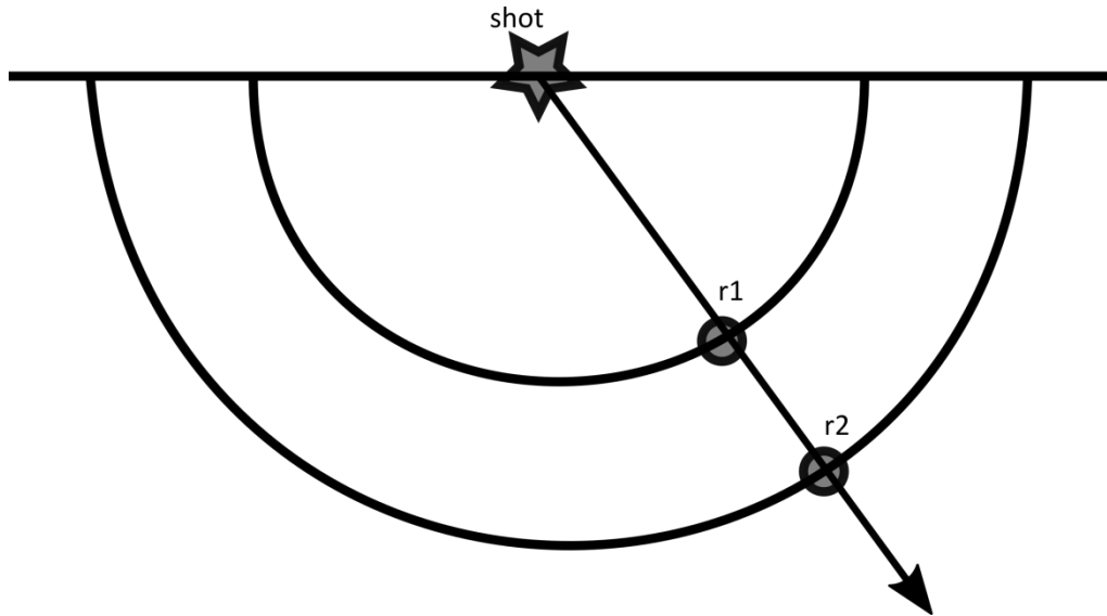
Figure 2.3: Energy losses due to spherical divergence of the seismic wave, r_1 and r_2 are the radial distance from the source (modified after Evans, 1997).
