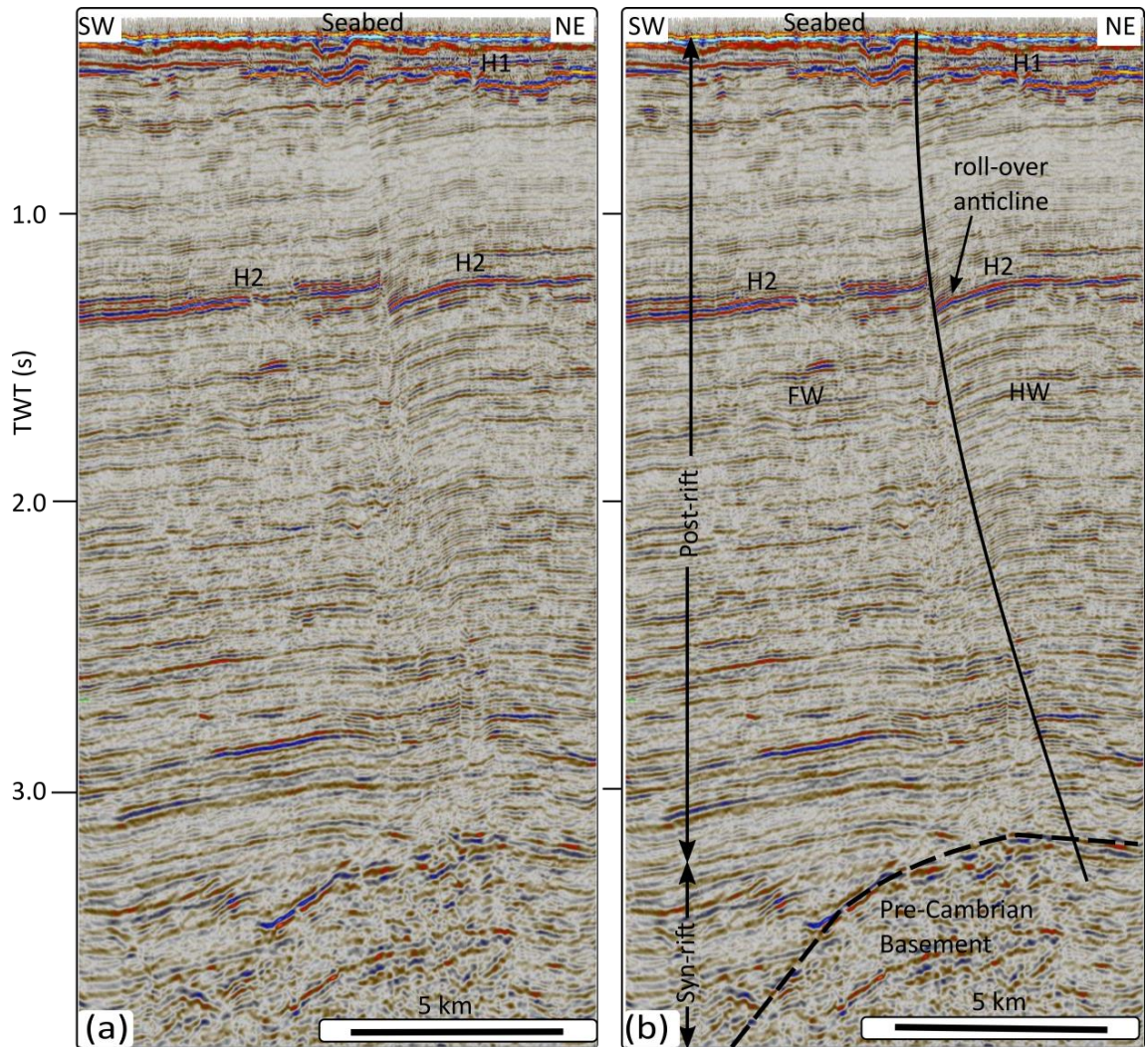
Figure 4.2: Seismic section across the northern segment of the AK Fault. (a) Uninterpreted section (b) Interpreted section showing the penetration of the fault from the underlying basement through the post-rift sediment up to the seabed, and the associated roll-over anticline. H2 and H1 horizons represent the primary reservoir seals of the Cretaceous and the Cenozoic deposits, respectively (Muntingh, 1993; Jungslager, 1999). FW- footwall, HW- hanging wall.
