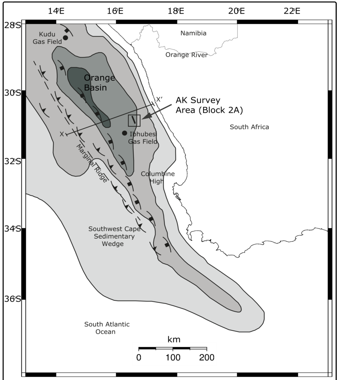
Figure 5.1: Map of the offshore southern Africa, showing the Orange Basin and the AK survey area of Block 2A in the Ibhuesi gas field (modified after Jungslager, 1999)
