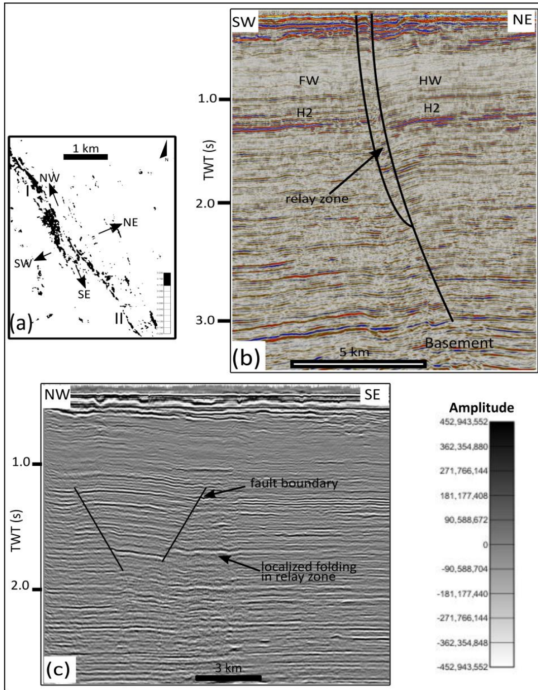
Figure 4.6: Interpreted perpendicular and parallel section across the relay zone between the two overlapping fault segments in the north. (a) Line of cross-sections across the overlapping zone. (b) Perpendicular section to the relay zone showing the linkage of the two overlapping faults at depth. (c) Parallel section with evidence of minor shear deformation revealed by localized folding of sedimentary layers in the relay zone. FW-footwall, HW- hanging wall
