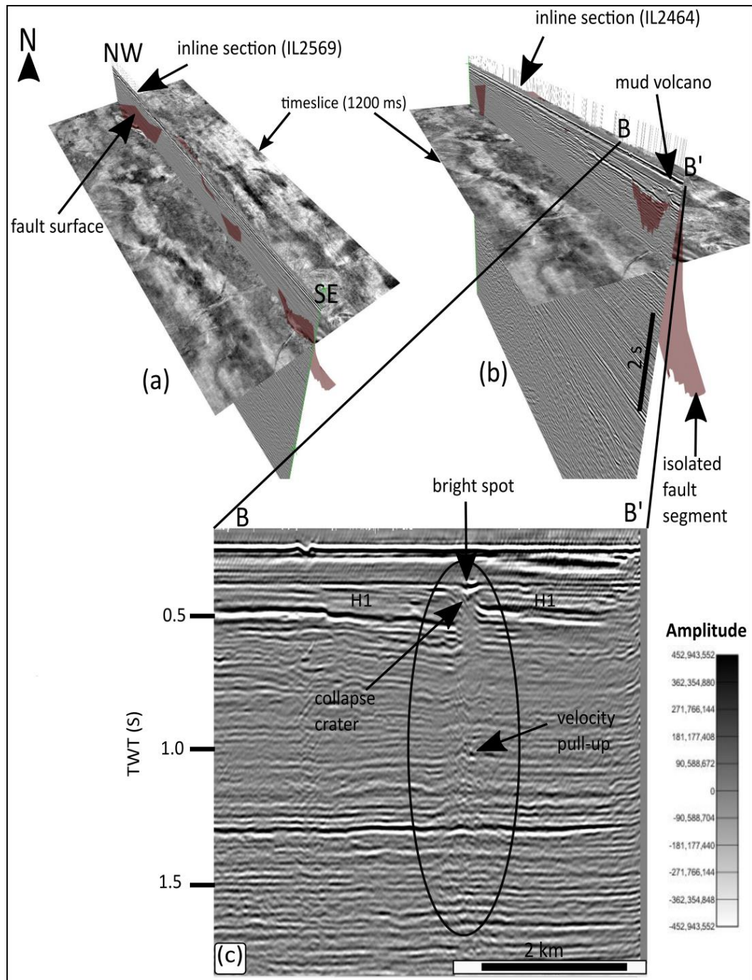
Figure 4.8: Vertical sections investigated for possible fluid leakage features. (a) Inline section along the fault surface and boundaries of the fault segments (see Fig. 9 for details). (b) Mud volcano along the boundary of the isolated curved fault segment in the south. (c) A detailed geometry of the buried mud volcano with associated collapse crater and bright spot above it. Note the displacement of the H1 horizon.
