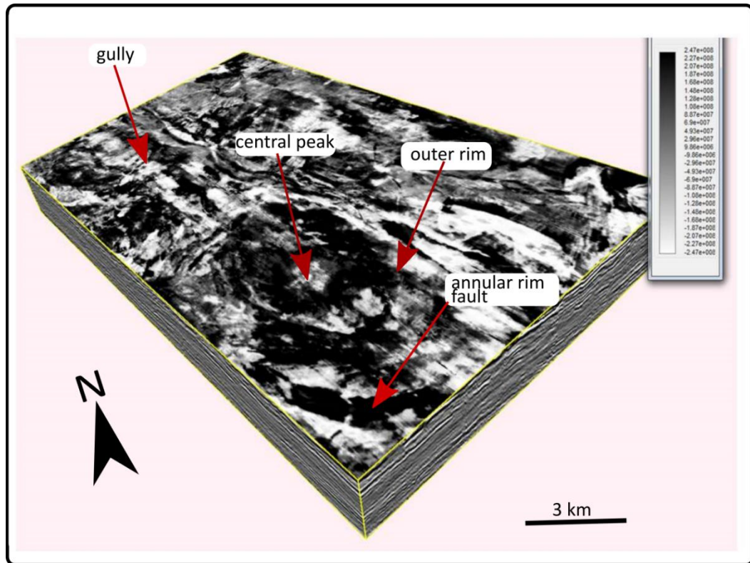
Figure 5.4: Volume rendering at 60-80% opacity showing the detailed geometry of the crater and the associated structures.
