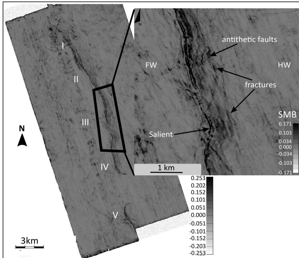
Figure 4.7: A detailed geometry of the fault zone in a semblance slice revealing a salient structure, where two previously isolated faults had linked together, as well as set of subsidiary antithetic faults and fault-parallel extensional fractures that have developed in the fault zone, especially in the hanging wall (HW) side. FW- footwall.
