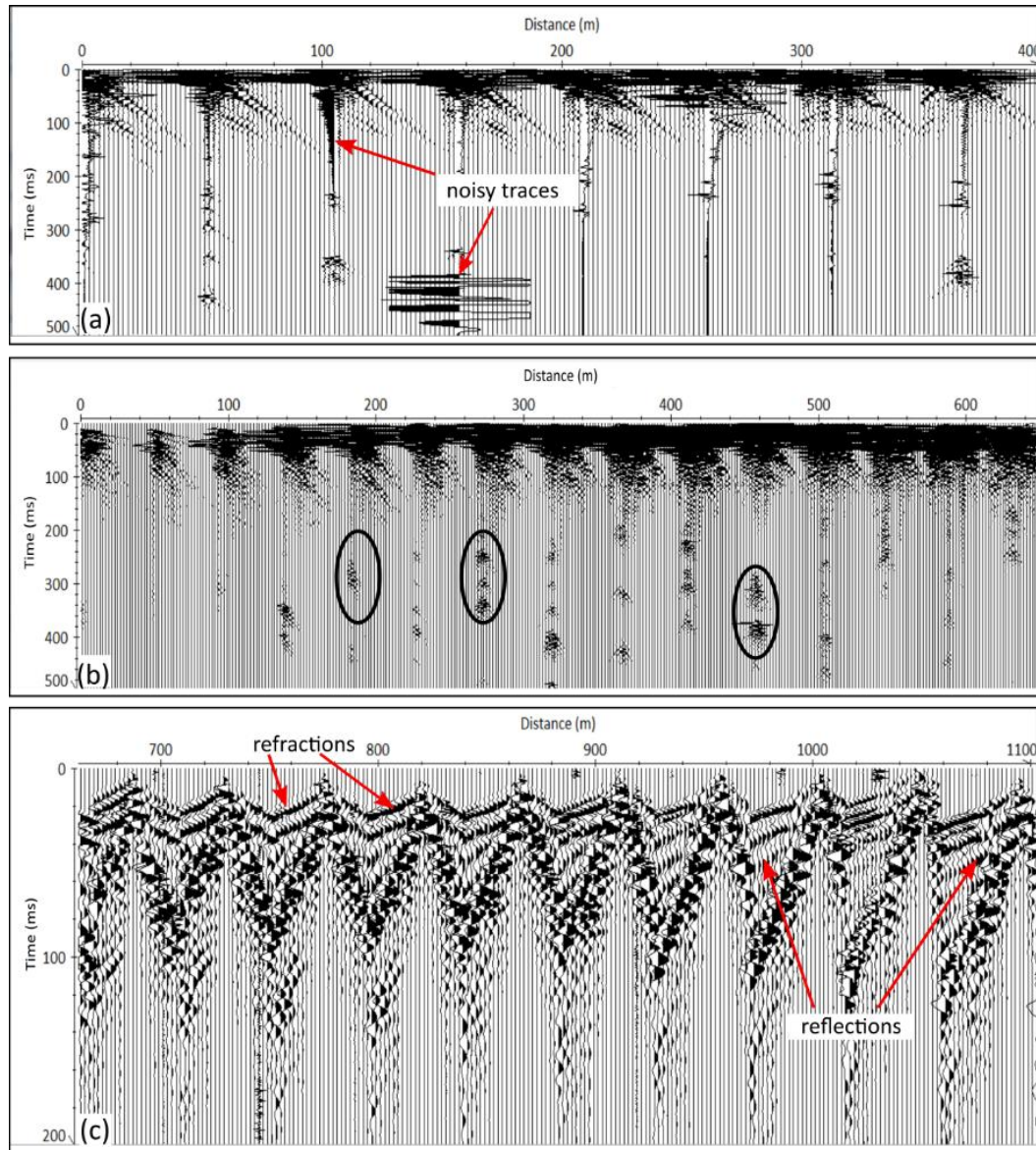
Figure 3.6: Trace editing (a) Raw shot gathers before trace editing and (b) after trace editing. Note the signal duplication due to reverberation of the base plate in the circled region below 200 ms. (c) Typical shot gathers from outside the undermined area showing the data after time-cut, with trace normalized gain applied for display. Note the reflection and refraction events in the raw shot gathers.
