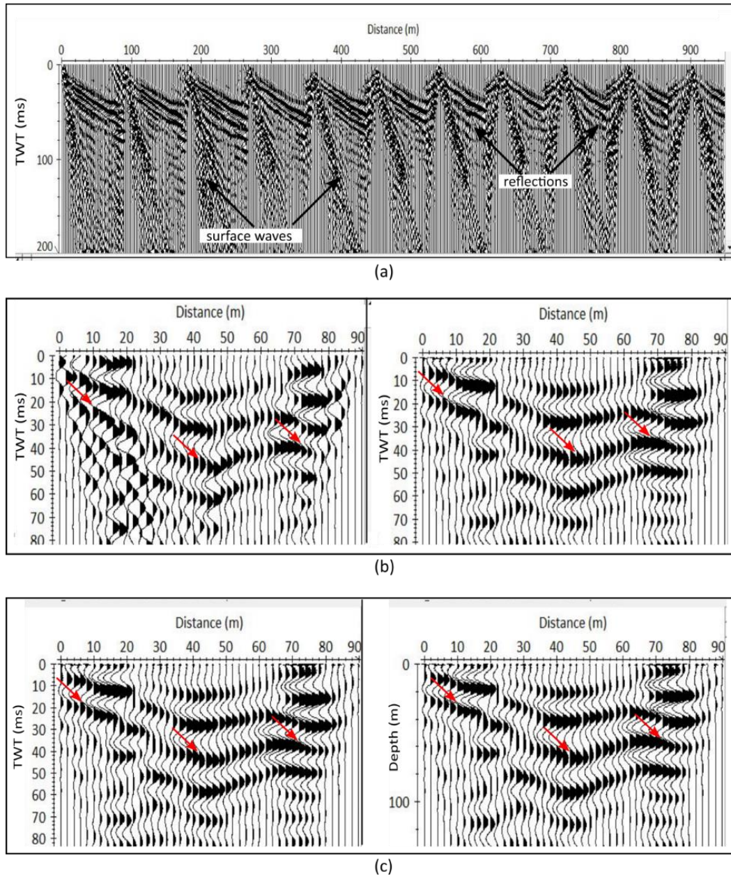
Figure 3.15: (a) Pre-stack shot gathers along LN2 showing visible reflection events after applying a bandpass Butterworth filter. Trace normalized gain is applied for display, (b) Stack and the corresponding time migrated section along LN2 with AGC applied, and (C) Time migrated (with AGC applied) and the corresponding depth section along LN2. The arrow indicates the top of the dolerite layer. Note the dipping of the dolerite layer from approximately 21 ms to about 41 ms.
