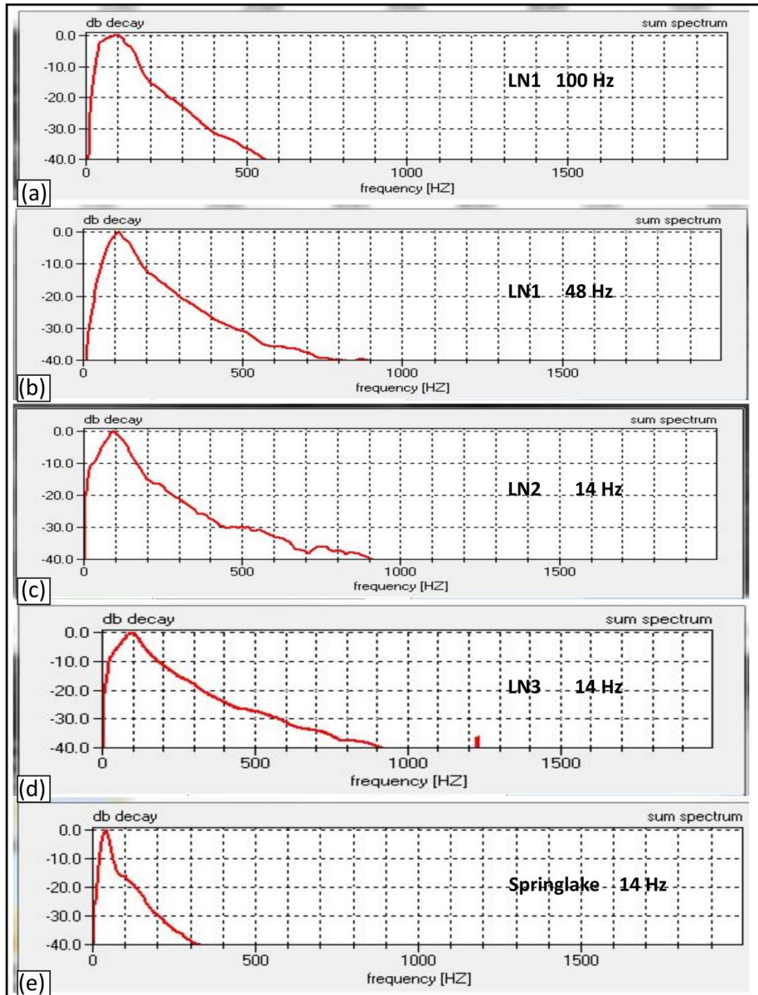
Figure 3.7: Frequency spectrum of the whole dataset acquired along each of the seismic lines. (a) LN1 using the 100 Hz geophone type, (b) LN1 using the 48 Hz geophone type, (c) LN2 using 14 Hz geophone type, (d) LN3 using 14 Hz geophone type, and (e) Springlake using 14 Hz geophone type.
