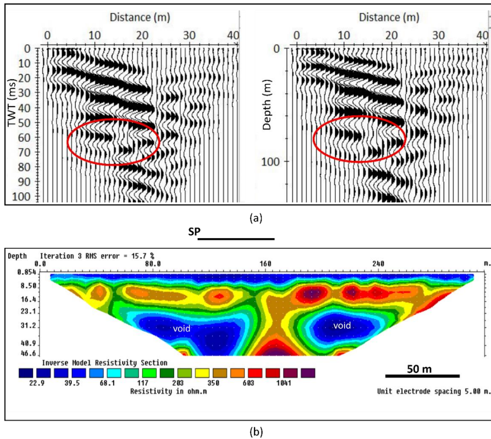
Figure 3.18: (a) The interpreted time migrated and depth section along the Springlake profile showing a disruptive zone probably due to collapsed pillar or void (circled region) (b) The 2D pseudosection from the ERT survey showing voids that probably extend to greater depth. SP indicates the region covered by the seismic line.
