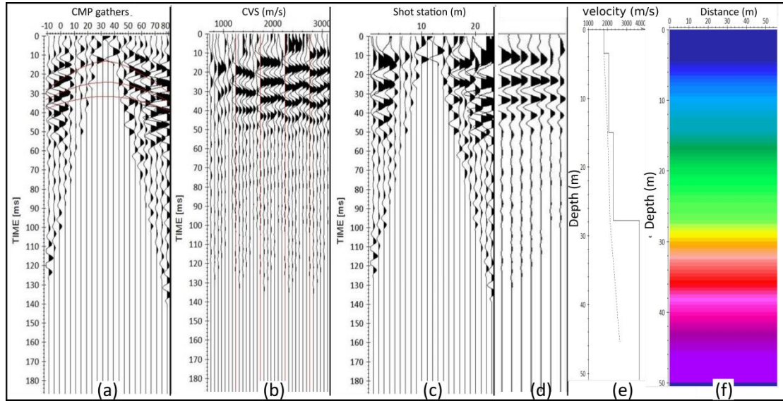
Figure 3.11: Illustration of the CVS analysis (a) Hyperbola fitting conducted on a CMP gather, (b) CVS panels generated using minimum and maximum velocity boundaries of 1000 and 4000 m/s, respectively at a constant velocity increment of 500 m/s, (c) An NMO corrected shot gather, (d) CMP stack displayed for 7 adjacent CMP gathers (e) 1-D velocity model picked from the CVS panels, and (d) The corresponding 2-D velocity model obtained from the stacking velocities that were picked from the CVS panels.
