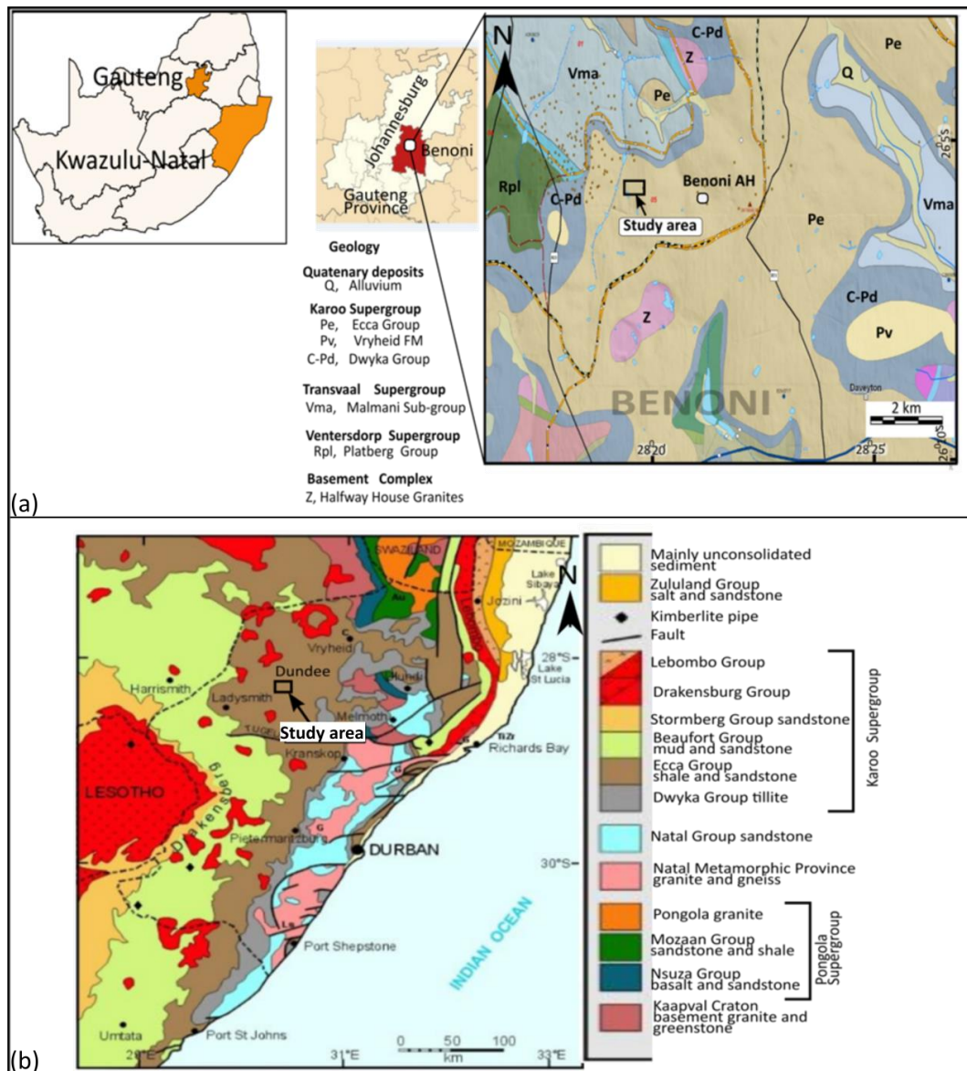
Figure 3.1: Location and regional geological map of Benoni (a) and Kwazulu-Natal (b) showing the two study areas (modified after Department of Water and Sanitation, 2009; Council for Geosciences, 2001).
