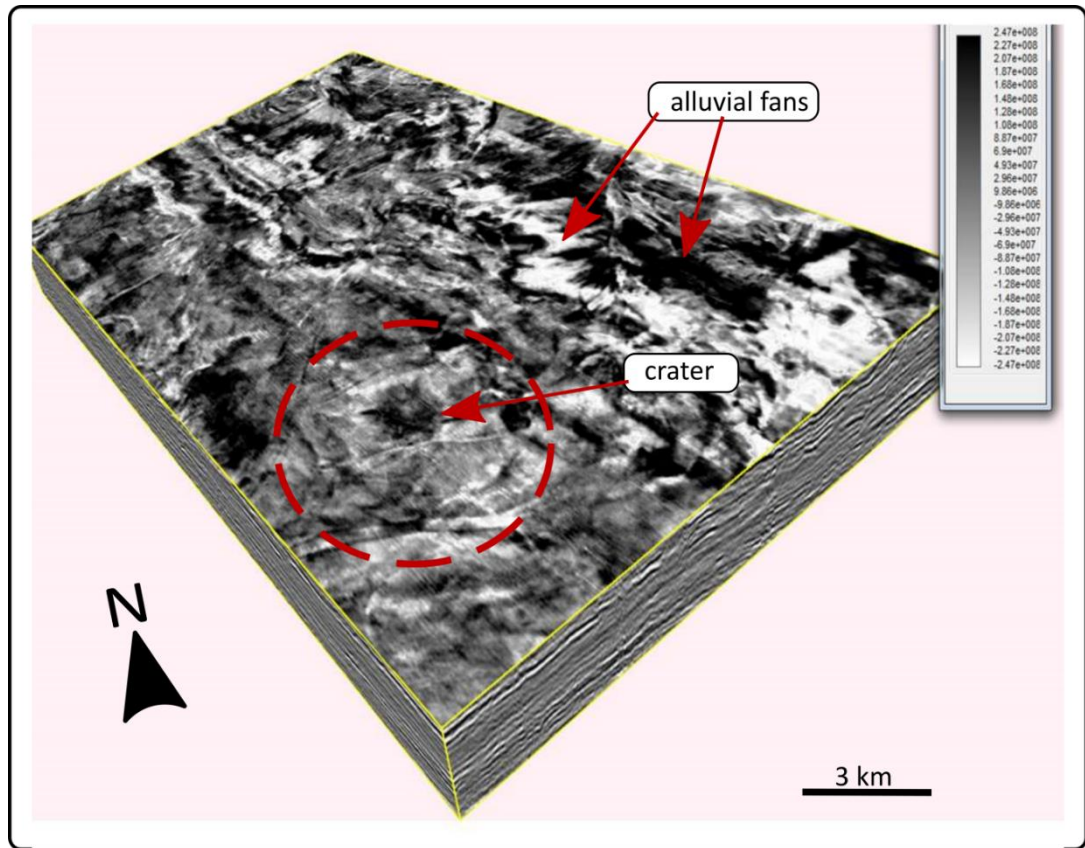
Figure 5.5: Volume rendering at 60-80% opacity showing the crater with the associated sub-marine alluvial fans, which probably suggests its quick burial and eventual preservation.
