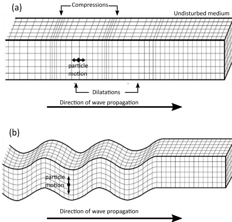
Figure 2.1: Elastic deformations and ground particle motions associated with the passage of body waves. (a) P-wave, (b) S-wave (modified after Kearey et al., 2002).
