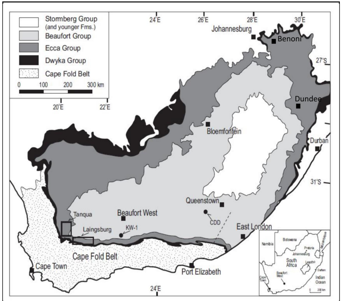
Figure 1.1: The geological map of Karoo Basin showing the different stratigraphic groups (modified from Catuneanu et al., 2005 and Fildani et al., 2009).
