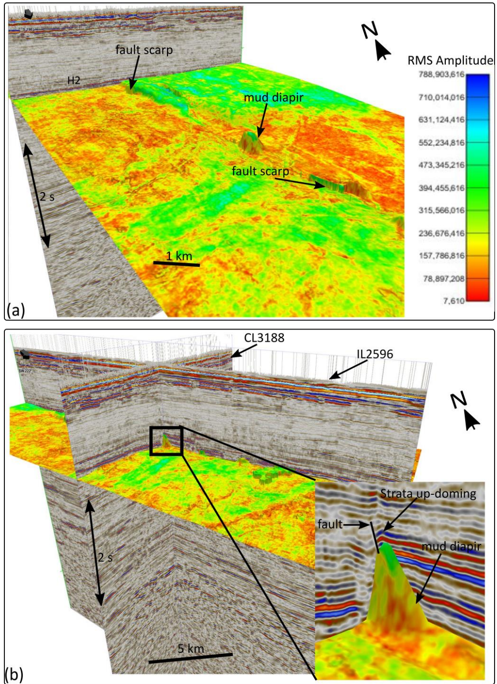
Figure 4.10: (a) A conically-shaped mud diapir at incipient stage along the AK Fault zone, with a base that is aligned parallel to the strike of the fault. (b) Structural deformation above the mud diapir is characterized by up-doming and faulting of the overlying strata.
