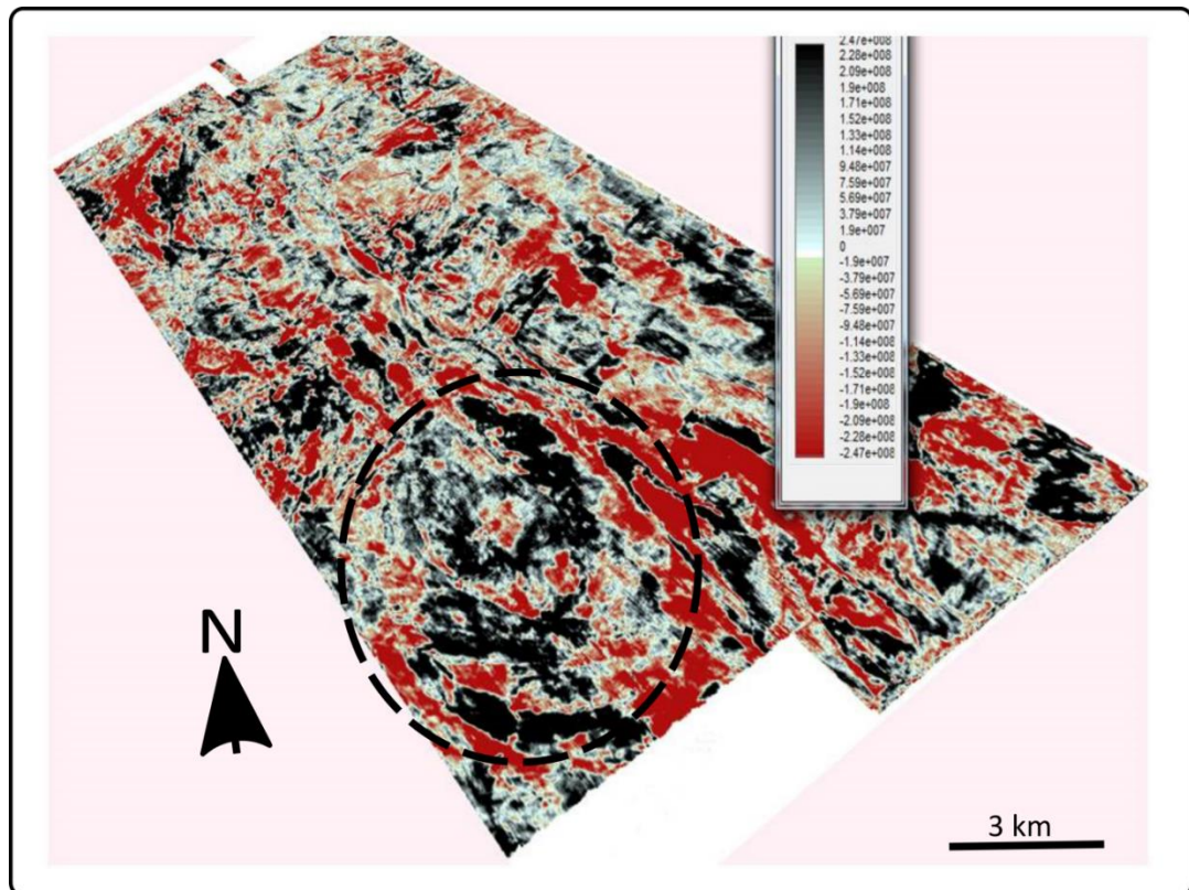
Figure 5.2: A time-slice at 550 ms showing the buried crater in the circled region
