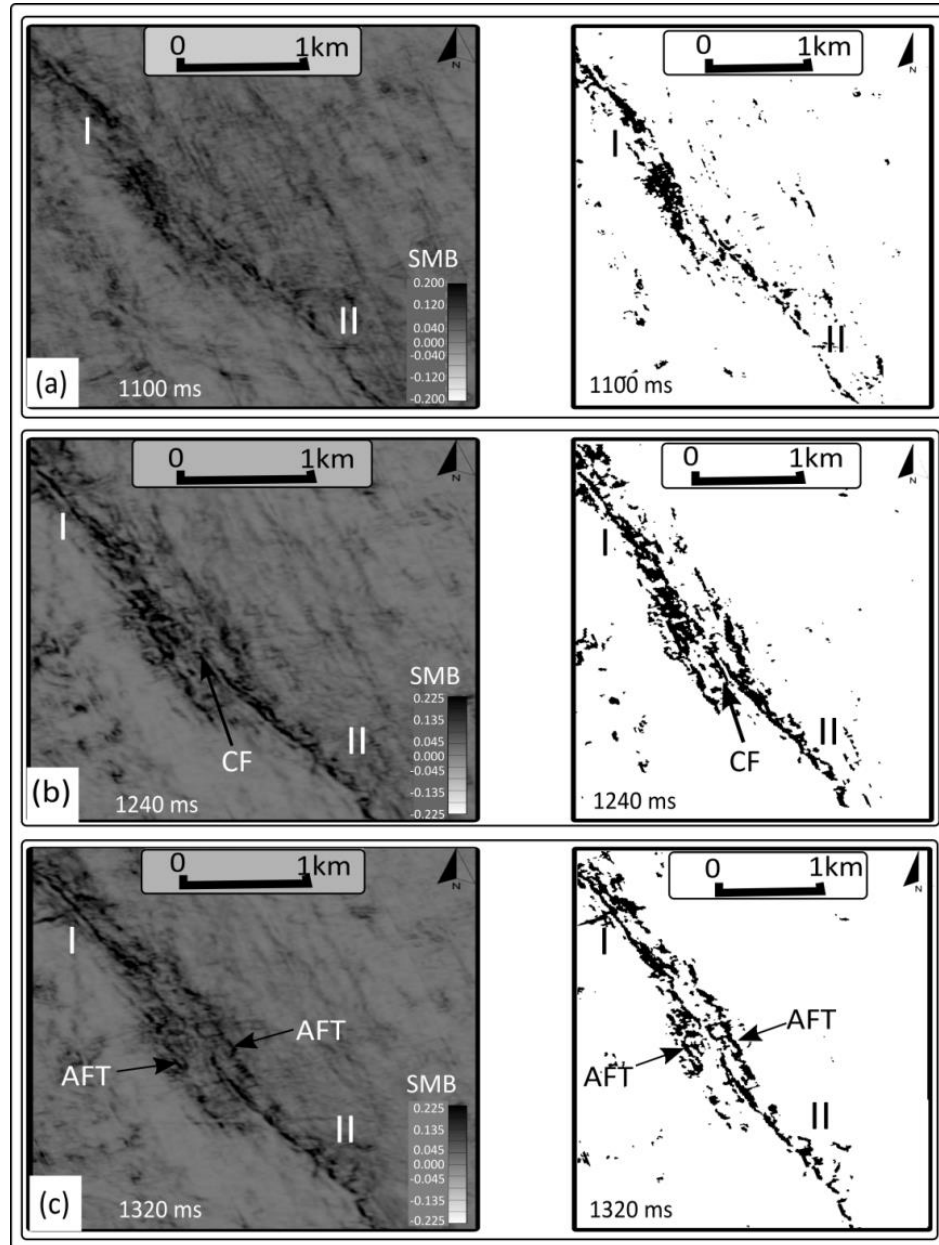
Figure 4.5: Variation in the geometry and map-view dimension of the relay zone between the two overlapping faults I and II with depth. (a) Relay zone at depth of 1100 ms showing the overlap between the two faults I and II. (b) Relay zone breaching at depth of 1240 ms along a central fault (CF) with increase in the map-view dimension. (c) A fully breached relay zone, where the two overlapping faults have abandoned their fault tips (AFT) to link together along the central fault (CF) with no changes in map-view dimension.
