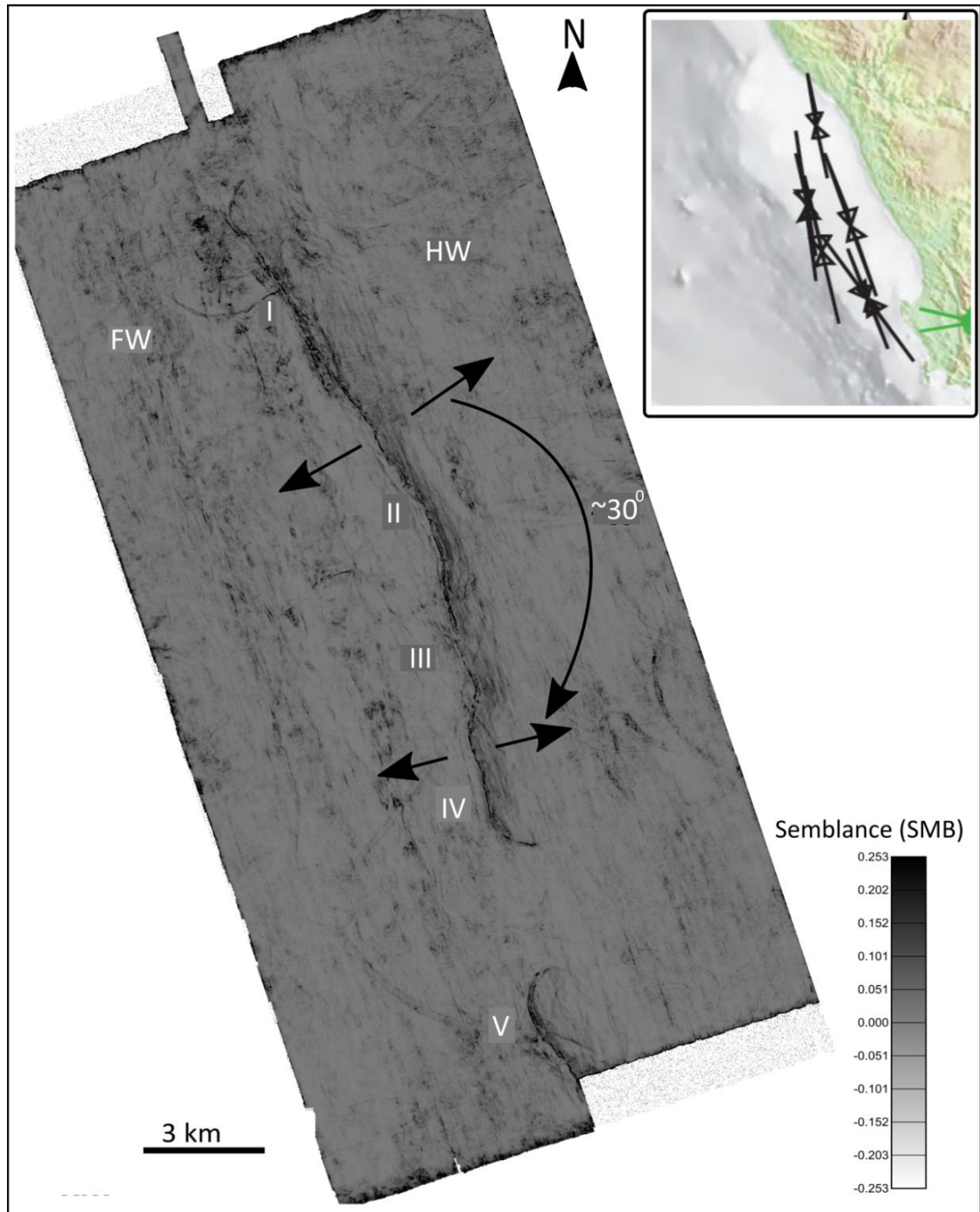
Figure 4.3: Geometry of the AK Fault in semblance slice at 1240 ms showing the different segments of the fault and a possible stress re-orientation through approximately 30^\circ . The inserted map shows the average orientation of the greatest horizontal compressive stress ( SH_{max} ) in the offshore Orange Basin as determined by Logue (2016) and copied from the World Stress Map (Heidbach et al., 2016). FW- footwall. HW- hanging wall.
