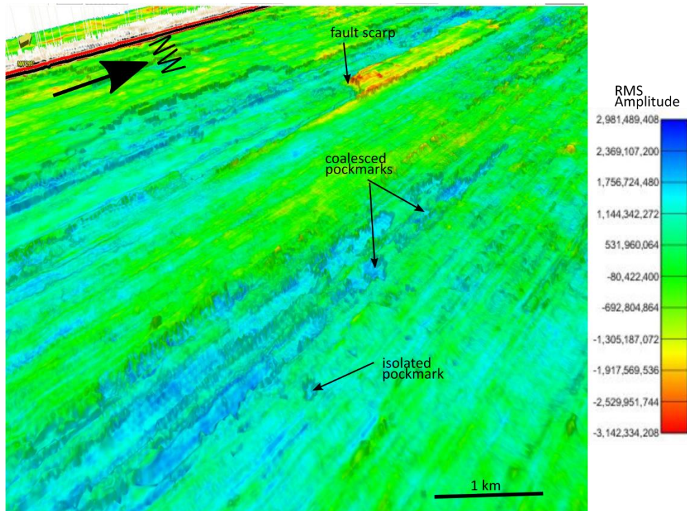
Figure 4.11: A horizon below the seabed showing both the isolated and the coalesced pockmarks. The coalesced pockmarks form elongations in a NW direction that are parallel to the direction of the AK Fault.
