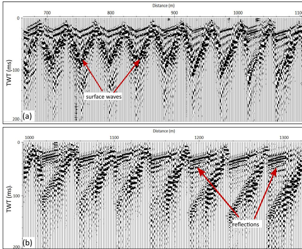
Figure 3.9: Pre-stack shot gathers (a) before and (b) after applying a Butterworth bandpass filter of 85-250 Hz. Note the suppression of the ground-rolls (surface waves) and the enhancement of the reflection events.
