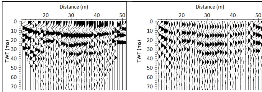
Figure 3.12: An example of a filtered stacked section obtained with the 48 Hz geophone along LN1 showing the stacked data before (left) and after (right) the application of a bandpass frequency of 85-95-140-160 Hz. Note the improvement in the resolution of the reflection events in the images on the right.
